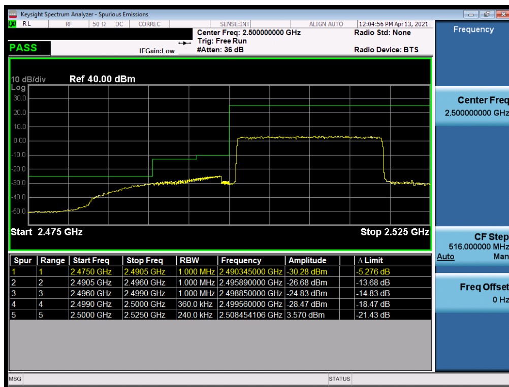
Plot 7-143. Lower ACP Plot (LTE Band 7 - 20MHz QPSK – Full RB)
