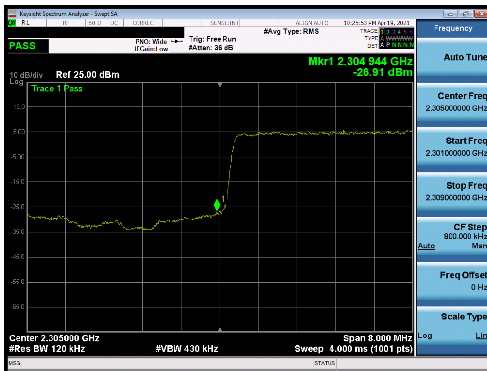
Plot 7-175. Lower Band Edge Plot (NR Band n30 - 10MHz CP-OFDM-QPSK – Full RB)
