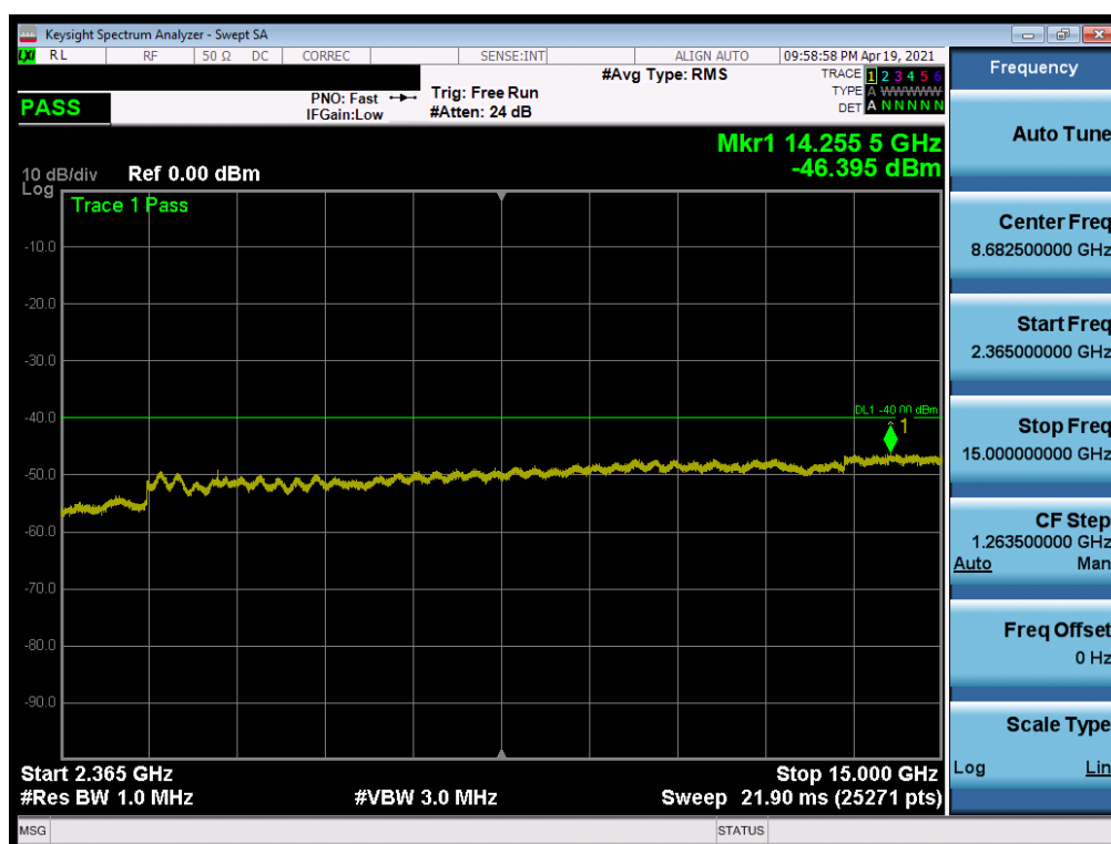
Plot 7-114. Conducted Spurious Plot (NR Band n30 - 10MHz QPSK - RB Size 1, RB Offset 0)
