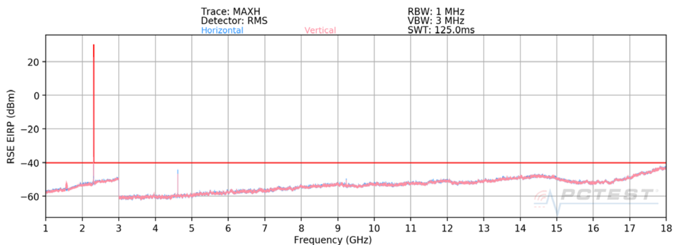
Plot 7-226. Radiated Spurious Plot (LTE Band 30) – Open
