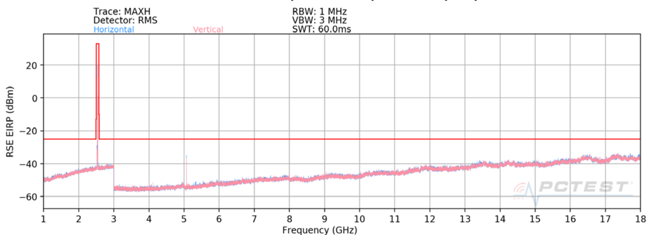
Plot 7-229. Radiated Spurious Plot (LTE Band 7) – Closed
