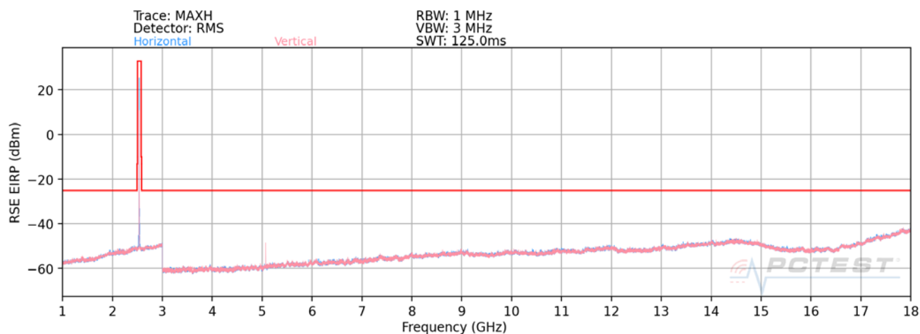
Plot 7-228. Radiated Spurious Plot (LTE Band 7) – Open
