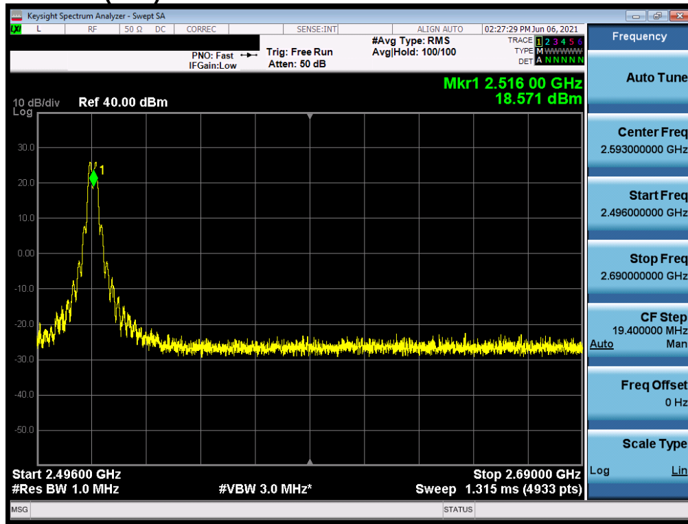
Plot 7-212. Conducted Spurious Plot (ULCA LTE B41(PC2) - 20MHz QPSK - RB Size 1, RB Offset 0 - Low Channel)
