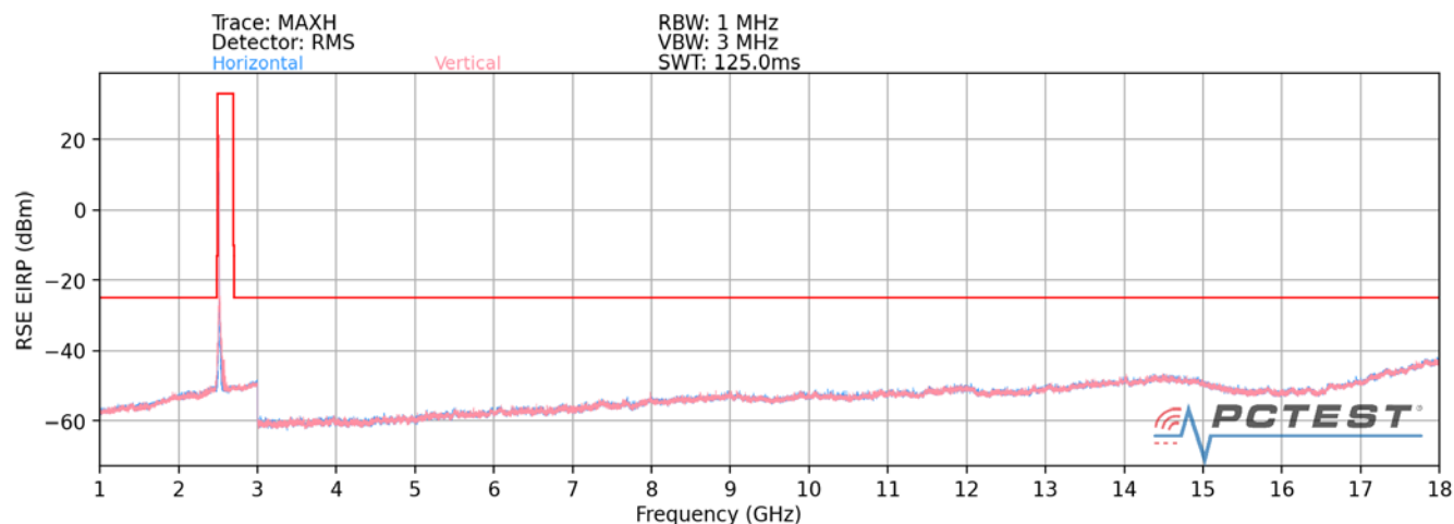
Plot 7-244. Radiated Spurious Plot (ULCA LTE B41(PC2) – Low Channel) – Open
