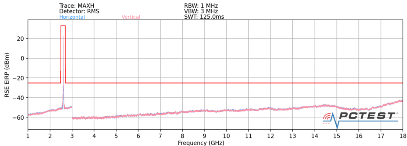
Plot 7-246. Radiated Spurious Plot (ULCA LTE B41(PC2) – Mid Channel) – Open
