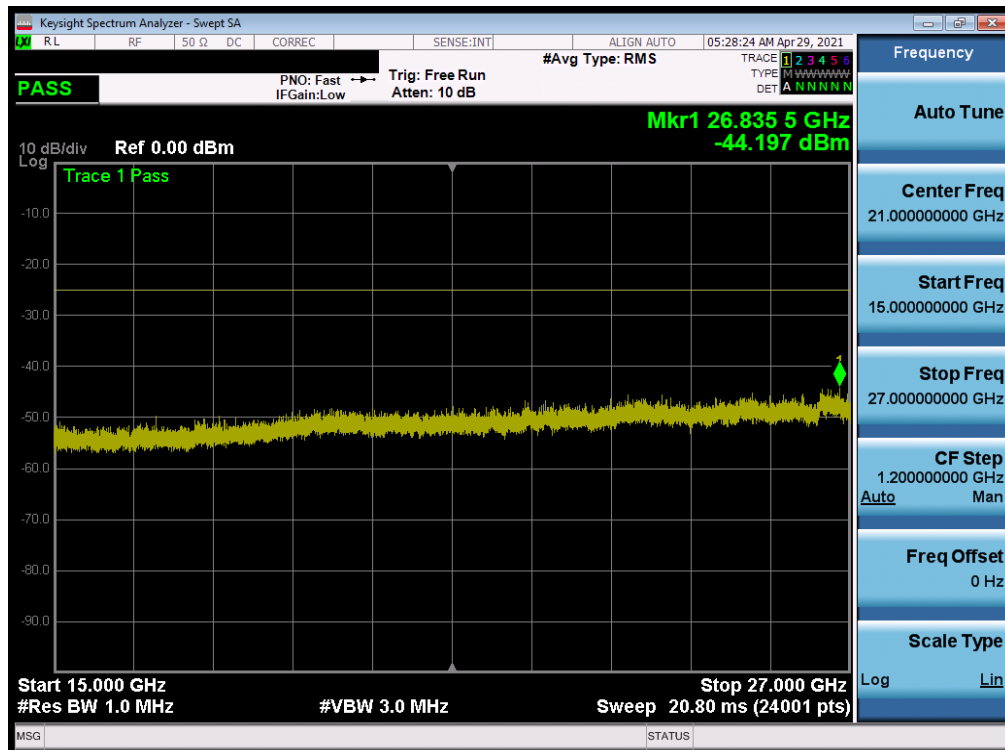
Plot 7-223. Conducted Spurious Plot (ULCA LTE B41(PC2) - 20MHz QPSK - RB Size 1, RB Offset 0 - High Channel)
