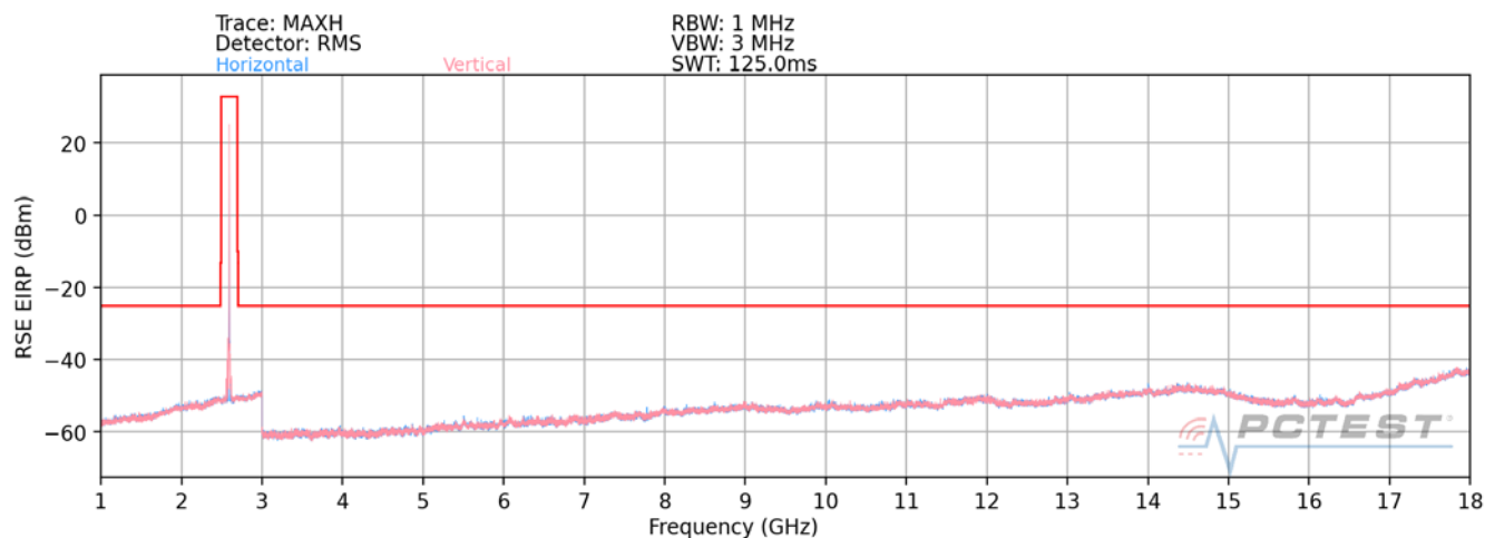
Plot 7-230. Radiated Spurious Plot (LTE Band 41(PC2)) – Open
