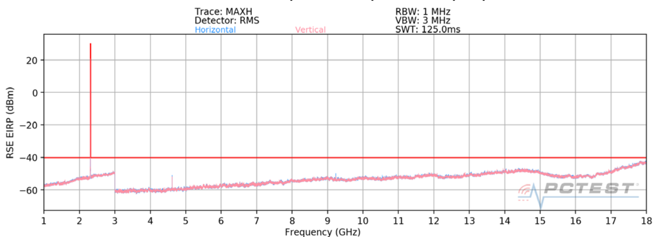
Plot 7-227. Radiated Spurious Plot (LTE Band 30) – Closed
