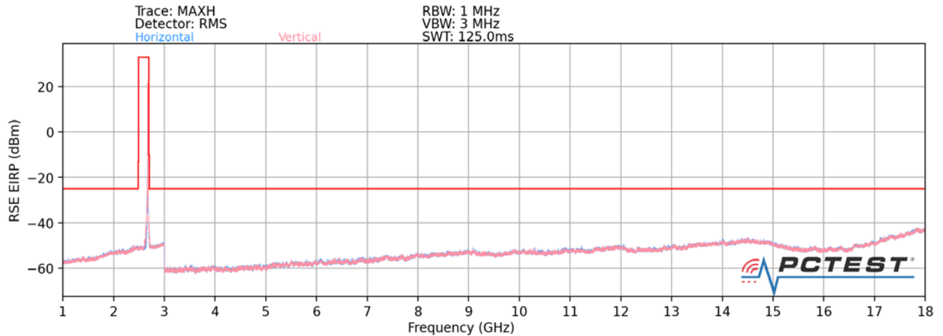
Plot 7-248. Radiated Spurious Plot (ULCA LTE B41(PC2) – High Channel) – Open
