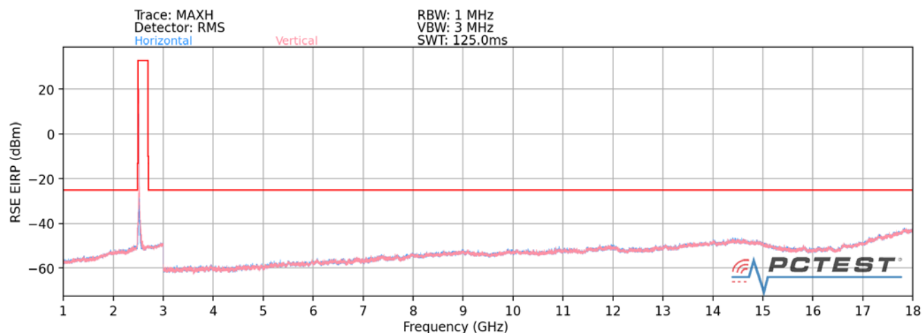
Plot 7-245. Radiated Spurious Plot (ULCA LTE B41(PC2) – Low Channel) – Closed
