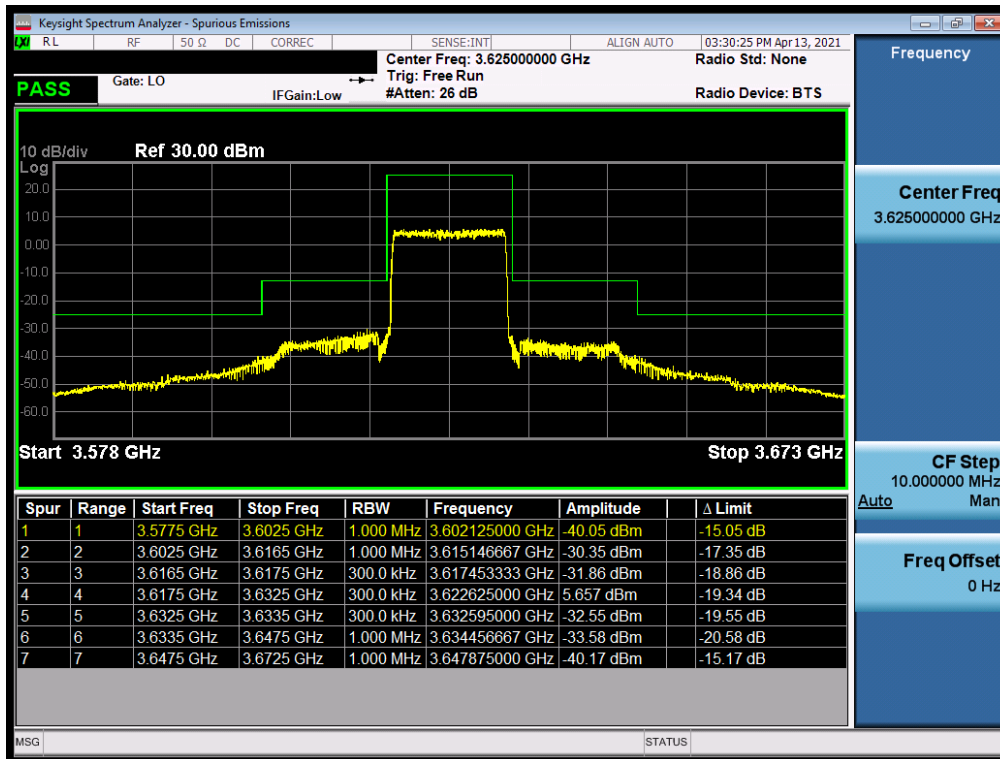
Plot 7-45. Channel Edge Plot (LTE Band 48 - 15MHz QPSK - Mid Channel)
