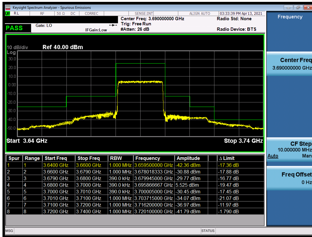
Plot 7-43. Channel Edge Plot (LTE Band 48 - 20MHz QPSK - High Channel)
