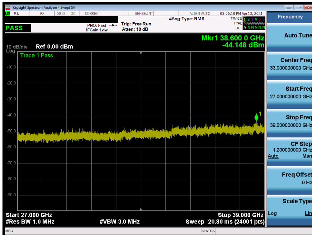
Plot 7-24. Conducted Spurious Plot (LTE Band 48 - 20MHz QPSK - RB Size 1, RB Offset 0 - Mid Channel)
