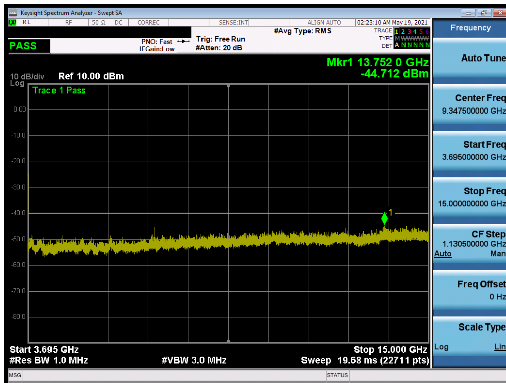
Plot 7-34. Conducted Spurious Plot (ULCA LTE Band 48 - 20+20MHz QPSK - Mid Channel)
