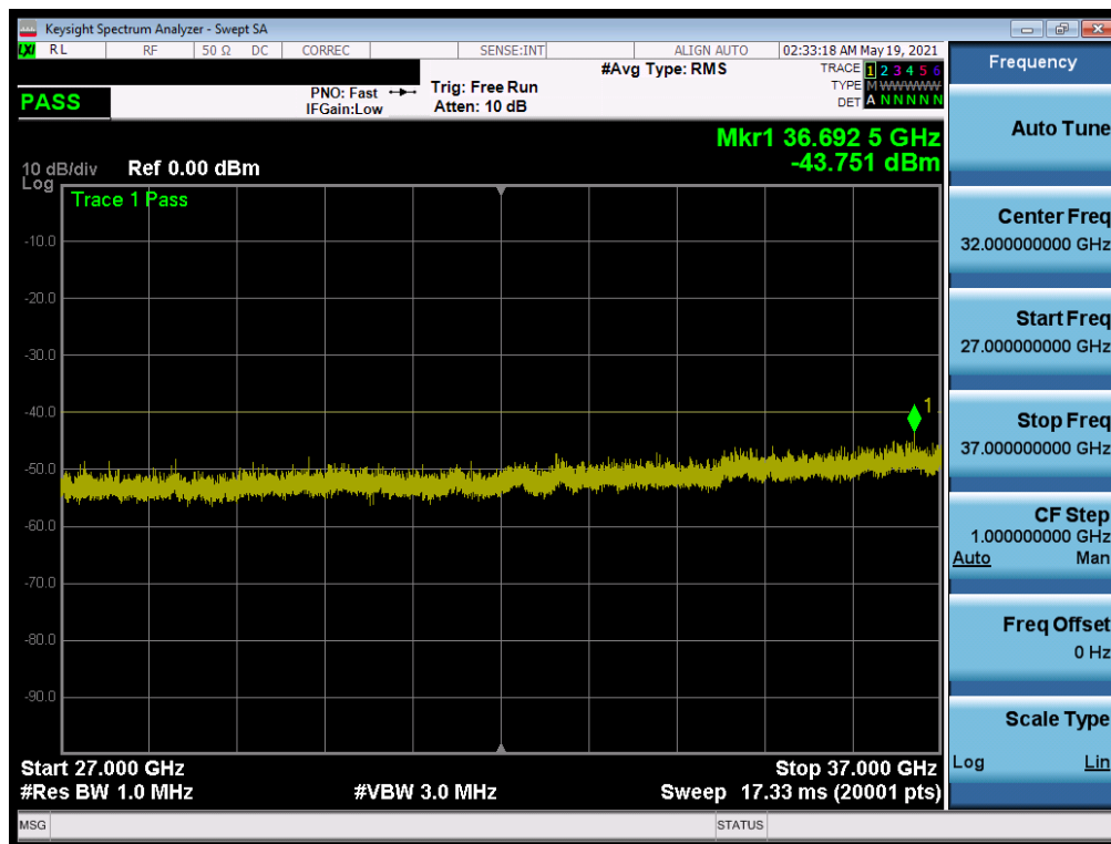
Plot 7-32. Conducted Spurious Plot (ULCA LTE Band 48 - 20+20MHz QPSK - Low Channel)
