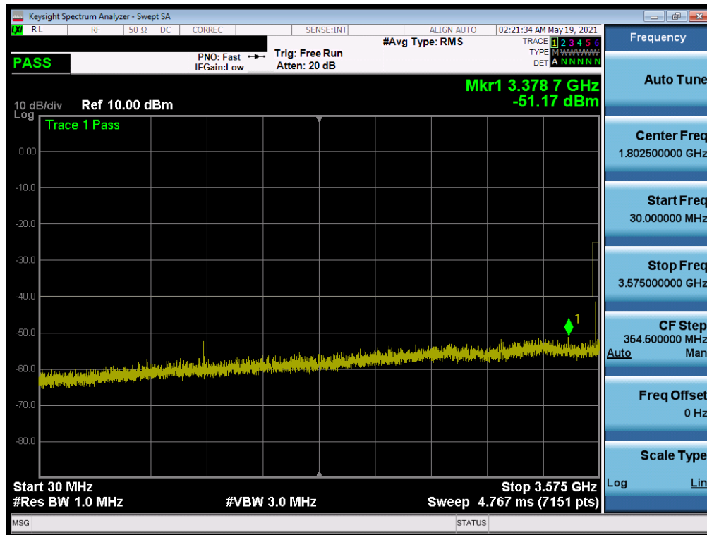
Plot 7-33. Conducted Spurious Plot (ULCA LTE Band 48 - 20+20MHz QPSK - Mid Channel)
