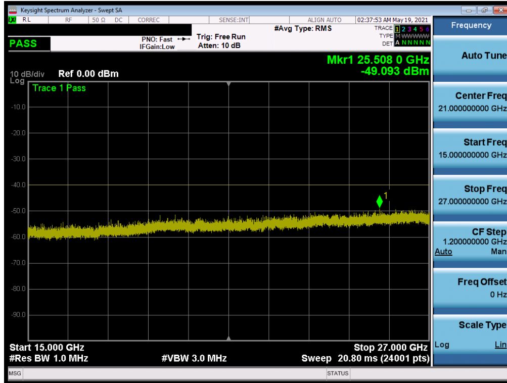
Plot 7-39. Conducted Spurious Plot (ULCA LTE Band 48 - 20+20MHz QPSK - High Channel)
