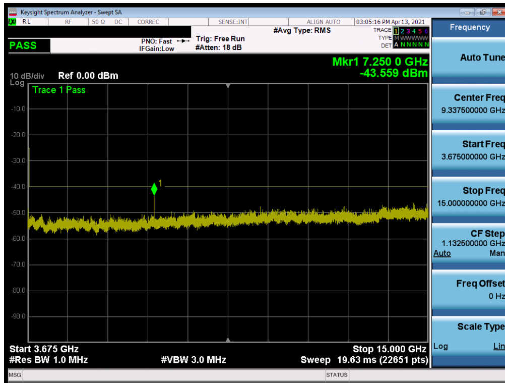
Plot 7-22. Conducted Spurious Plot (LTE Band 48 - 20MHz QPSK - RB Size 1, RB Offset 0 - Mid Channel)
