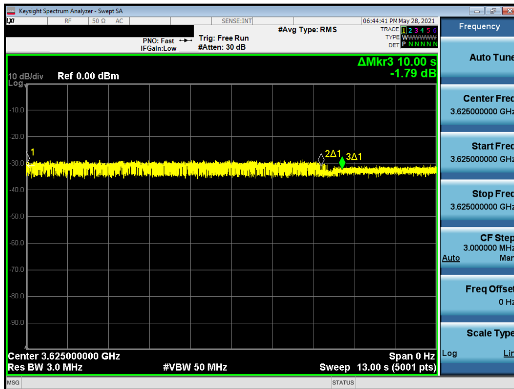
Plot 7-67. Run#1 End User Device Discontinues Operations within 10s
