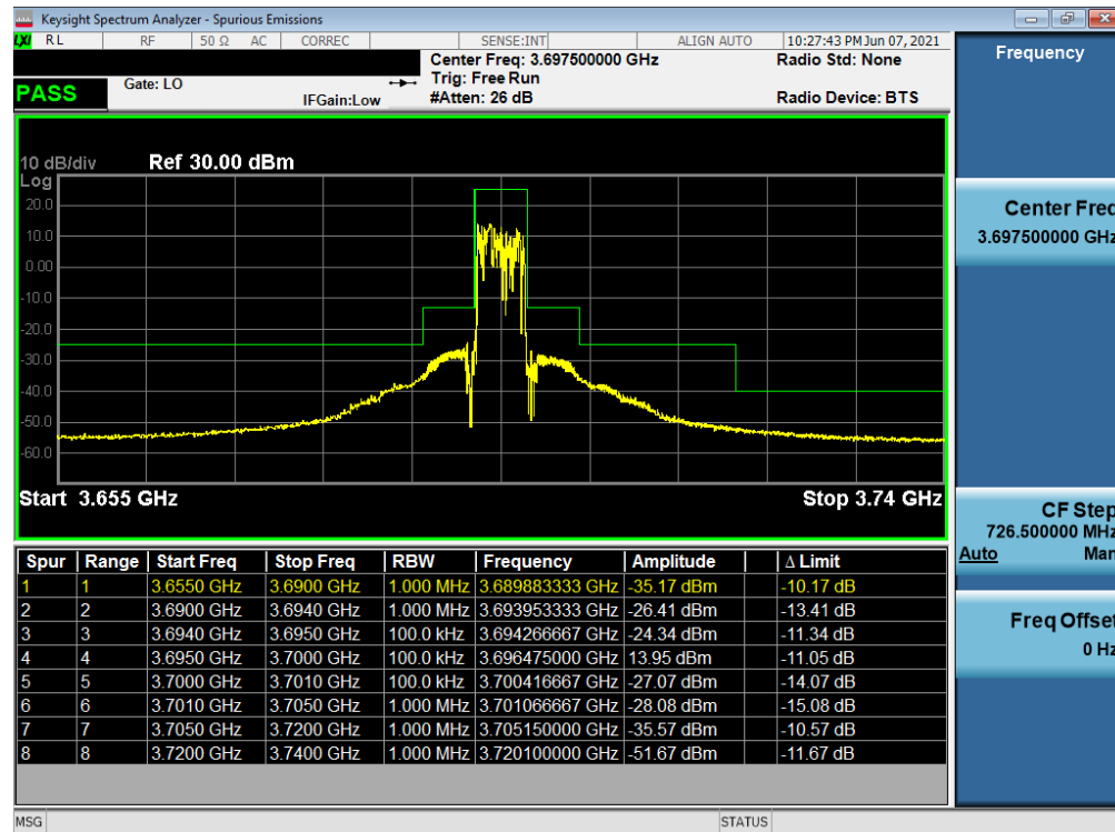
Plot 7-52. Channel Edge Plot (LTE Band 48 - 5MHz QPSK - High Channel)
