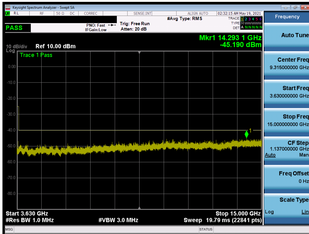
Plot 7-30. Conducted Spurious Plot (ULCA LTE Band 48 - 20+20MHz QPSK - Low Channel)
