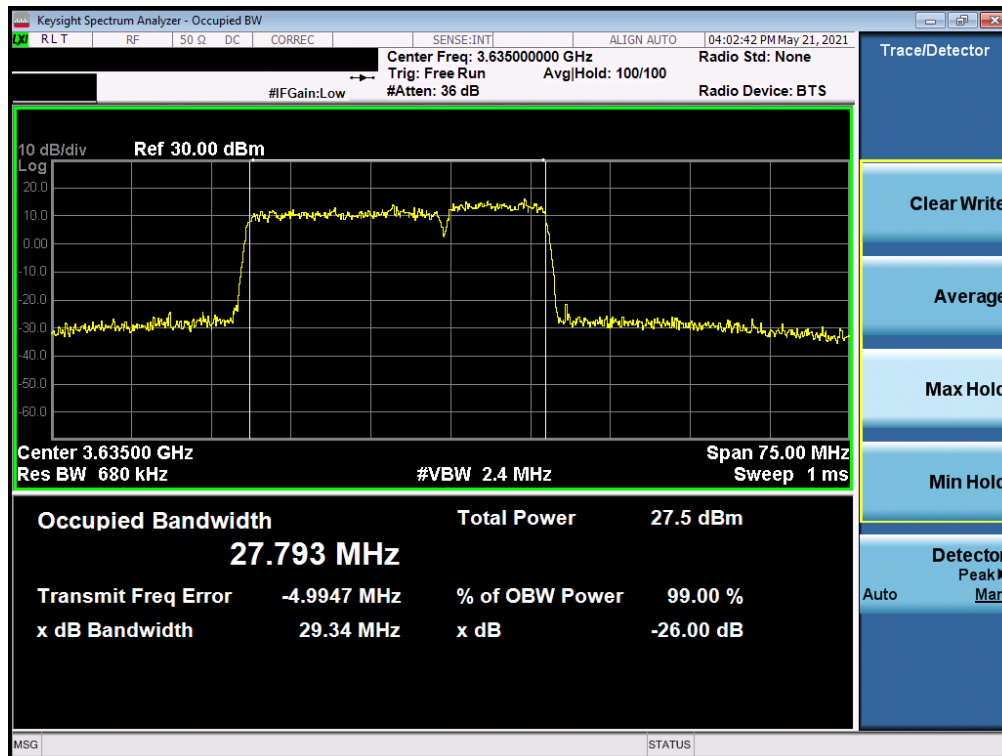
Plot 7-14. Occupied Bandwidth Plot (ULCA LTE Band 48 - 20+10MHz 16-QAM - Full RB Configuration)
