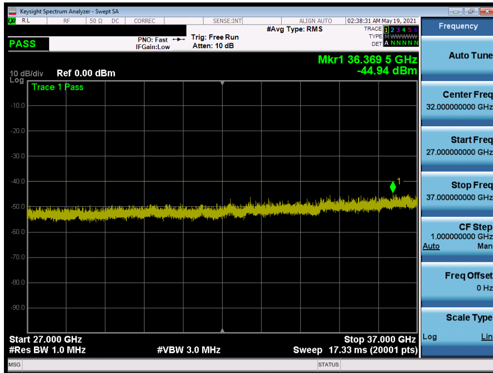
Plot 7-40. Conducted Spurious Plot (ULCA LTE Band 48 - 20+20MHz QPSK - High Channel)
