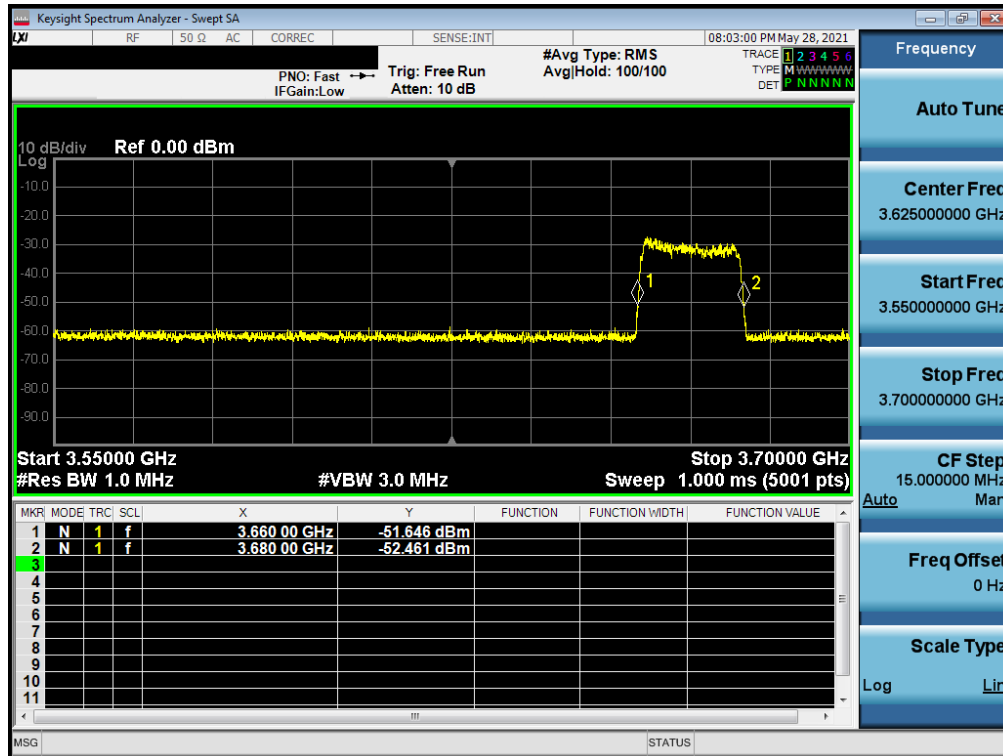
Plot 7-68. Run#2 End User Device Frequency of Operations
