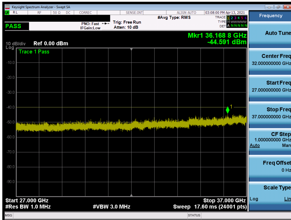
Plot 7-20. Conducted Spurious Plot (LTE Band 48 - 20MHz QPSK - RB Size 1, RB Offset 0 - Low Channel)
