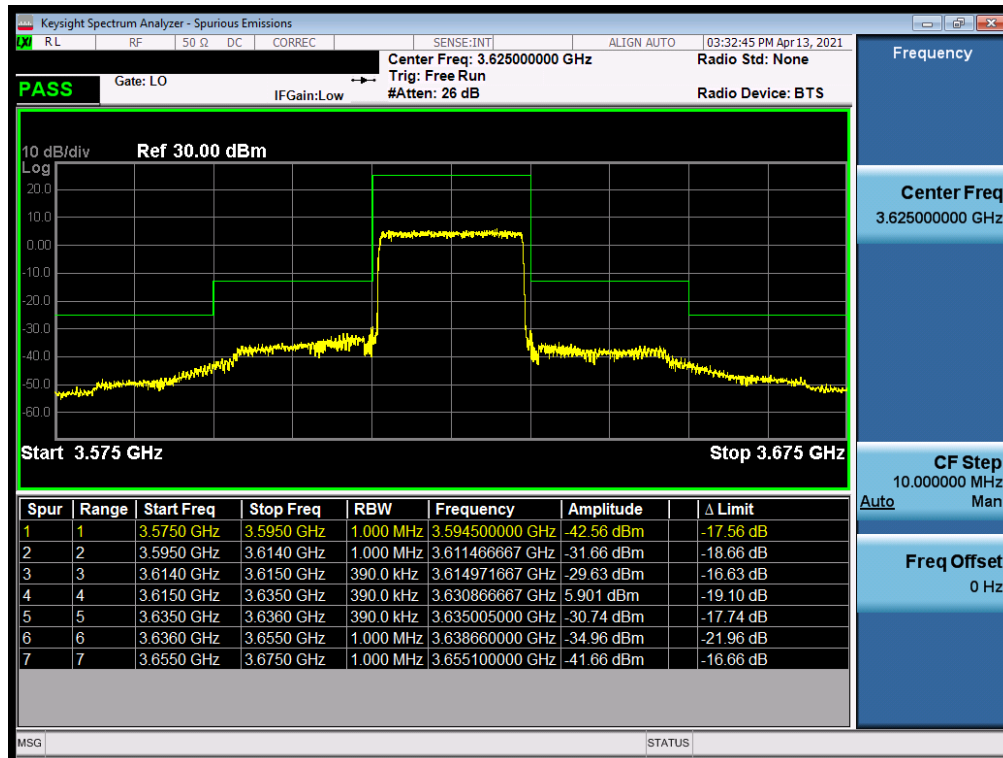
Plot 7-42. Channel Edge Plot (LTE Band 48 - 20MHz QPSK - Mid Channel)
