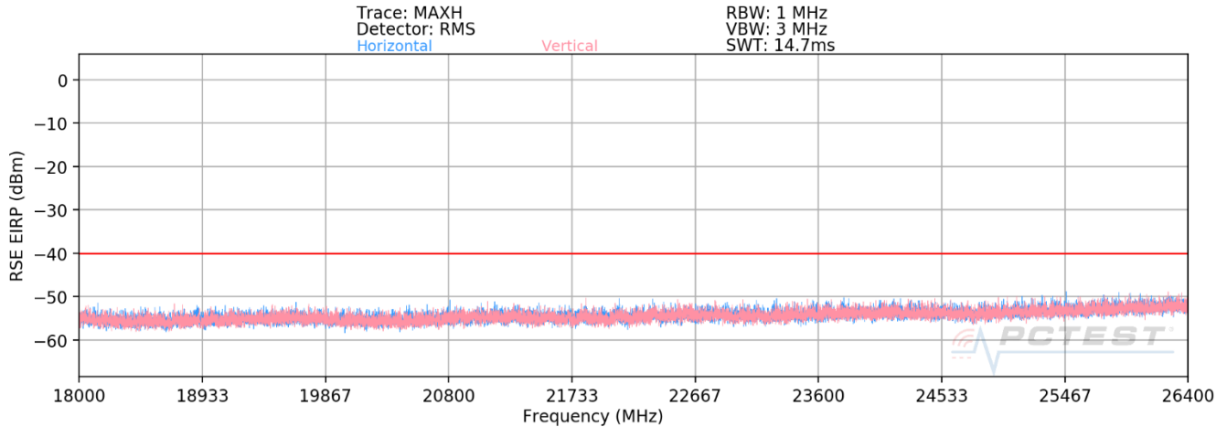
Plot 7-59. Radiated Spurious Plot - 18-26.5 GHz (LTE Band 48) – Closed
