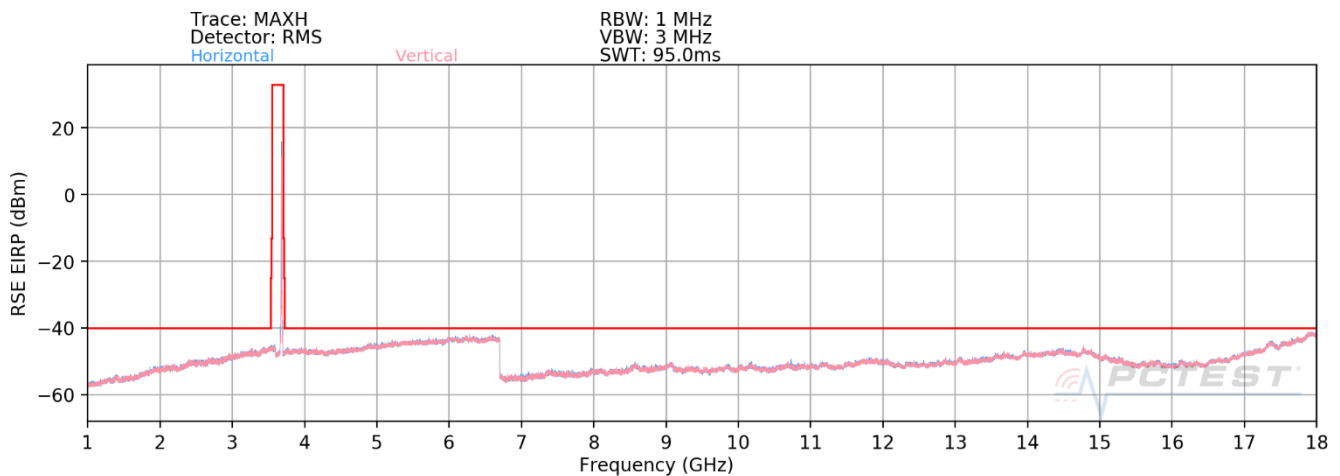
Plot 7-64. Radiated Spurious Plot - 1-18 GHz (ULCA Band 48 – High Channel – PCC/SCC: 1 RB)
