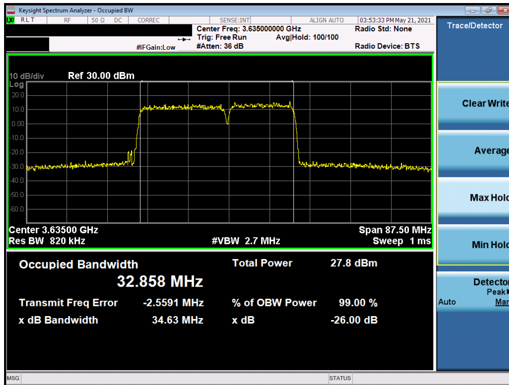
Plot 7-11. Occupied Bandwidth Plot (ULCA LTE Band 48 - 20+15MHz QPSK - Full RB Configuration)
