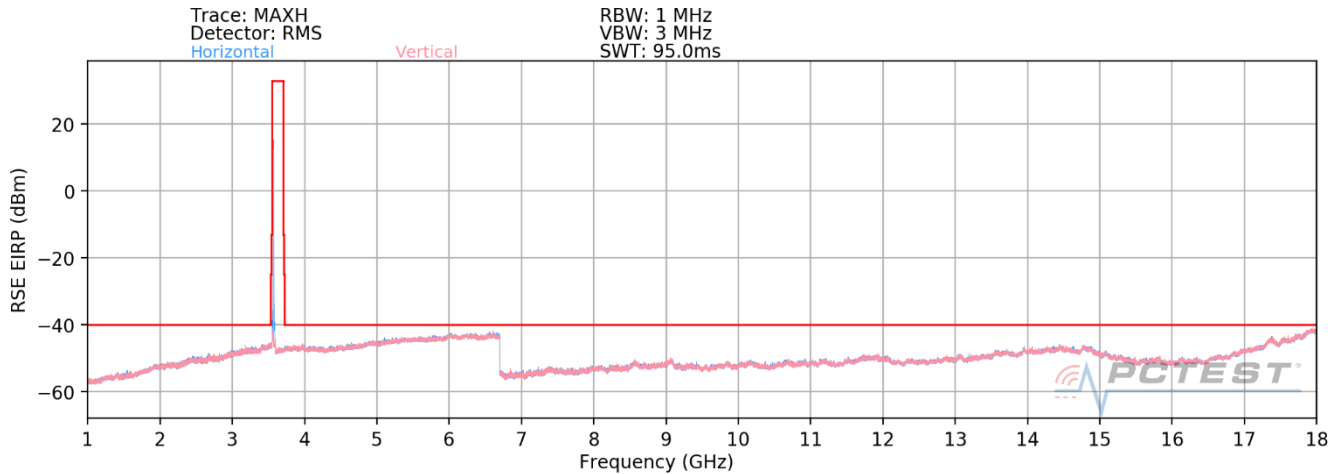
Plot 7-62. Radiated Spurious Plot - 1-18 GHz (ULCA Band 48 – Low Channel – PCC/SCC: 1 RB)
