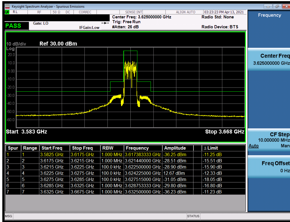
Plot 7-51. Channel Edge Plot (LTE Band 48 - 5MHz QPSK - Mid Channel)
