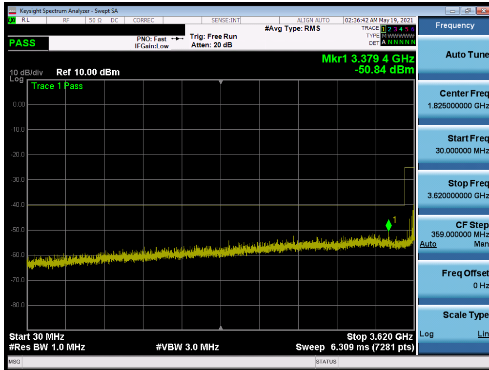
Plot 7-37. Conducted Spurious Plot (ULCA LTE Band 48 - 20+20MHz QPSK - High Channel)
