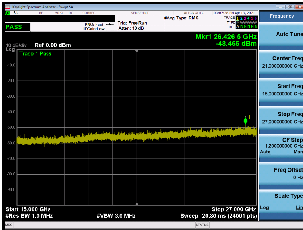
Plot 7-19. Conducted Spurious Plot (LTE Band 48 - 20MHz QPSK - RB Size 1, RB Offset 0 - Low Channel)
