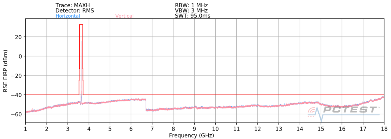
Plot 7-63. Radiated Spurious Plot - 1-18 GHz (ULCA Band 48 – Mid Channel – PCC/SCC: 1 RB)
