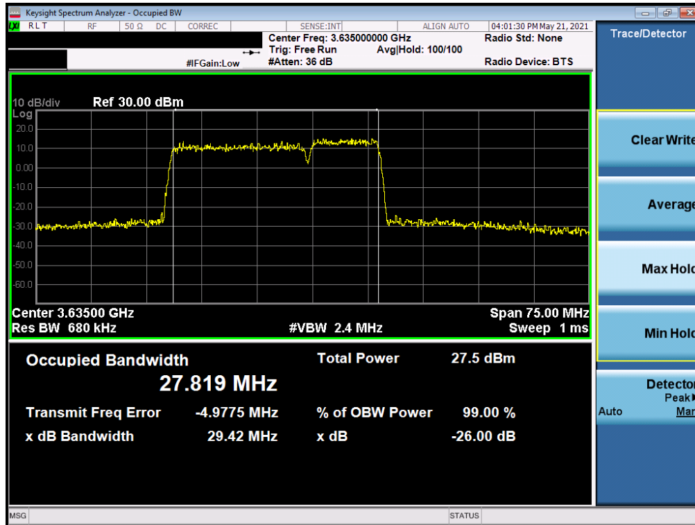
Plot 7-13. Occupied Bandwidth Plot (ULCA LTE Band 48 - 20+10MHz QPSK - Full RB Configuration)
