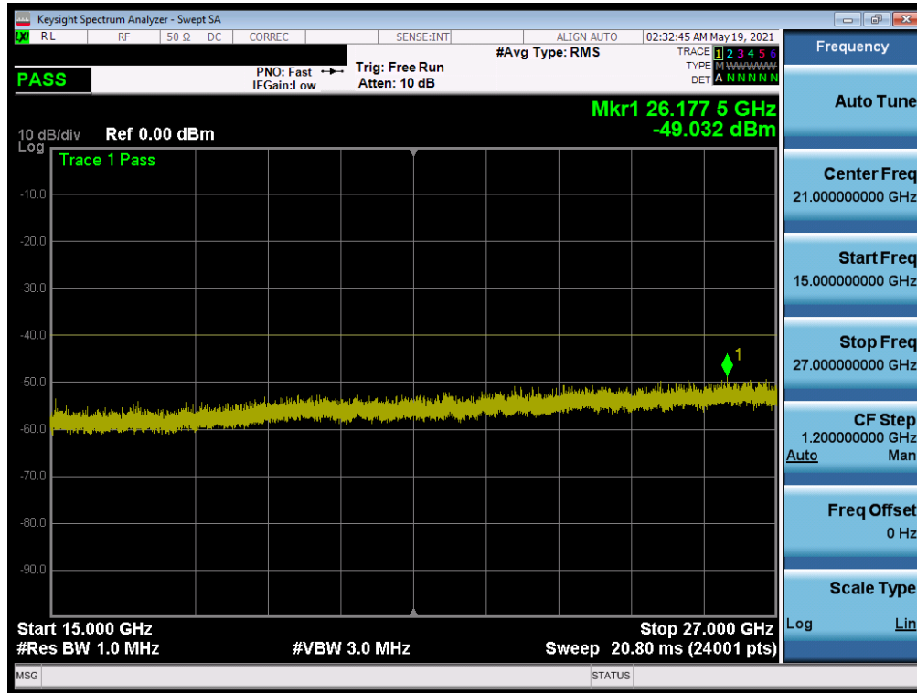
Plot 7-31. Conducted Spurious Plot (ULCA LTE Band 48 - 20+20MHz QPSK - Low Channel)
