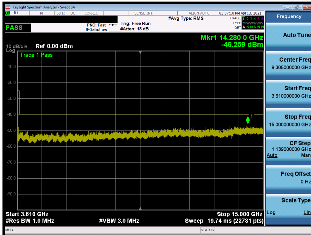
Plot 7-18. Conducted Spurious Plot (LTE Band 48 - 20MHz QPSK - RB Size 1, RB Offset 0 - Low Channel)
