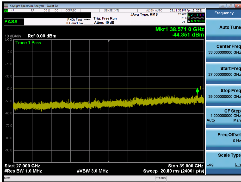
Plot 7-28. Conducted Spurious Plot (LTE Band 48 - 20MHz QPSK - RB Size 1, RB Offset 0 - High Channel)
