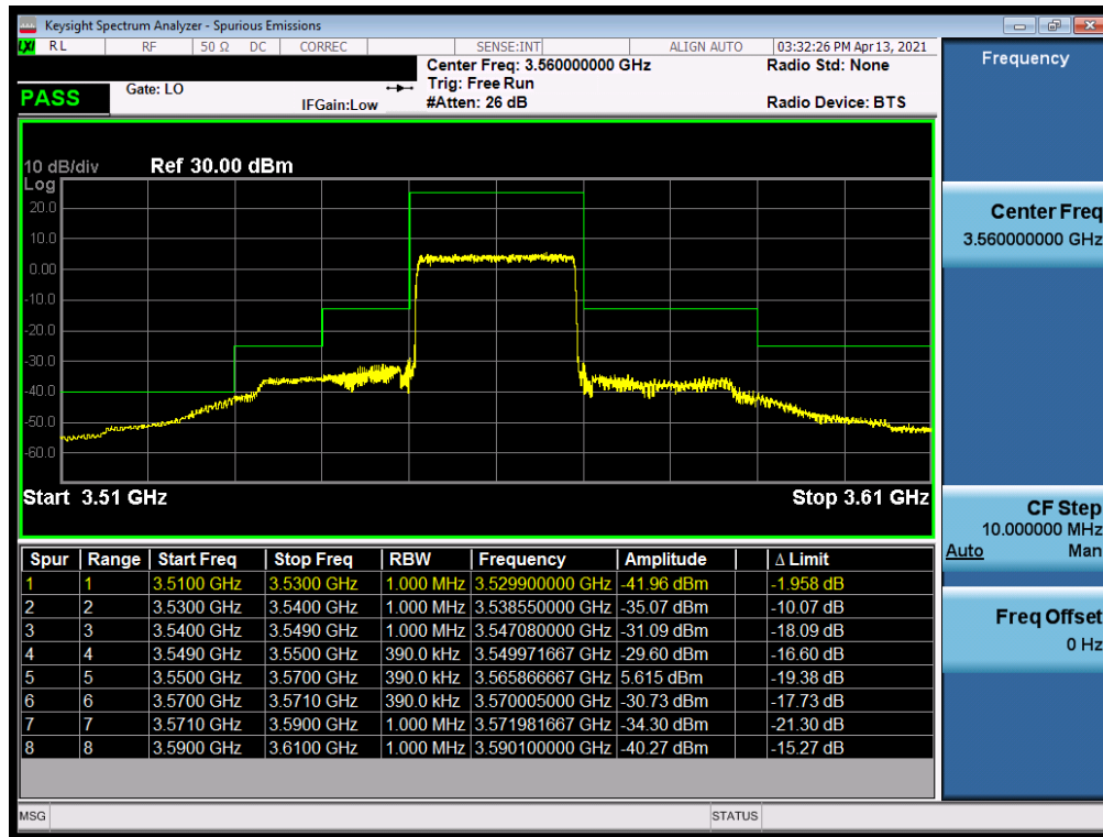
Plot 7-41. Channel Edge Plot (LTE Band 48 - 20MHz QPSK - Low Channel)
