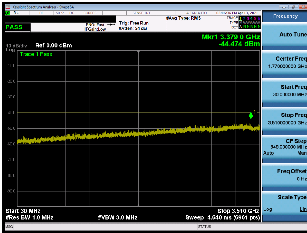
Plot 7-17. Conducted Spurious Plot (LTE Band 48 - 20MHz QPSK - RB Size 1, RB Offset 0 - Low Channel)
