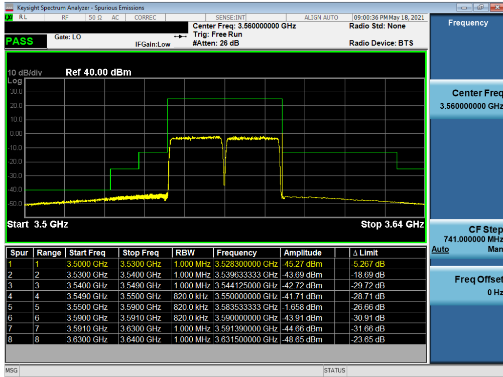
Plot 7-53. Channel Edge Plot (LTE Band 48 – 20+20MHz QPSK - Low Channel)
