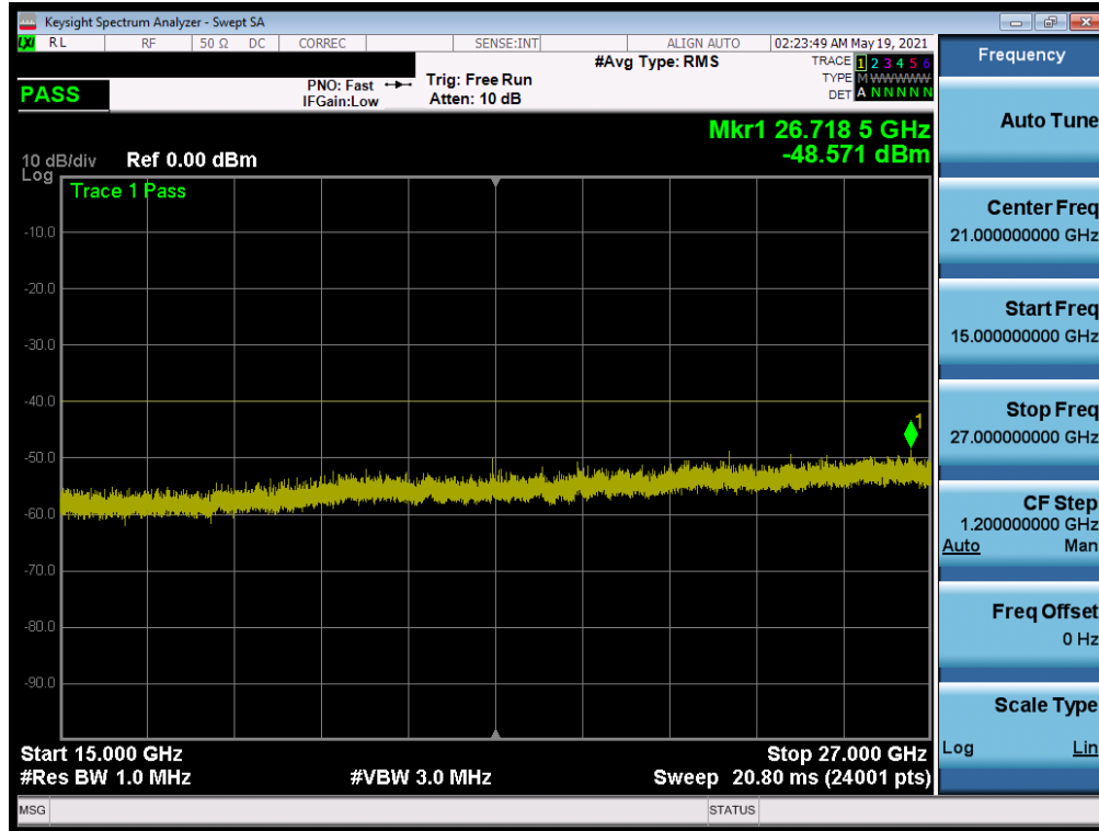
Plot 7-35. Conducted Spurious Plot (ULCA LTE Band 48 - 20+20MHz QPSK - Mid Channel)
