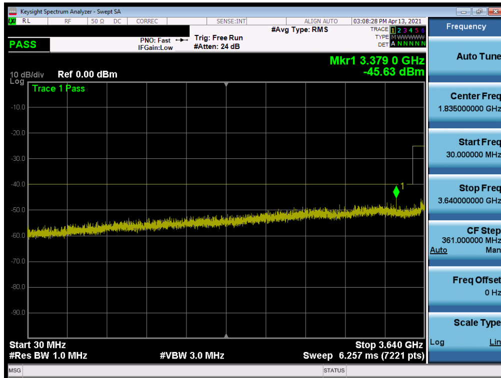
Plot 7-25. Conducted Spurious Plot (LTE Band 48 - 20MHz QPSK - RB Size 1, RB Offset 0 - High Channel)
