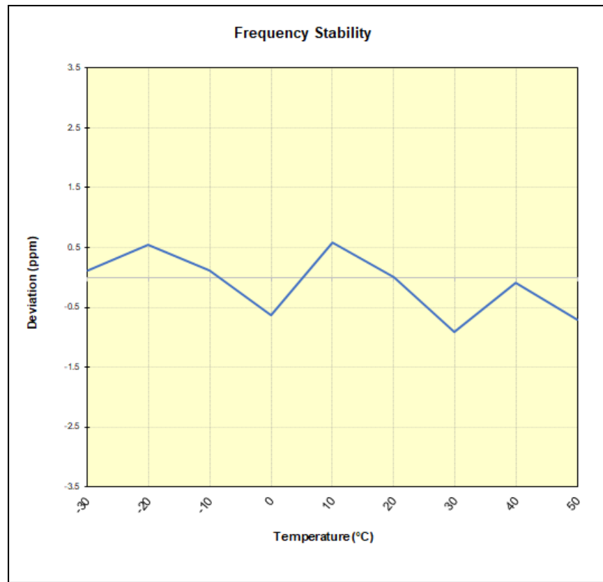
Plot 7-65. LTE Band 48 Frequency Stability Chart
