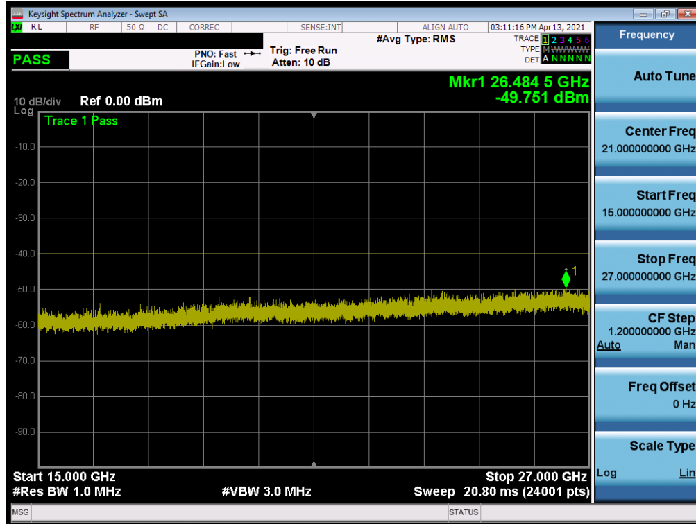
Plot 7-27. Conducted Spurious Plot (LTE Band 48 - 20MHz QPSK - RB Size 1, RB Offset 0 - High Channel)
