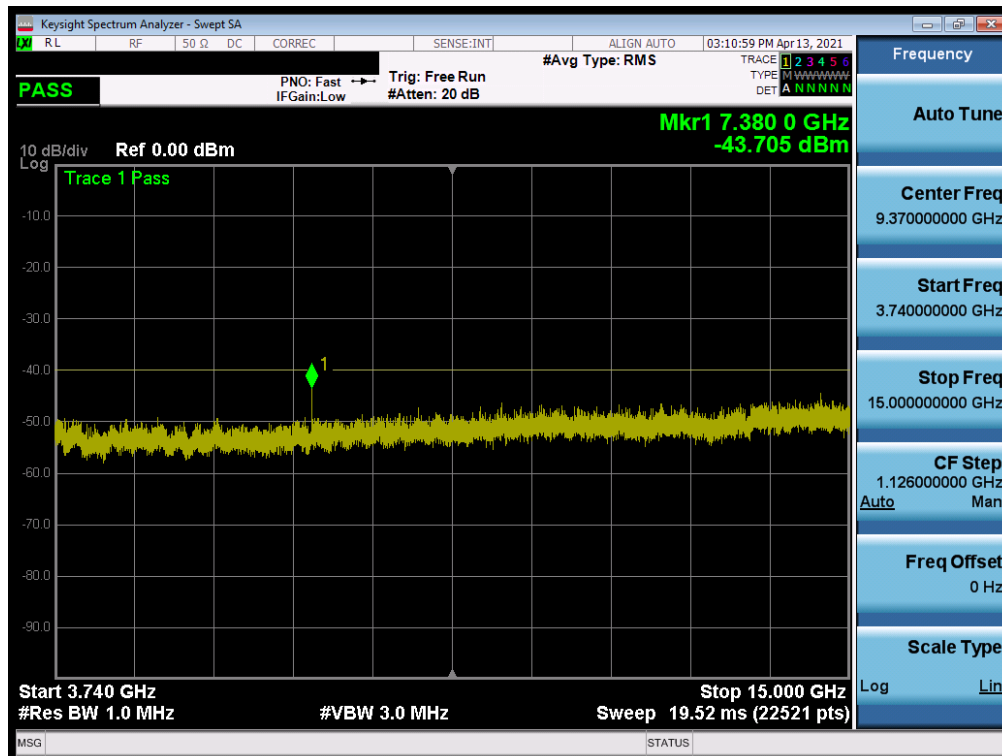
Plot 7-26. Conducted Spurious Plot (LTE Band 48 - 20MHz QPSK - RB Size 1, RB Offset 0 - High Channel)
