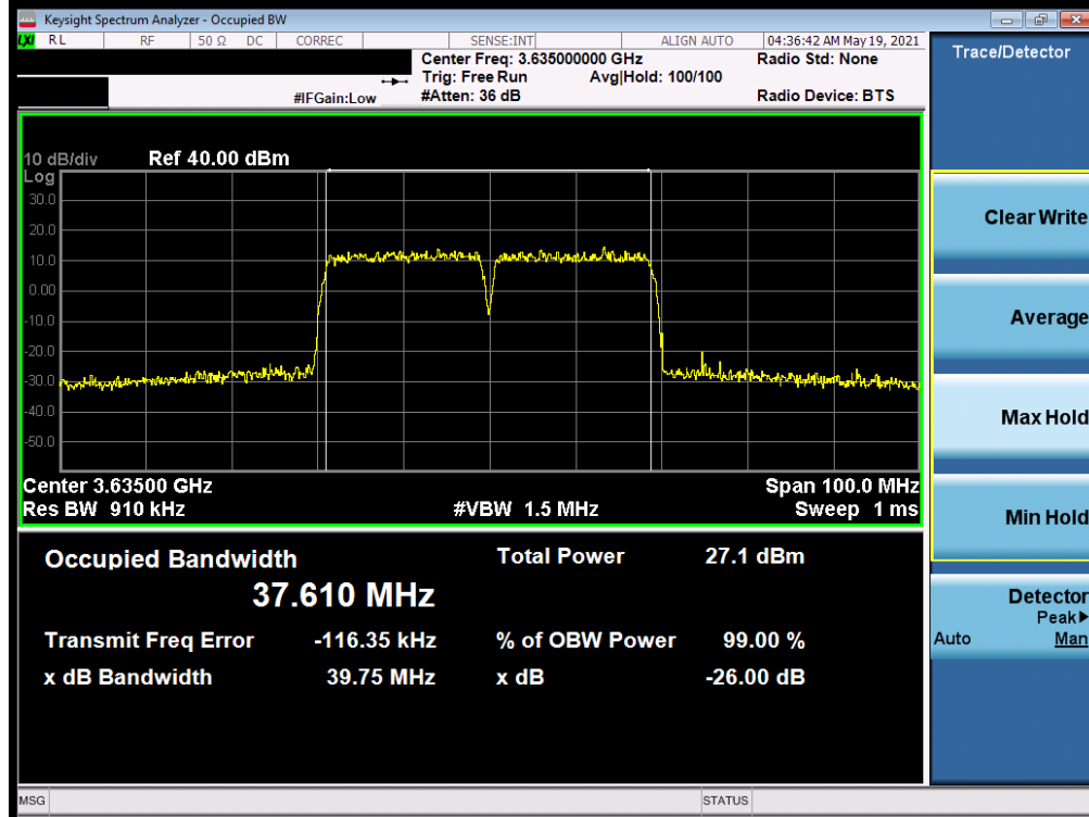
Plot 7-10. Occupied Bandwidth Plot (ULCA LTE Band 48 - 20+20MHz 16-QAM - Full RB Configuration)
