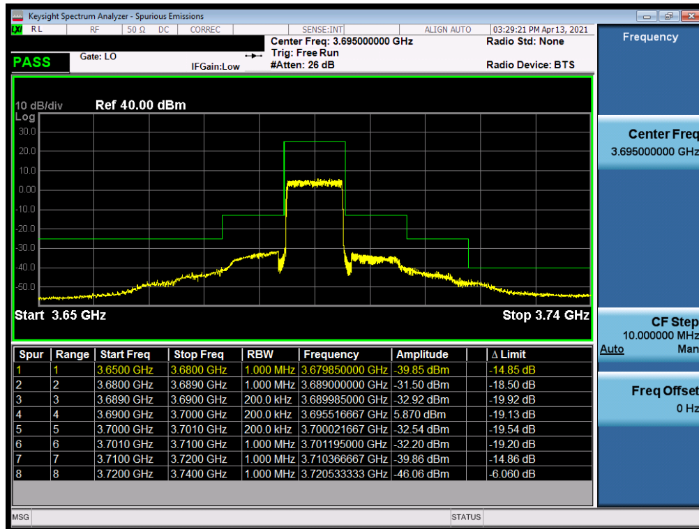
Plot 7-49. Channel Edge Plot (LTE Band 48 - 10MHz QPSK - High Channel)
