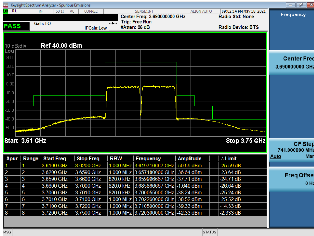
Plot 7-55. Channel Edge Plot (LTE Band 48 – 20+20MHz QPSK - High Channel)
