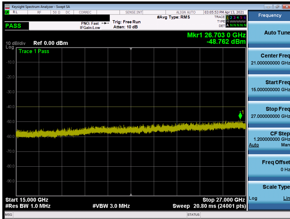
Plot 7-23. Conducted Spurious Plot (LTE Band 48 - 20MHz QPSK - RB Size 1, RB Offset 0 - Mid Channel)
