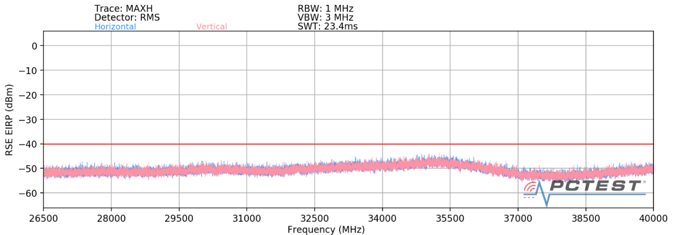
Plot 7-60. Radiated Spurious Plot - 26.5-40 GHz (LTE Band 48) – Open
