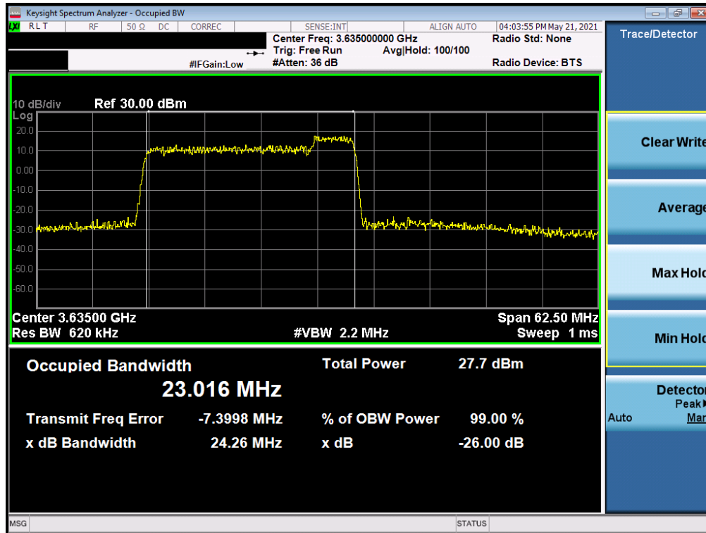
Plot 7-15. Occupied Bandwidth Plot (ULCA LTE Band 48 - 20+5MHz QPSK - Full RB Configuration)
