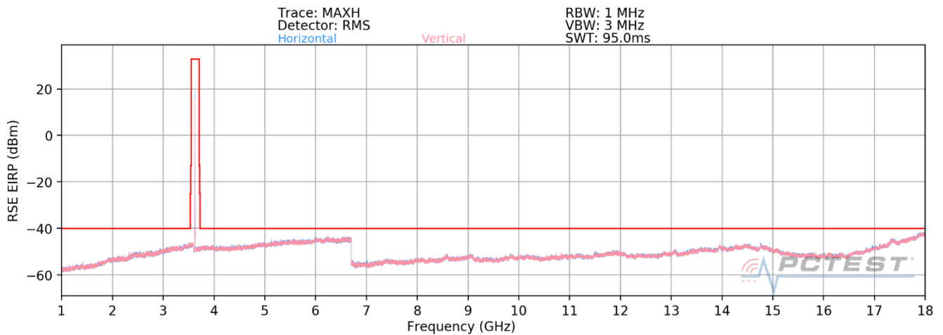
Plot 7-57. Radiated Spurious Plot - 1-18 GHz (LTE Band 48) – Closed
