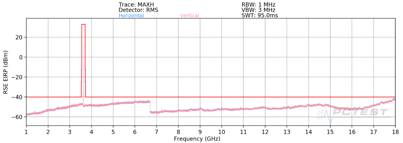
Plot 7-56. Radiated Spurious Plot - 1-18 GHz (LTE Band 48) – Open
