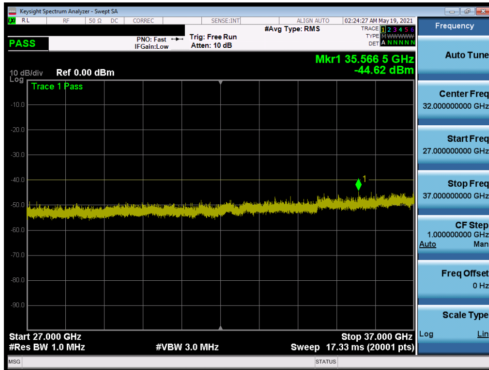
Plot 7-36. Conducted Spurious Plot (ULCA LTE Band 48 - 20+20MHz QPSK - Mid Channel)
