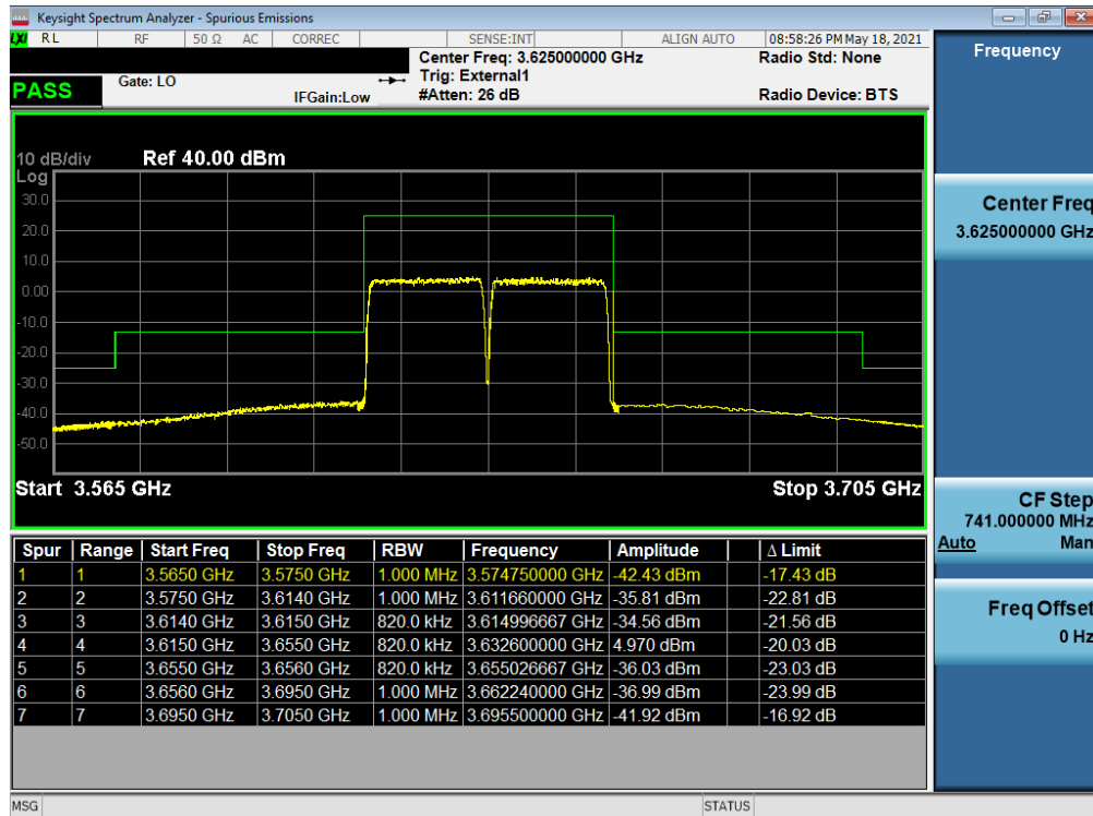
Plot 7-54. Channel Edge Plot (LTE Band 48 – 20+20MHz QPSK - Mid Channel)
