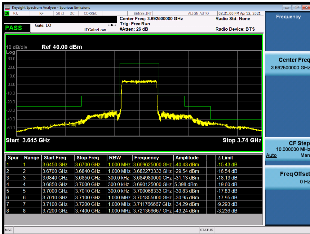
Plot 7-46. Channel Edge Plot (LTE Band 48 - 15MHz QPSK - High Channel)
