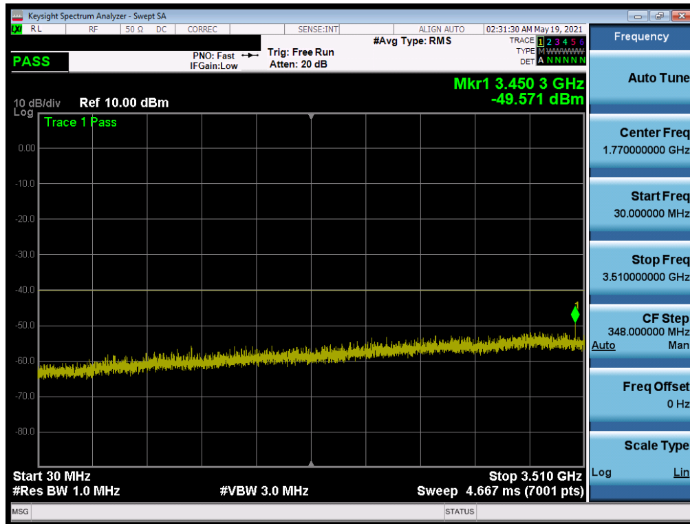
Plot 7-29. Conducted Spurious Plot (ULCA LTE Band 48 - 20+20MHz QPSK - Low Channel)
