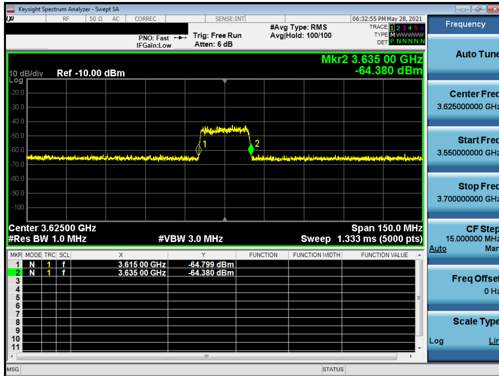
Plot 7-66. Run#1 End User Device Frequency of Operations
