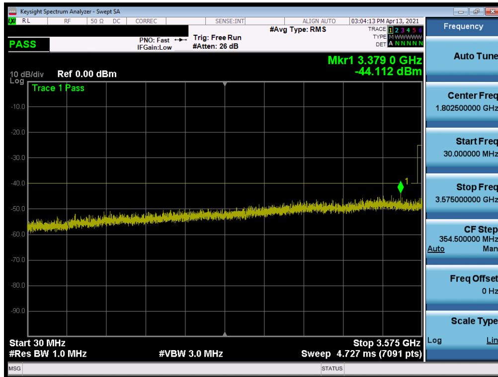
Plot 7-21. Conducted Spurious Plot (LTE Band 48 - 20MHz QPSK - RB Size 1, RB Offset 0 - Mid Channel)
