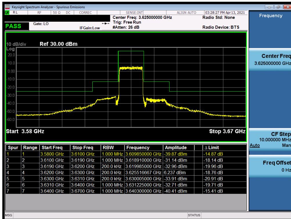
Plot 7-48. Channel Edge Plot (LTE Band 48 - 10MHz QPSK - Mid Channel)
