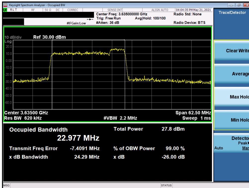
Plot 7-16. Occupied Bandwidth Plot (ULCA LTE Band 48 - 20+5MHz 16-QAM - Full RB Configuration)
