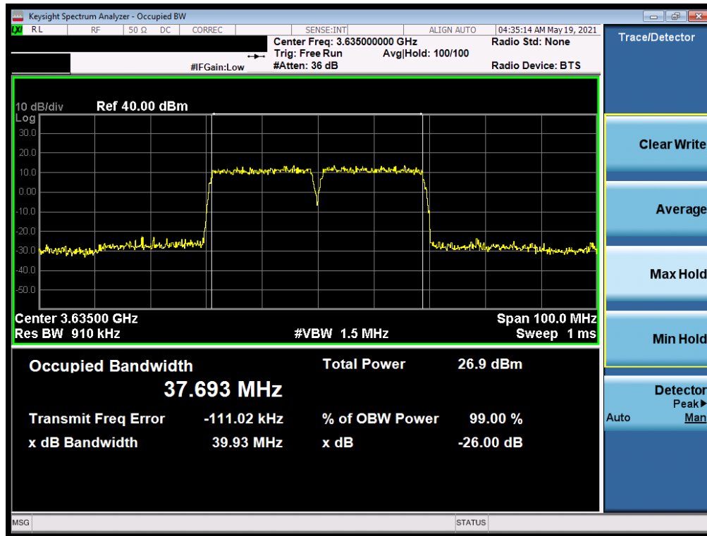
Plot 7-9. Occupied Bandwidth Plot (ULCA LTE Band 48 - 20+20MHz QPSK - Full RB Configuration)
