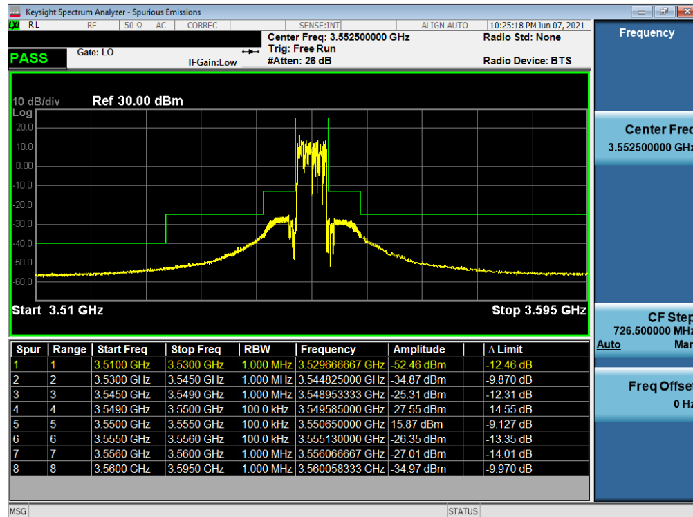
Plot 7-50. Channel Edge Plot (LTE Band 48 - 5MHz QPSK - Low Channel)
