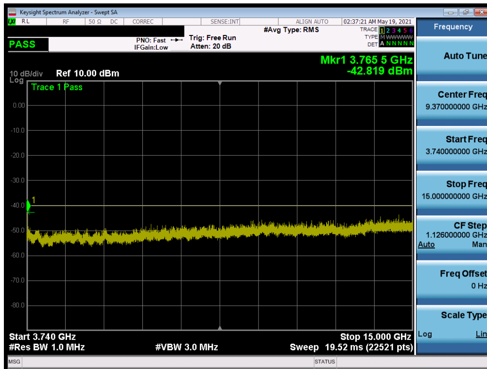
Plot 7-38. Conducted Spurious Plot (ULCA LTE Band 48 - 20+20MHz QPSK - High Channel)
