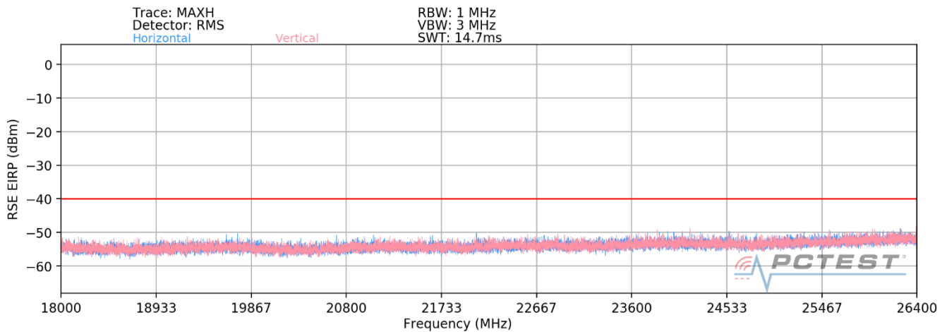
Plot 7-58. Radiated Spurious Plot - 18-26.5 GHz (LTE Band 48) – Open
