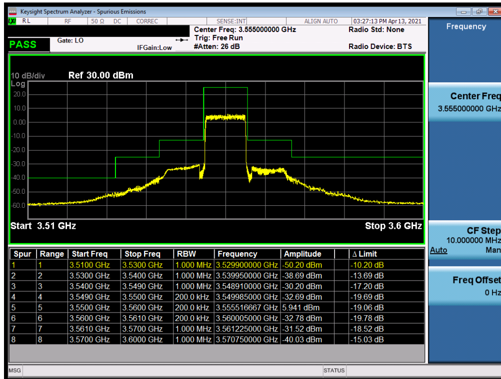
Plot 7-47. Channel Edge Plot (LTE Band 48 - 10MHz QPSK - Low Channel)
