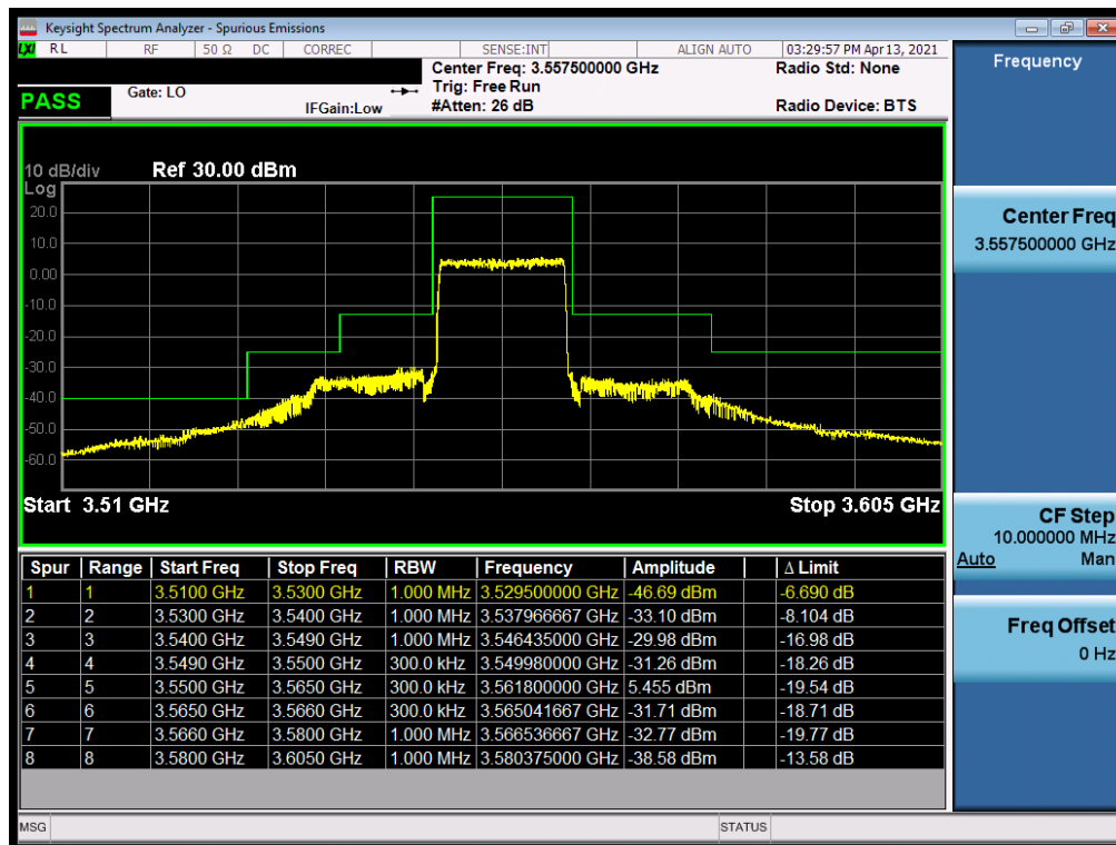
Plot 7-44. Channel Edge Plot (LTE Band 48 - 15MHz QPSK - Low Channel)
