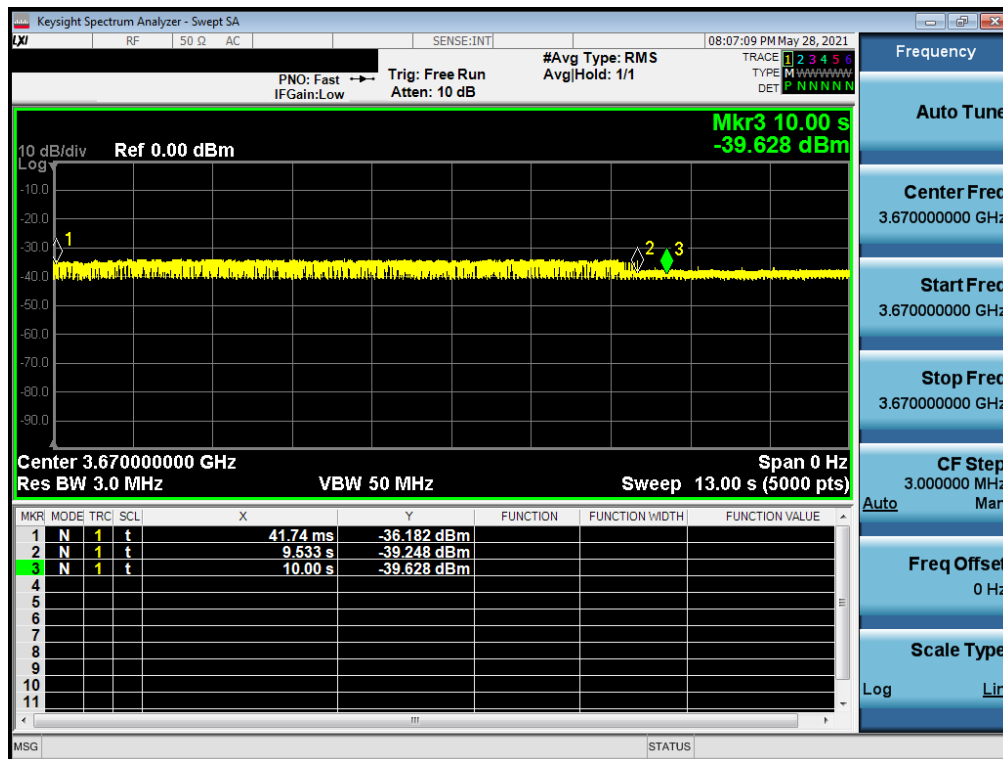
Plot 7-69. Run#2 End User Device Discontinues Operations within 10s
