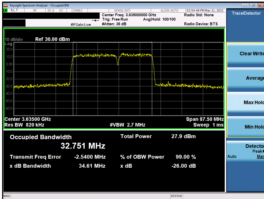
Plot 7-12. Occupied Bandwidth Plot (ULCA LTE Band 48 - 20+15MHz 16-QAM - Full RB Configuration)
