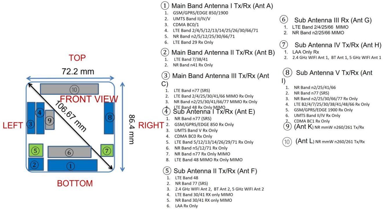
Figure E-3 DUT Antenna Locations Closed Configuration
