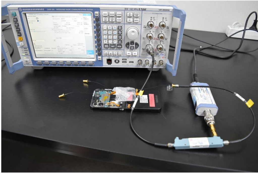
A,1 : Conducted test in CMW500 callbox
