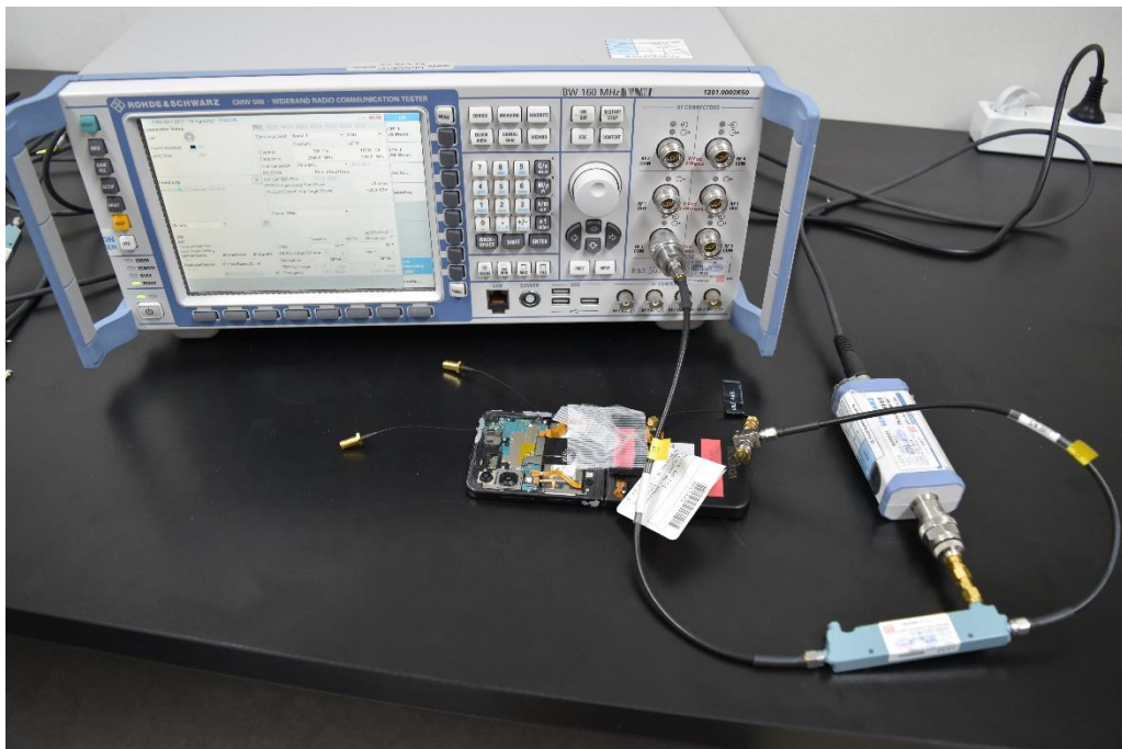
A,2 : Conducted test in CMW500 callbox
