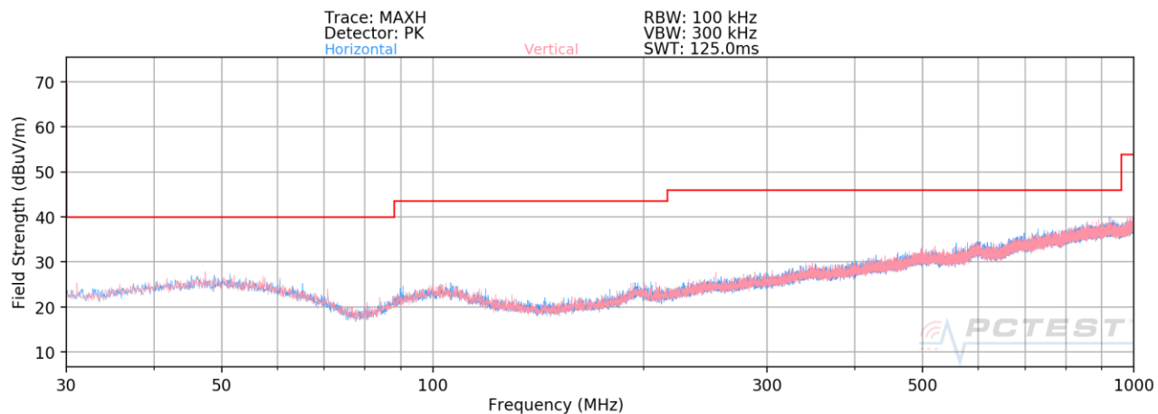
Plot 7-8. Radiated Spurious Plot 30MHz – 1GHz – CLOSE
