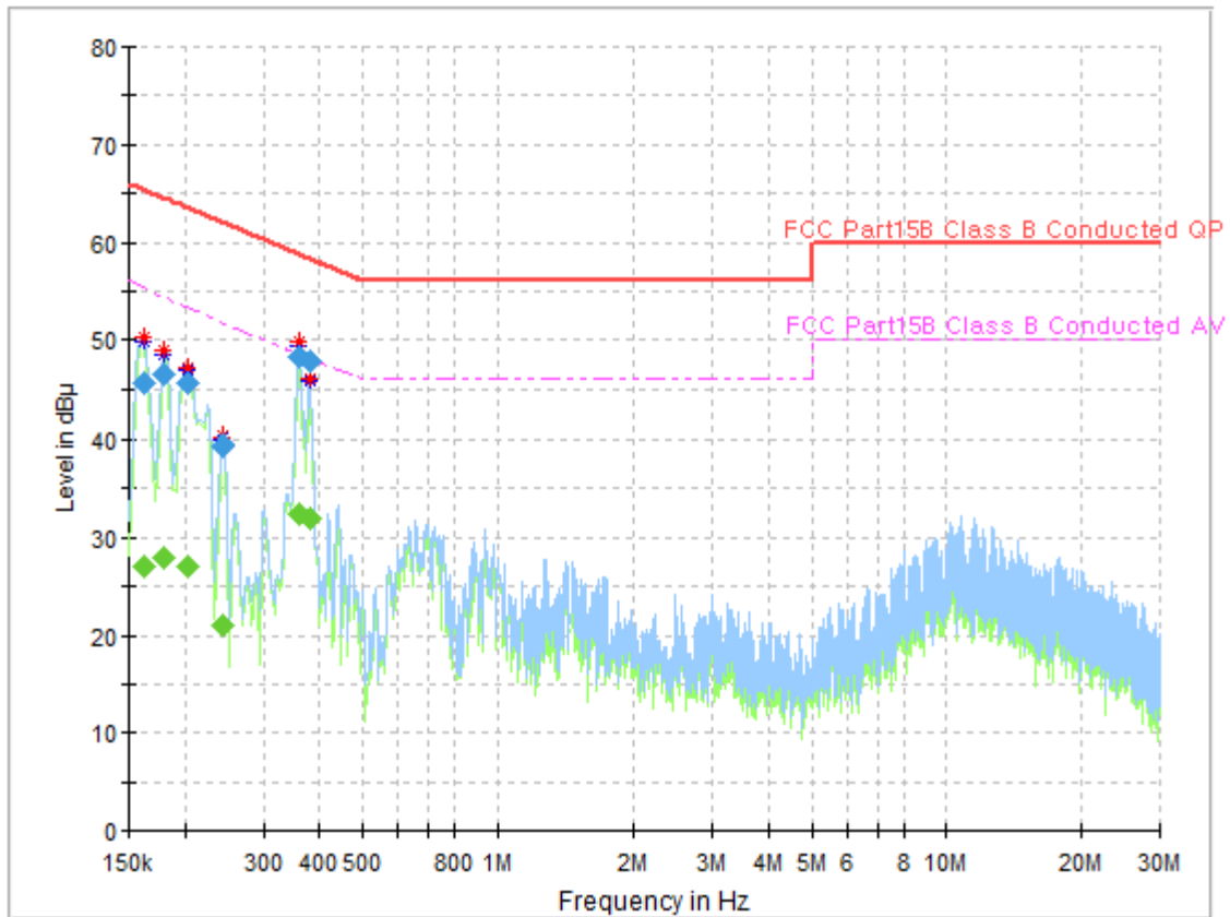
Plot 7-14. Line-Conducted Test Plot (N)
