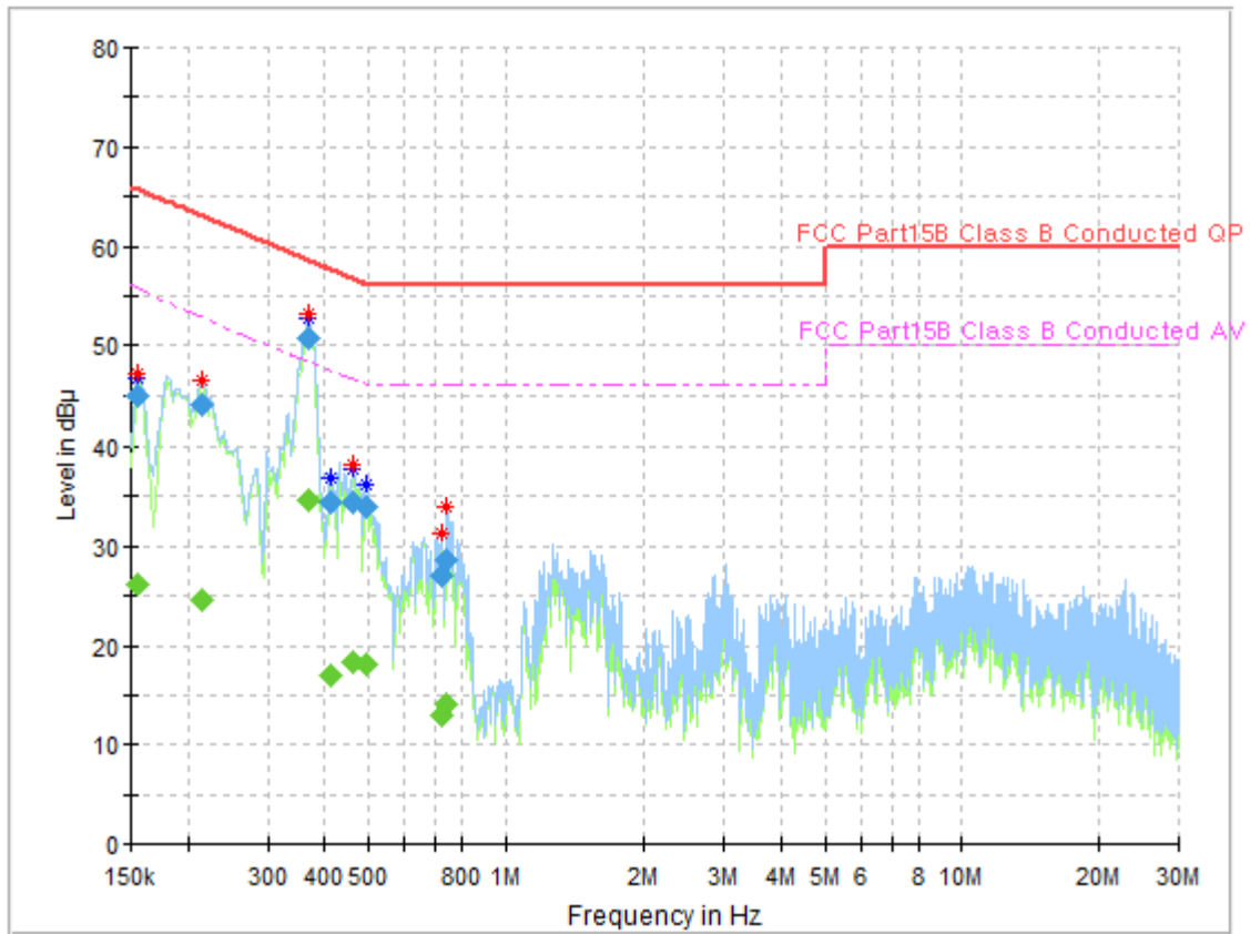
Plot 7-13. Line-Conducted Test Plot (L1)
