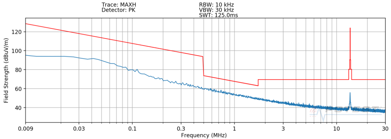
Plot 7-6. Radiated Spurious Plot 9kHz – 30MHz (Pol. Y) – CLOSE
