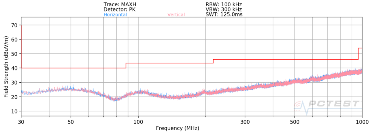
Plot 7-12. Radiated Spurious Plot 30MHz – 1GHz – HALF OPEN
