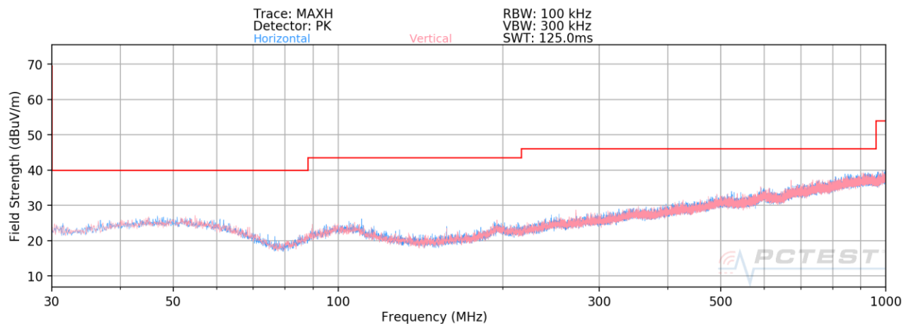
Plot 7-4. Radiated Spurious Plot 30MHz – 1GHz – OPEN
