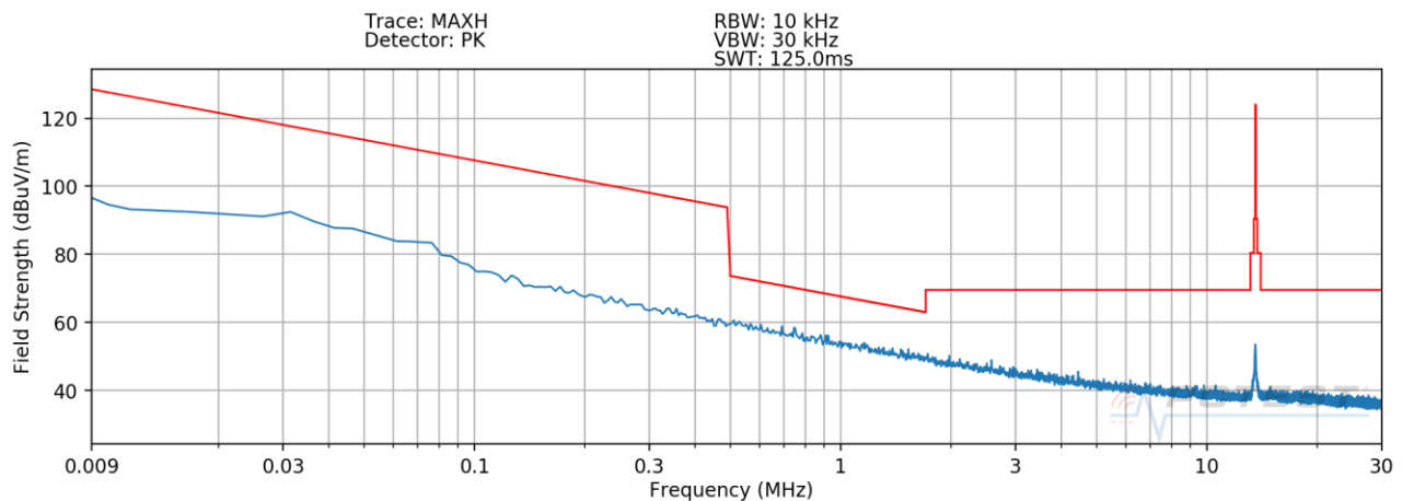
Plot 7-7. Radiated Spurious Plot 9kHz – 30MHz (Pol. Z) – CLOSE
