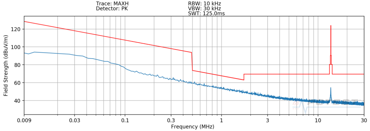
Plot 7-9. Radiated Spurious Plot 9kHz – 30MHz (Pol. X) – HALF OPEN
