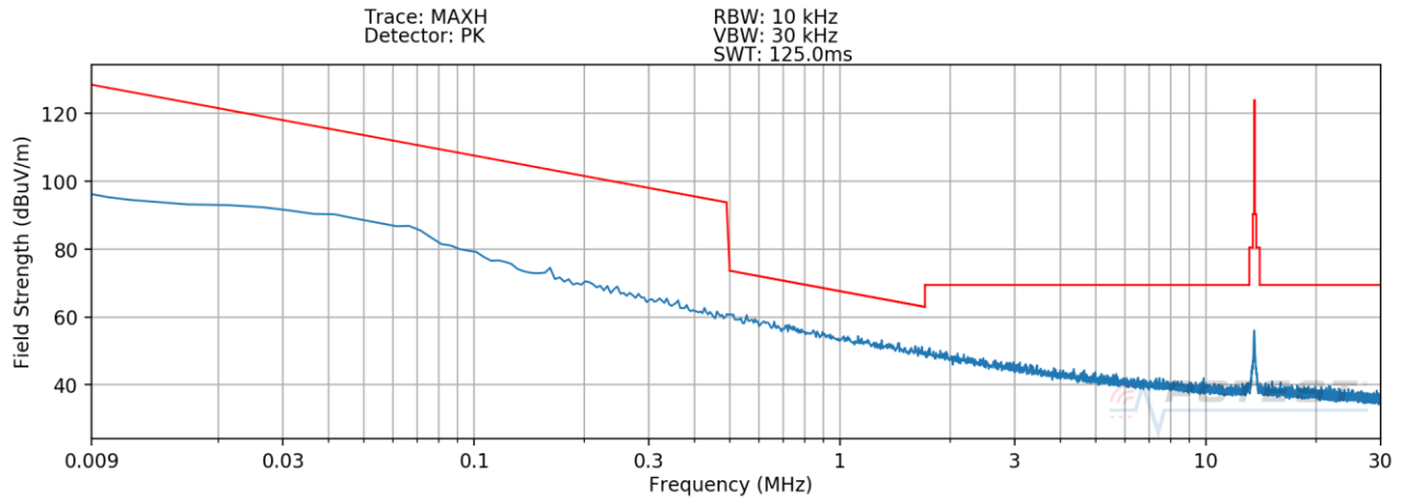
Plot 7-10. Radiated Spurious Plot 9kHz – 30MHz (Pol. Y) – HALF OPEN
