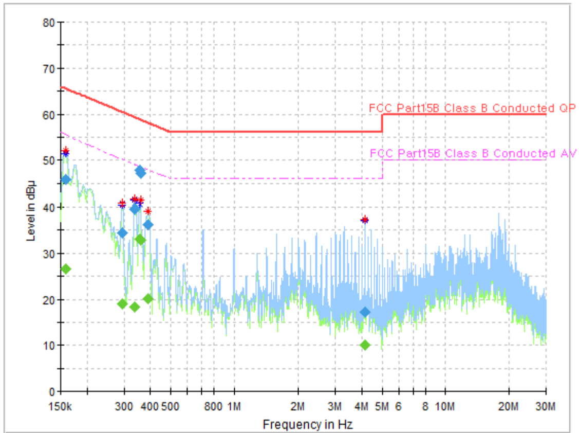
Plot 7-16. Line-Conducted Test Plot (N) with WCP
