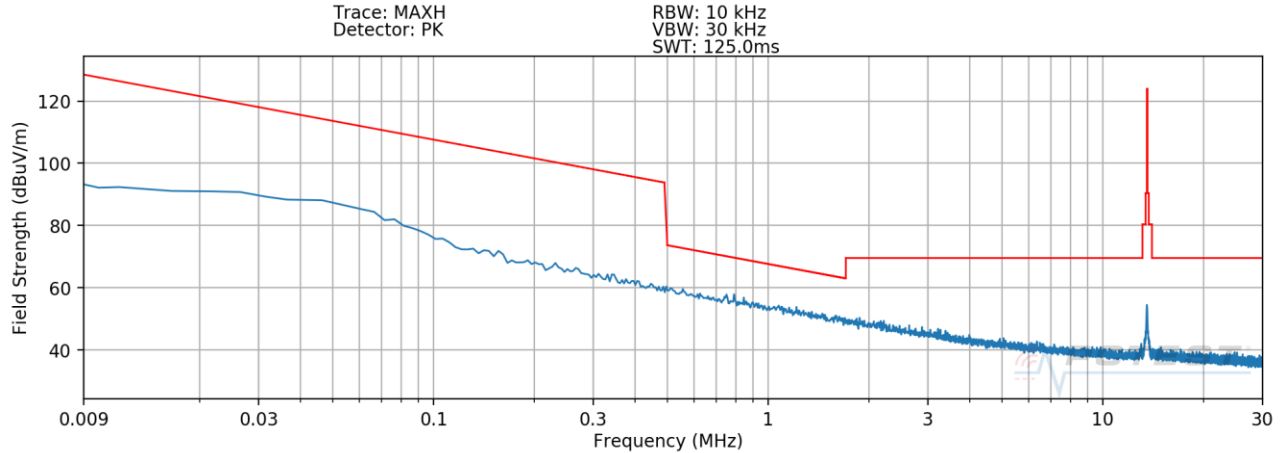
Plot 7-5. Radiated Spurious Plot 9kHz – 30MHz (Pol. X) – CLOSE
