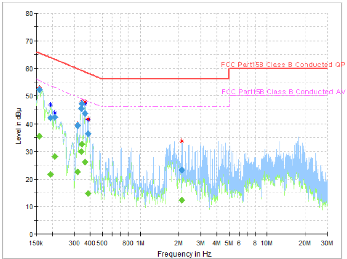
Plot 7-15. Line-Conducted Test Plot (L1) with WCP
