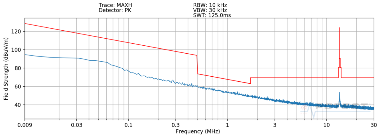
Plot 7-11. Radiated Spurious Plot 9kHz – 30MHz (Pol. Z) – HALF OPEN
