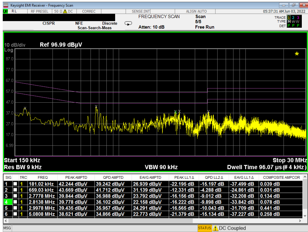
Plot 7-109. Line-Conducted Test Plot (L1) - OPEN
