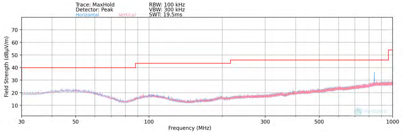
Plot 7-107. Radiated Spurious Plot below 1GHz – ANT 2 – Open
