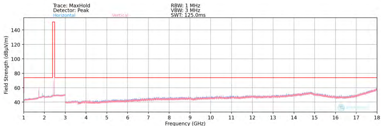
Plot 7-85. Radiated Spurious Plot above 1GHz (BT– Ch. 78) - ANT1 – Open
