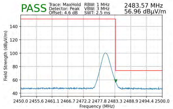
Plot 7-102. Radiated Restricted Upper Band Edge Measurement (Peak) – ANT 2
