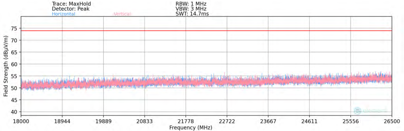
Plot 7-97. Radiated Spurious Plot above 18GHz – ANT2 – Half Open
