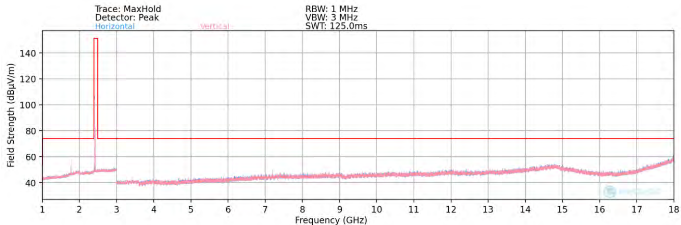
Plot 7-86. Radiated Spurious Plot above 1GHz (BT- Ch. 0) - ANT1 – Half Open
