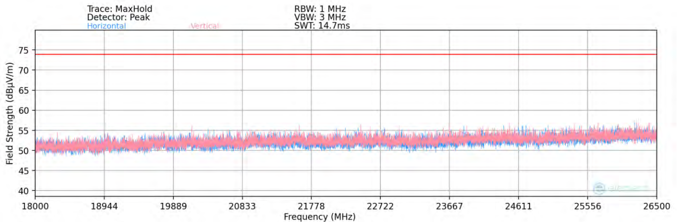
Plot 7-98. Radiated Spurious Plot above 18GHz – ANT2 – Open
