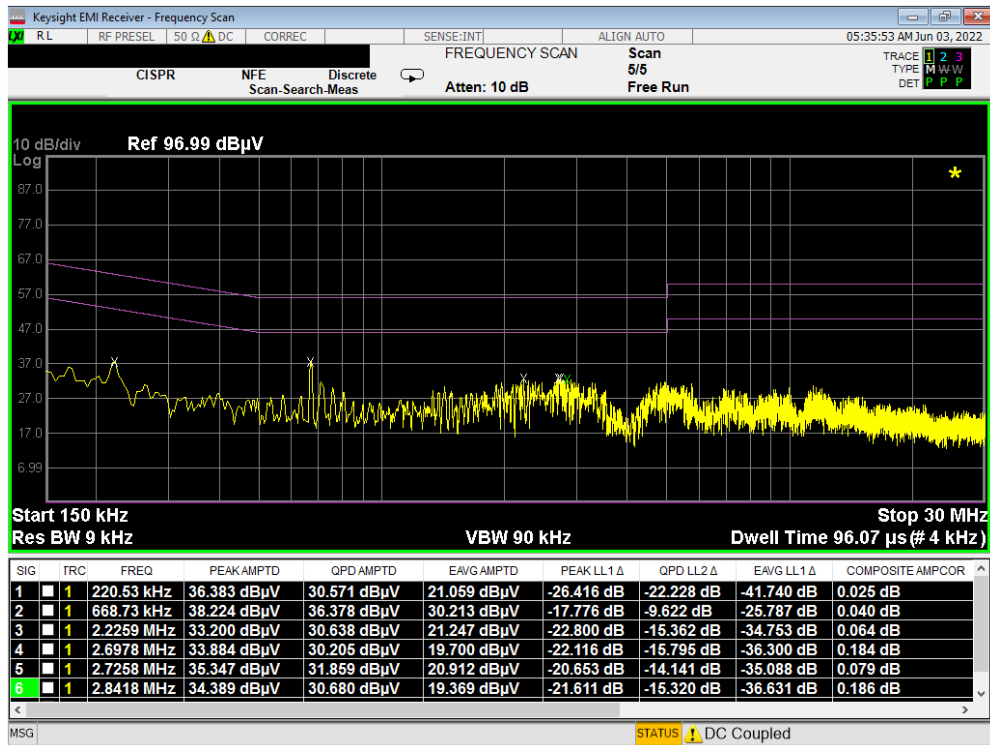
Plot 7-110. Line-Conducted Test Plot (N) - OPEN
