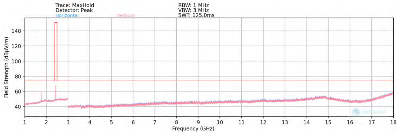
Plot 7-92. Radiated Spurious Plot above 1GHz (BT– Ch. 39) – ANT2 – Half Open
