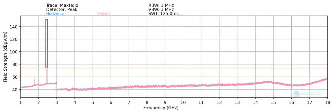
Plot 7-88. Radiated Spurious Plot above 1GHz (BT- Ch. 78) - ANT1 – Half Open
