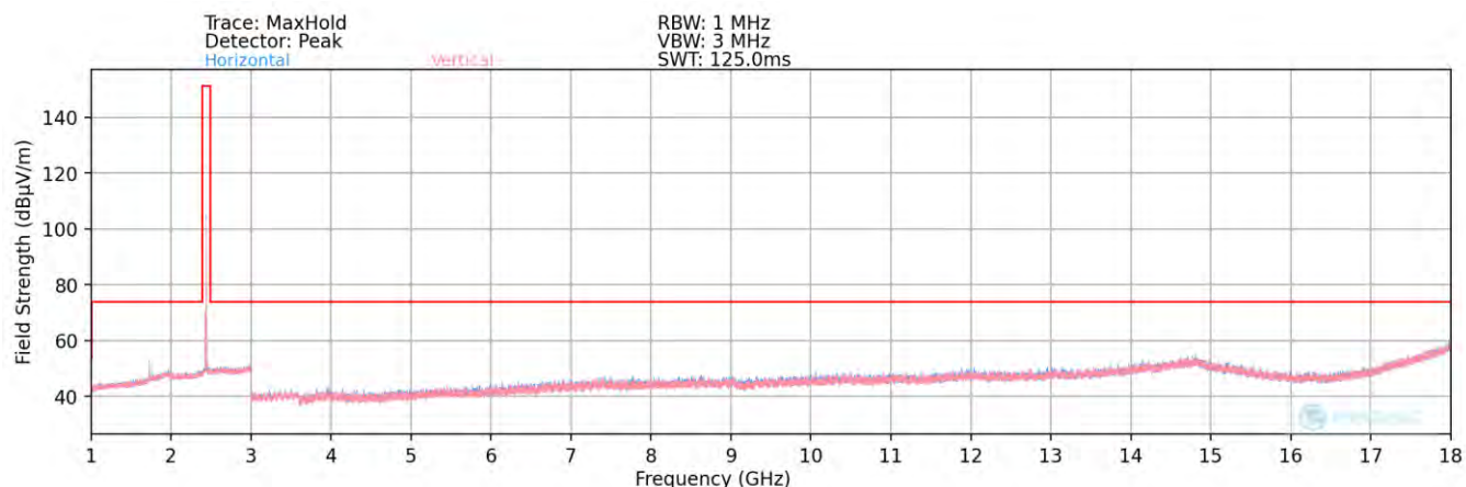
Plot 7-84. Radiated Spurious Plot above 1GHz (BT– Ch. 39) - ANT1 – Open
