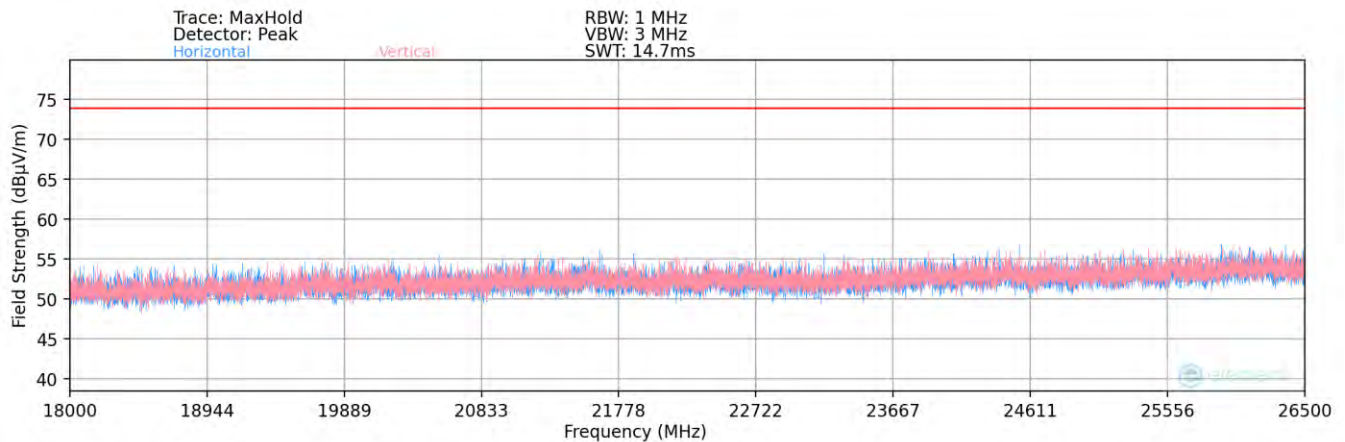
Plot 7-90. Radiated Spurious Plot above 18GHz - ANT1 – Half Open
