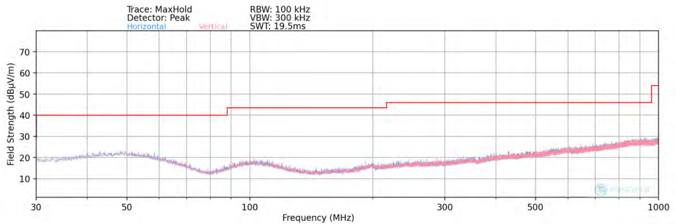
Plot 7-108. Radiated Spurious Plot below 1GHz – ANT 2 – Half Open
