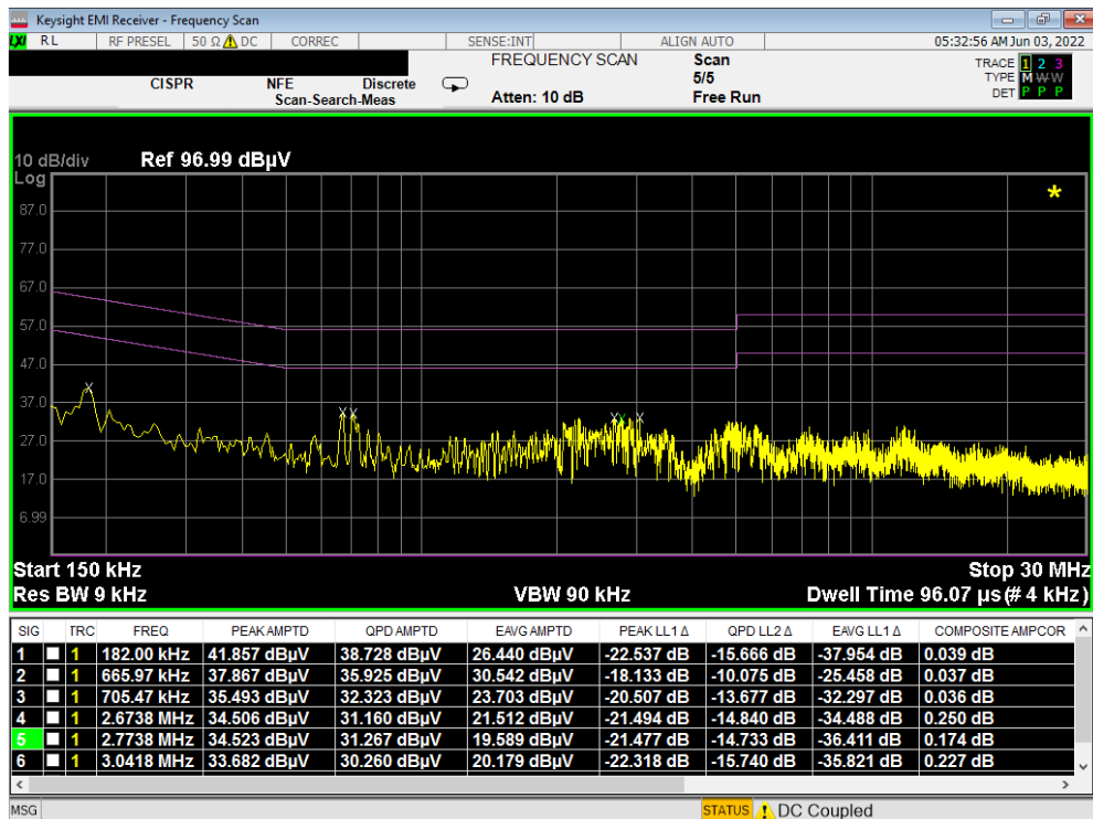
Plot 7-112. Line-Conducted Test Plot (N) - CLOSED
