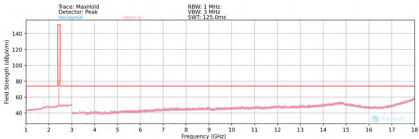
Plot 7-87. Radiated Spurious Plot above 1GHz (BT- Ch. 39) - ANT1 – Half Open
