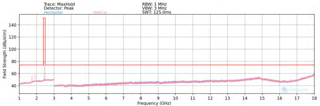
Plot 7-96. Radiated Spurious Plot above 1GHz (BT– Ch. 78) – ANT2 – Open
