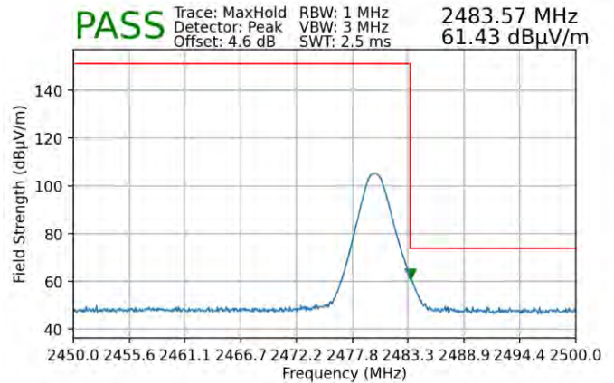
Plot 7-100. Radiated Restricted Upper Band Edge Measurement (Peak) – ANT 1
