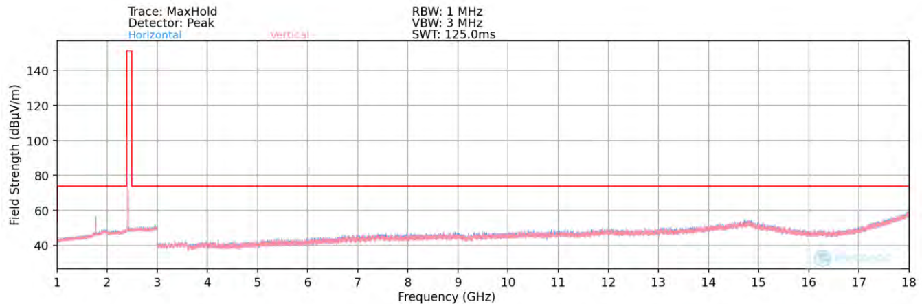
Plot 7-91. Radiated Spurious Plot above 1GHz (BT– Ch. 0) – ANT2 – Half Open
