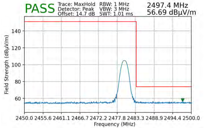
Plot 7-104. Radiated Restricted Upper Band Edge Measurement with WCP (Peak) – ANT 1
