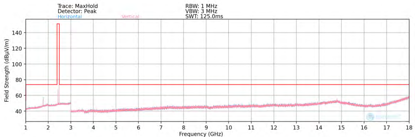
Plot 7-93. Radiated Spurious Plot above 1GHz (BT– Ch. 78) – ANT2 – Half Open
