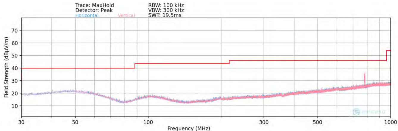
Plot 7-106. Radiated Spurious Plot below 1GHz – ANT 1 – Half Open
