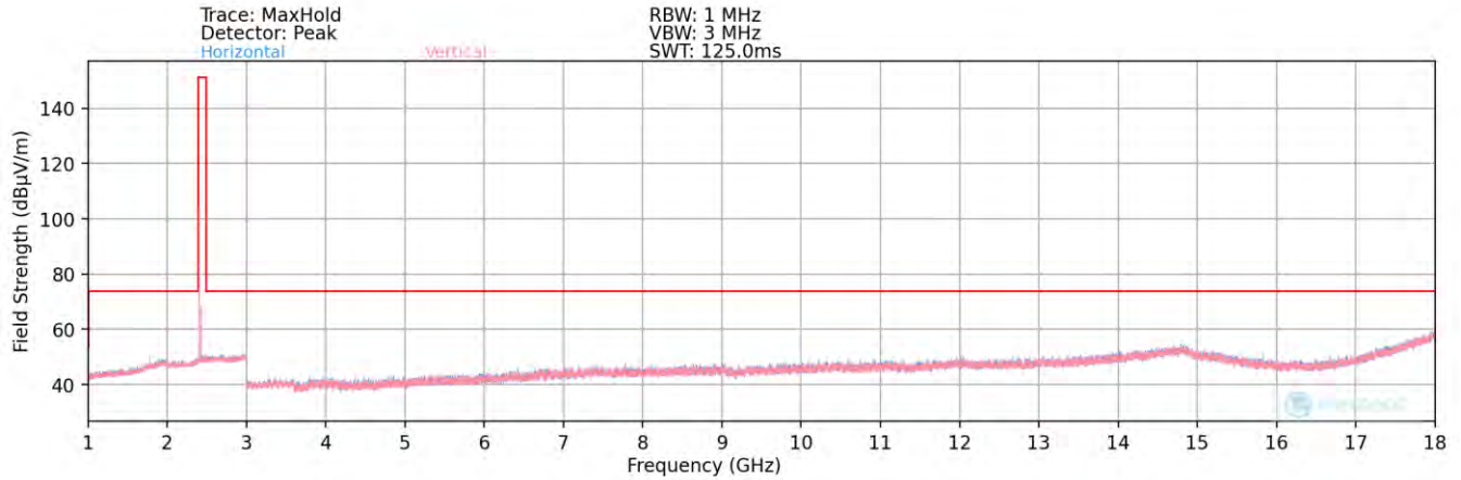
Plot 7-94. Radiated Spurious Plot above 1GHz (BT– Ch. 0) – ANT2 – Open
