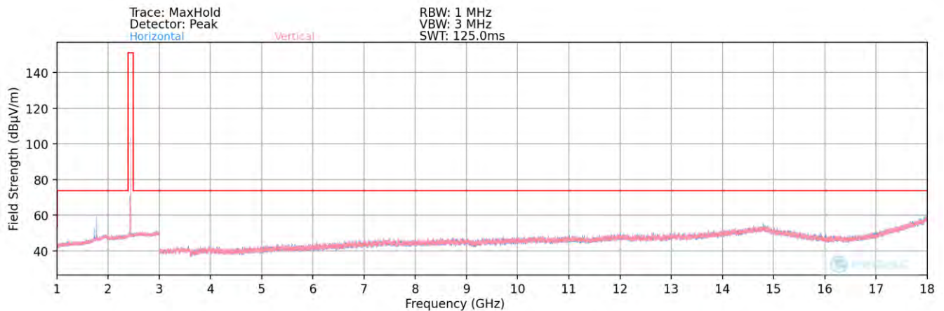
Plot 7-95. Radiated Spurious Plot above 1GHz (BT– Ch. 39) – ANT2 – Open
