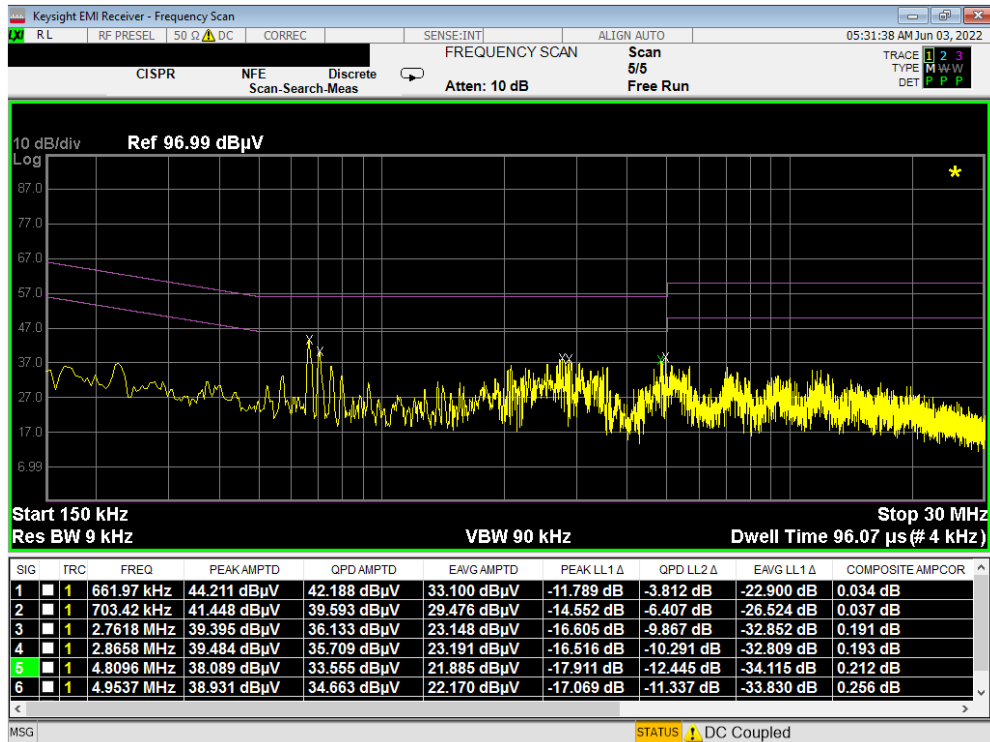
Plot 7-111. Line-Conducted Test Plot (L1) - CLOSED
