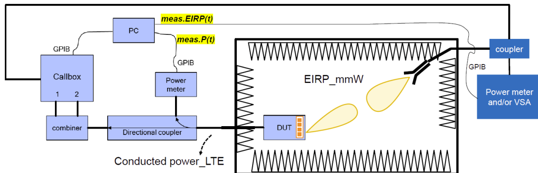
Figure 7-1 mmW NR radiated power measurement setup – Test Setup Photo 11
