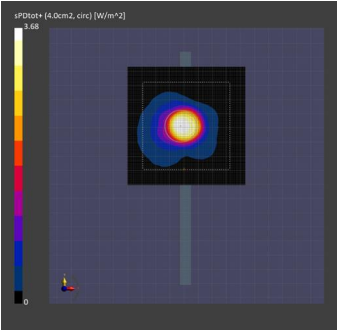
Figure 12-2 4cm 2 psPD distribution measured at input.power.limit of 10.2 dBm on the Left Edge for n260 beam 2
