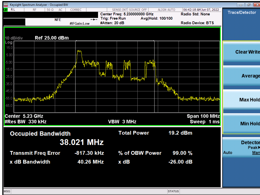
Plot 7-55. 26dB Bandwidth Plot ANT2 (40MHz BW 802.11ax – 26 Tones (UNII Band 1) – Ch. 46)
