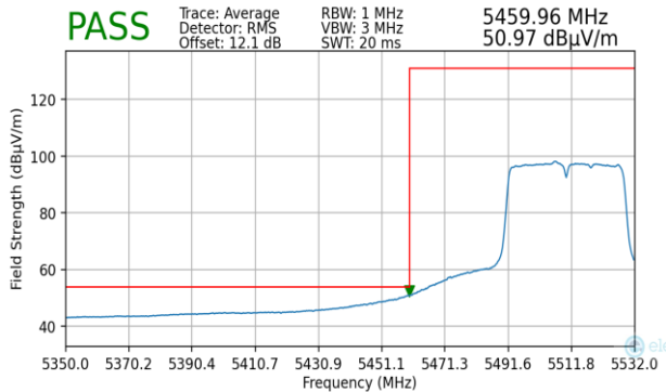
Plot 7-455. Radiated Lower Band Edge Plot MIMO (Average – UNII Band 2C)
