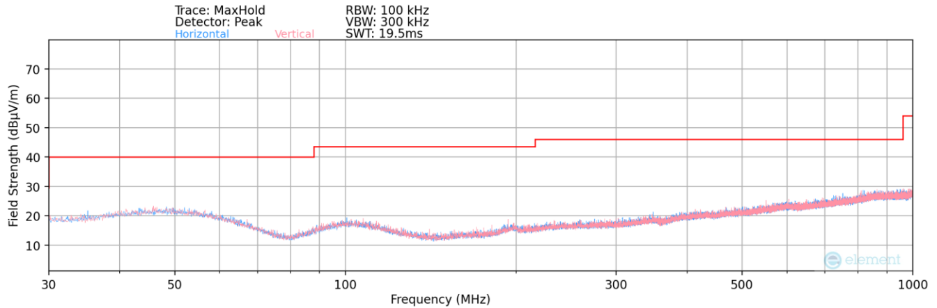
Plot 7-478. Radiated Spurious Plot below 1GHz (2.4GHz – 5GHz)
