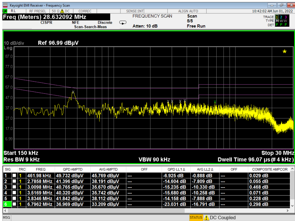
Plot 7-493. Line Conducted Plot with 802.11a UNII Band 3 (L1) – Open
