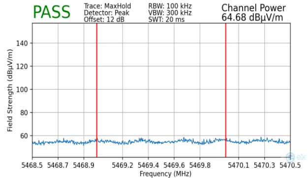
Plot 7-456. Radiated Lower Band Edge Plot MIMO (Peak – UNII Band 2C)
