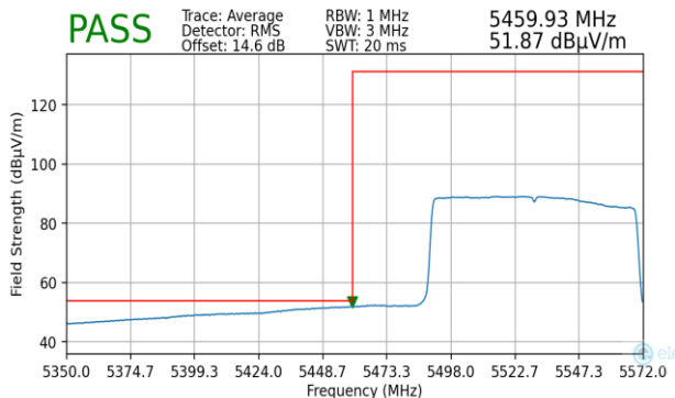
Plot 7-464. Radiated Lower Band Edge Plot MIMO (Average – UNII Band 2C)
