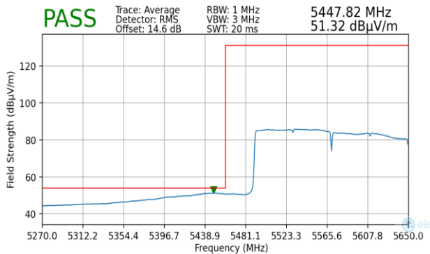
Plot 7-473. Radiated Lower Band Edge Plot MIMO (Average – UNII Band 2C)
