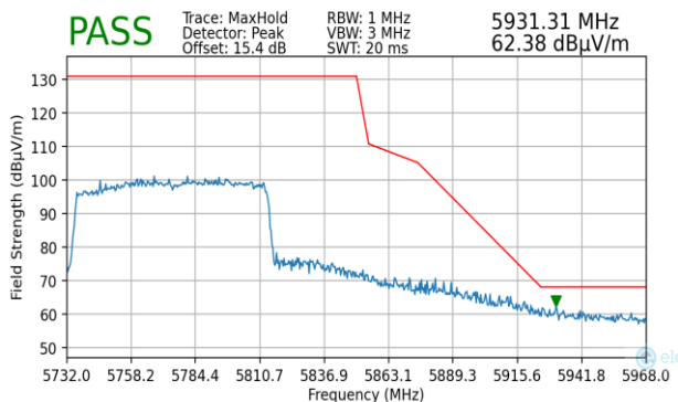
Plot 7-466. Radiated Upper Band Edge Plot MIMO (Peak – UNII Band 3)
