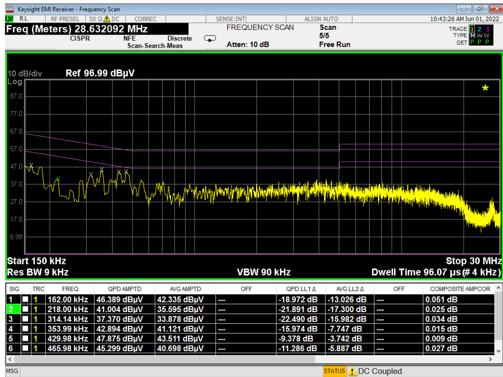
Plot 7-495. Line Conducted Plot with 802.11a UNII Band 3 (N) – Open
