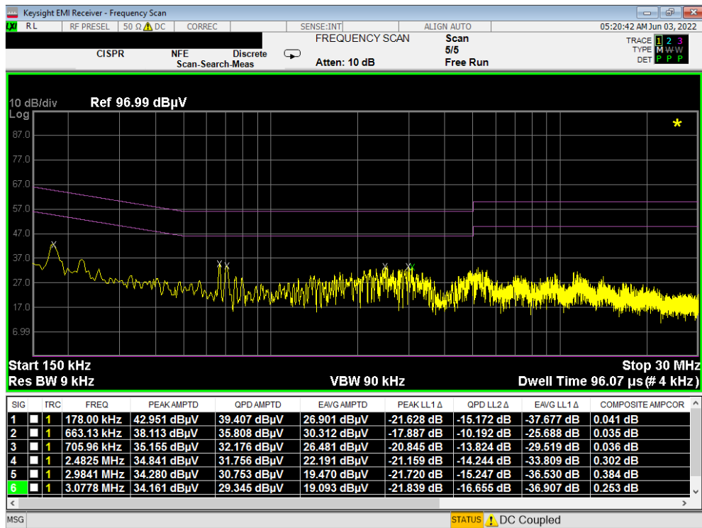
Plot 7-484. Line Conducted Plot with 802.11a UNII Band 1 (N) – Closed
