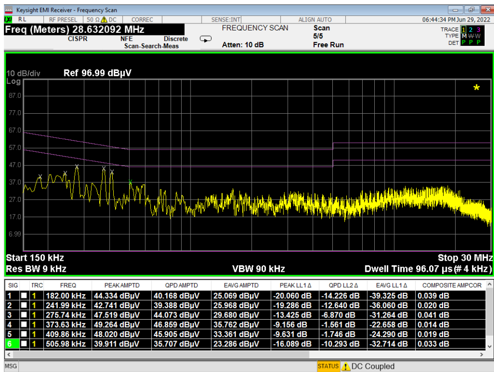
Plot 7-490. Line Conducted Plot with 802.11a UNII Band 2C (L1) – Closed
