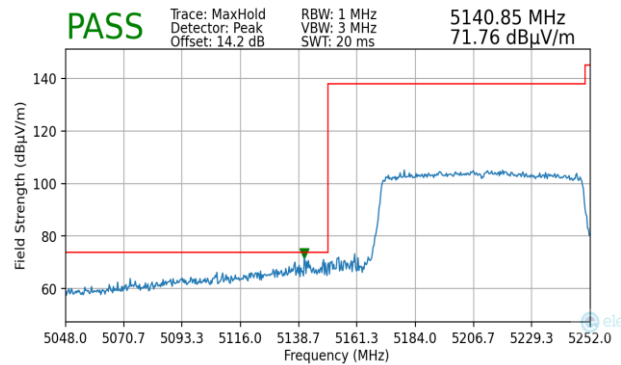
Plot 7-461. Radiated Lower Band Edge Plot MIMO (Peak – UNII Band 1)
