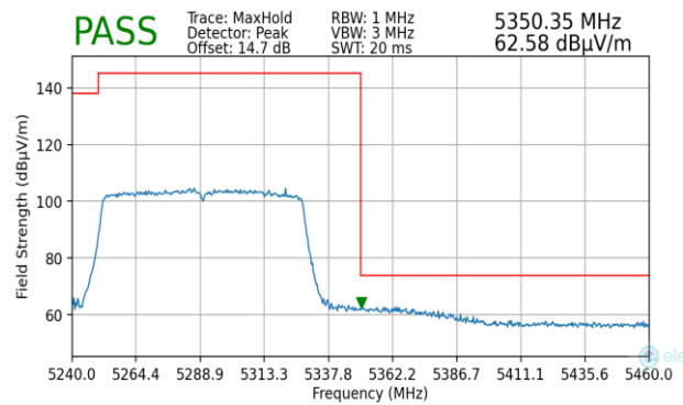
Plot 7-463. Radiated Upper Band Edge Plot MIMO (Peak – UNII Band 2A)
