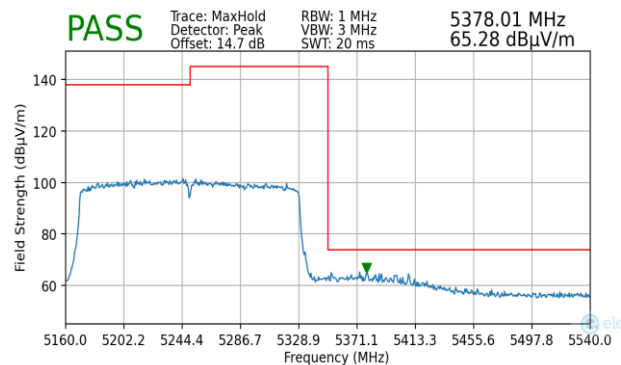
Plot 7-472. Radiated Upper Band Edge Plot MIMO (Peak – UNII Band 2A)
