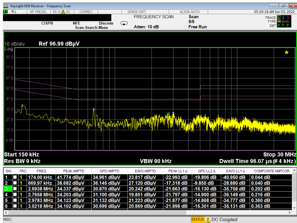
Plot 7-496. Line Conducted Plot with 802.11a UNII Band 3 (N) – Closed
