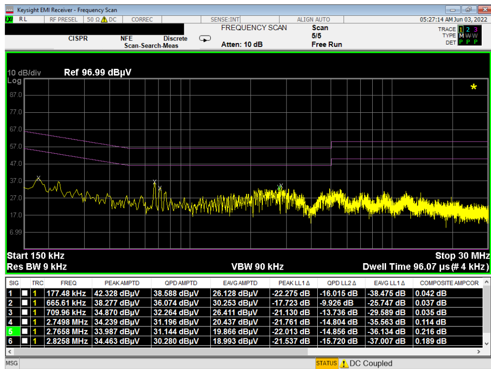
Plot 7-492. Line Conducted Plot with 802.11a UNII Band 2C (N) – Closed
