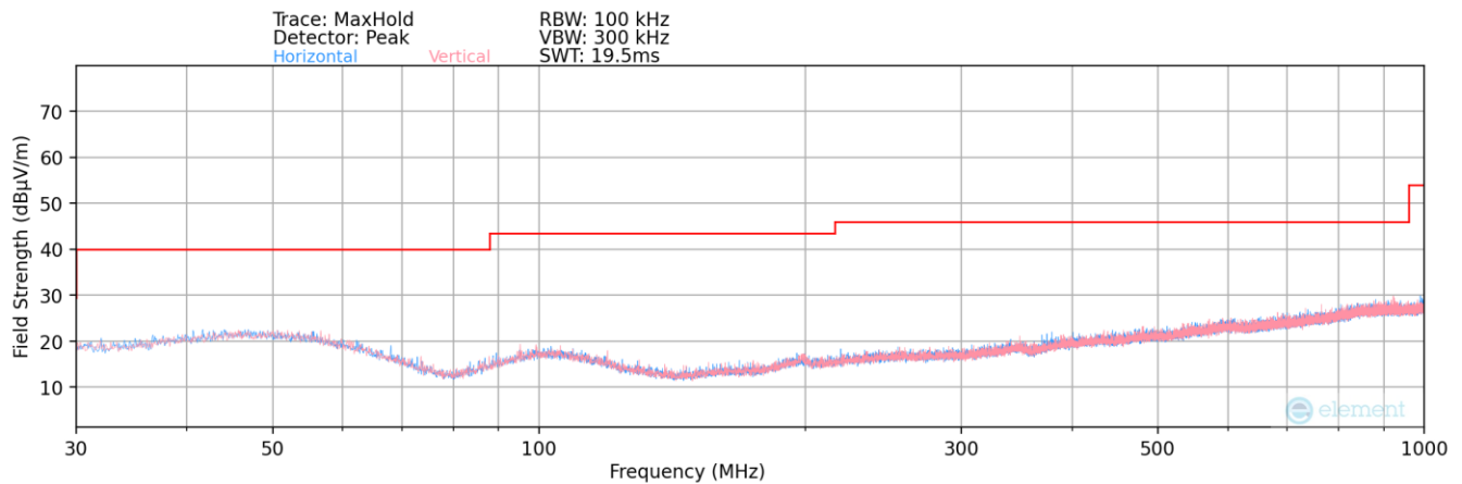
Plot 7-479. Radiated Spurious Plot below 1GHz (5GHz – 2.4 GHz)
