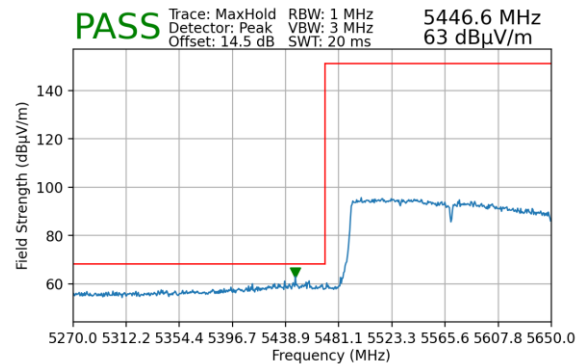
Plot 7-474. Radiated Lower Band Edge Plot MIMO (Peak – UNII Band 2C)
