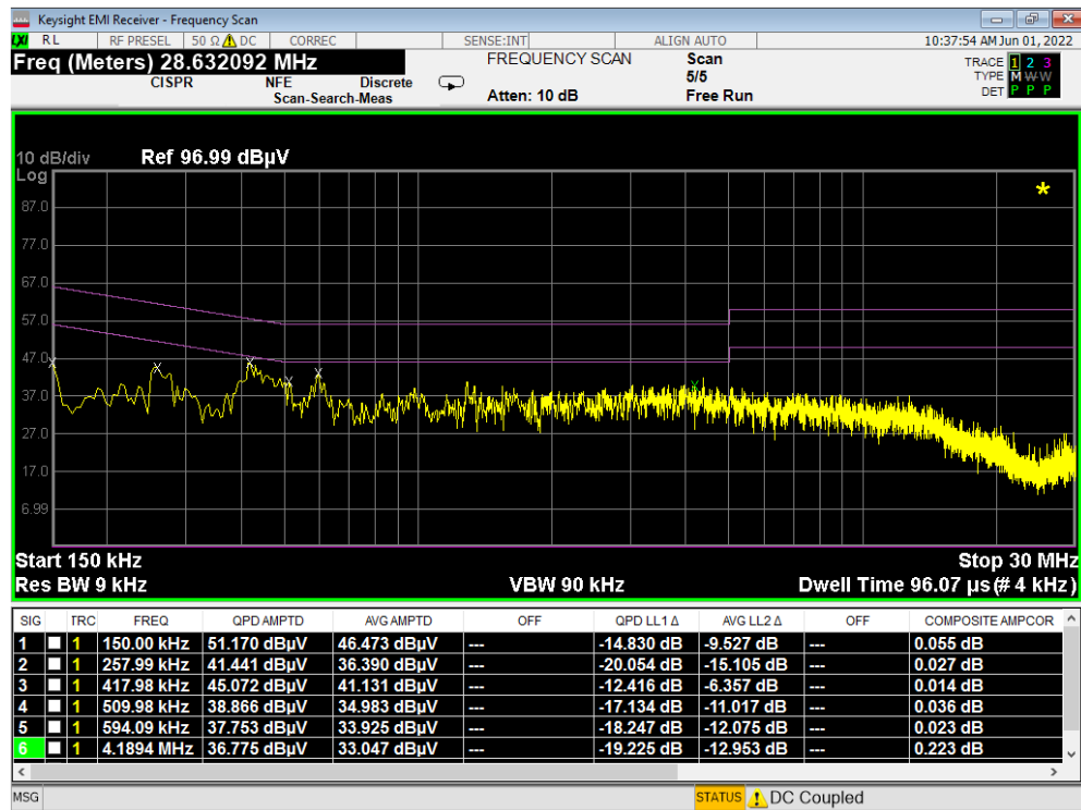
Plot 7-491. Line Conducted Plot with 802.11a UNII Band 2C (N) – Open
