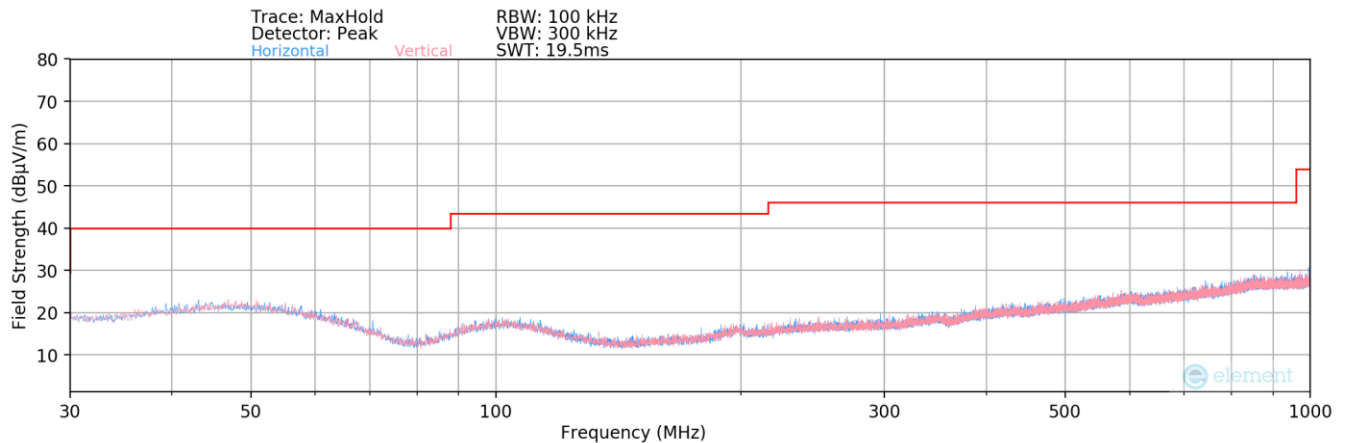
Plot 7-480. Radiated Spurious Plot below 1GHz (Dual Band Simult. Tx)
