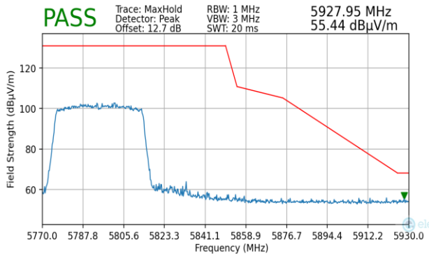
Plot 7-457. Radiated Upper Band Edge Plot MIMO (Peak – UNII Band 3)
