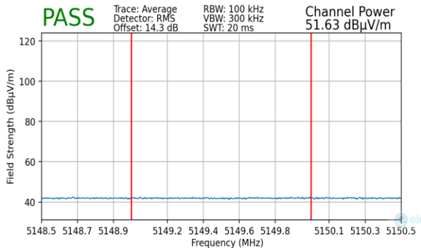
Plot 7-469. Radiated Lower Band Edge Plot MIMO (Average – UNII Band 1)
