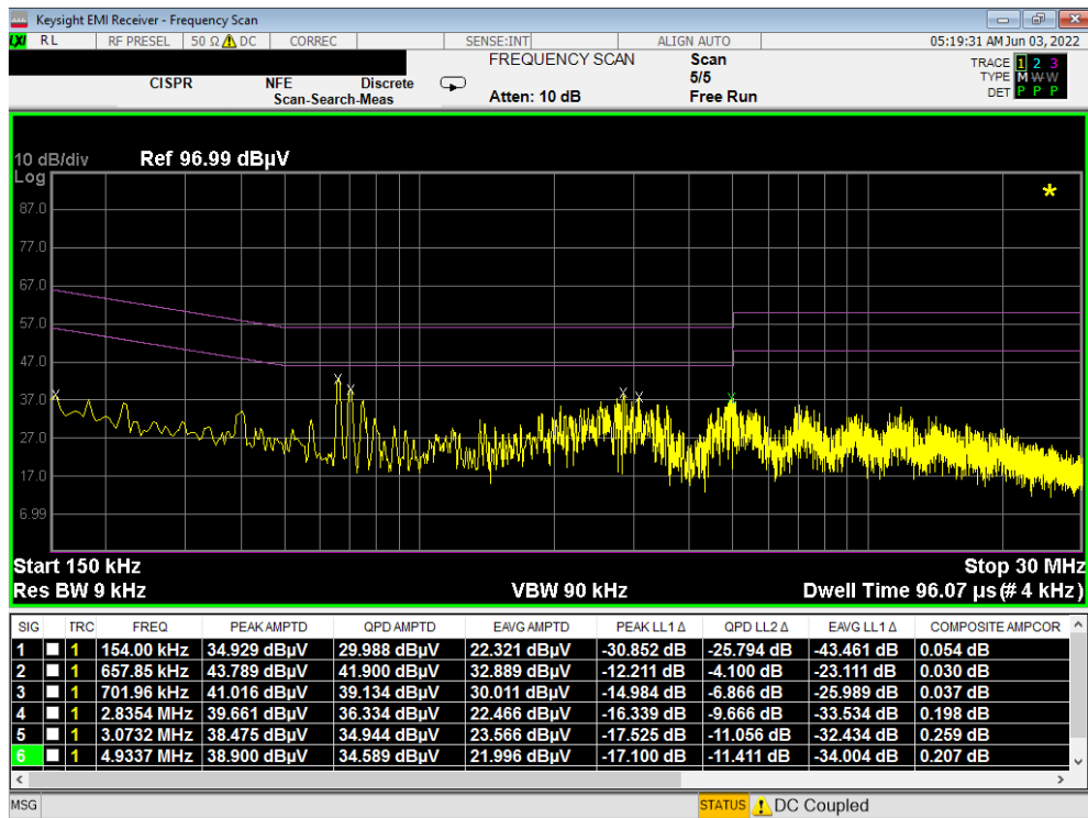
Plot 7-482. Line Conducted Plot with 802.11a UNII Band 1 (L1) – Closed
