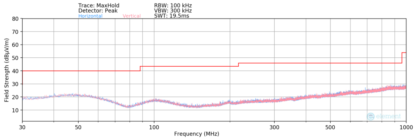
Plot 7-477. Radiated Spurious Plot below MIMO (802.11a – 2C Ch. 120)
