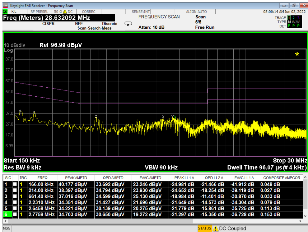
Plot 7-483. Line Conducted Plot with 802.11a UNII Band 1 (N) – Open
