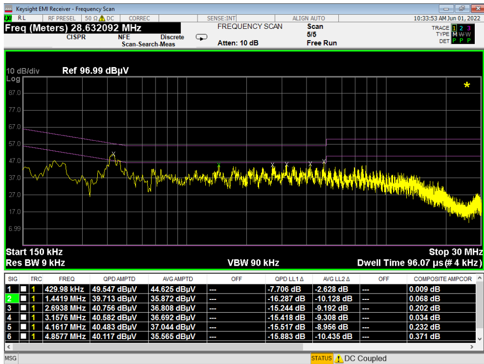
Plot 7-485. Line Conducted Plot with 802.11a UNII Band 2A (L1) – Open
