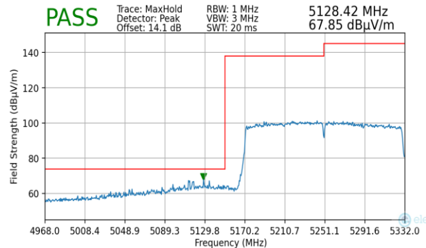
Plot 7-470. Radiated Lower Band Edge Plot MIMO (Peak – UNII Band 1)
