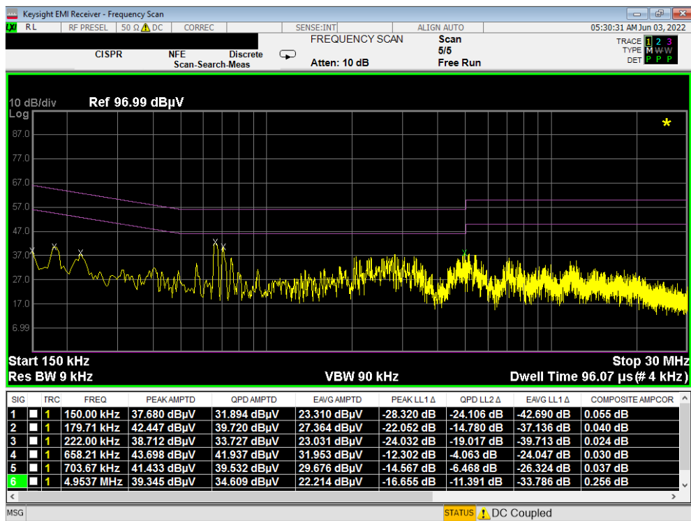
Plot 7-494. Line Conducted Plot with 802.11a UNII Band 3 (L1) – Closed
