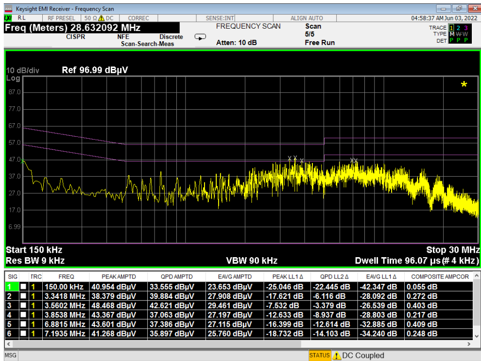
Plot 7-481. Line Conducted Plot with 802.11a UNII Band 1 (L1) – Open
