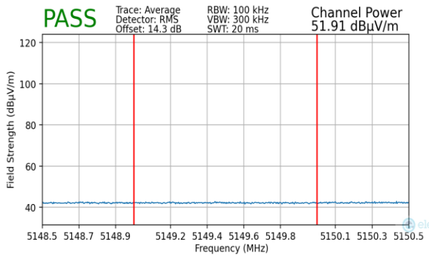
Plot 7-460. Radiated Lower Band Edge Plot MIMO (Average – UNII Band 1)
