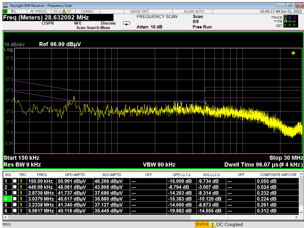
Plot 7-489. Line Conducted Plot with 802.11a UNII Band 2C (L1) – Open
