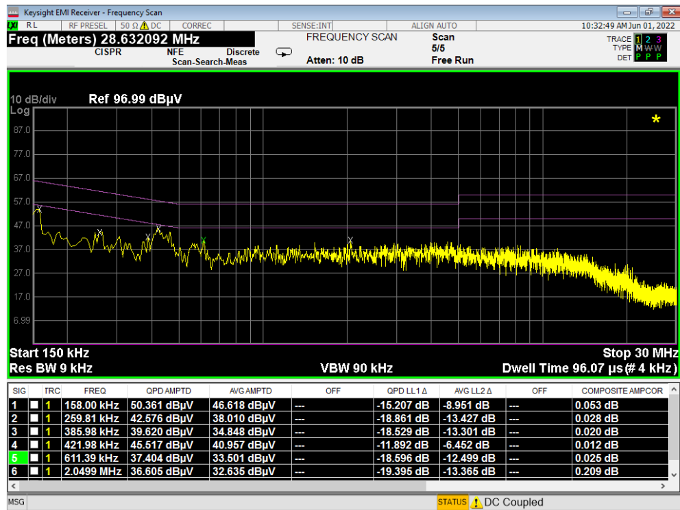
Plot 7-487. Line Conducted Plot with 802.11a UNII Band 2A (N) – Open
