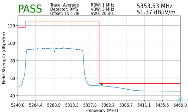
Plot 7-462. Radiated Upper Band Edge Plot MIMO (Average – UNII Band 2A)
