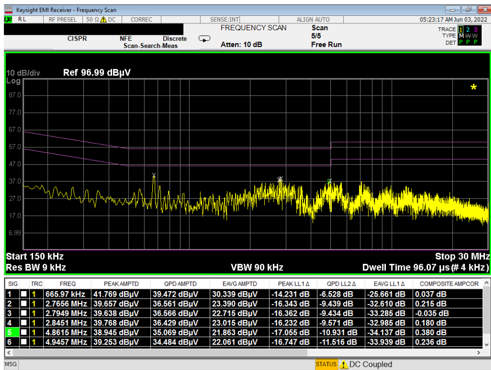
Plot 7-486. Line Conducted Plot with 802.11a UNII Band 2A (L1) – Closed
