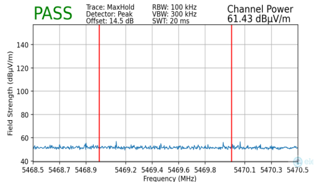
Plot 7-465. Radiated Lower Band Edge Plot MIMO (Peak – UNII Band 2C)
