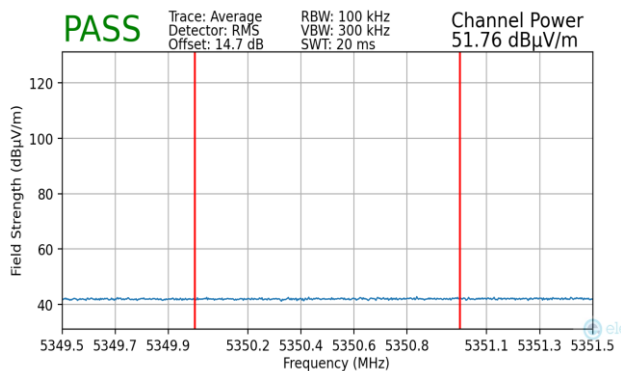
Plot 7-471. Radiated Upper Band Edge Plot MIMO (Average – UNII Band 2A)
