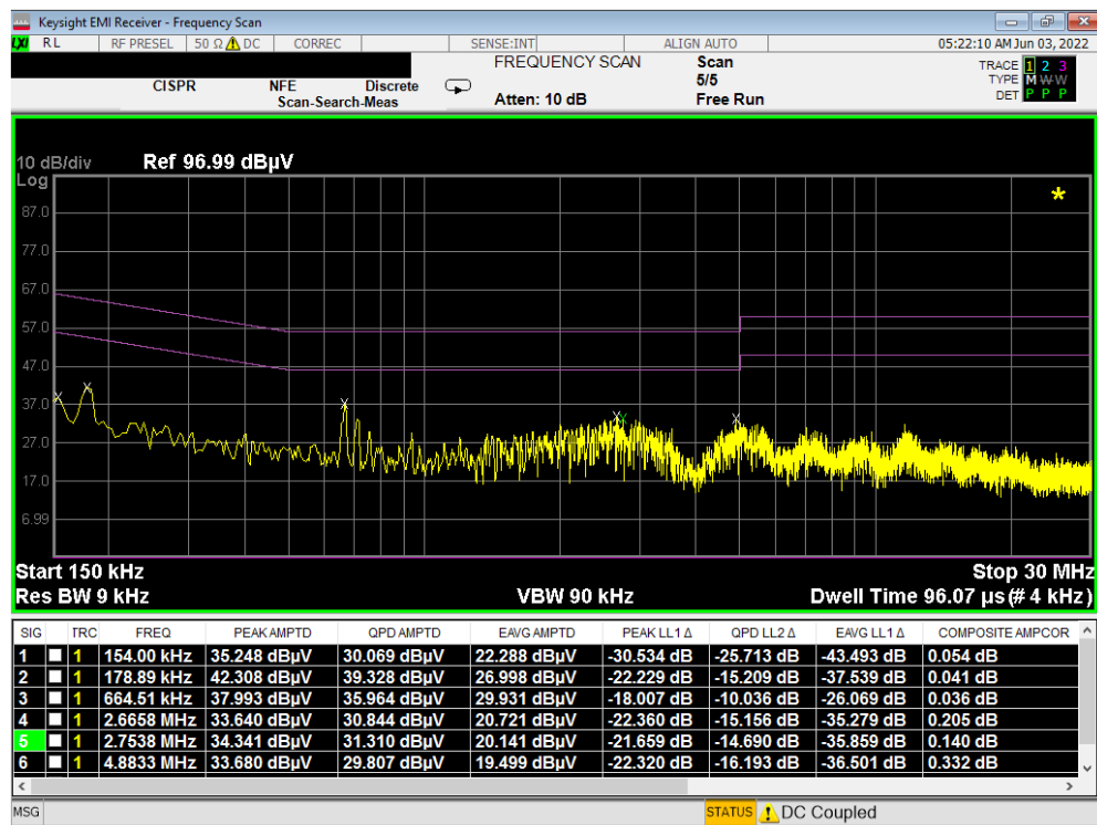
Plot 7-488. Line Conducted Plot with 802.11a UNII Band 2A (N) – Closed
