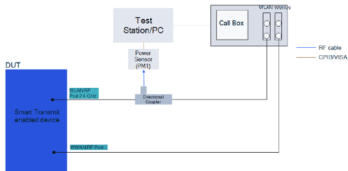
(e) Appendix A – Test Setup Photo 8
