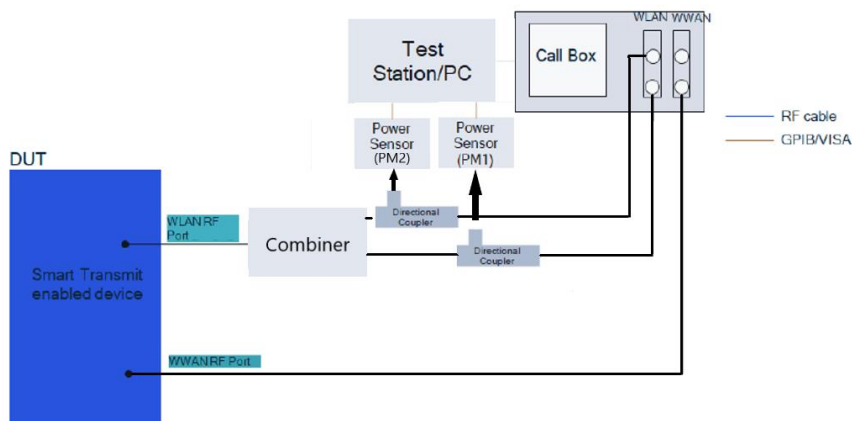
(f) Appendix A – Test Setup Photo 9
