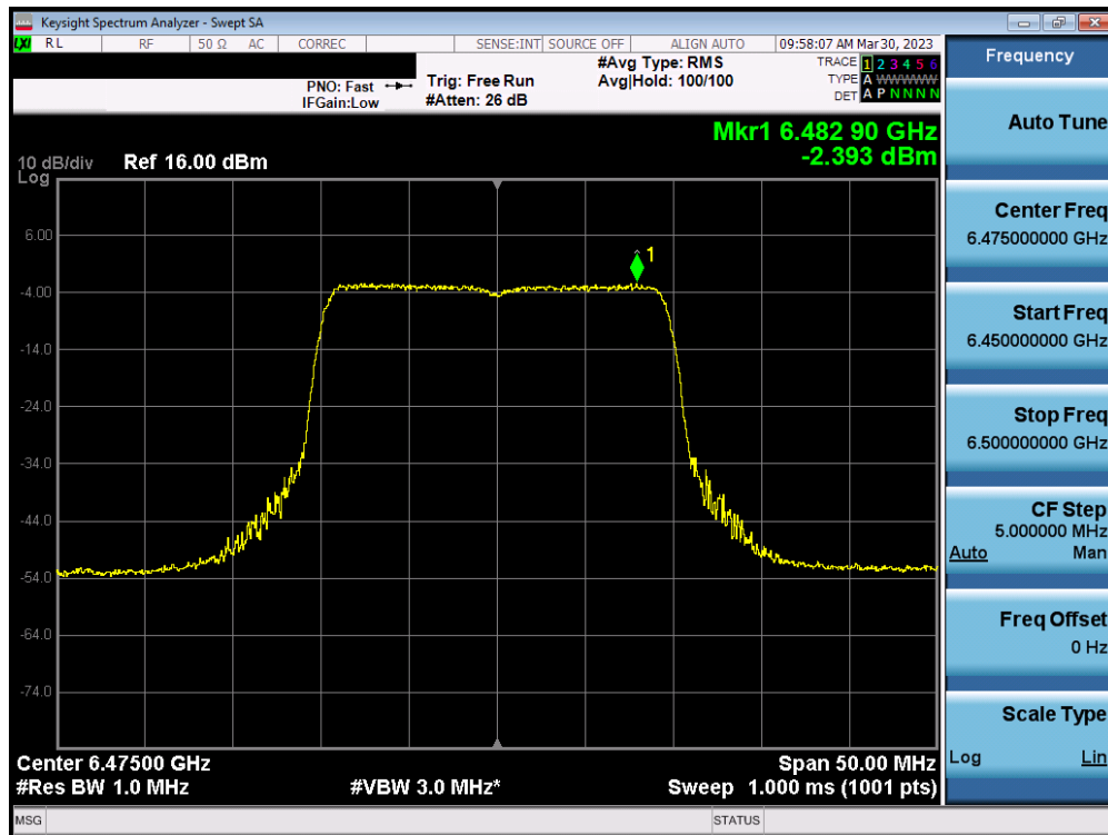
Plot 7-85. Power Spectral Density Plot MIMO ANT1 (20MHz BW 802.11ax (Full Tone) (UNII Band 6) – Ch. 105)
