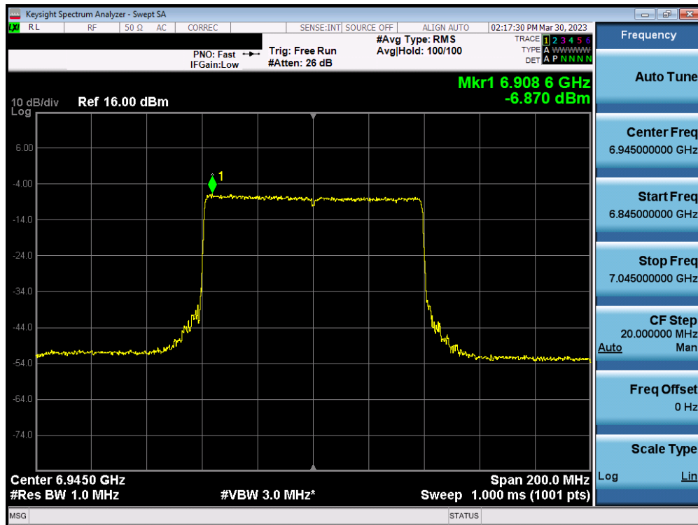
Plot 7-95. Power Spectral Density Plot MIMO ANT1 (80MHz BW 802.11ax (Full Tone) (UNII Band 8) – Ch. 199)
