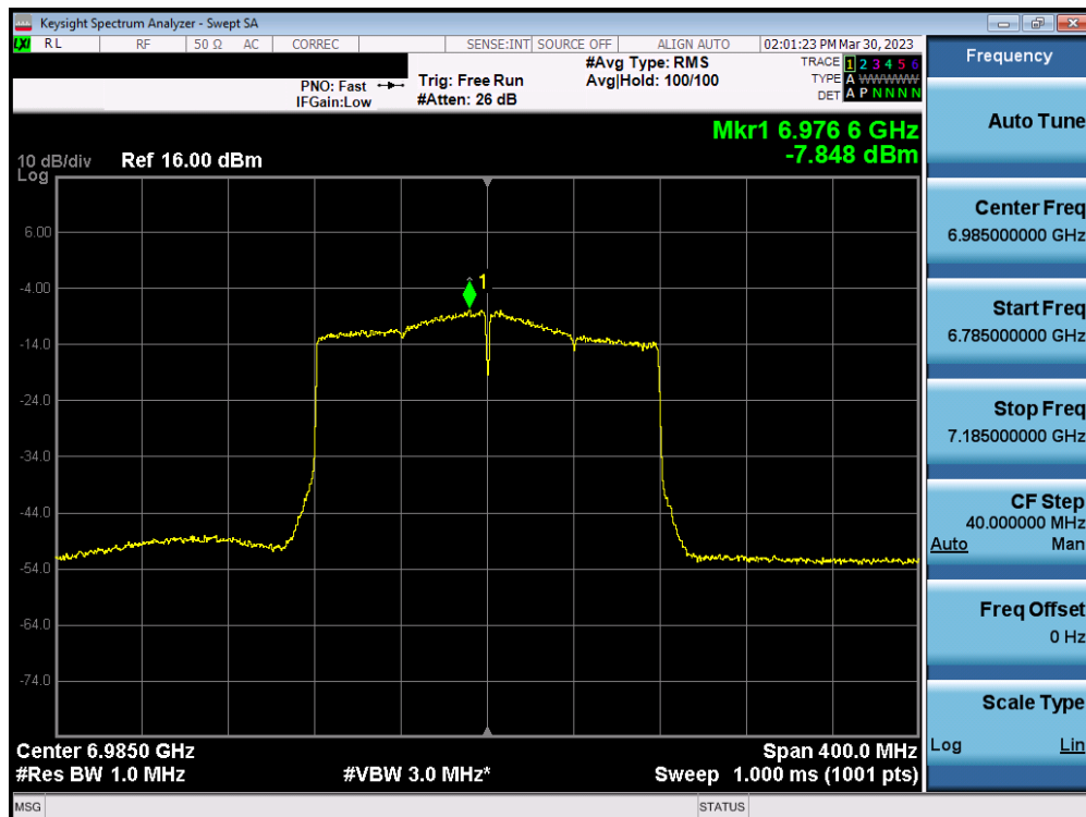
Plot 7-96. Power Spectral Density Plot MIMO ANT1 (160MHz BW 802.11ax (Full Tone) (UNII Band 8) – Ch. 207)
