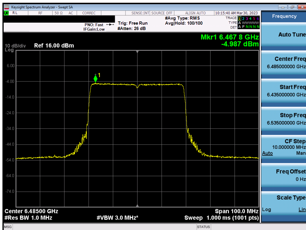
Plot 7-86. Power Spectral Density Plot MIMO ANT1 (40MHz BW 802.11ax (Full Tone) (UNII Band 6) – Ch. 107)
