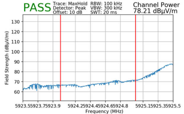
Plot 7-231. Radiated Lower Band Edge Plot MIMO (Peak – UNII Band 5 – 106T)
