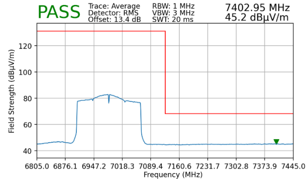
Plot 7-248. Radiated Upper Band Edge Plot MIMO (Average – UNII Band 8 – 2x996T)
