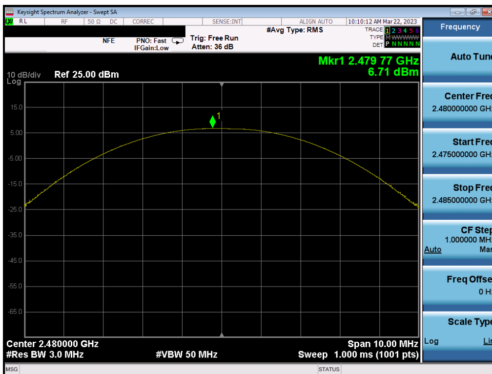
Plot 7-42. Peak Power Plot (Bluetooth (LE), 500kbps – Ch. 39) – ANT 2
