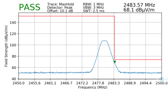
Plot 7-104. Radiated Restricted Upper Band Edge Measurement (Peak) – ANT 2
