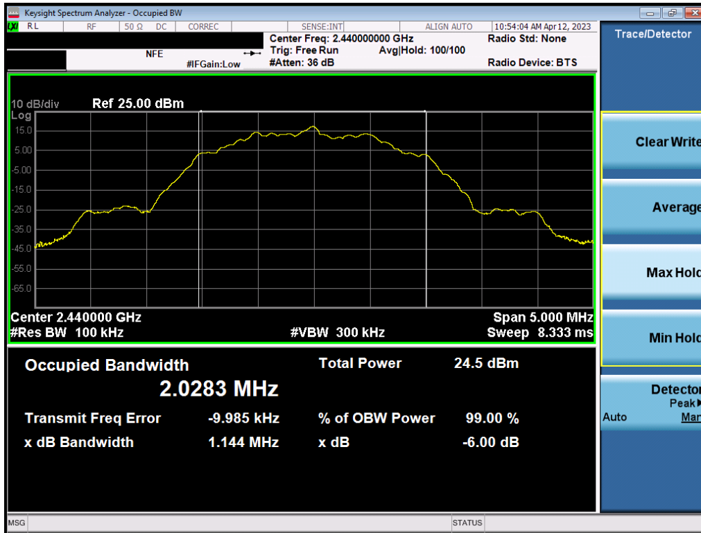
Plot 7-23. 6dB Bandwidth Plot (Bluetooth (LE), 2Mbps – Ch. 19) – ANT 2
