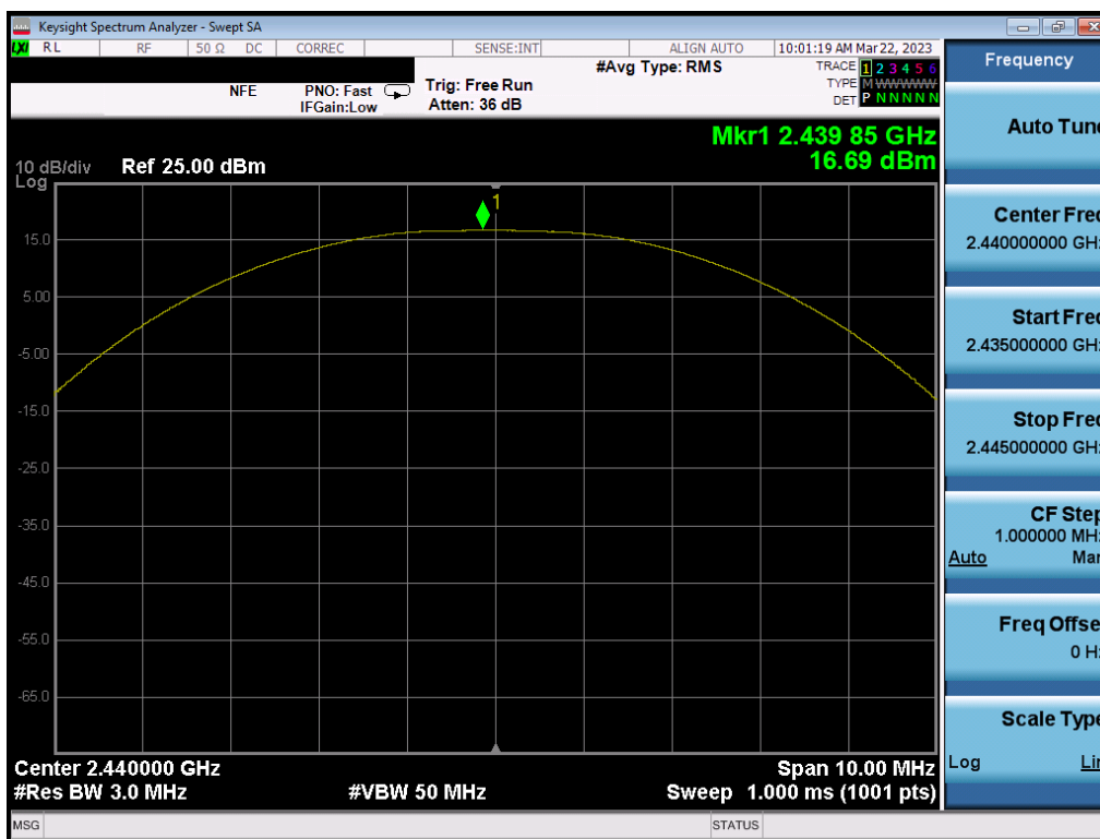
Plot 7-35. Peak Power Plot (Bluetooth (LE), 2Mbps – Ch. 19) – ANT 1
