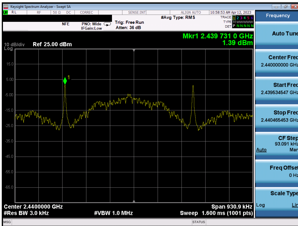
Plot 7-62. Power Spectral Density Plot (Bluetooth (LE), 125kbps – Ch. 19) – ANT 2
