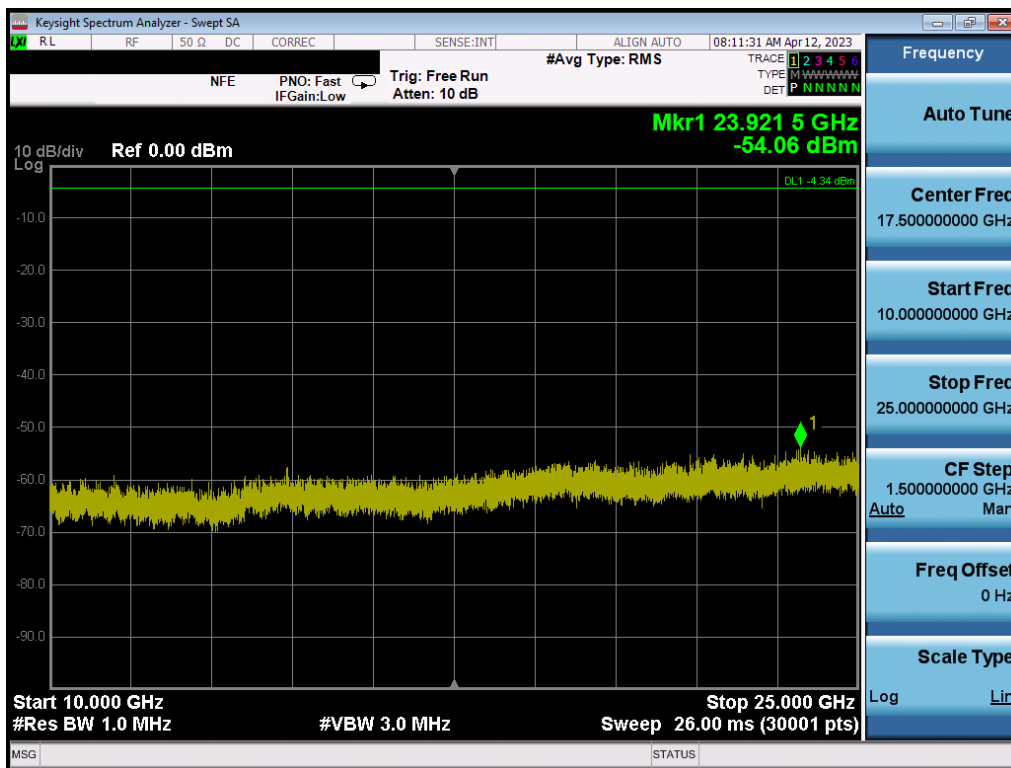
Plot 7-92. Conducted Spurious Plot (Bluetooth (LE), 1Mbps - Ch. 19) - ANT 1
