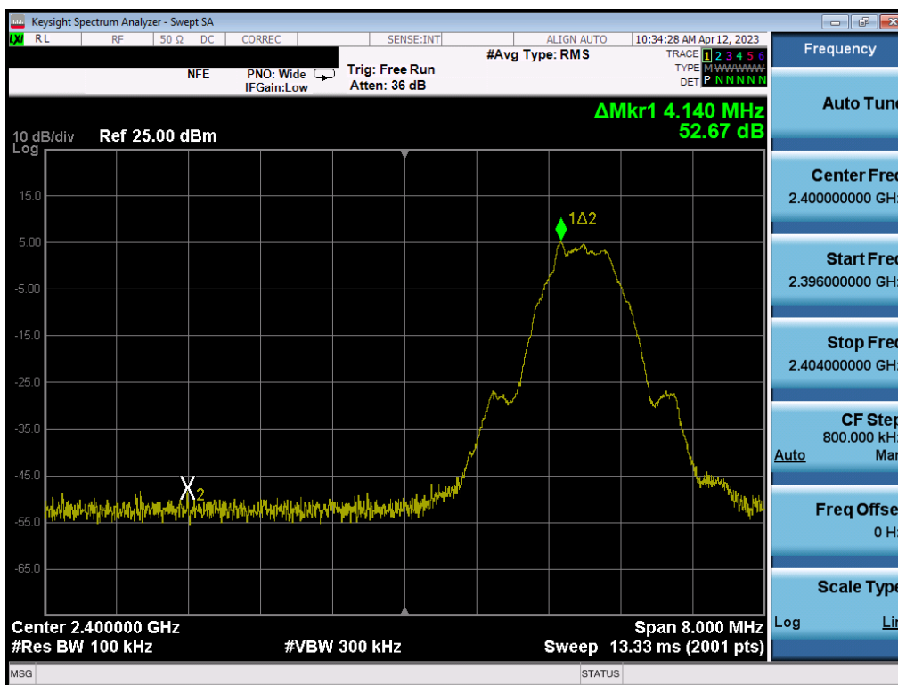
Plot 7-75. Band Edge Plot (Bluetooth (LE), 500kbps – Ch. 0) – ANT 1
