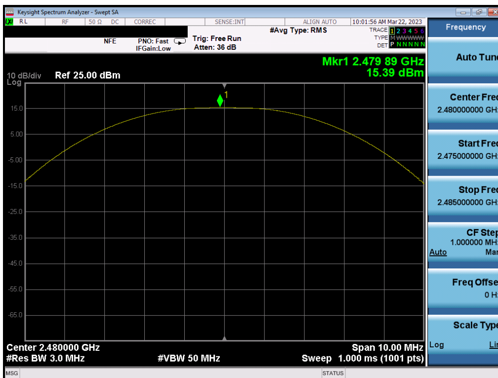
Plot 7-36. Peak Power Plot (Bluetooth (LE), 2Mbps – Ch. 39) – ANT 1
