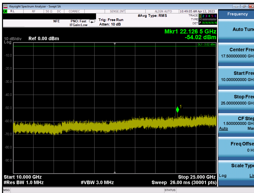
Plot 7-96. Conducted Spurious Plot (Bluetooth (LE), 1Mbps – Ch. 0) – ANT 2
