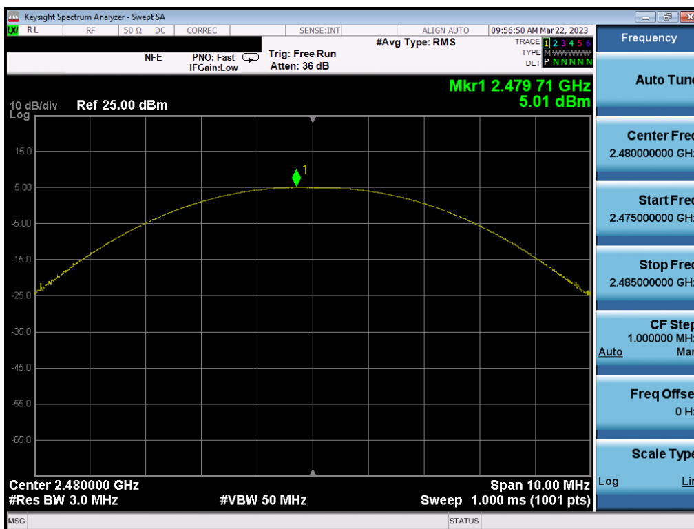
Plot 7-30. Peak Power Plot (Bluetooth (LE), 500kbps – Ch. 39) – ANT 1
