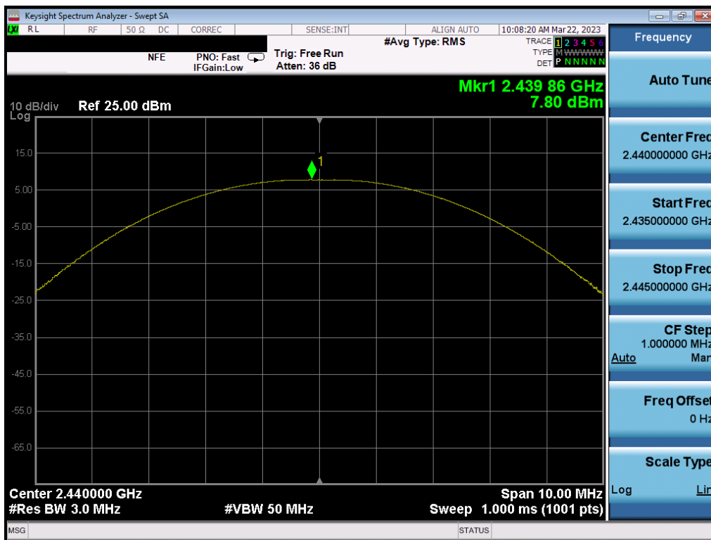
Plot 7-38. Peak Power Plot (Bluetooth (LE), 125kbps – Ch. 19) – ANT 2
