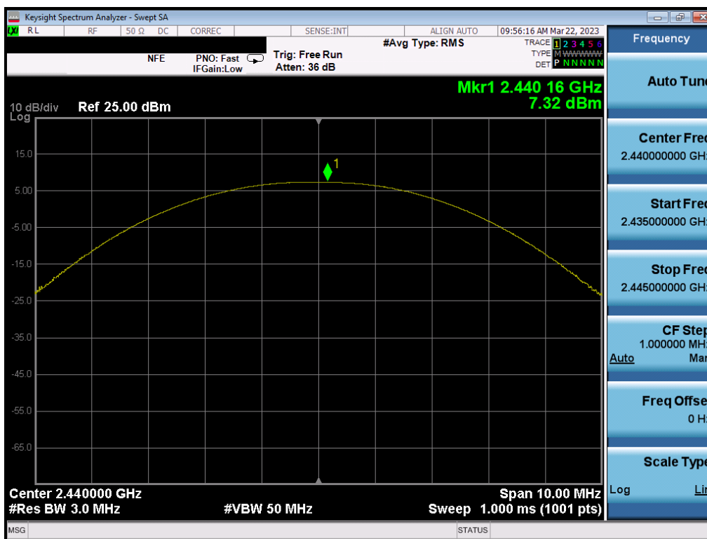
Plot 7-29. Peak Power Plot (Bluetooth (LE), 500kbps – Ch. 19) – ANT 1
