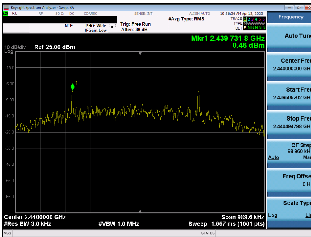
Plot 7-53. Power Spectral Density Plot (Bluetooth (LE), 500kbps – Ch. 19) – ANT 1
