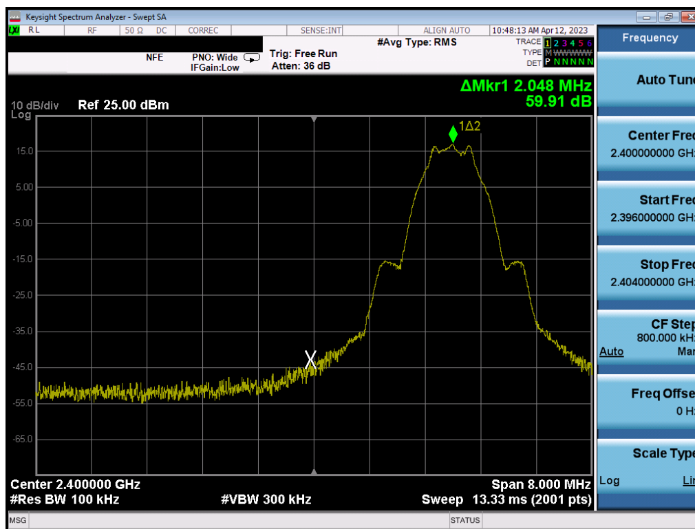
Plot 7-85. Band Edge Plot (Bluetooth (LE), 1Mbps – Ch. 0) – ANT 2
