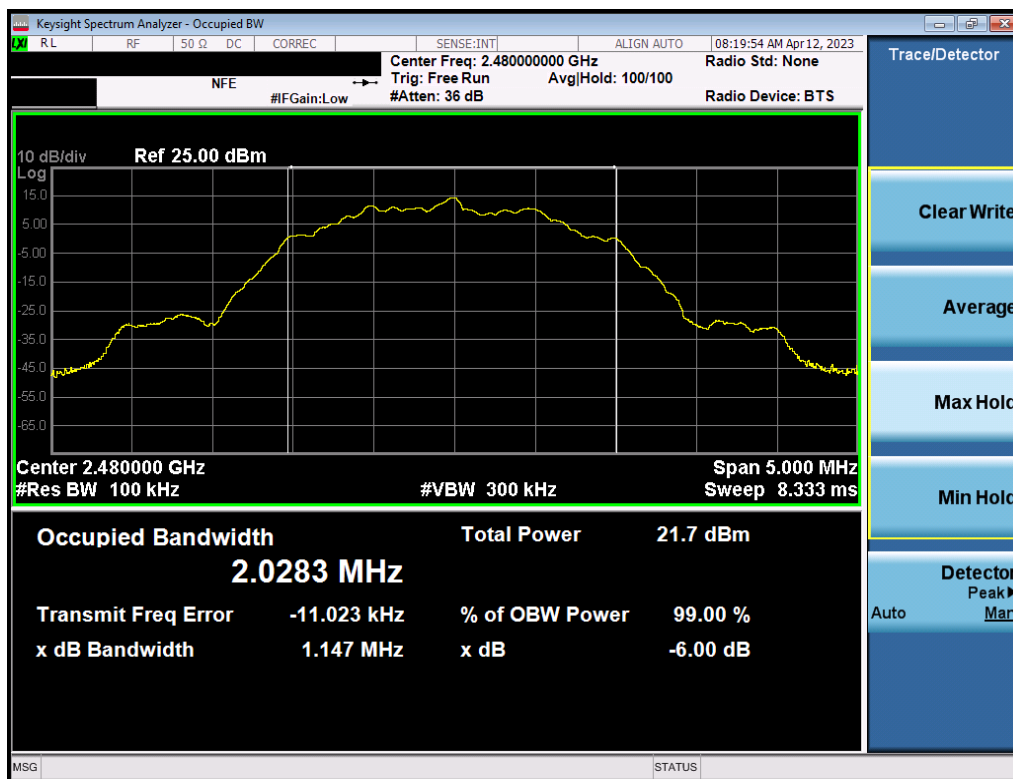
Plot 7-12. 6dB Bandwidth Plot (Bluetooth (LE), 2Mbps – Ch. 39) – ANT 1
