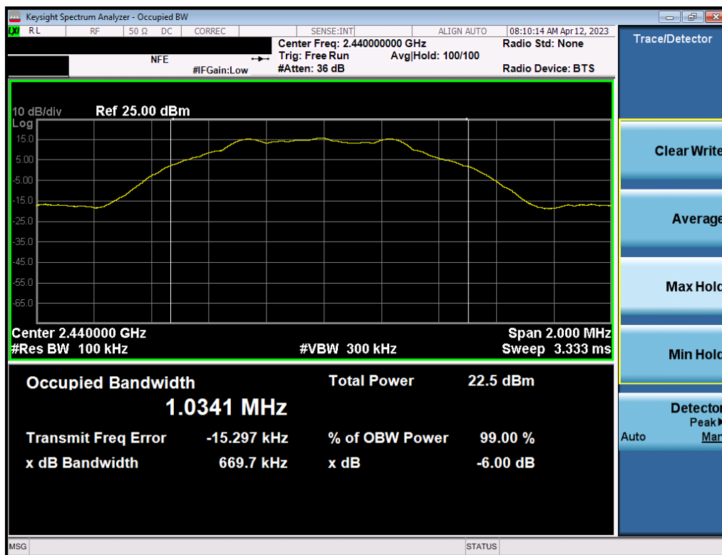
Plot 7-8. 6dB Bandwidth Plot (Bluetooth (LE), 1Mbps – Ch. 19) – ANT 1
