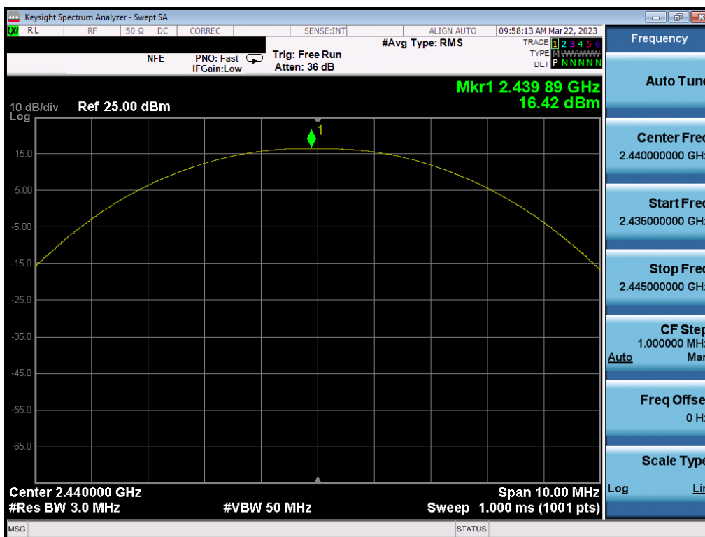
Plot 7-32. Peak Power Plot (Bluetooth (LE), 1Mbps – Ch. 19) – ANT 1
