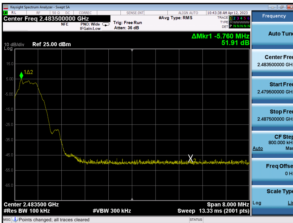
Plot 7-76. Band Edge Plot (Bluetooth (LE), 500kbps – Ch. 39) – ANT 1
