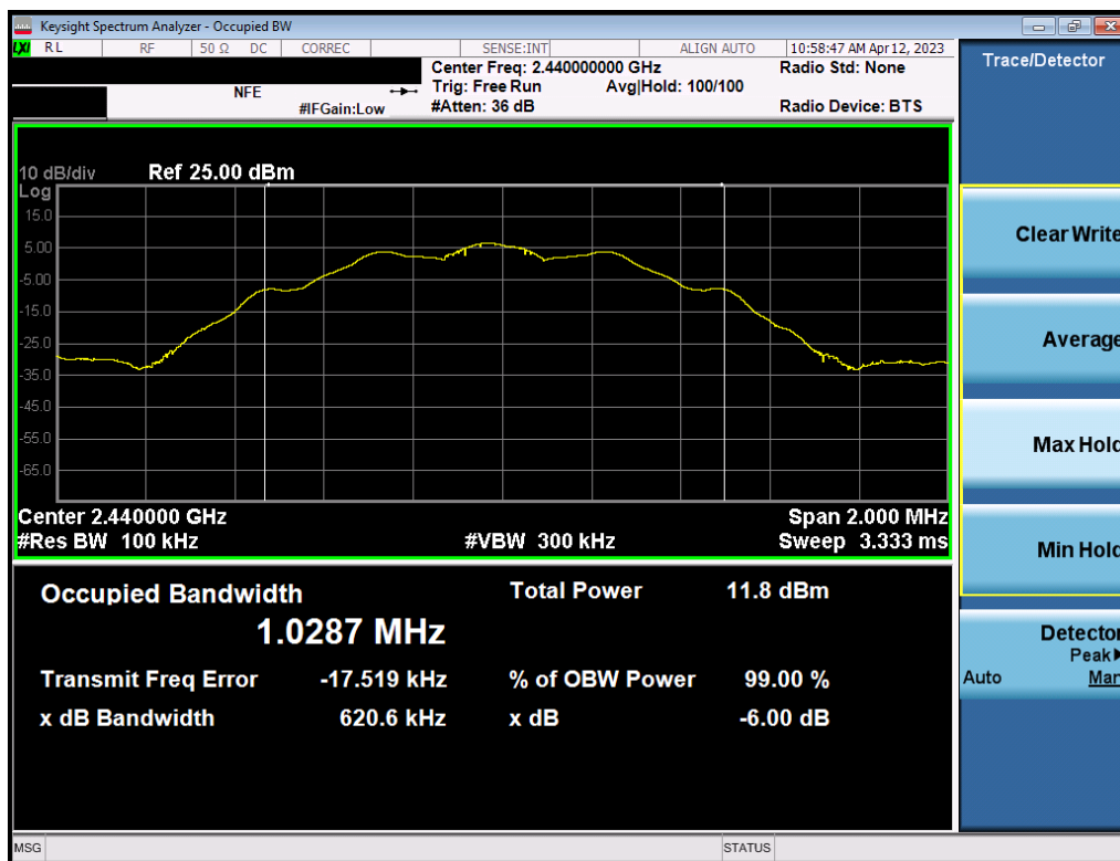
Plot 7-14. 6dB Bandwidth Plot (Bluetooth (LE), 125kbps – Ch. 19) – ANT 2
