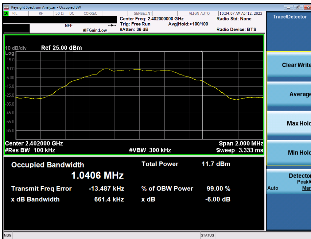
Plot 7-4. 6dB Bandwidth Plot (Bluetooth (LE), 500kbps – Ch. 0) – ANT 1
