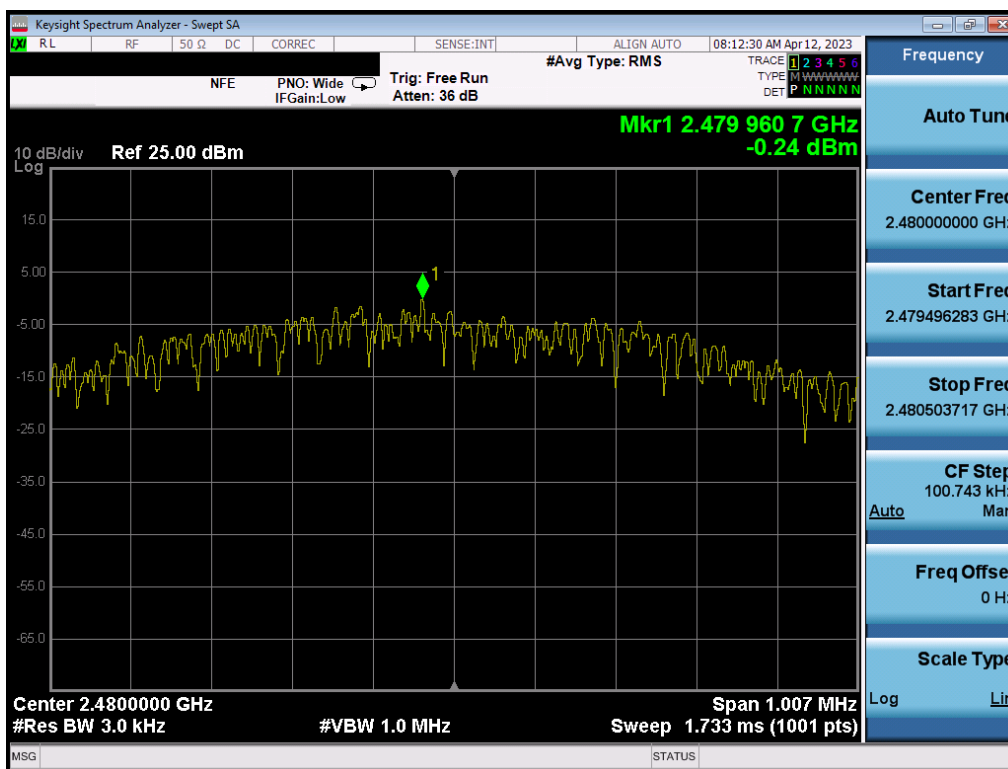
Plot 7-57. Power Spectral Density Plot (Bluetooth (LE), 1Mbps – Ch. 39) – ANT 1
