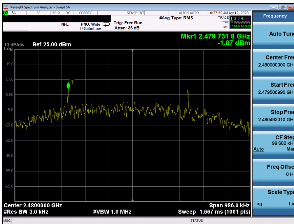
Plot 7-54. Power Spectral Density Plot (Bluetooth (LE), 500kbps – Ch. 39) – ANT 1
