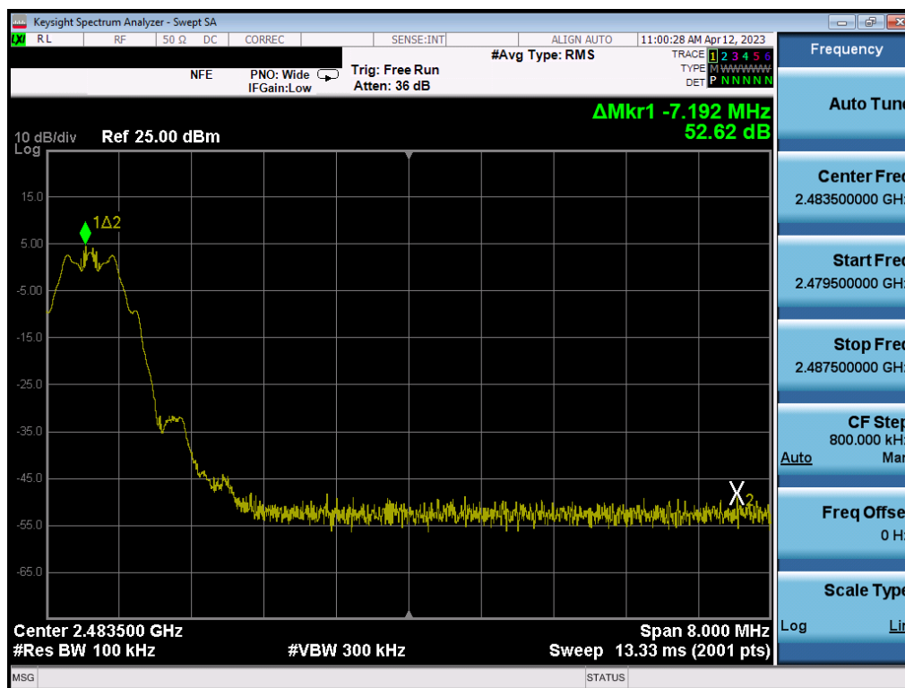
Plot 7-82. Band Edge Plot (Bluetooth (LE), 125kbps – Ch. 39) – ANT 2
