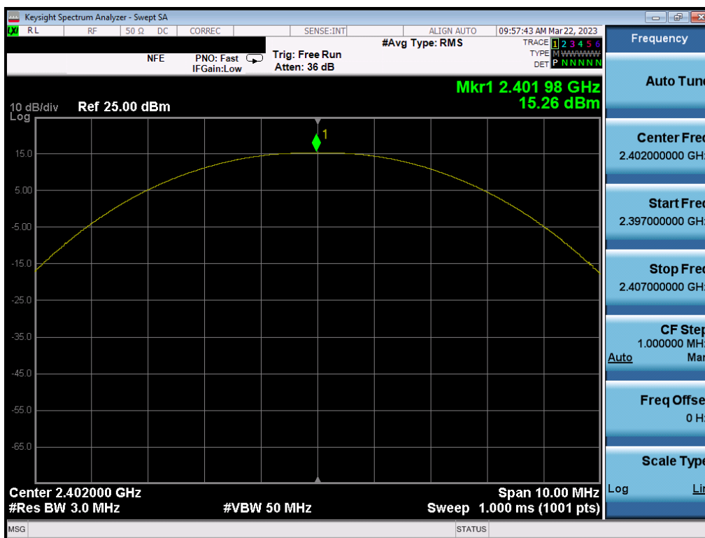
Plot 7-31. Peak Power Plot (Bluetooth (LE), 1Mbps – Ch. 0) – ANT 1
