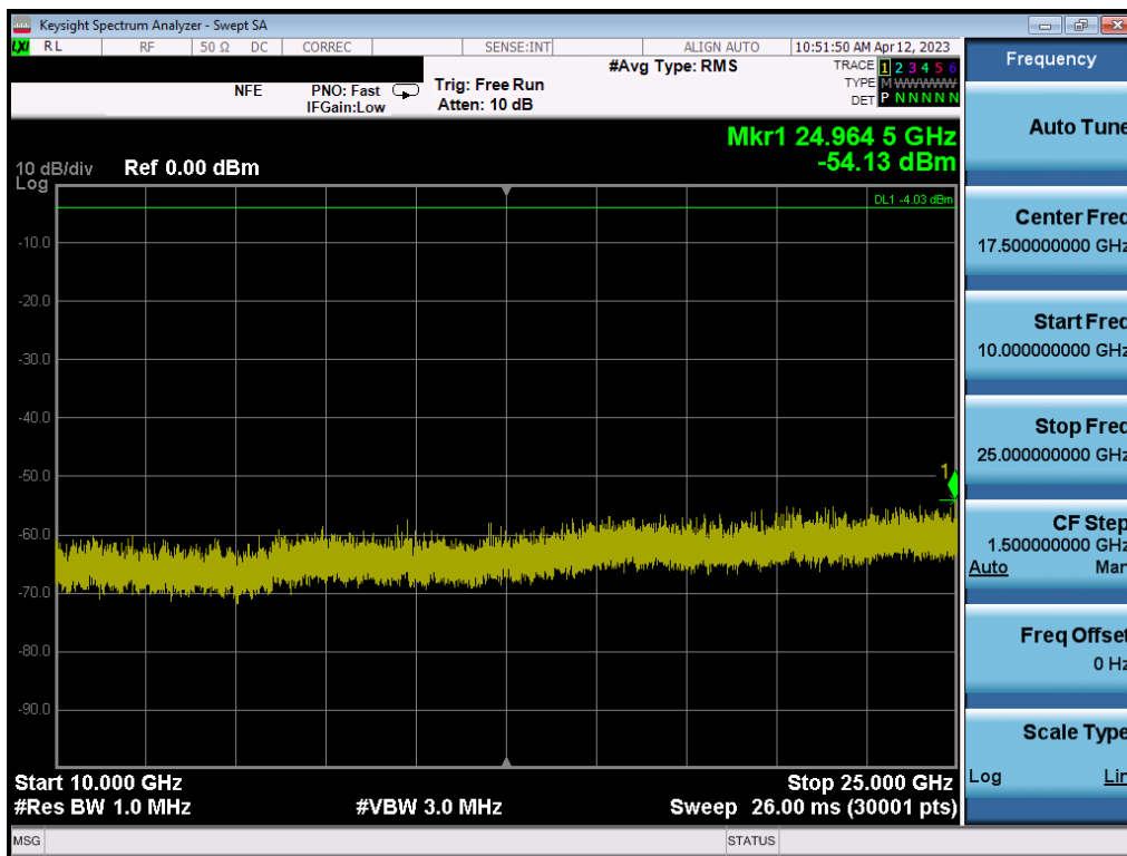
Plot 7-100. Conducted Spurious Plot (Bluetooth (LE), 1Mbps – Ch. 39) – ANT 2
