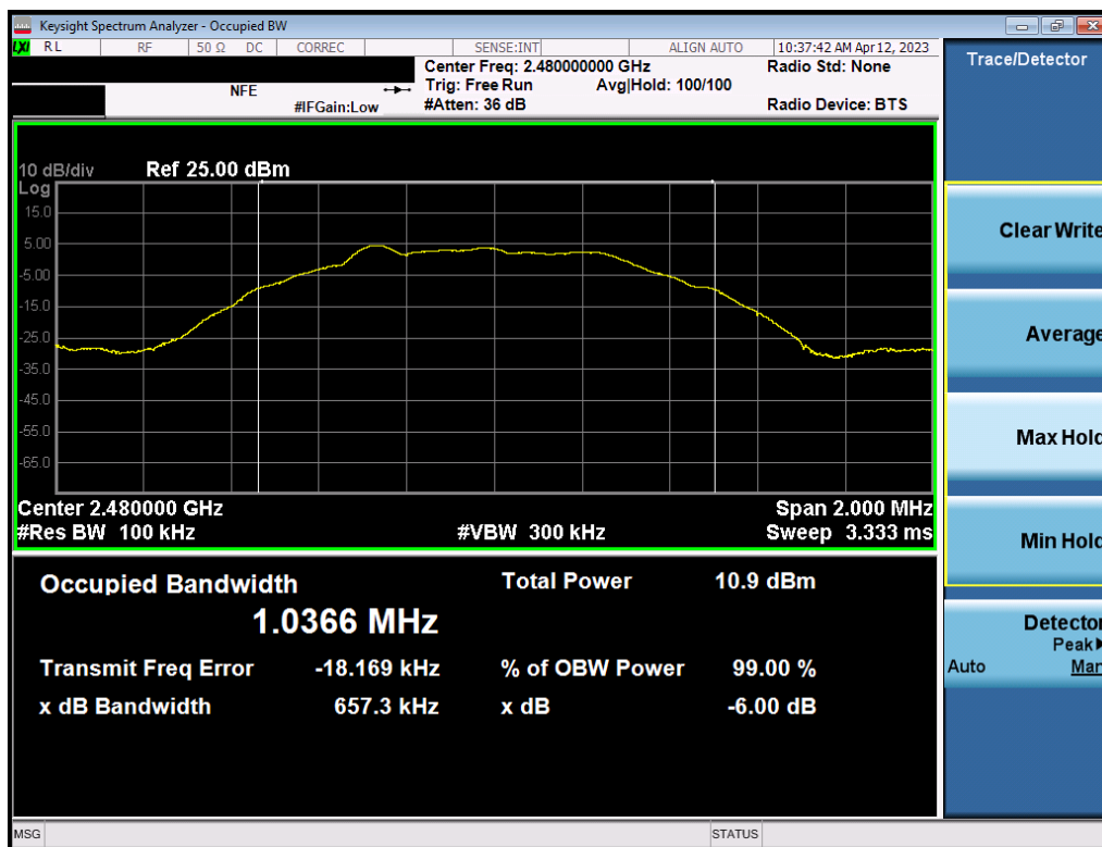
Plot 7-6. 6dB Bandwidth Plot (Bluetooth (LE), 500kbps – Ch. 39) – ANT 1
