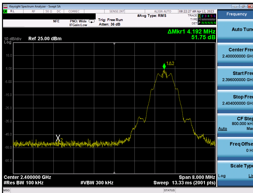
Plot 7-73. Band Edge Plot (Bluetooth (LE), 125kbps – Ch. 0) – ANT 1
