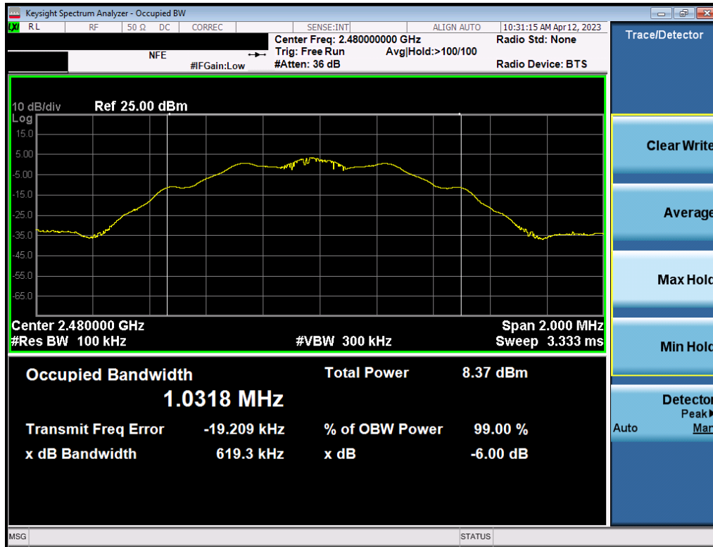
Plot 7-3. 6dB Bandwidth Plot (Bluetooth (LE), 125kbps – Ch. 39) – ANT 1
