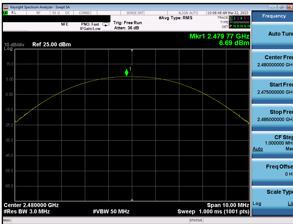
Plot 7-39. Peak Power Plot (Bluetooth (LE), 125kbps – Ch. 39) – ANT 2
