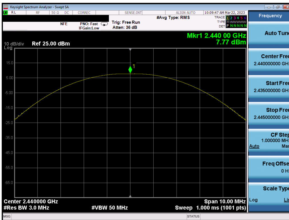
Plot 7-41. Peak Power Plot (Bluetooth (LE), 500kbps – Ch. 19) – ANT 2
