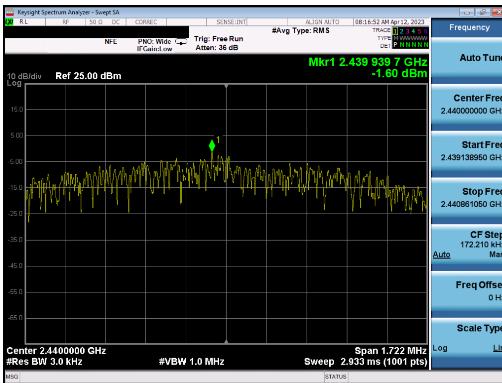
Plot 7-59. Power Spectral Density Plot (Bluetooth (LE), 2Mbps – Ch. 19) – ANT 1
