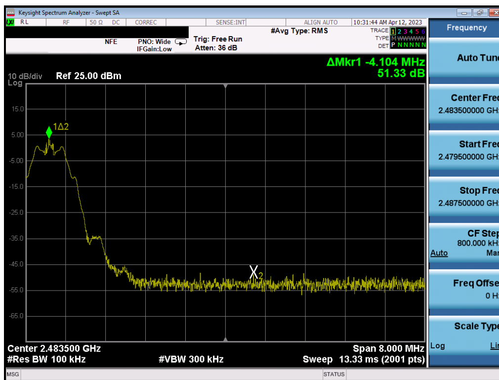
Plot 7-74. Band Edge Plot (Bluetooth (LE), 125kbps – Ch. 39) – ANT 1
