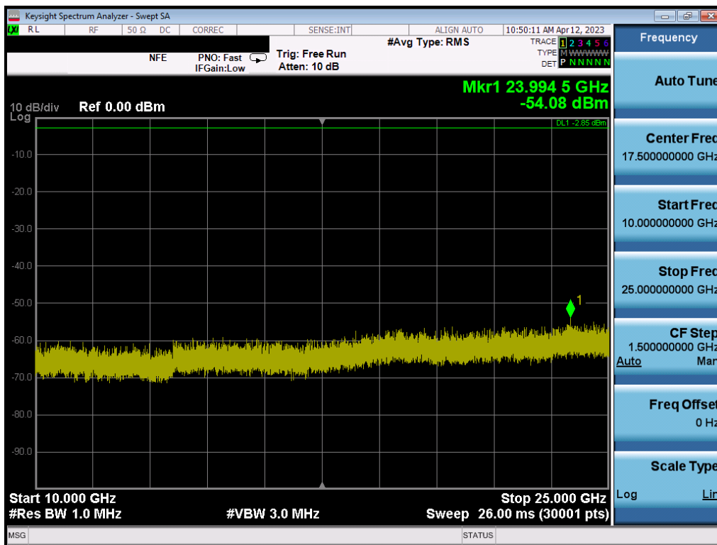
Plot 7-98. Conducted Spurious Plot (Bluetooth (LE), 1Mbps – Ch. 19) – ANT 2
