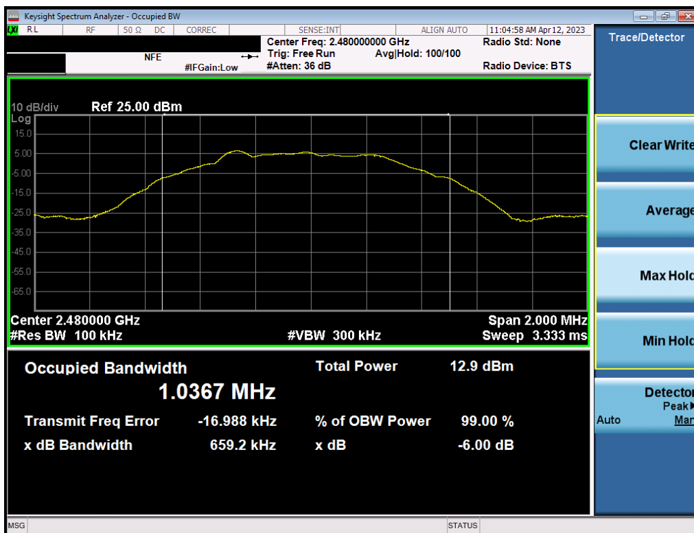
Plot 7-18. 6dB Bandwidth Plot (Bluetooth (LE), 500kbps – Ch. 39) – ANT 2
