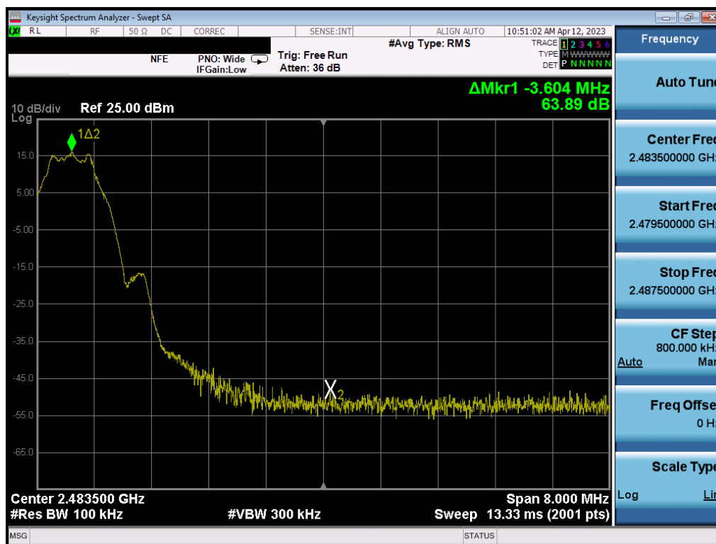
Plot 7-86. Band Edge Plot (Bluetooth (LE), 1Mbps – Ch. 39) – ANT 2
