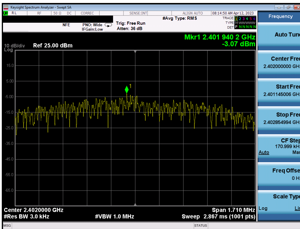
Plot 7-58. Power Spectral Density Plot (Bluetooth (LE), 2Mbps – Ch. 0) – ANT 1
