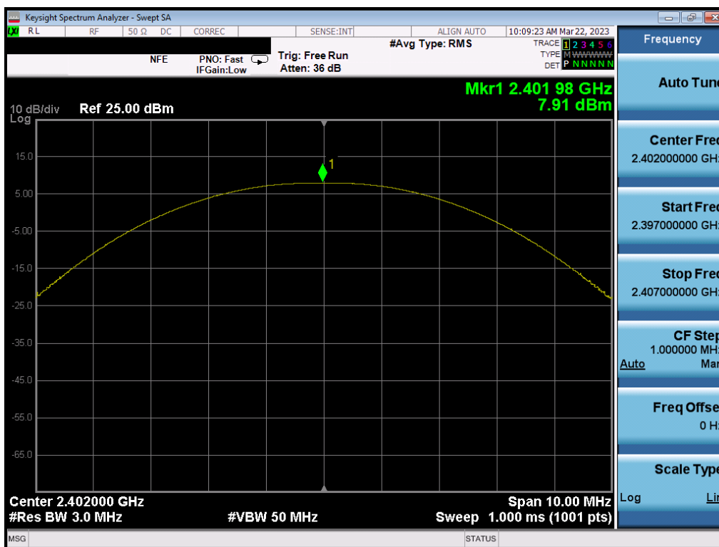
Plot 7-40. Peak Power Plot (Bluetooth (LE), 500kbps – Ch. 0) – ANT 2
