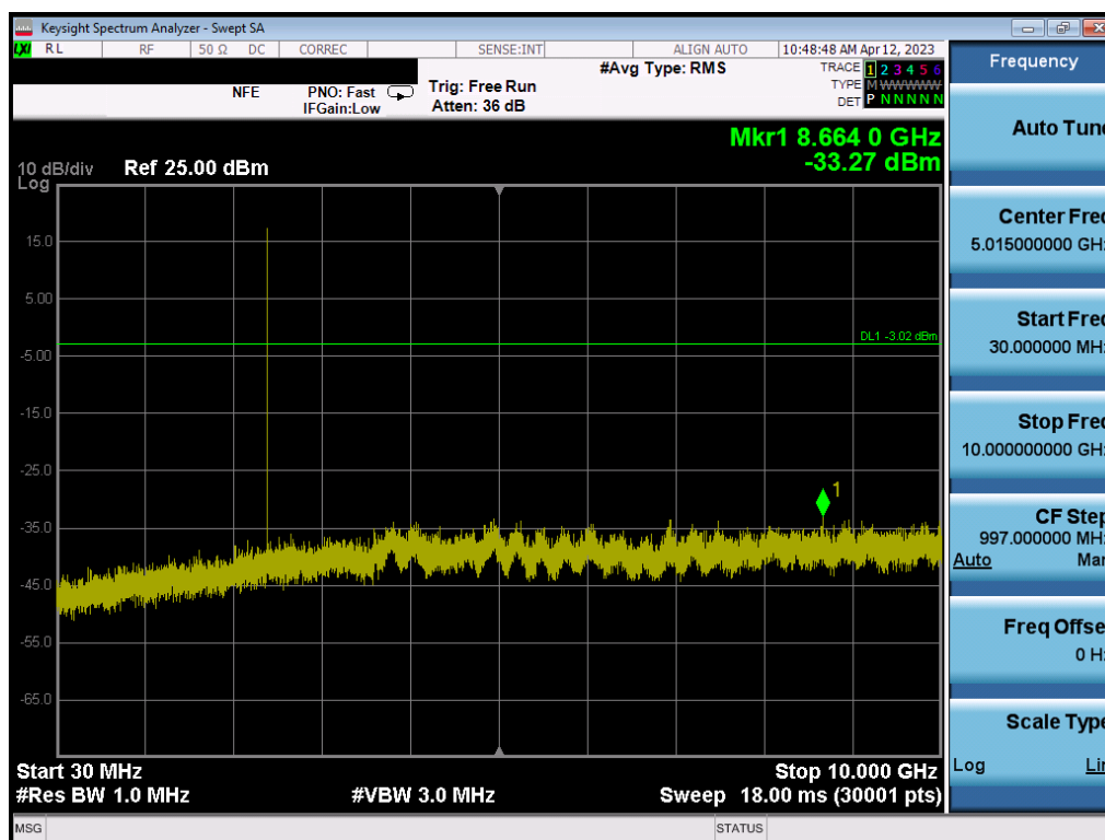
Plot 7-95. Conducted Spurious Plot (Bluetooth (LE), 1Mbps – Ch. 0) – ANT 2
