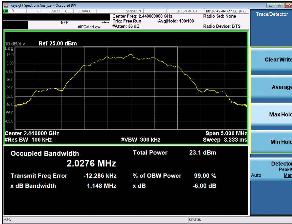
Plot 7-11. 6dB Bandwidth Plot (Bluetooth (LE), 2Mbps – Ch. 19) – ANT 1
