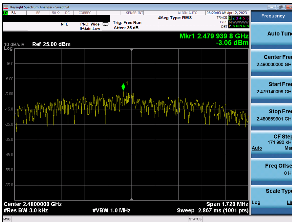
Plot 7-60. Power Spectral Density Plot (Bluetooth (LE), 2Mbps – Ch. 39) – ANT 1
