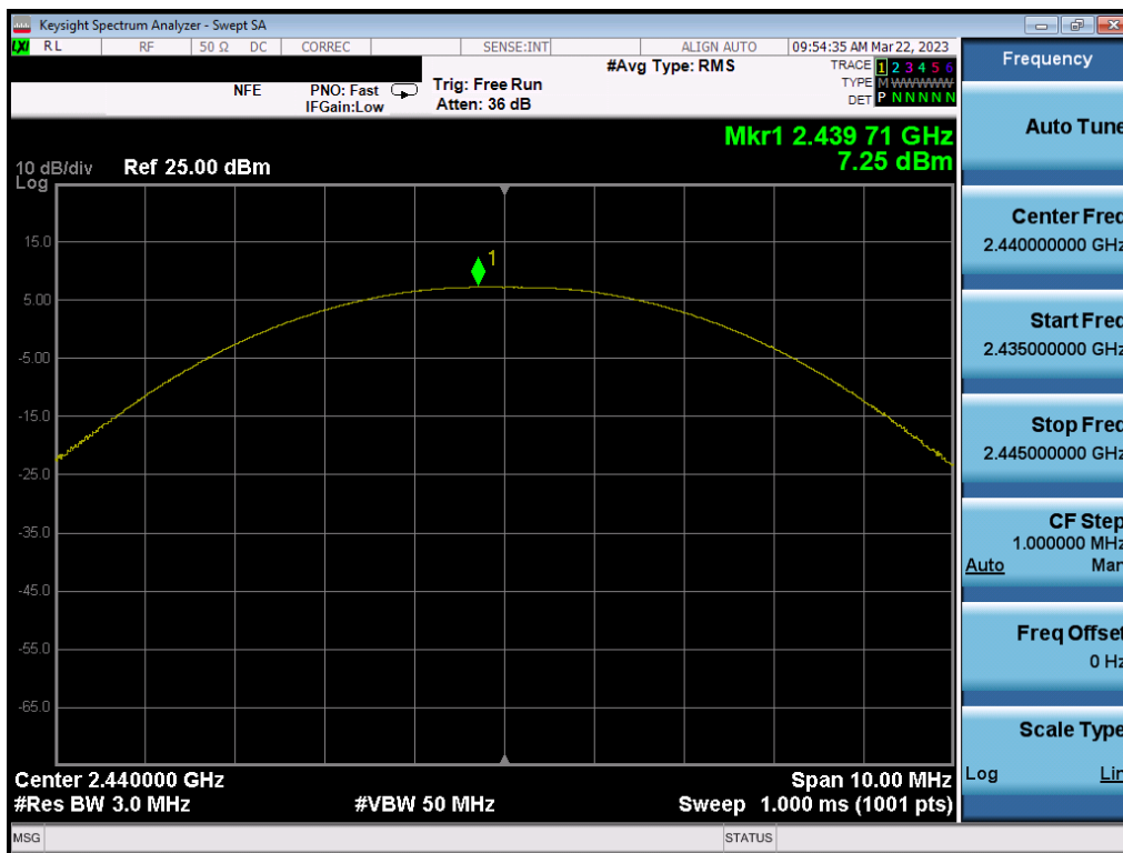
Plot 7-26. Peak Power Plot (Bluetooth (LE), 125kbps – Ch. 19) – ANT 1
