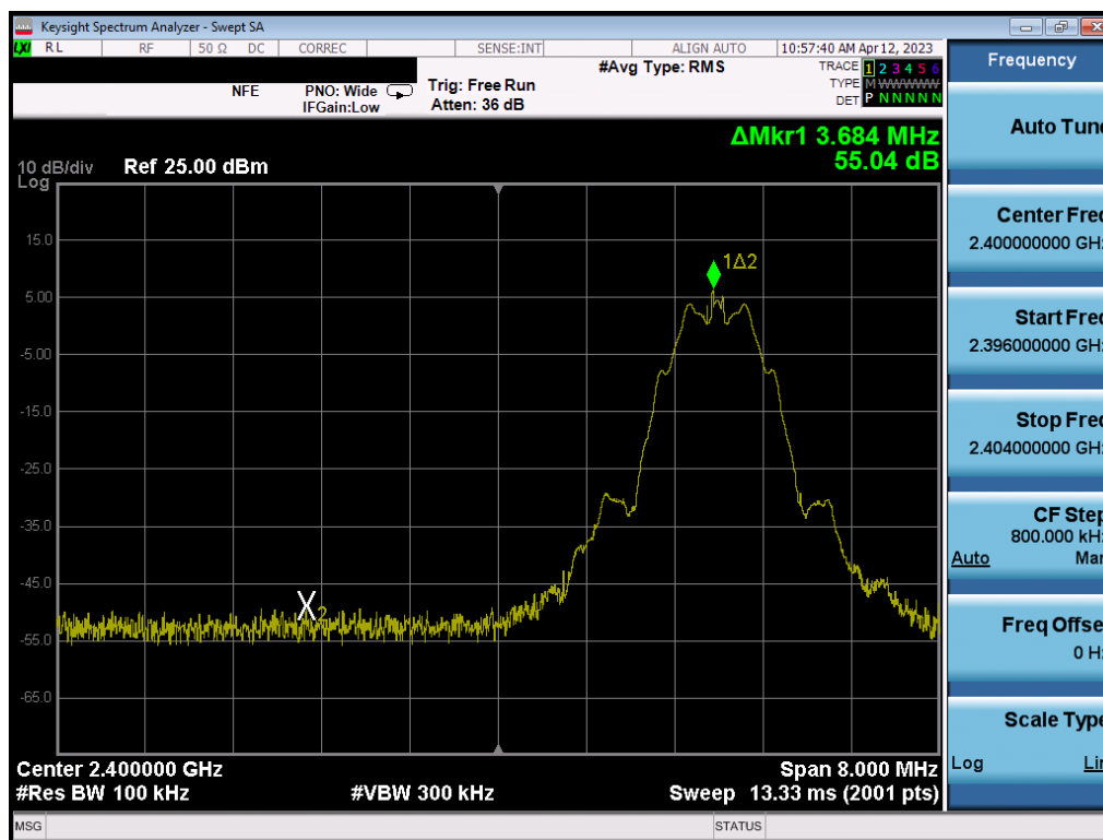
Plot 7-81. Band Edge Plot (Bluetooth (LE), 125kbps – Ch. 0) – ANT 2
