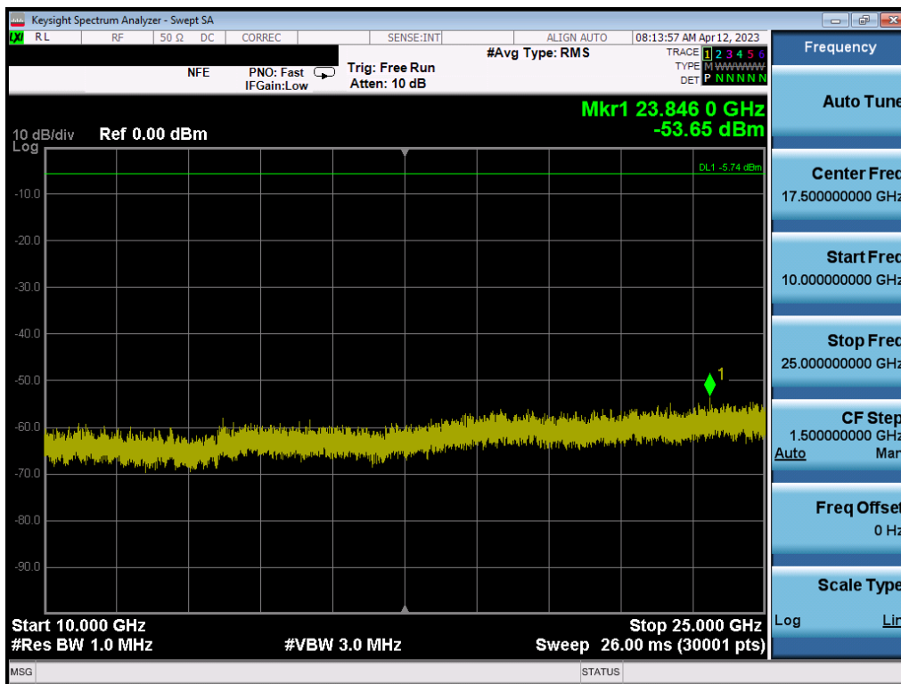
Plot 7-94. Conducted Spurious Plot (Bluetooth (LE), 1Mbps - Ch. 39) - ANT 1
