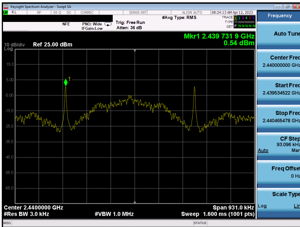
Plot 7-50. Power Spectral Density Plot (Bluetooth (LE), 125kbps – Ch. 19) – ANT 1
