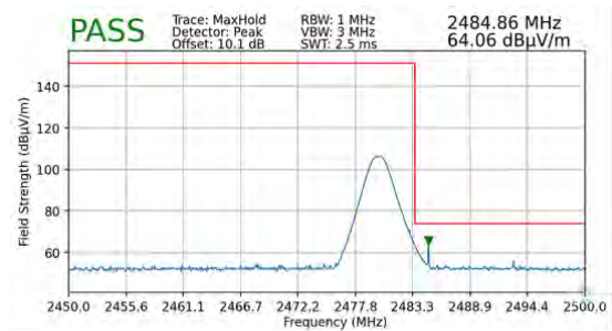
Plot 7-104. Radiated Restricted Upper Band Edge Measurement (Peak) – ANT2
