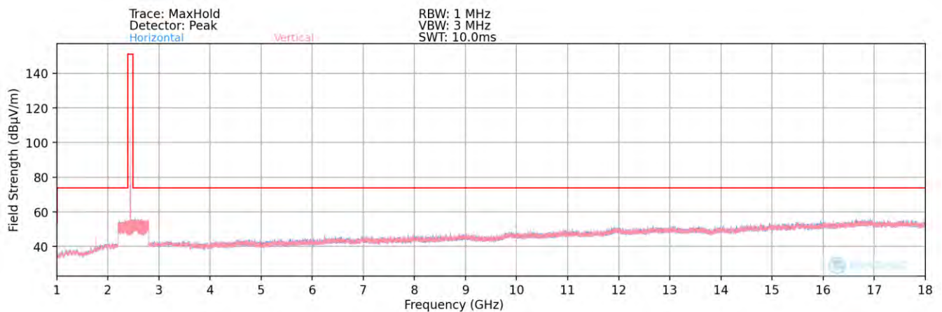
Plot 7-85. Radiated Spurious Plot above 1GHz (BT– Ch. 39) – ANT1 Open
