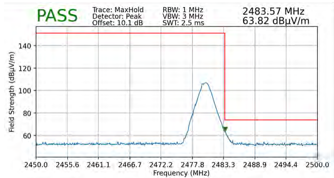
Plot 7-100. Radiated Restricted Upper Band Edge Measurement (Peak) – ANT1
