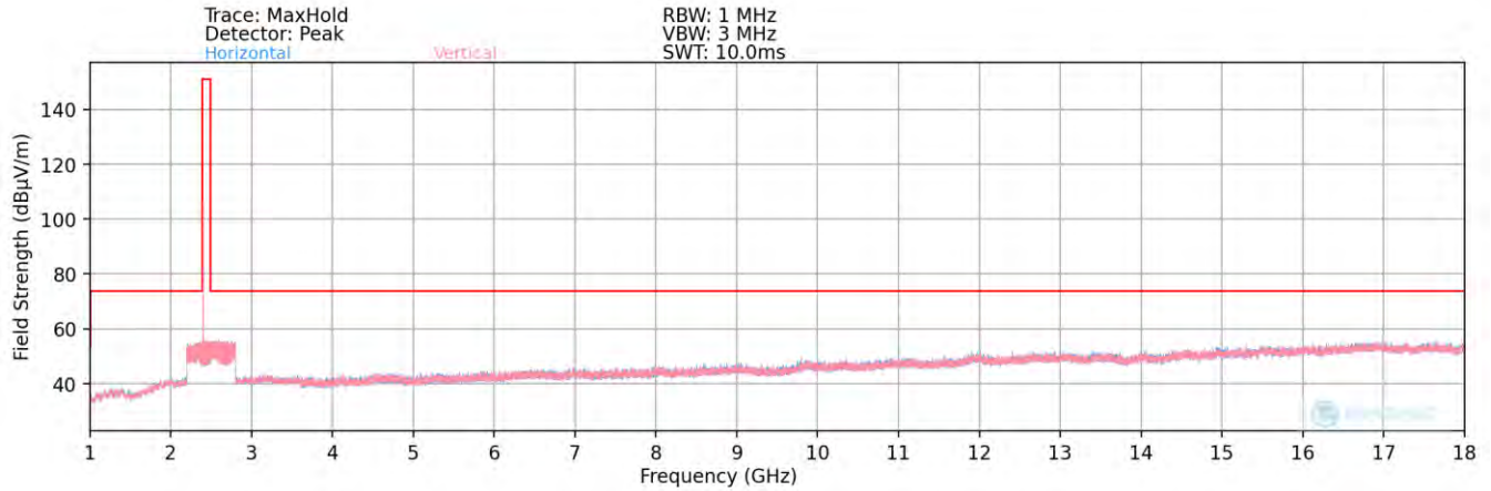
Plot 7-91. Radiated Spurious Plot above 1GHz (BT– Ch. 0) – ANT2 Open
