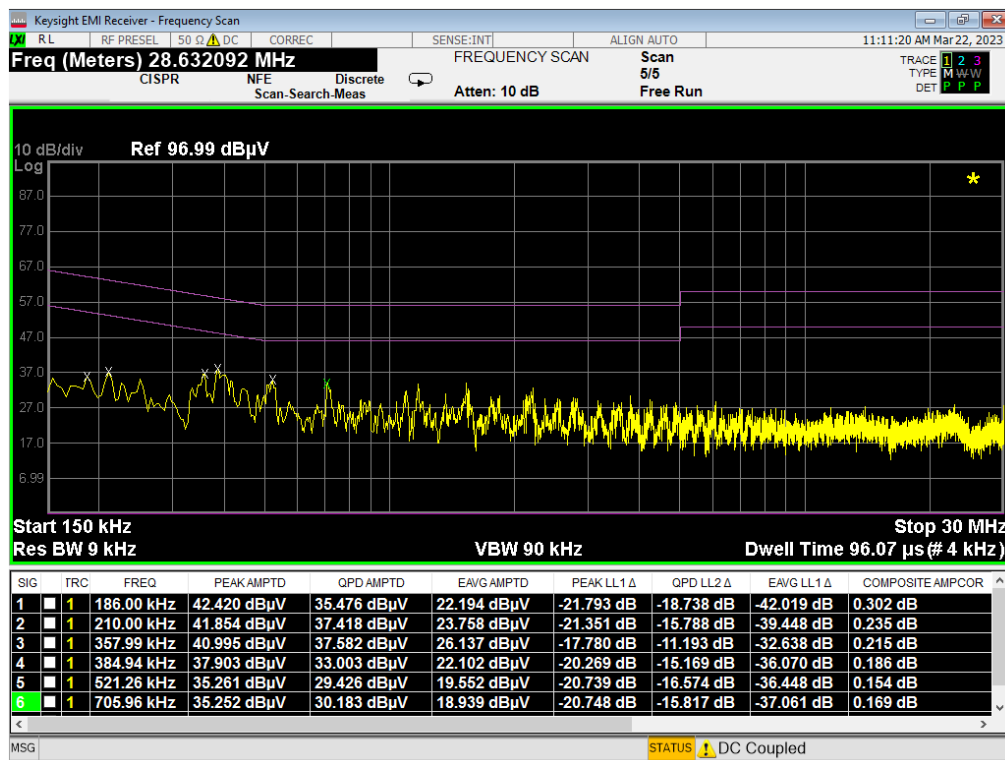
Plot 7-108. Line-Conducted Test Plot (N)
