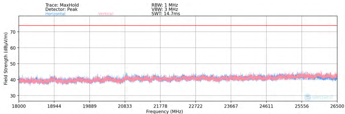
Plot 7-89. Radiated Spurious Plot above 18GHz – ANT1 Open
