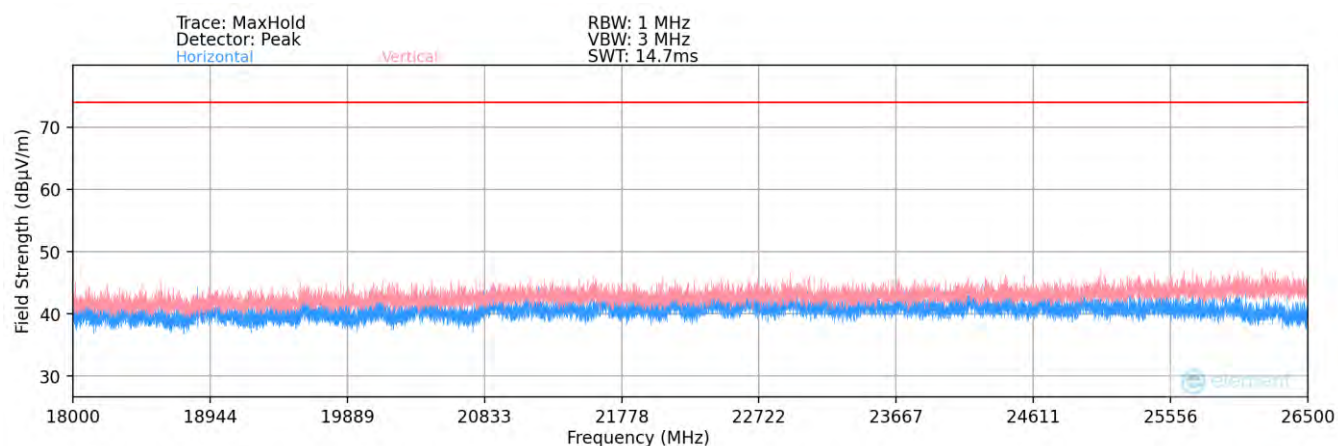
Plot 7-98. Radiated Spurious Plot above 18GHz – ANT2 Half
