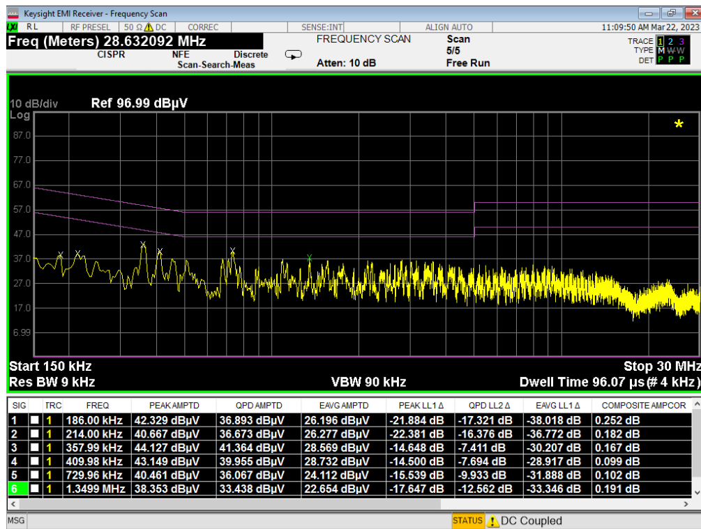
Plot 7-107. Line-Conducted Test Plot (L1)
