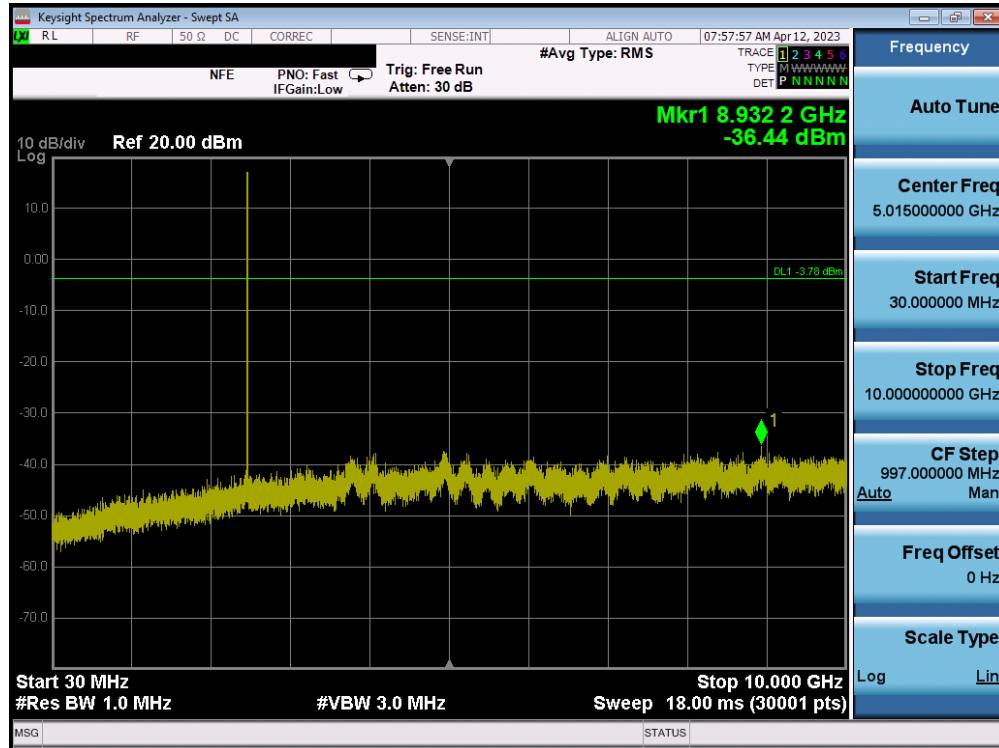
Plot 7-81. Conducted Spurious Plot (Bluetooth, N/AMbps – Ch. 78) – ANT2
