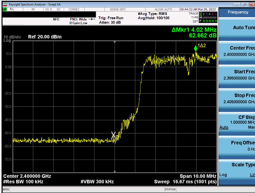
Plot 7-61. Band Edge Plot (Bluetooth with Hopping Enabled, 3 Mbps – Ch. 0) – ANT2
