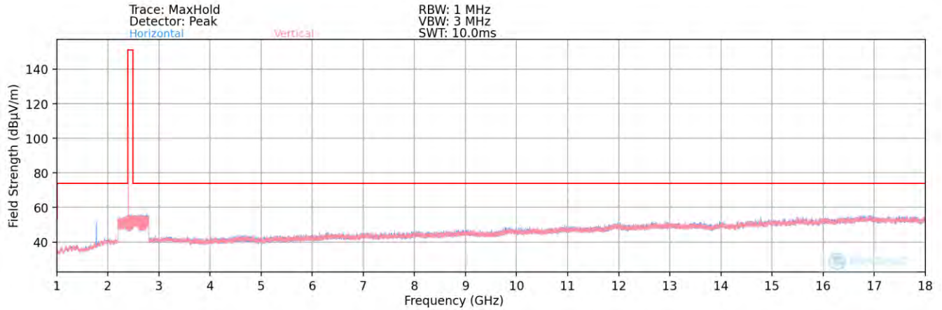
Plot 7-83. Radiated Spurious Plot above 1GHz (BT– Ch. 0) – ANT1 Open
