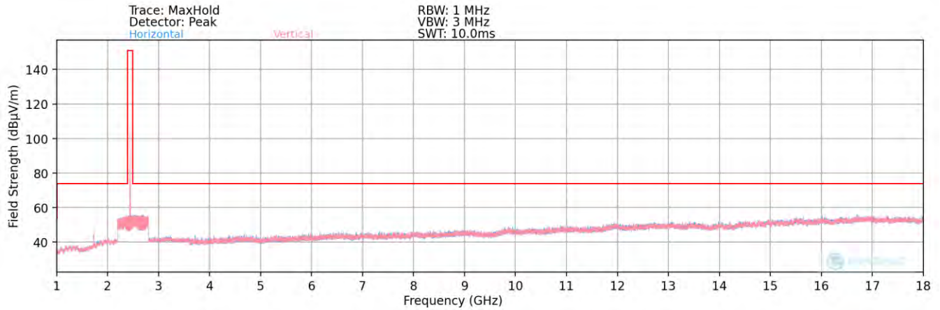
Plot 7-94. Radiated Spurious Plot above 1GHz (BT– Ch. 39) – ANT2 Half
