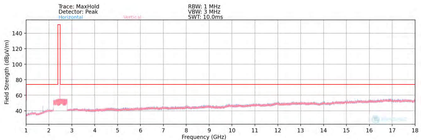
Plot 7-87. Radiated Spurious Plot above 1GHz (BT– Ch. 78) – ANT1 Open
