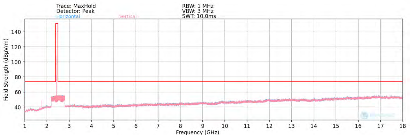
Plot 7-93. Radiated Spurious Plot above 1GHz (BT– Ch. 39) – ANT2 Open
