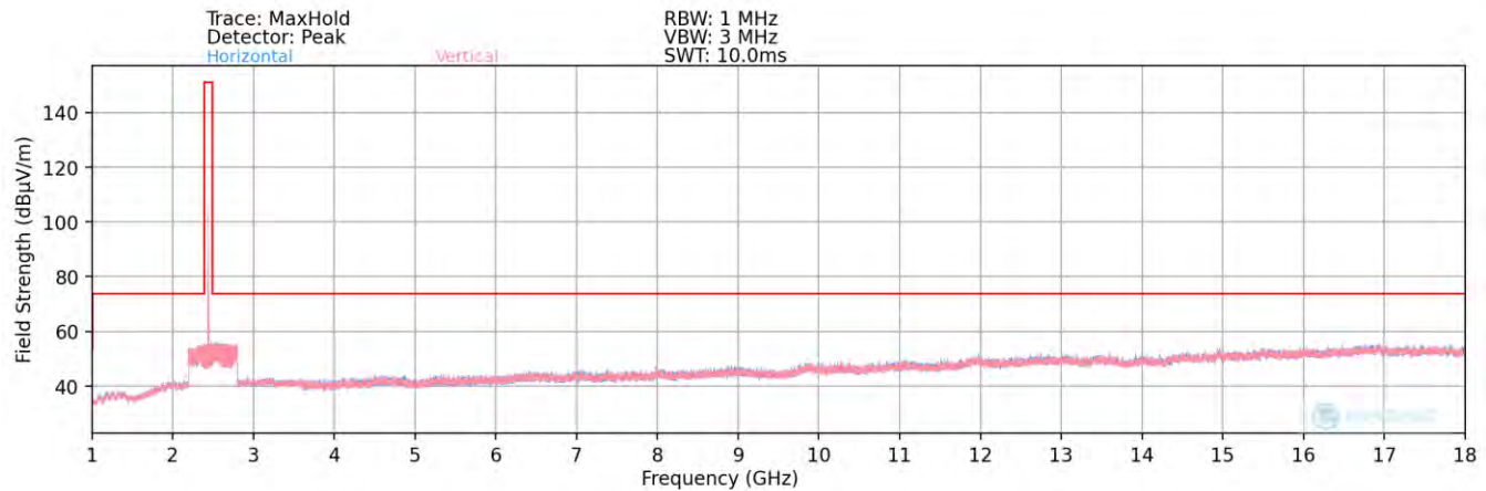
Plot 7-86. Radiated Spurious Plot above 1GHz (BT– Ch. 39) – ANT1 Half
