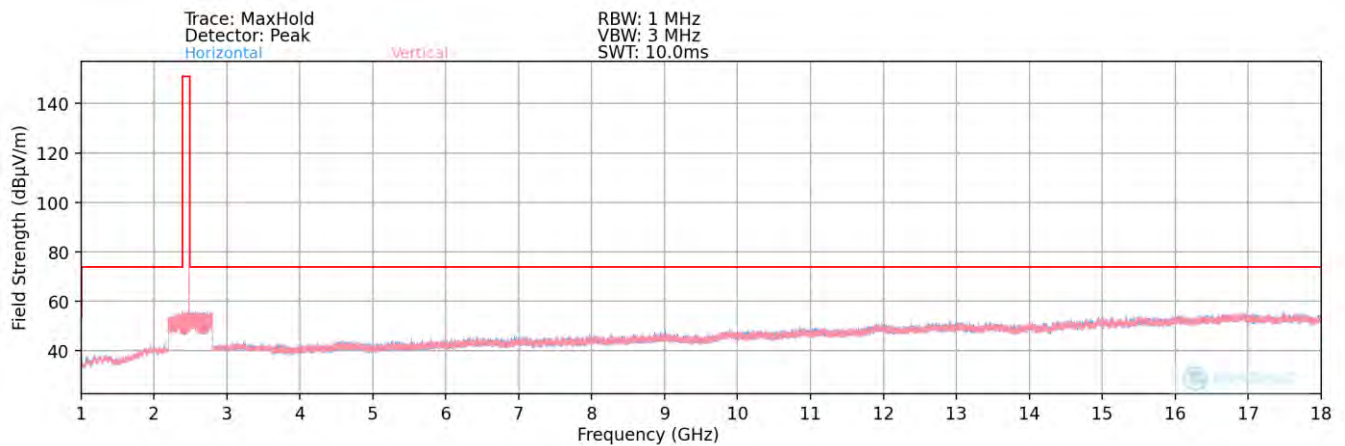
Plot 7-95. Radiated Spurious Plot above 1GHz (BT– Ch. 78) – ANT2 Open
