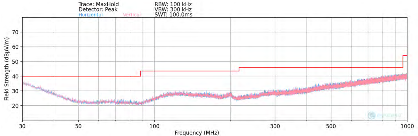
Plot 7-105. Radiated Spurious Plot below 1GHz – ANT1 Open
