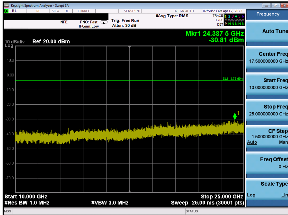
Plot 7-82. Conducted Spurious Plot (Bluetooth, N/AMbps – Ch. 78) – ANT2
