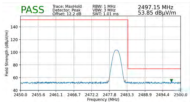
Plot 7-102. Radiated Restricted Upper Band Edge Measurement with WCP (Peak) – ANT1
