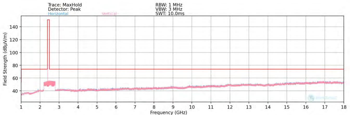
Plot 7-92. Radiated Spurious Plot above 1GHz (BT– Ch. 0) – ANT2 Half
