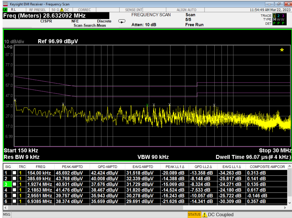
Plot 7-109. Line-Conducted Test Plot (L1) - WCP
