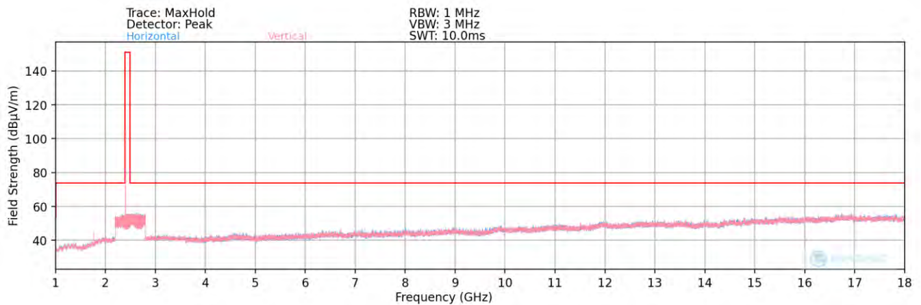
Plot 7-84. Radiated Spurious Plot above 1GHz (BT– Ch. 0) – ANT1 Half
