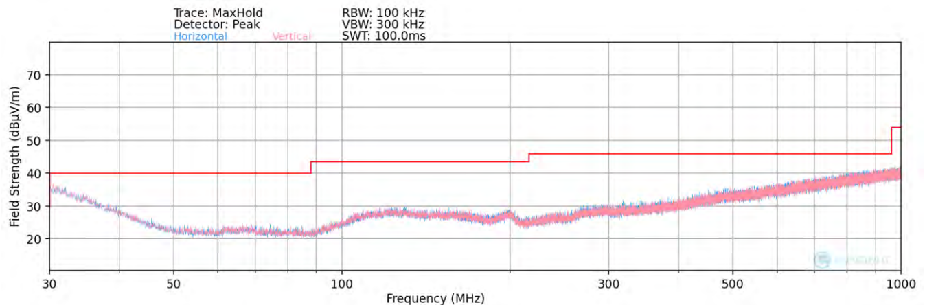
Plot 7-106. Radiated Spurious Plot below 1GHz – ANT1 Half
