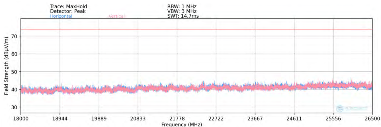
Plot 7-90. Radiated Spurious Plot above 18GHz – ANT1 Half
