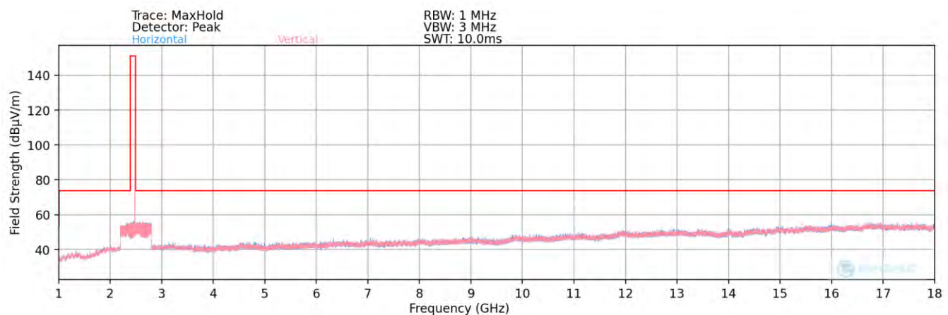
Plot 7-88. Radiated Spurious Plot above 1GHz (BT– Ch. 78) – ANT1 Half
