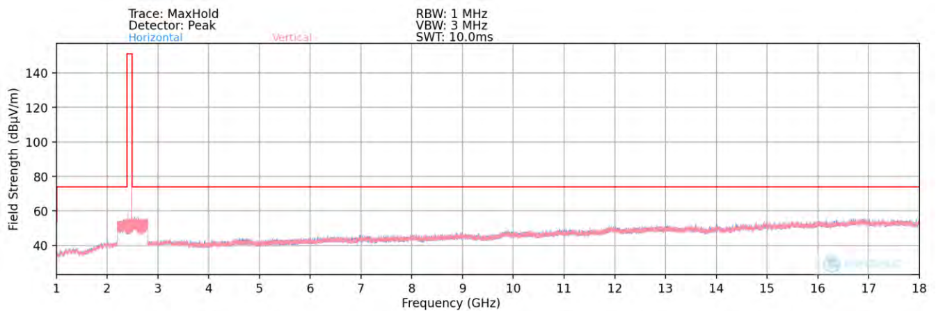
Plot 7-96. Radiated Spurious Plot above 1GHz (BT– Ch. 78) – ANT2 Half
