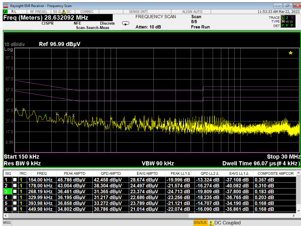
Plot 7-110. Line-Conducted Test Plot (N) - WCP
