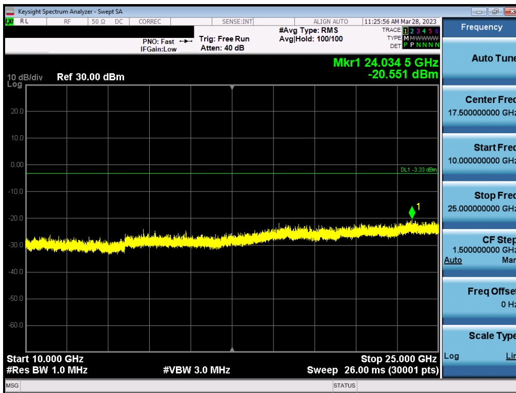
Plot 7-74. Conducted Spurious Plot (Bluetooth, N/AMbps – Ch. 39) – ANT1
