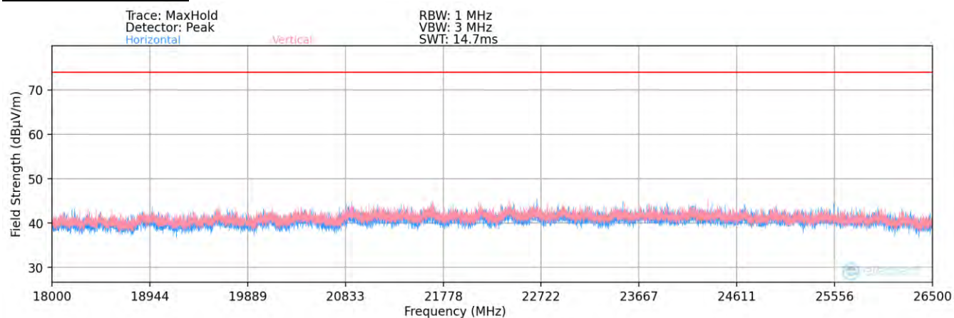
Plot 7-97. Radiated Spurious Plot above 18GHz – ANT2 Open
