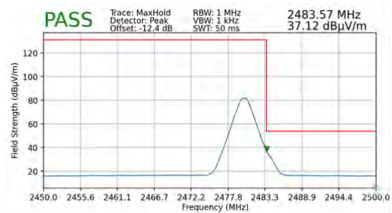
Plot 7-103. Radiated Restricted Upper Band Edge Measurement (Average) – ANT2
