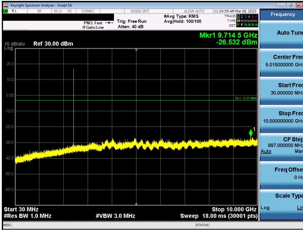
Plot 7-73. Conducted Spurious Plot (Bluetooth, N/AMbps – Ch. 39) – ANT1
