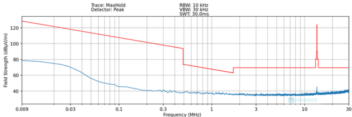
Plot 7-6. Radiated Spurious Plot 9kHz – 30MHz (Pol. Z) - Closed
