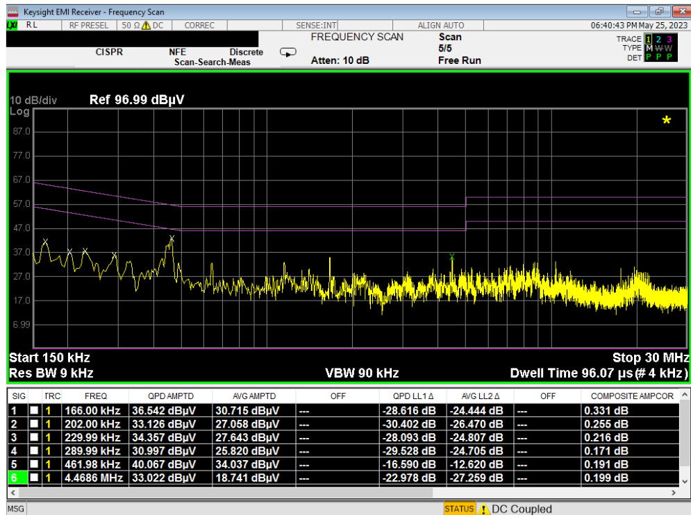
Plot 7-11. Line-Conducted Test Plot (N) - WCP
