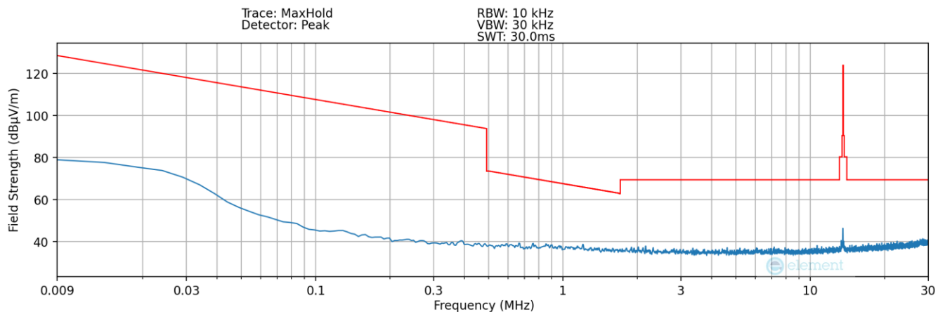
Plot 7-3. Radiated Spurious Plot 9kHz – 30MHz (Pol. Y) - Open
