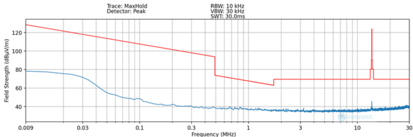
Plot 7-4. Radiated Spurious Plot 9kHz – 30MHz (Pol. Y) - Half
