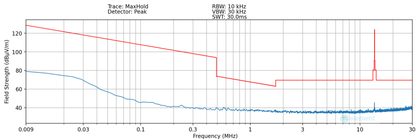
Plot 7-5. Radiated Spurious Plot 9kHz – 30MHz (Pol. Z) – Half
