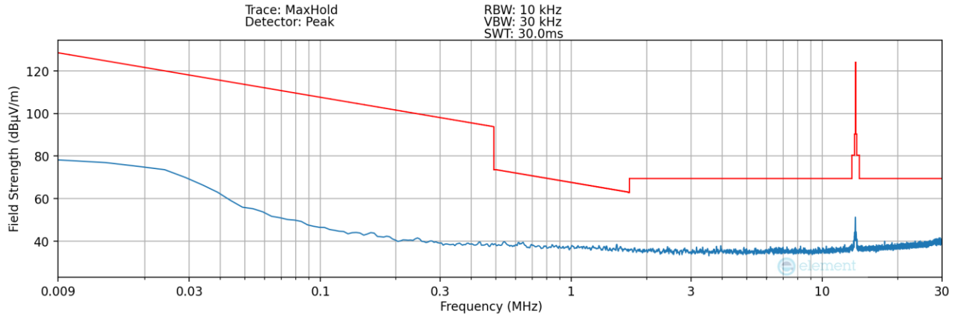
Plot 7-1. Radiated Spurious Plot 9kHz – 30MHz (Pol. X) - Open
