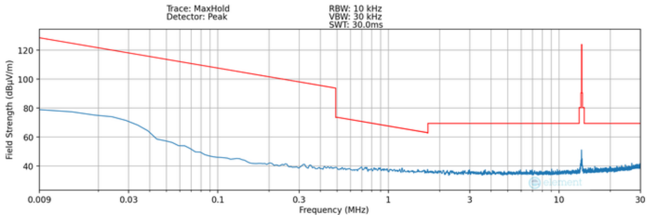
Plot 7-2. Radiated Spurious Plot 9kHz – 30MHz (Pol. X) - Half
