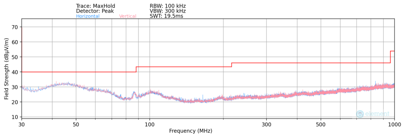
Plot 7-7. Radiated Spurious Plot 30MHz – 1GHz
