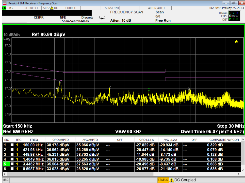
Plot 7-10. Line-Conducted Test Plot (L1) - WCP
