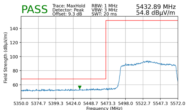
Plot 7-211. Radiated Lower Band Edge Plot MIMO (Peak – UNII Band 2C) with WCP
