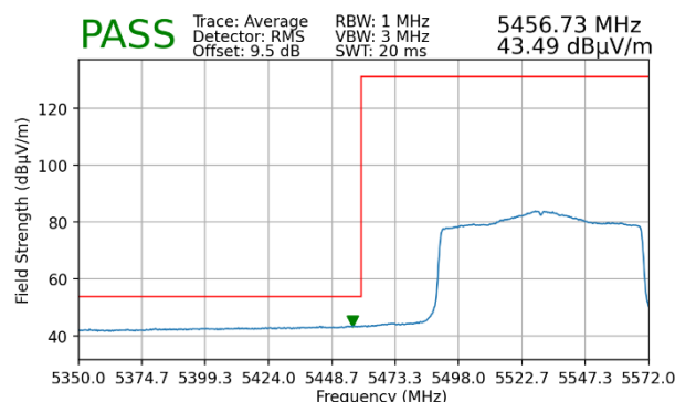
Plot 7-210. Radiated Lower Band Edge Plot MIMO (Average – UNII Band 2C) with WCP
