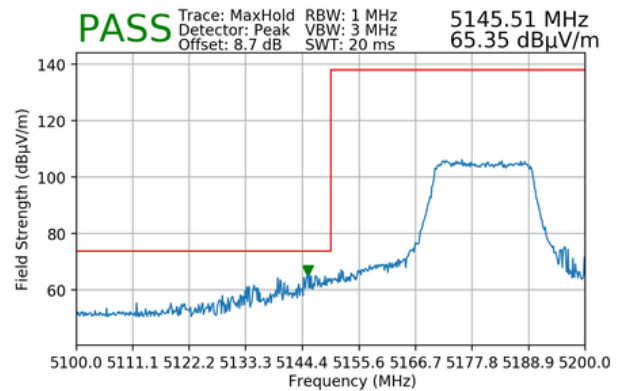
Plot 7-182. Radiated Lower Band Edge Plot MIMO (Peak – UNII Band 1 – 242 Tones)
