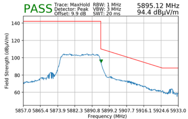
Plot 7-191. Radiated Upper Band Edge Plot MIMO (Peak – UNII Band 4 – 242 Tones)
