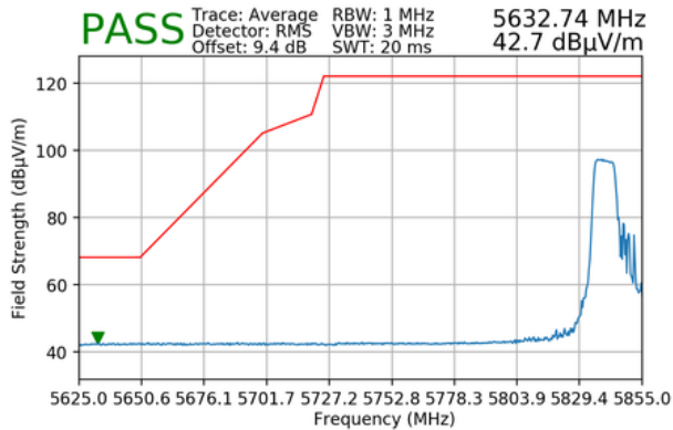
Plot 7-177. Radiated Lower Band Edge Plot MIMO (Average – UNII Band 4 – 106 Tones)
