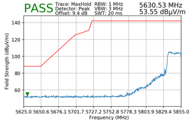
Plot 7-189. Radiated Lower Band Edge Plot MIMO (Peak – UNII Band 4 – 242 Tones)
