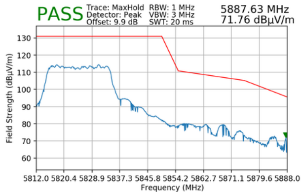
Plot 7-187. Radiated Upper Band Edge Plot MIMO (Peak – UNII Band 3 – 242 Tones)
