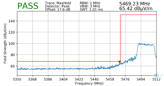
Plot 7-186. Radiated Lower Band Edge Plot MIMO (Peak – UNII Band 2C – 242 Tones)
