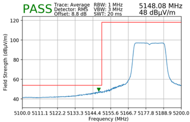
Plot 7-181. Radiated Lower Band Edge Plot MIMO (Average – UNII Band 1 – 242 Tones)
