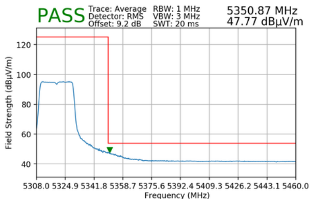
Plot 7-183. Radiated Upper Band Edge Plot MIMO (Average – UNII Band 2A – 242 Tones)
