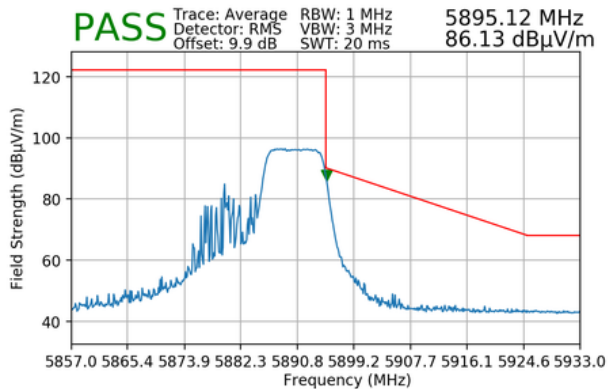
Plot 7-179. Radiated Upper Band Edge Plot MIMO (Average – UNII Band 4 – 106 Tones)
