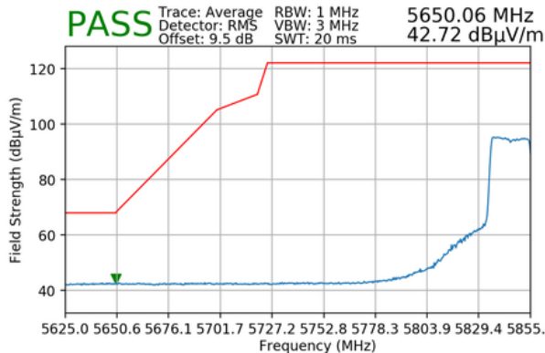
Plot 7-188. Radiated Lower Band Edge Plot MIMO (Average – UNII Band 4 – 242 Tones)
