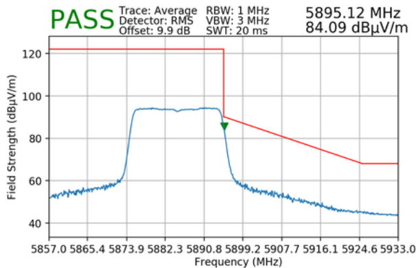
Plot 7-190. Radiated Upper Band Edge Plot MIMO (Average – UNII Band 4 – 242 Tones)
