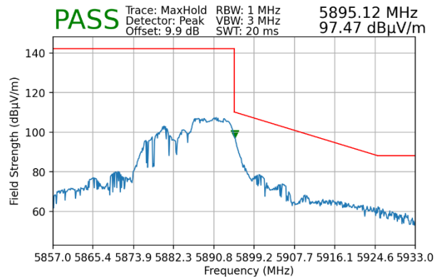
Plot 7-180. Radiated Upper Band Edge Plot MIMO (Peak – UNII Band 4 – 106 Tones)
