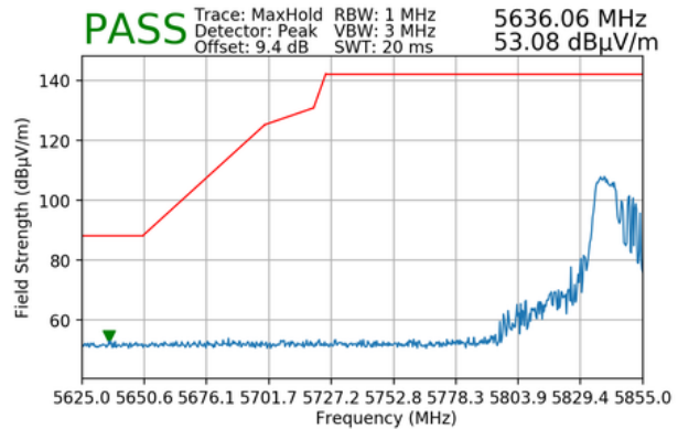
Plot 7-178. Radiated Lower Band Edge Plot MIMO (Peak – UNII Band 4 – 106 Tones)
