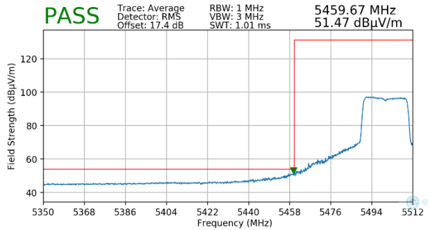
Plot 7-185. Radiated Lower Band Edge Plot MIMO (Average – UNII Band 2C – 242 Tones)
