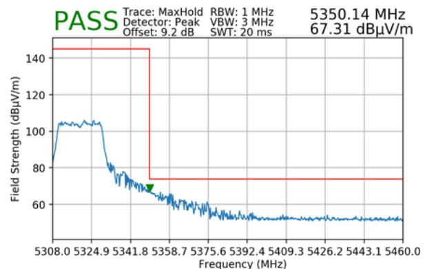
Plot 7-184. Radiated Upper Band Edge Plot MIMO (Peak – UNII Band 2A – 242 Tones)
