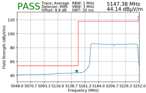
Plot 7-203. Radiated Lower Band Edge Plot MIMO (Average – UNII Band 1 – 996 Tones)
