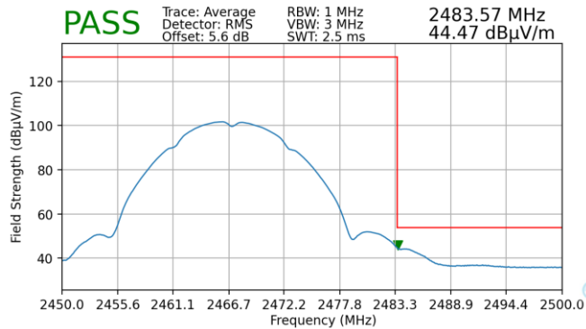
Plot 7-149. Radiated Restricted Upper Band Edge Measurement SISO ANT2 (Average)
