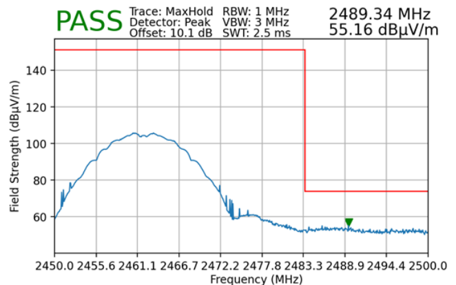
Plot 7-148. Radiated Restricted Upper Band Edge Measurement SISO ANT2 (Peak)
