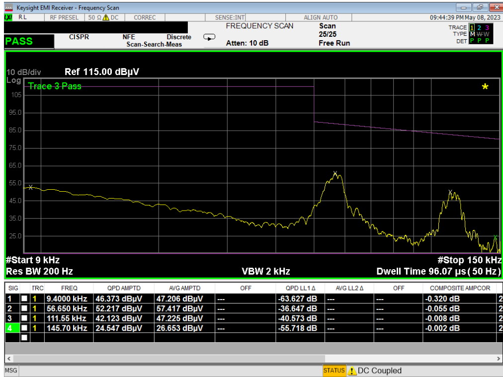
Plot 7-7. Line-Conducted Test Plot (N) - Device to Device – 9kHz to 150kHz
