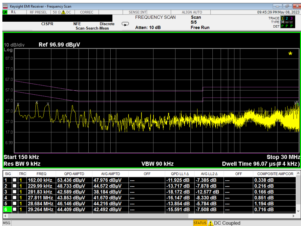
Plot 7-8. Line-Conducted Test Plot (N) - Device to Device – 150kHz to 30MHz
