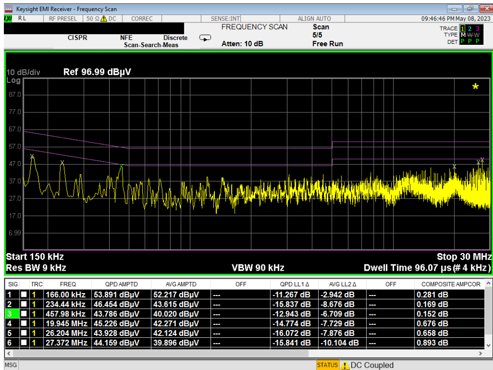
Plot 7-6. Line-Conducted Test Plot (L1) - Device to Device – 150kHz to 30MHz
