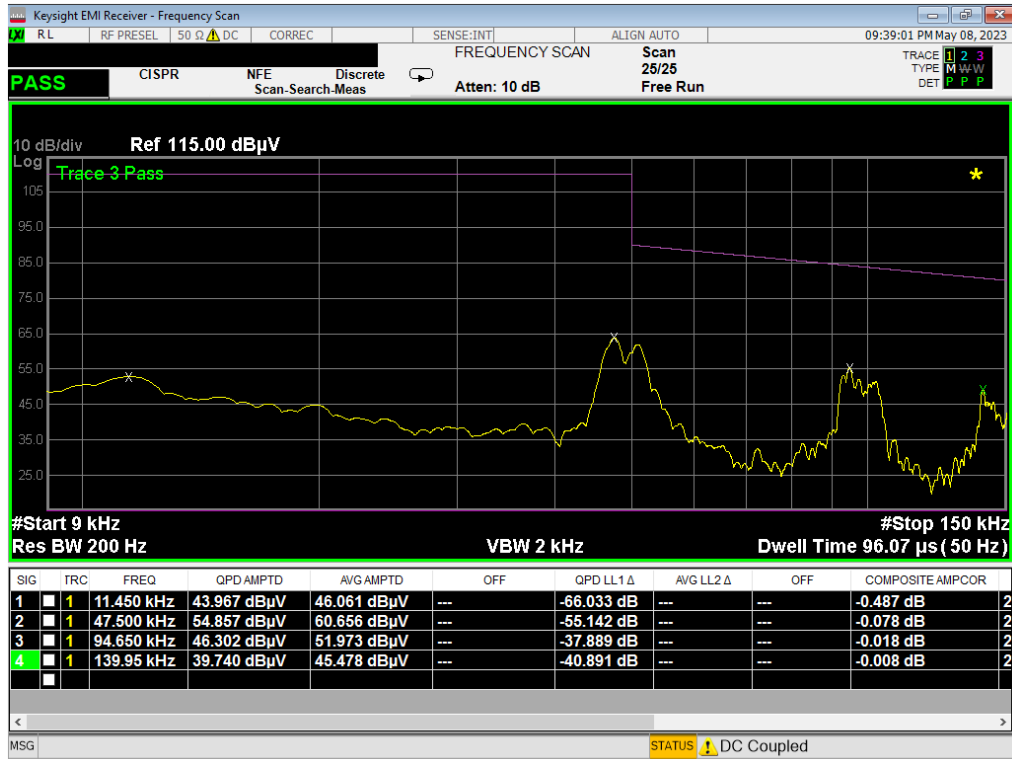
Plot 7-5. Line-Conducted Test Plot (L1) - Device to Device – 9kHz to 150kHz
