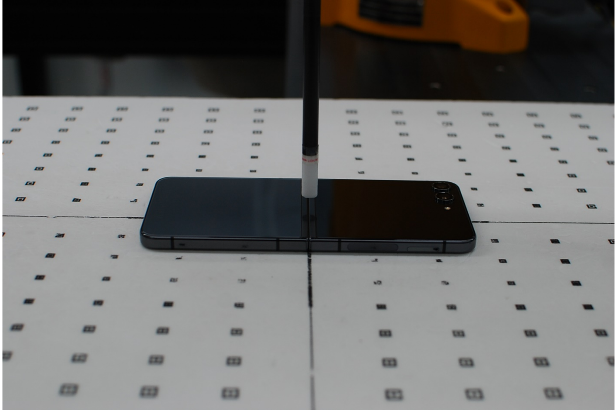
Figure F-16 Near Field Power Density Test Setup Photo – Back Side at 9.16 mm, Open
