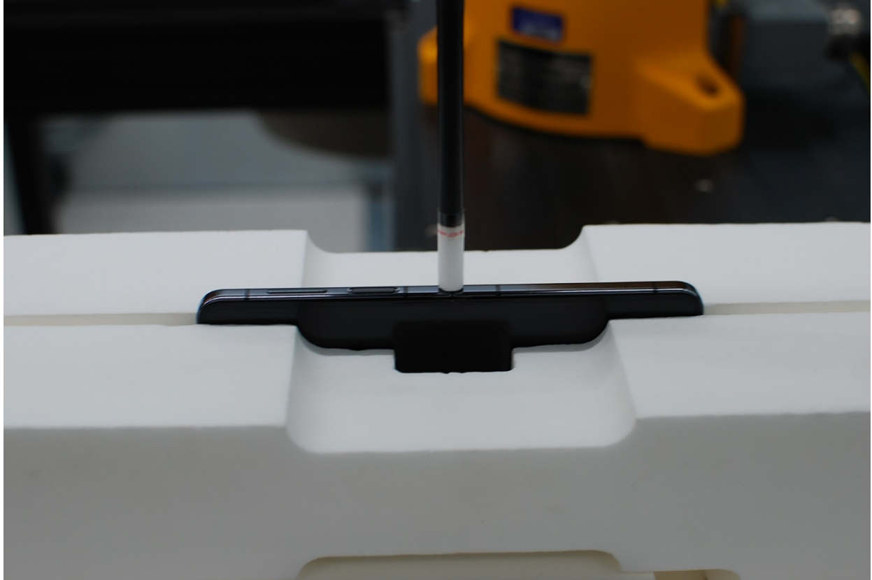
Figure F-19 Near Field Power Density Test Setup Photo – Right Edge at 2 mm, Open
