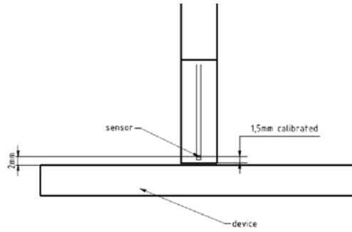
Figure F-2 EImmWVx Probe
