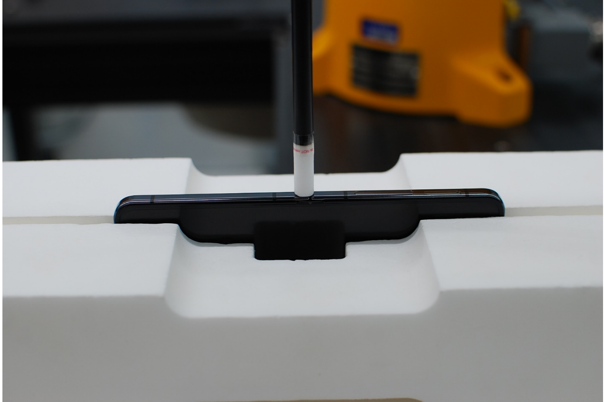
Figure F-20 Near Field Power Density Test Setup Photo – Left Edge at 2 mm, Open
