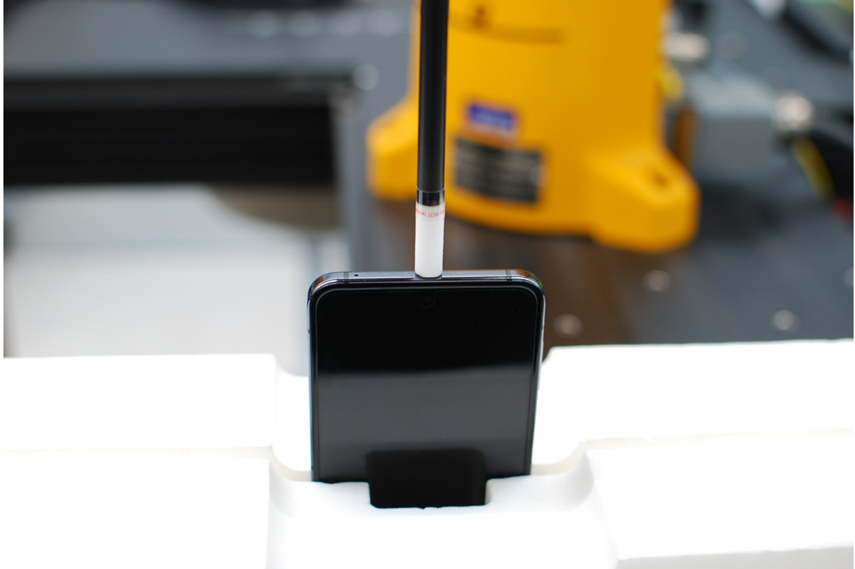
Figure F-18 Near Field Power Density Test Setup Photo – Top Edge at 2 mm, Open
