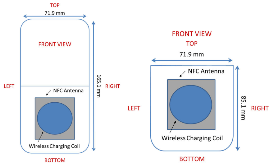
Figure I-2 NFC Antenna Locations
