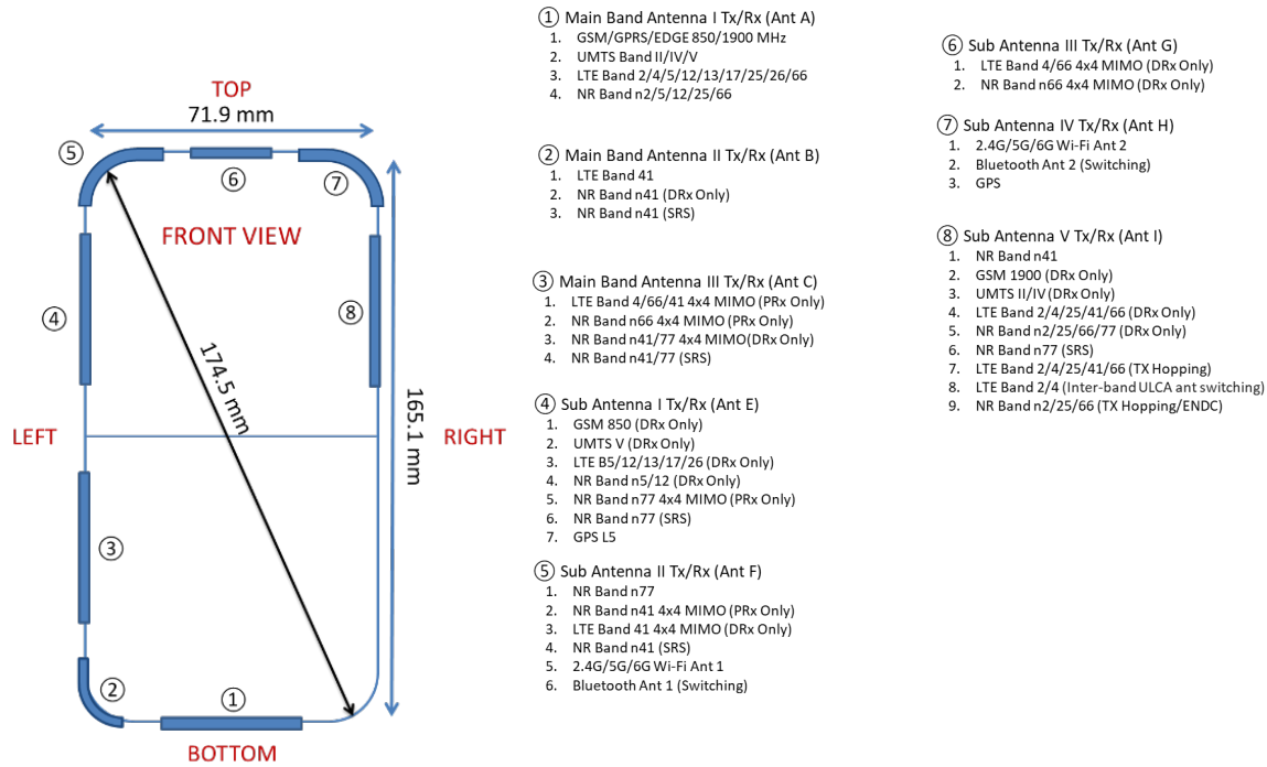
Figure K-1 DUT Antenna Locations
