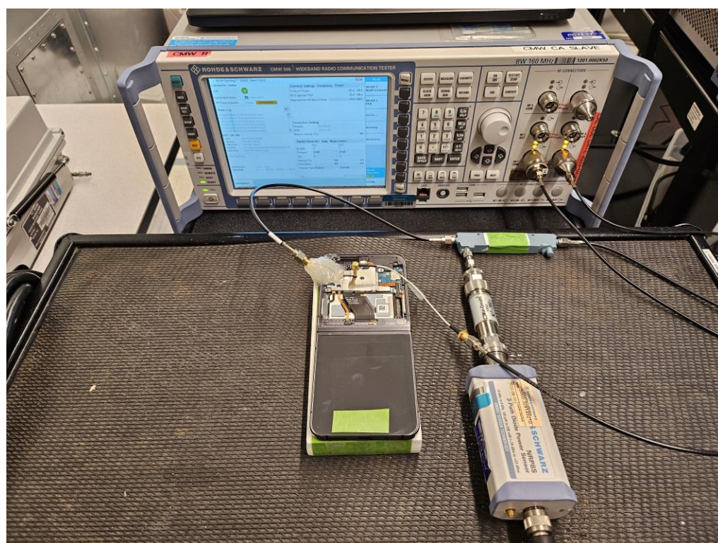
Test Setup Photo 8 – Conducted Test Setup (Figure 5-1e)
