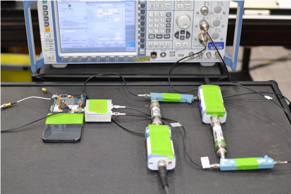
Test Setup Photo 3 – Conducted Test Setup (Figure 5-1d)
