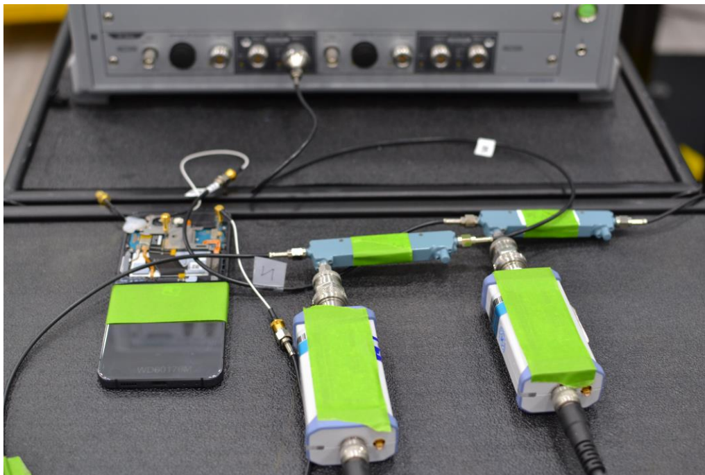
Test Setup Photo 7 – Conducted Test Setup (Figure 5-1c)
