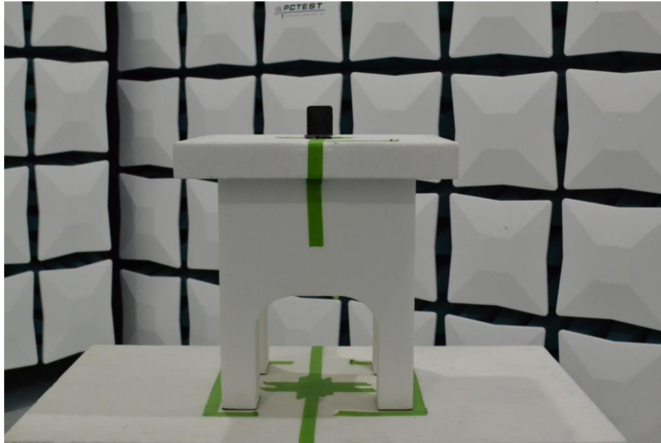
Figure 9. Test Setup – X Position – 1GHz-18GHz – Half
