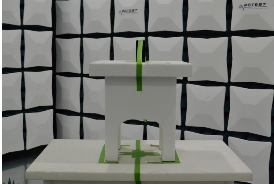
Figure 7. Test Setup – Z Position – 1GHz-18GHz – Open
