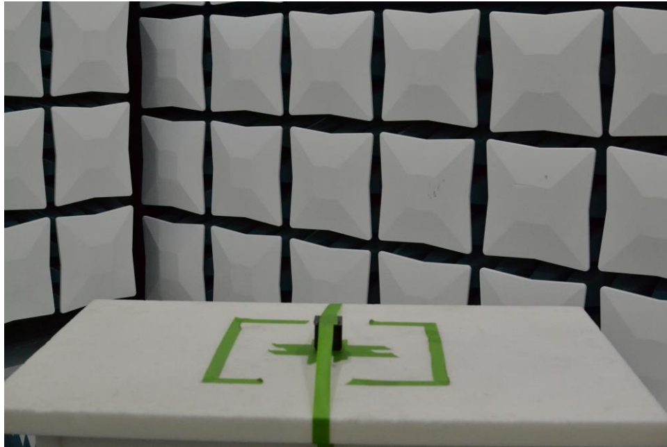
Figure 23. Test Setup – Z Position – 30MHz-1GHz – Half
