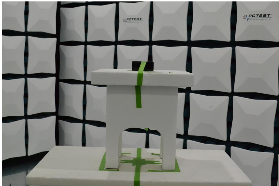
Figure 6. Test Setup – Y Position – 1GHz-18GHz – Open
