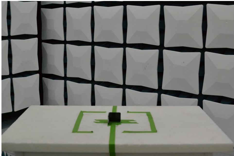
Figure 22. Test Setup – Y Position – 30MHz-1GHz – Half
