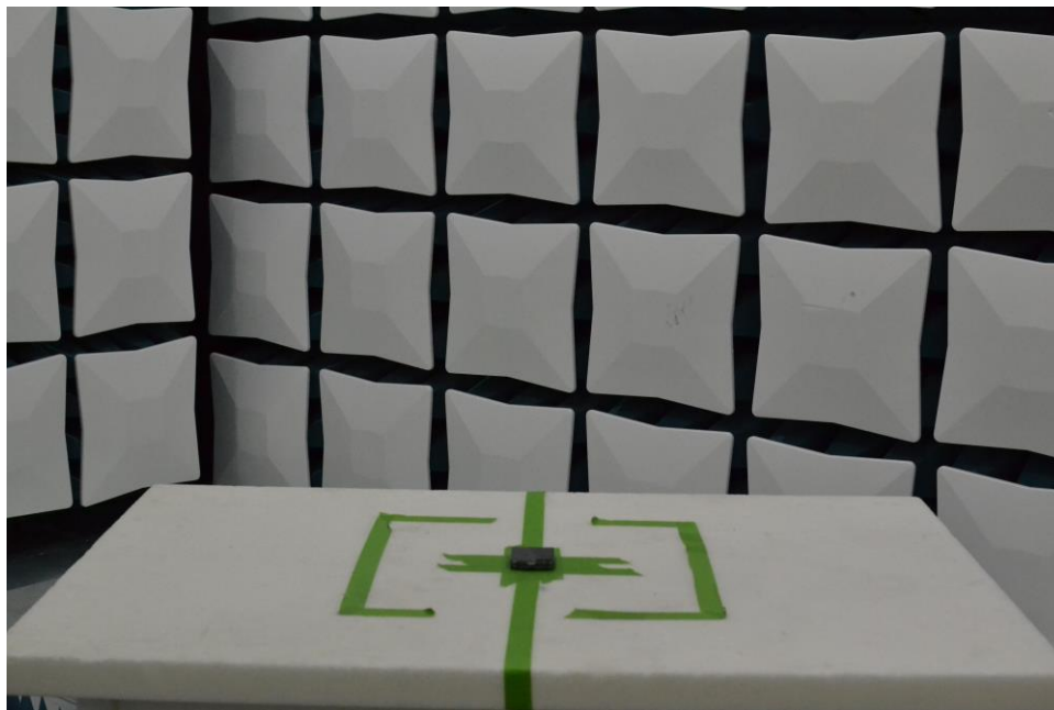
Figure 24. Test Setup – X Position – 30MHz-1GHz – Closed
