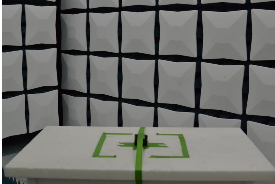
Figure 25. Test Setup – Y Position – 30MHz-1GHz – Closed
