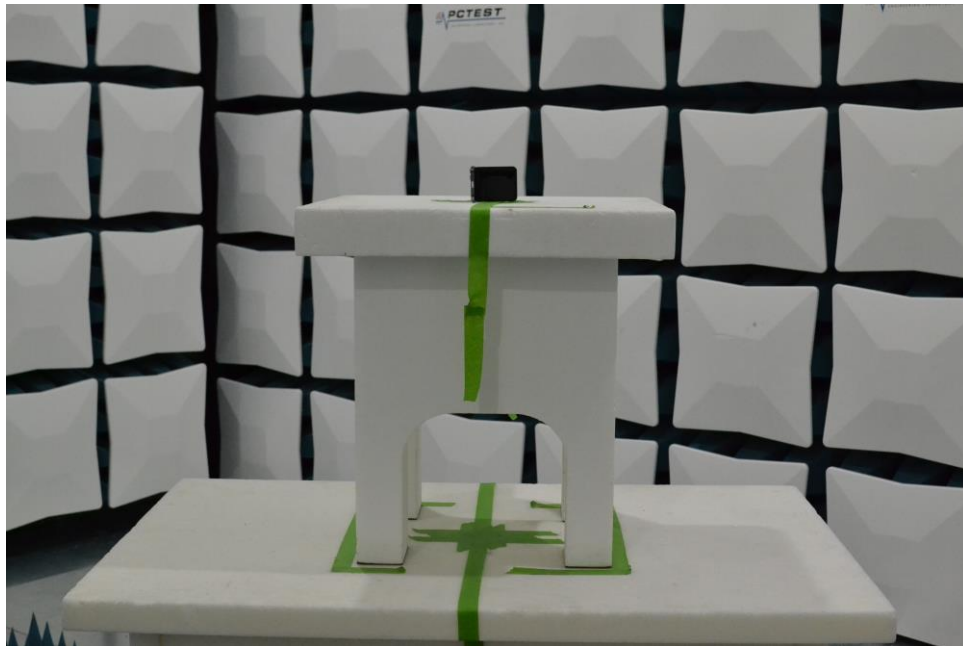
Figure 10. Test Setup – Y Position – 1GHz-18GHz – Half
