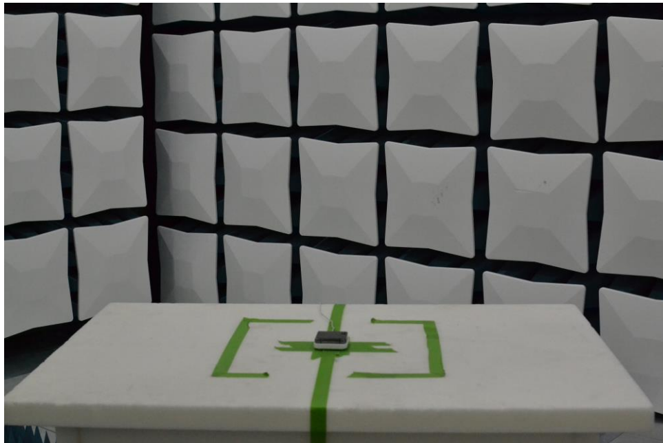
Figure 28. Test Setup – WCP Position – 30MHz-1GHz – Closed
