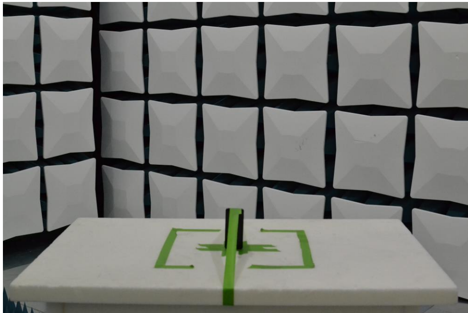
Figure 18. Test Setup – Z Position – 30MHz-1GHz – Open
