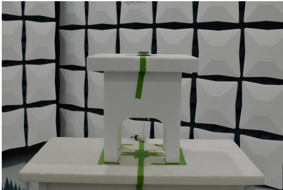
Figure 8. Test Setup – WCP Position – 1GHz-18GHz – Open
