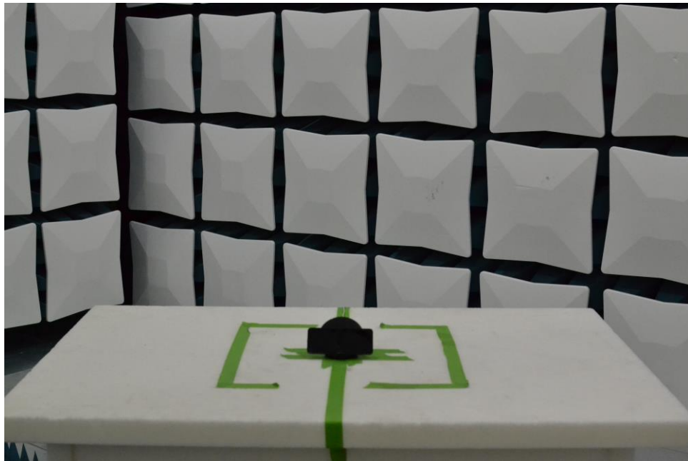
Figure 20. Test Setup – WCP Position – 30MHz-1GHz – Open
