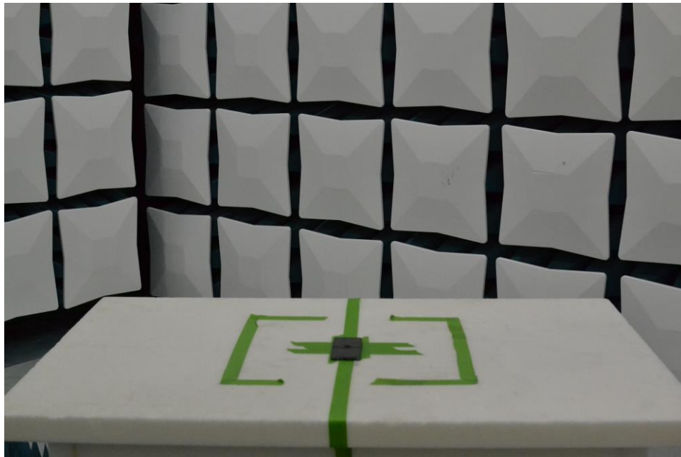
Figure 16. Test Setup – X Position – 30MHz-1GHz – Open
