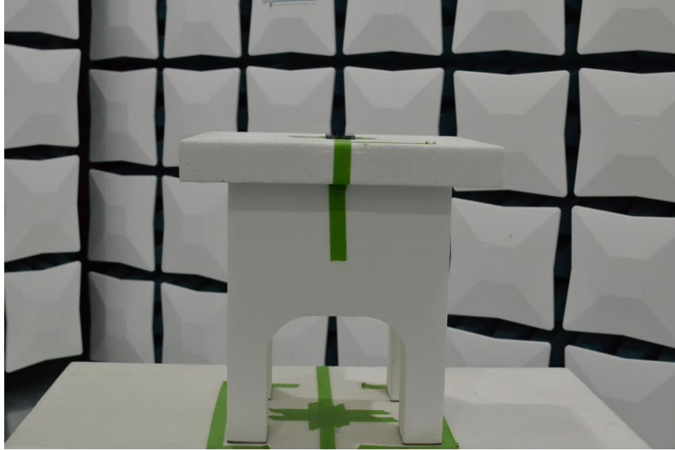
Figure 5. Test Setup – X Position – 1GHz-18GHz – Open
