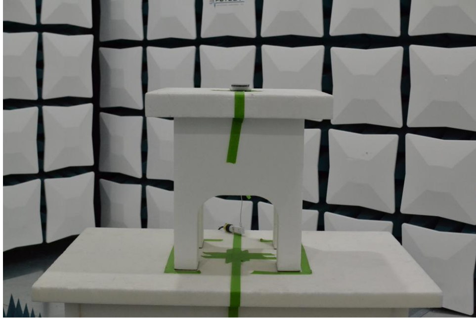
Figure 15. Test Setup – WCP Position – 1GHz-18GHz – Closed
