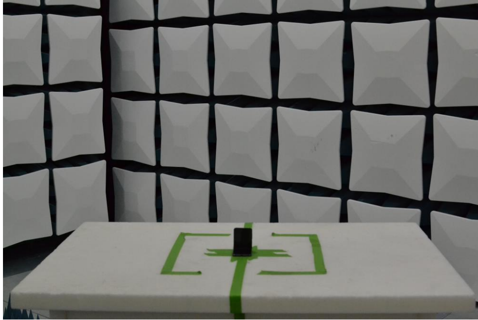
Figure 21. Test Setup – X Position – 30MHz-1GHz – Half
