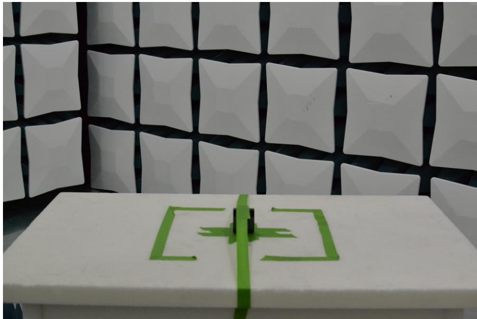
Figure 26. Test Setup – Z Position – 30MHz-1GHz – Closed
