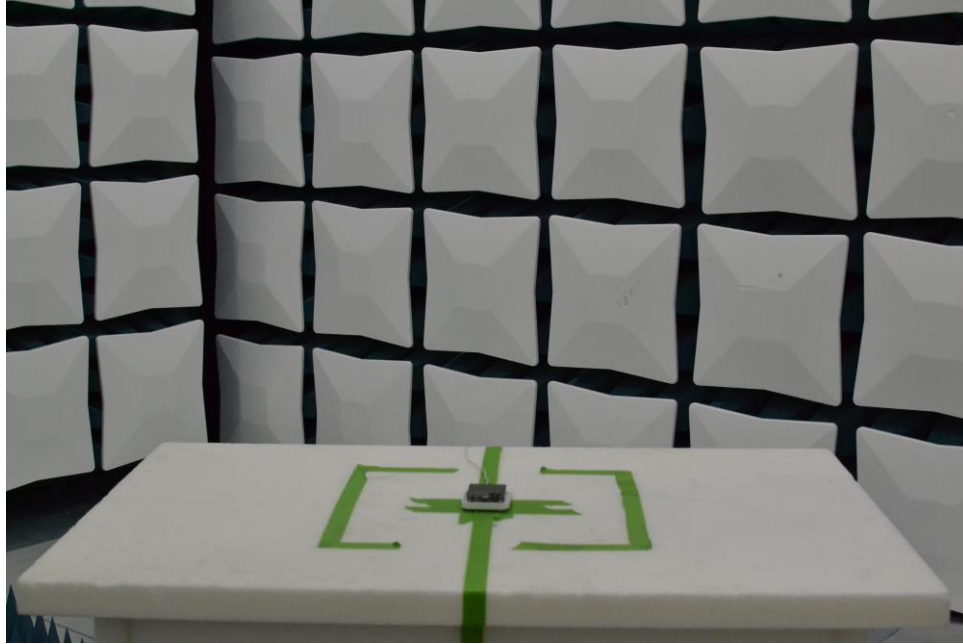
Figure 27. Test Setup – WCP Position – 30MHz-1GHz – Closed
