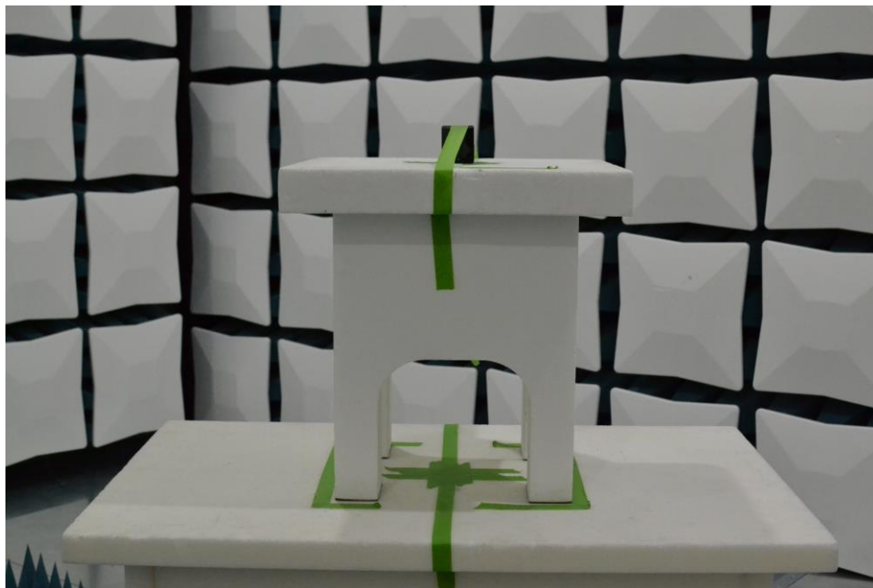
Figure 14. Test Setup – Z Position – 1GHz-18GHz – Closed
