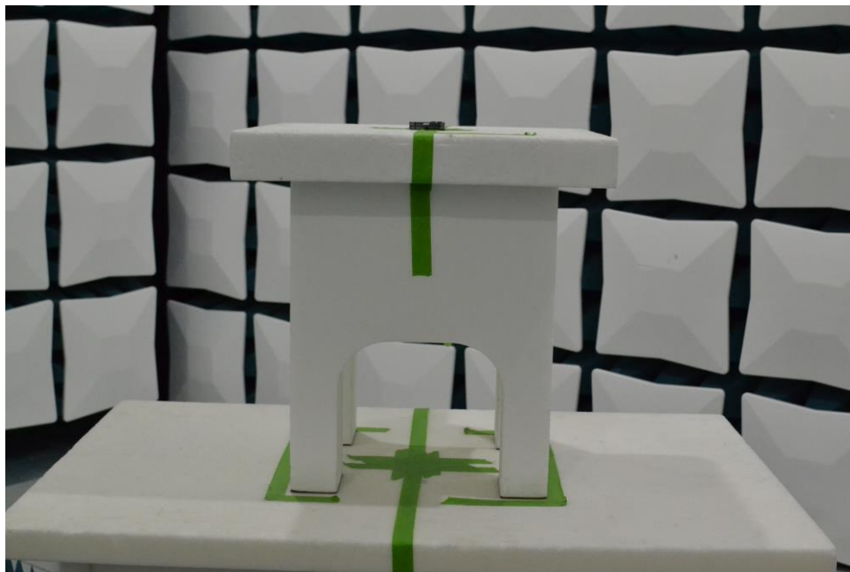
Figure 12. Test Setup – X Position – 1GHz-18GHz – Closed
