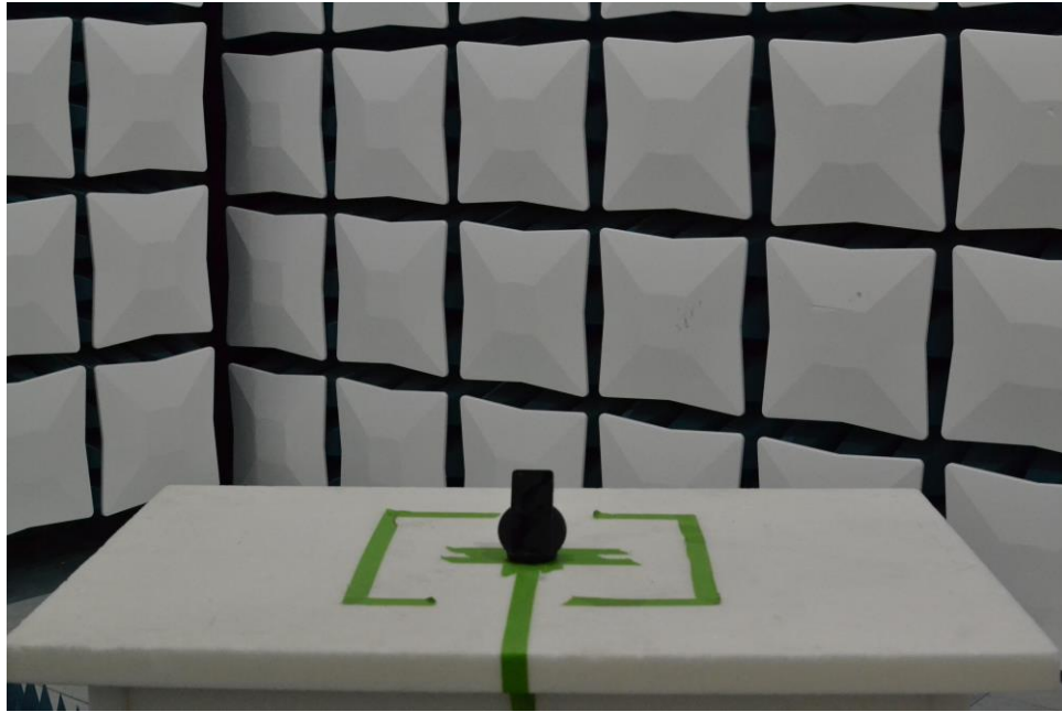
Figure 19. Test Setup – WCP Position – 30MHz-1GHz – Open
