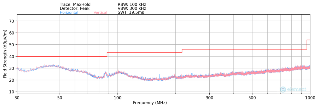
Plot 7-7. Radiated Spurious Plot 30MHz – 1GHz
