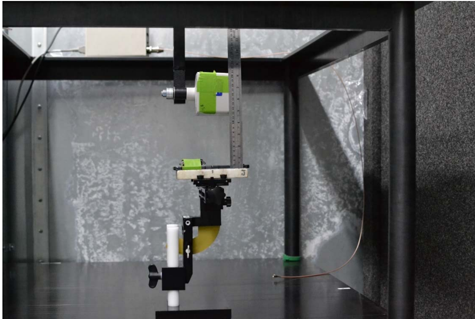
Test Setup Photo 27 E-field, Back side, 15cm
