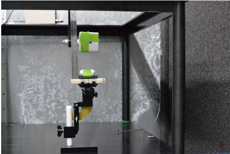
Test Setup Photo 31 E-field, Back side, 15cm
