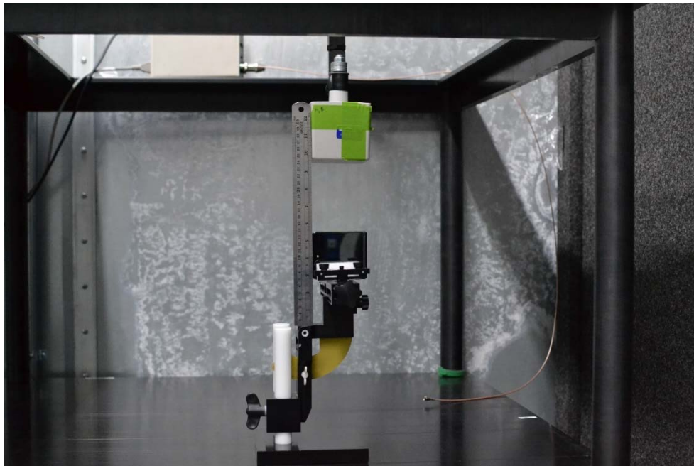
Test Setup Photo 28 H-field, Back side, 15cm
