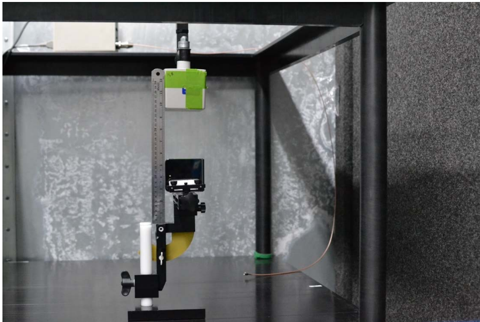
Test Setup Photo 32 H-field, Back side, 15cm
