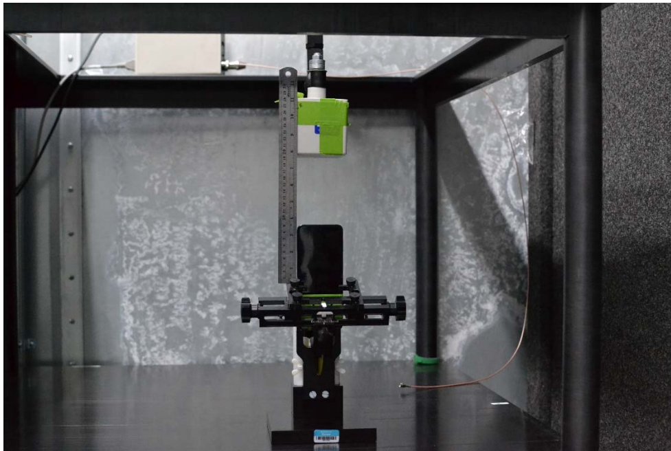
Test Setup Photo 30 H-field, Back side, 15cm
