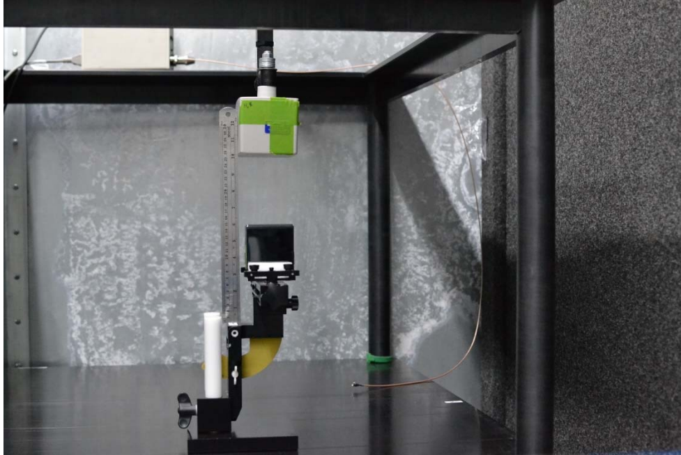
Test Setup Photo 21 H-field, Top edge, 15cm
