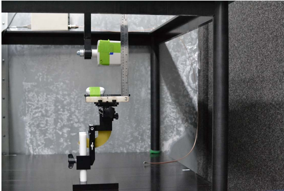
Test Setup Photo 29 E-field, Back side, 15cm
