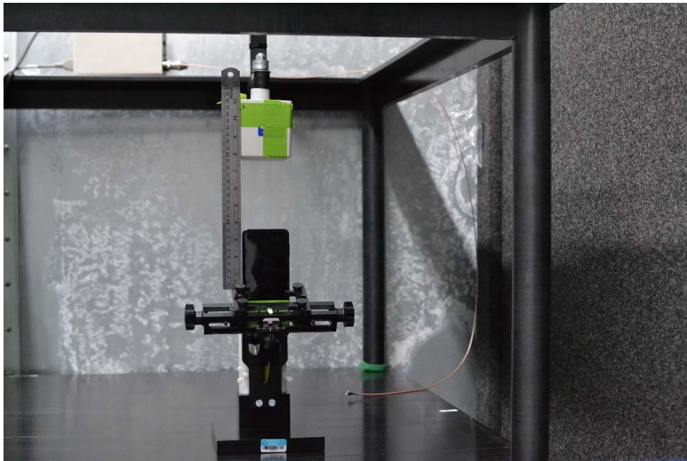
Test Setup Photo 26 H-field, Back side, 15cm
