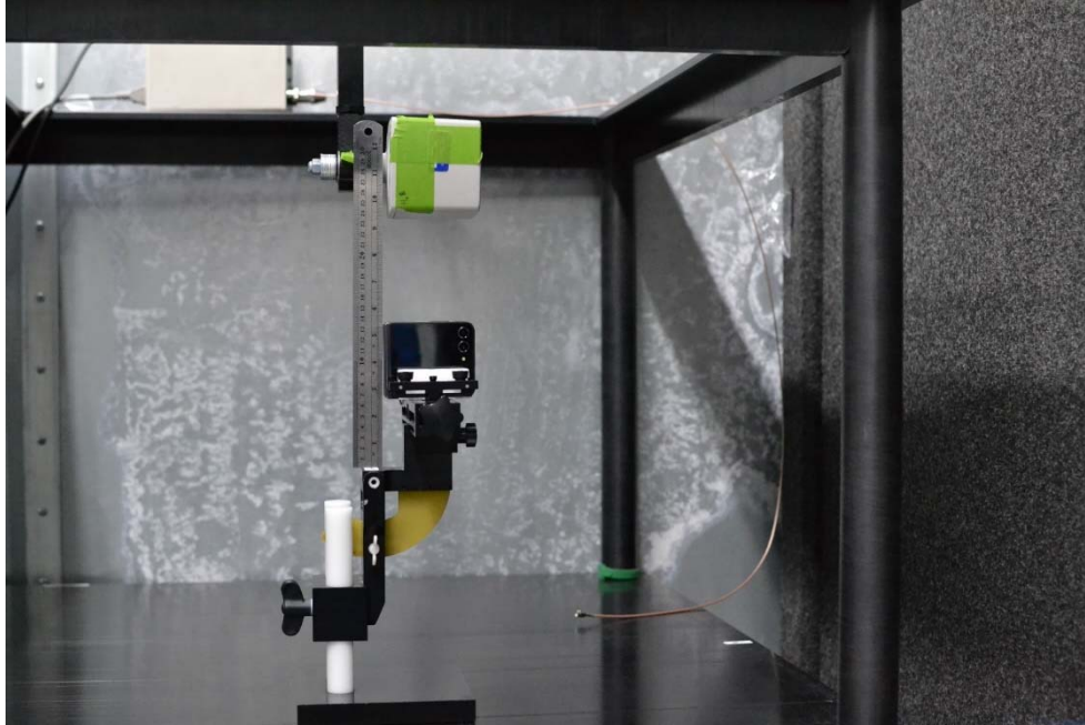
Test Setup Photo 17 E-field, Right edge, 15cm
