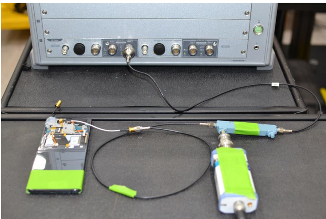
Test Setup Photo 4 - Conducted Test Setup (Figure 5-1a)
