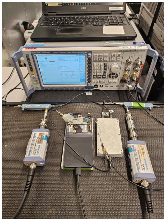
Test Setup Photo 7 – Conducted Test Setup (Figure 5-1e)
