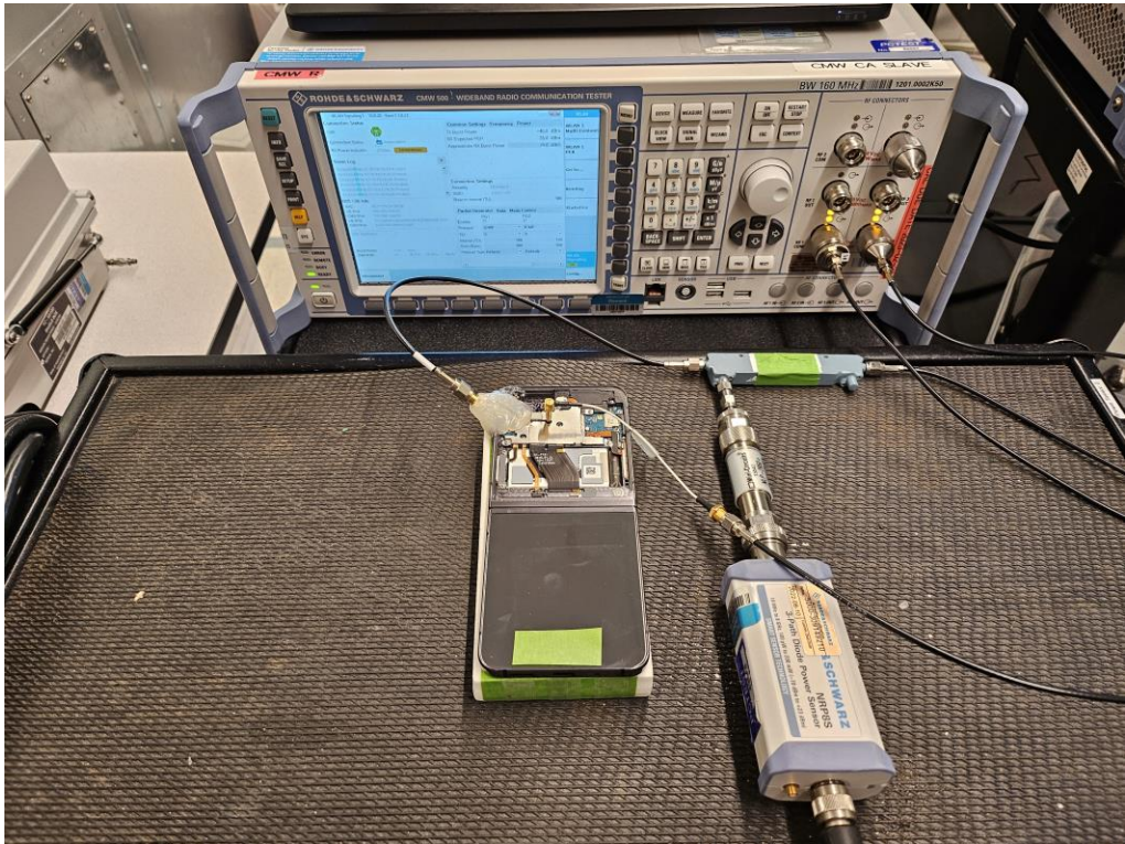
Test Setup Photo 6 – Conducted Test Setup (Figure 5-1d)
