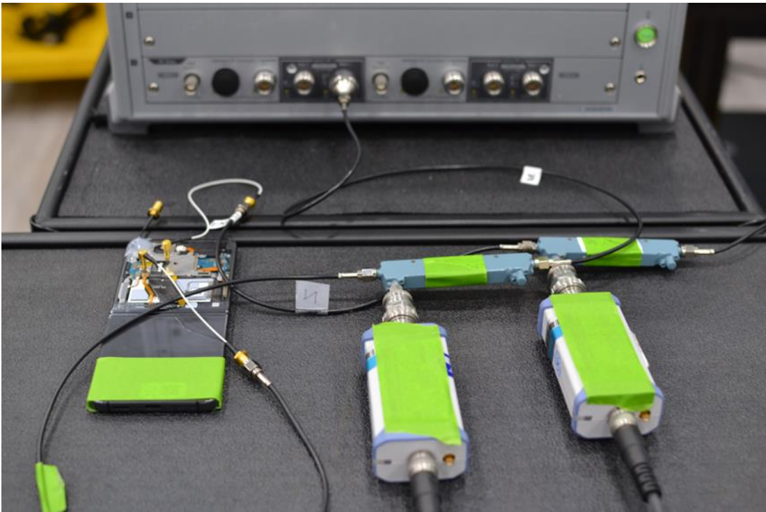
Test Setup Photo 5 - Conducted Test Setup (Figure 5-1c)
