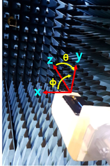
Figure 1: Geometry for SM-F731U for Radiation patterns.
