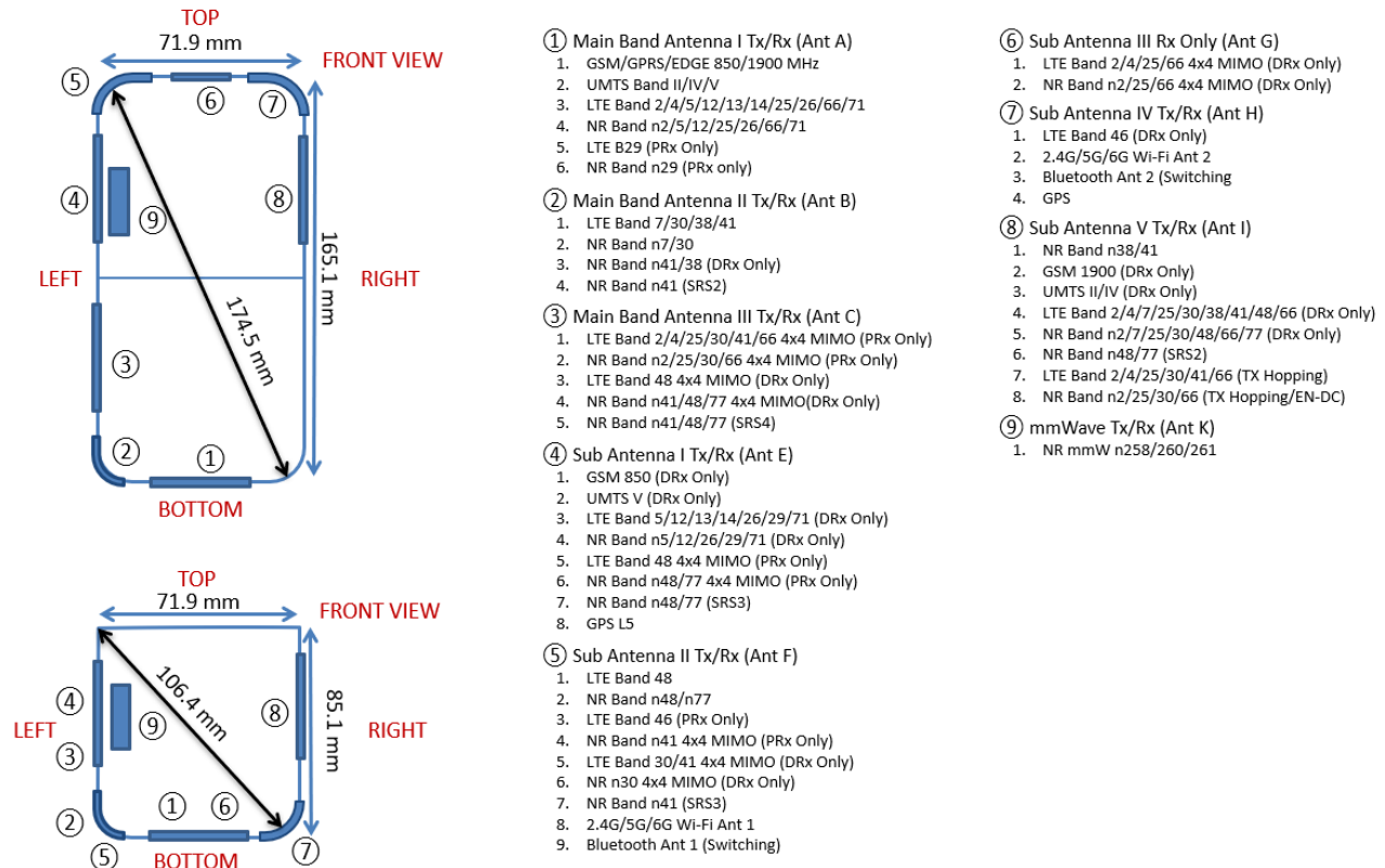
Figure K-1 DUT Antenna Locations
