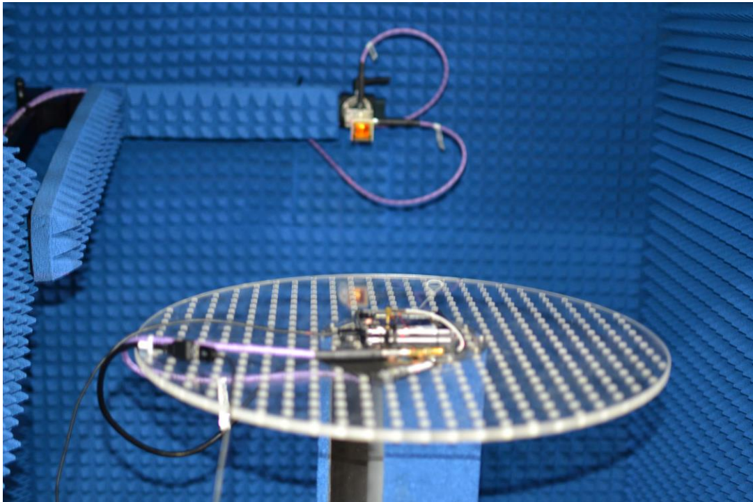
Test Setup Photo 17 – Radiated Power Measurement Setup, Closed (Figure 7-1)
