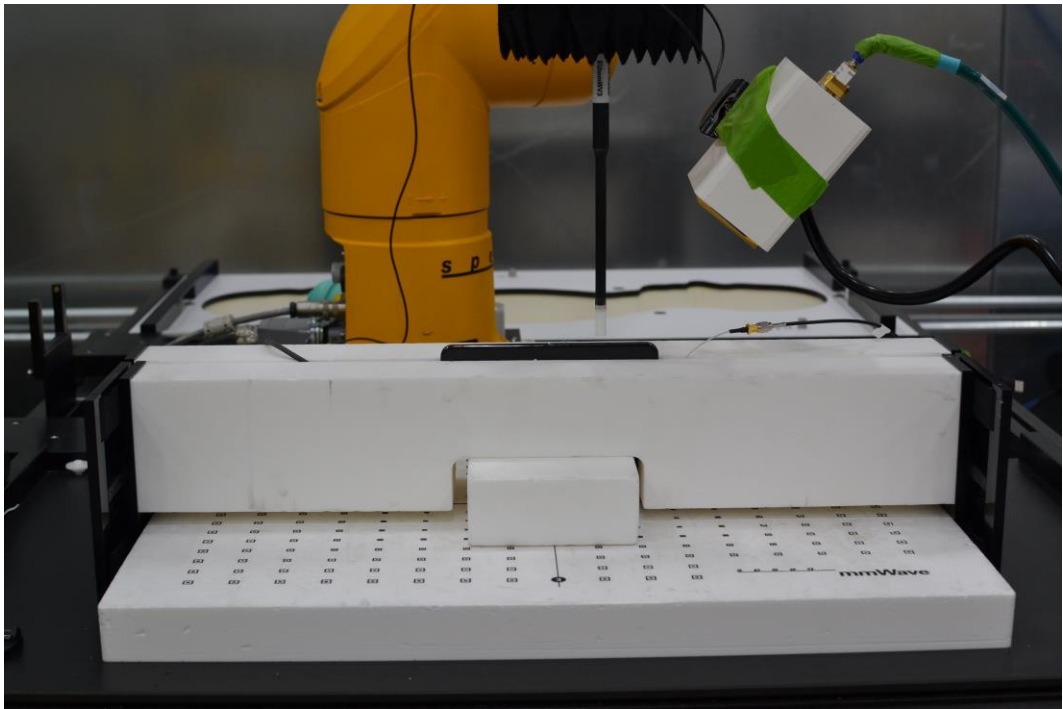
Test Setup Photo 14 – Power Density Setup Left Edge, Open (Figure 7-2)
