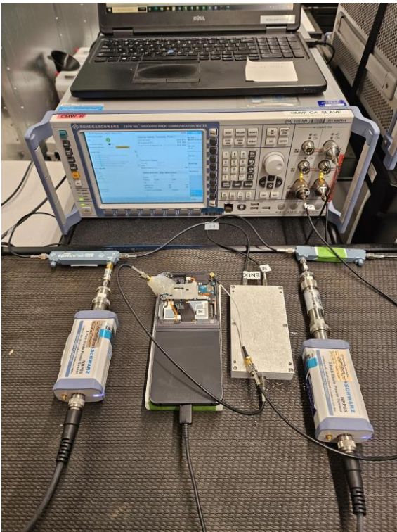
Test Setup Photo 8 – Conducted Test Setup (Figure 6-1e)
