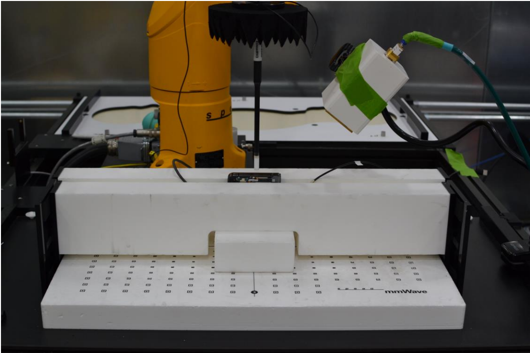
Test Setup Photo 15 – Power Density Setup Left Edge, Closed (Figure 7-2)
