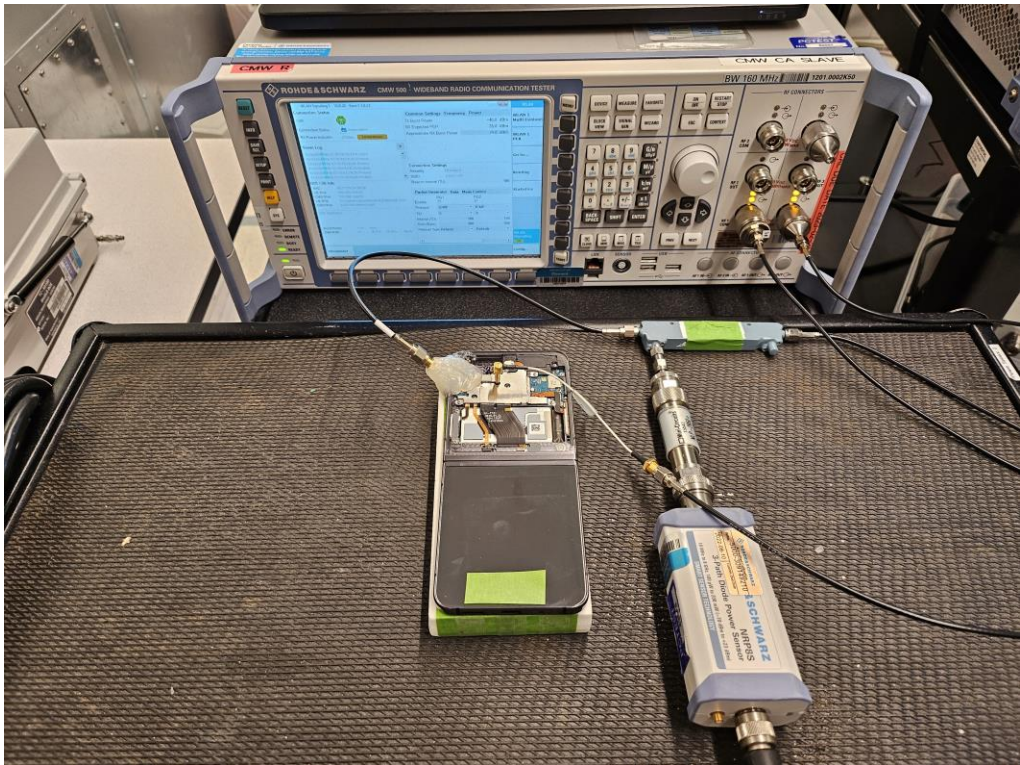
Test Setup Photo 7 – Conducted Test Setup (Figure 6-1d)
