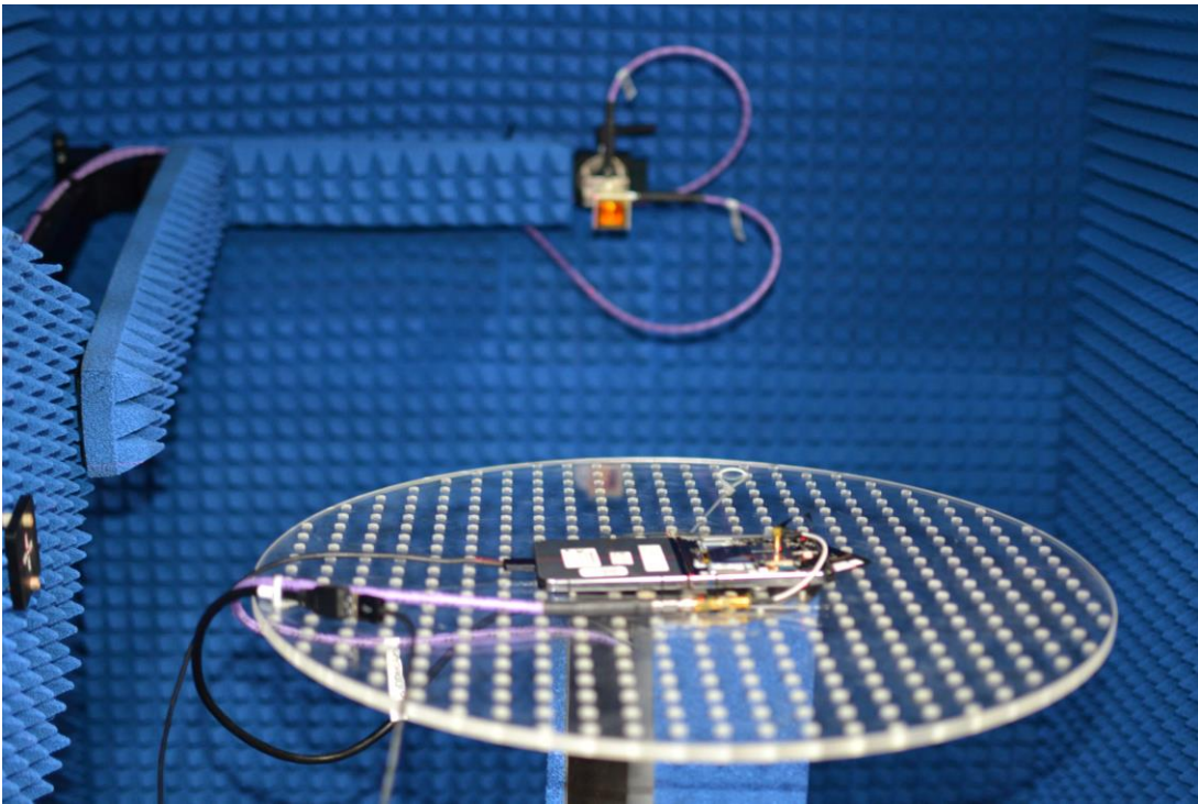
Test Setup Photo 16 – Radiated Power Measurement Setup, Open (Figure 7-1)
