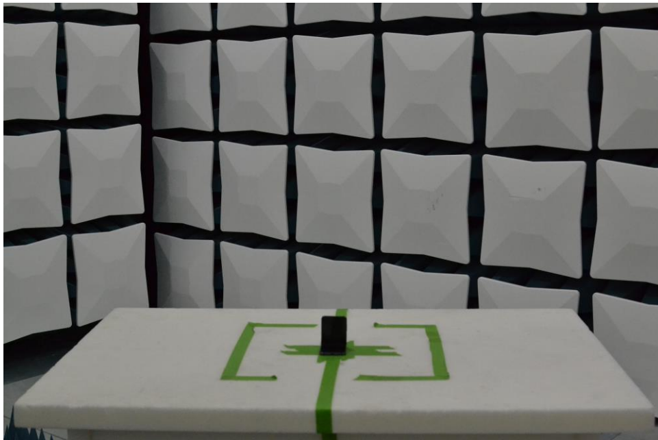
Figure 18. Test Setup – X Position – 30MHz-1GHz – Half
