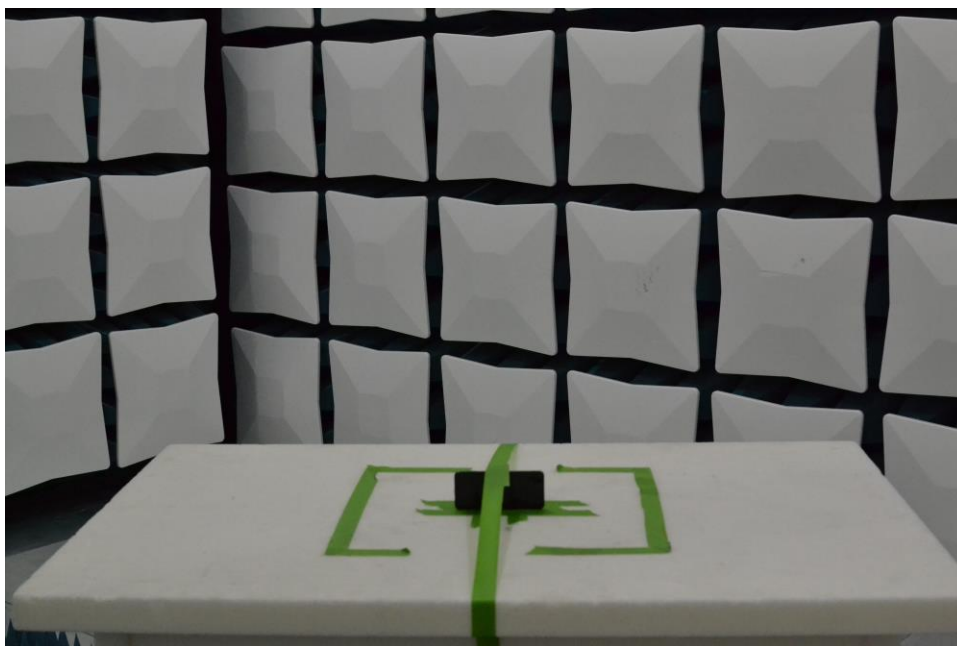
Figure 14. Test Setup – Y Position – 30MHz-1GHz – Open
