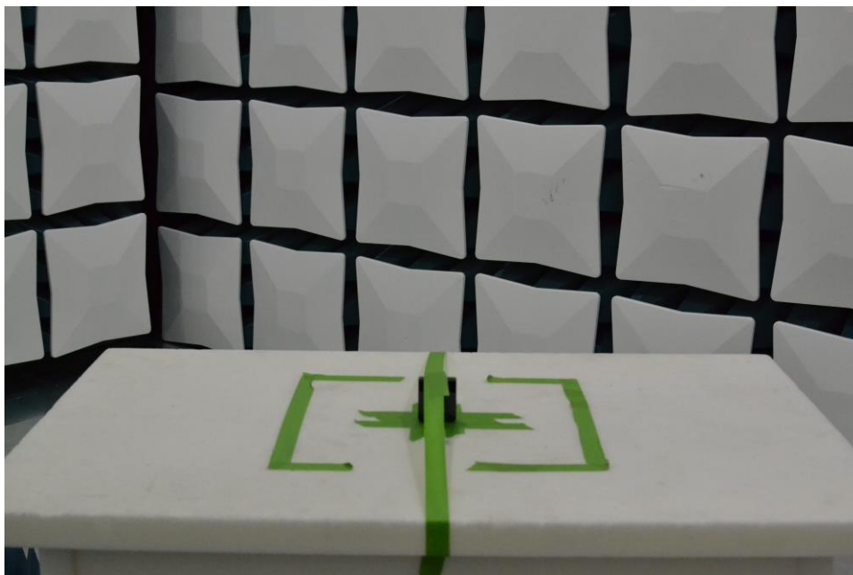
Figure 23. Test Setup – Z Position – 30MHz-1GHz – Closed
