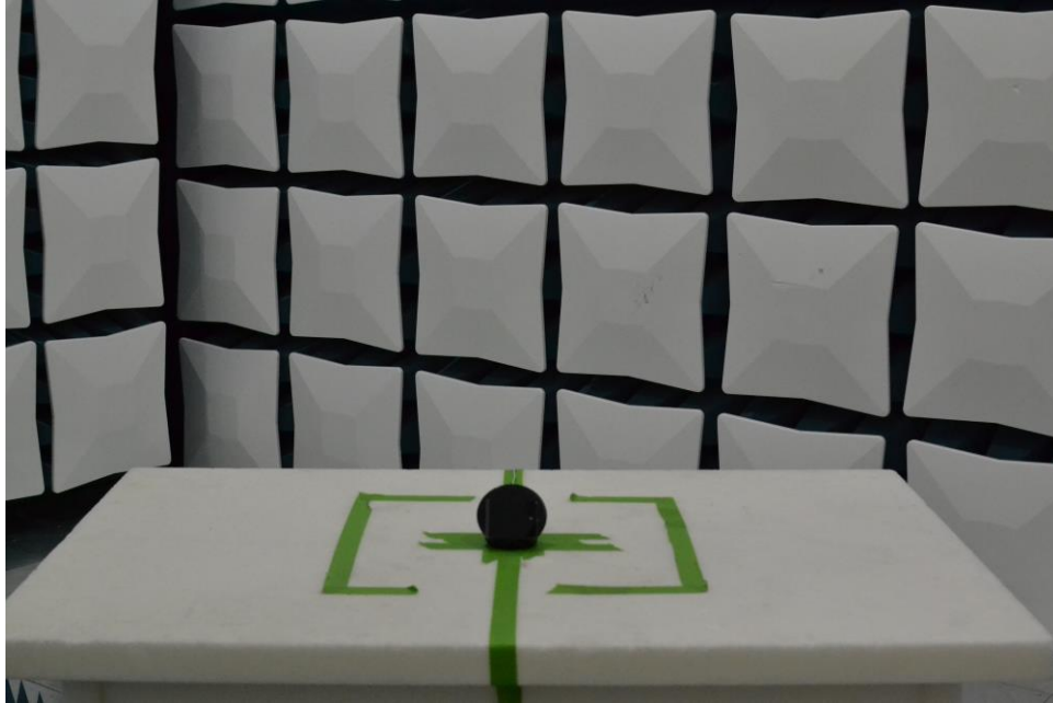
Figure 25. Test Setup – WCP Position – 30MHz-1GHz – Closed
