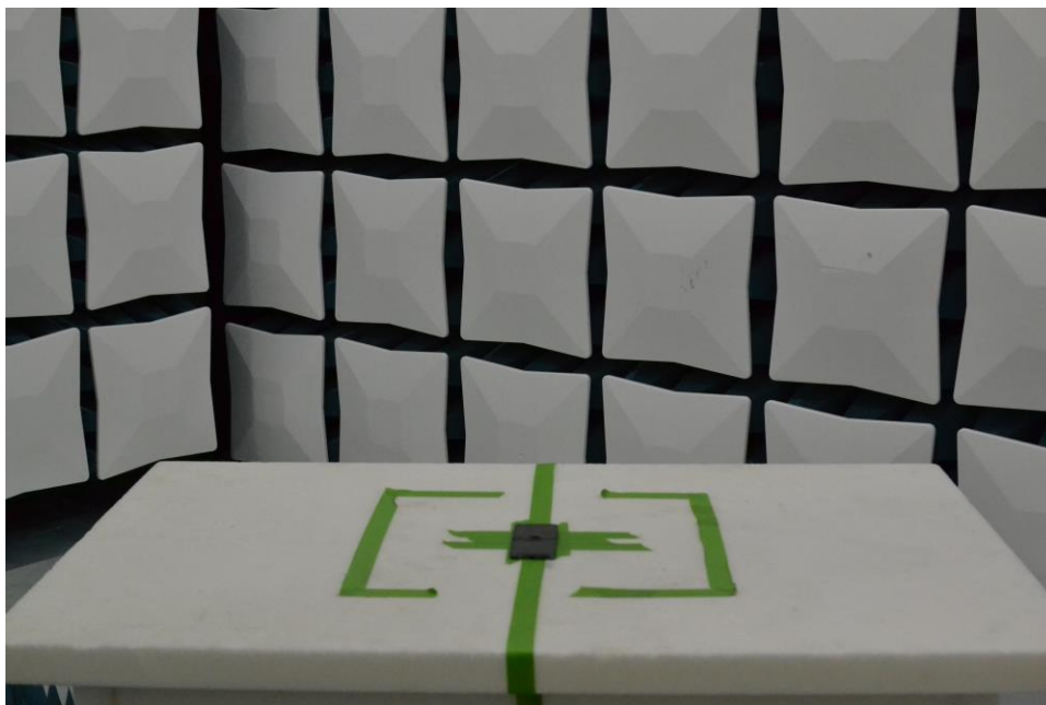
Figure 13. Test Setup – X Position – 30MHz-1GHz – Open
