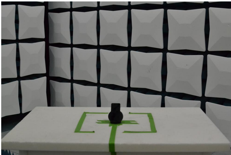
Figure 16. Test Setup – WCP Position – 30MHz-1GHz – Open
