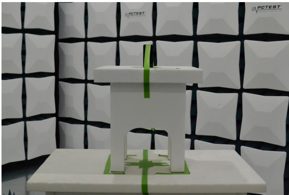
Figure 3. Test Setup – Z Position – 1GHz-18GHz – Open
