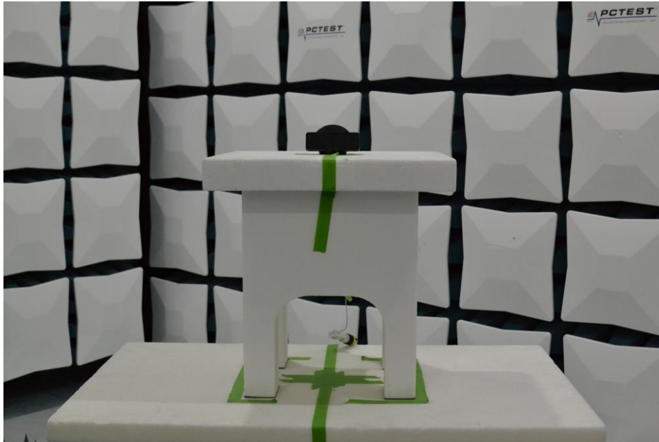
Figure 5. Test Setup – WCP Position – 1GHz-18GHz – Open
