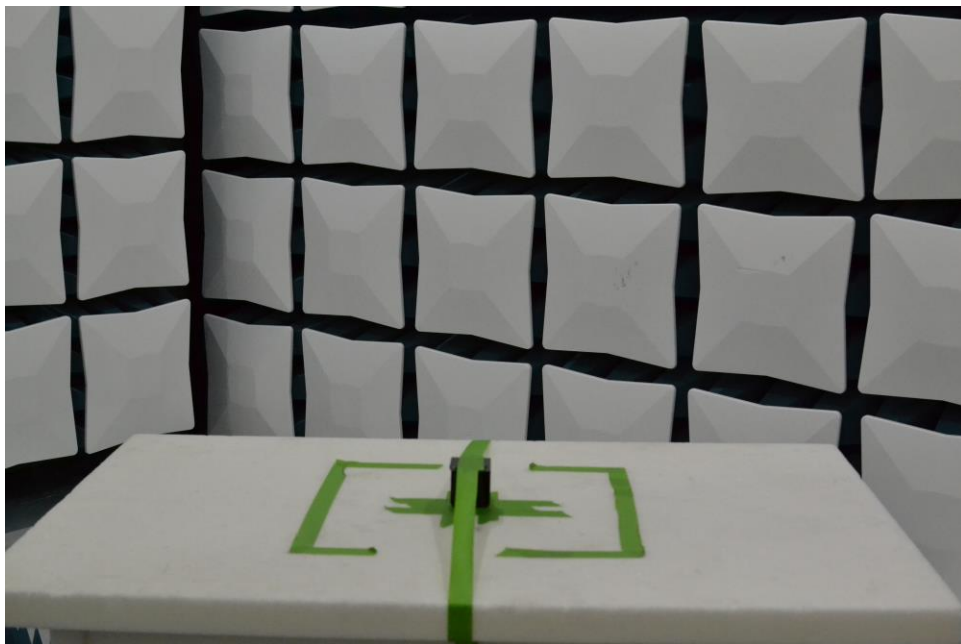
Figure 20. Test Setup – Z Position – 30MHz-1GHz – Half
