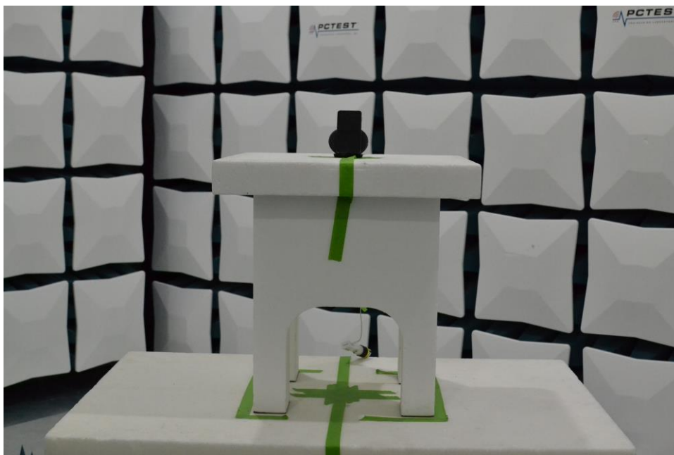
Figure 4. Test Setup – WCP Position – 1GHz-18GHz – Open
