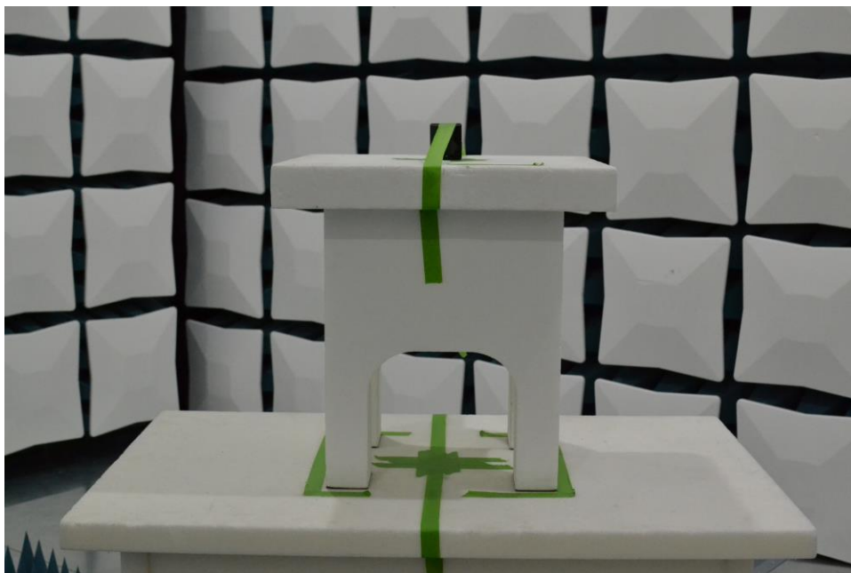
Figure 11. Test Setup – Z Position – 1GHz-18GHz – Closed
