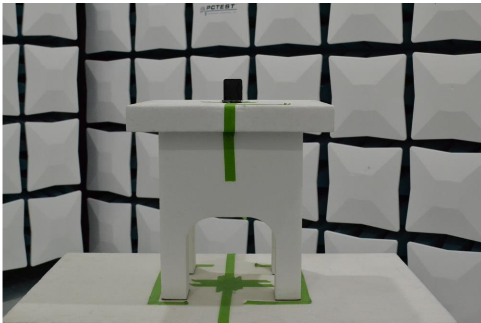
Figure 6. Test Setup – X Position – 1GHz-18GHz – Half
