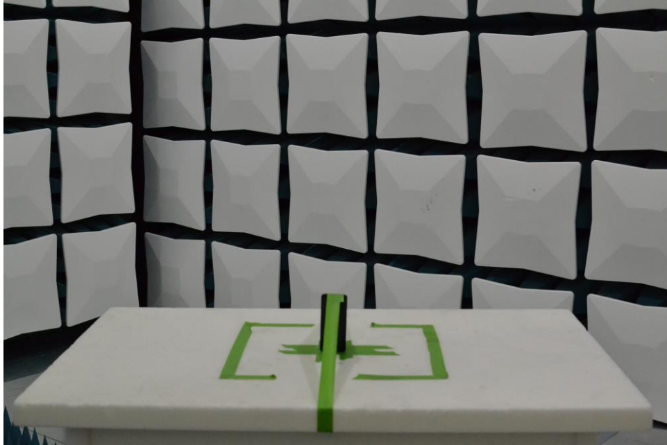
Figure 15. Test Setup – Z Position – 30MHz-1GHz – Open
