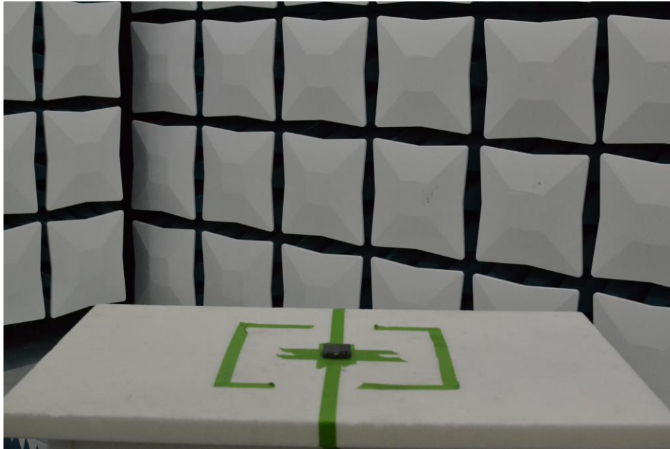
Figure 21. Test Setup – X Position – 30MHz-1GHz – Closed
