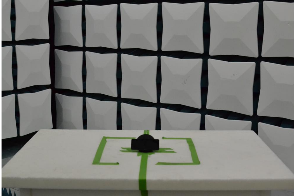
Figure 17. Test Setup – WCP Position – 30MHz-1GHz – Open
