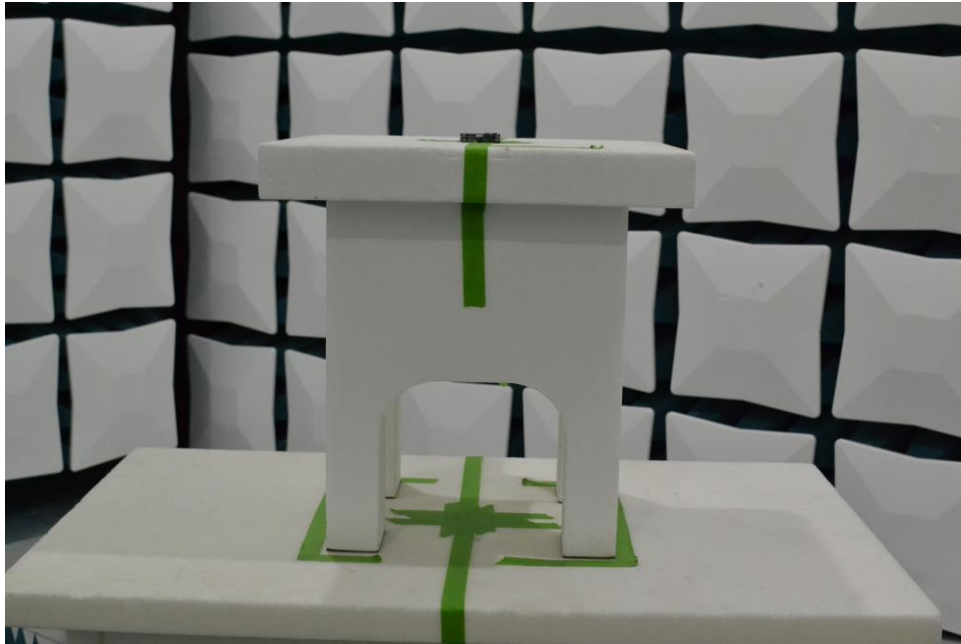
Figure 9. Test Setup – X Position – 1GHz-18GHz – Closed
