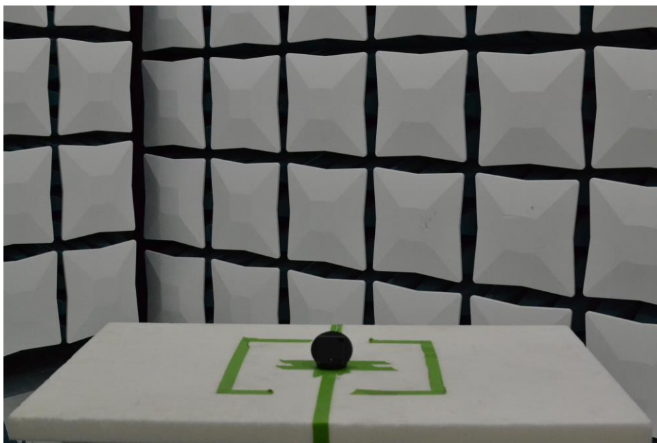
Figure 24. Test Setup – WCP Position – 30MHz-1GHz – Closed
