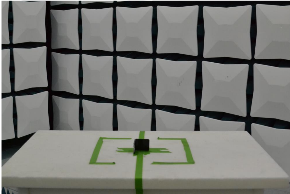
Figure 19. Test Setup – Y Position – 30MHz-1GHz – Half
