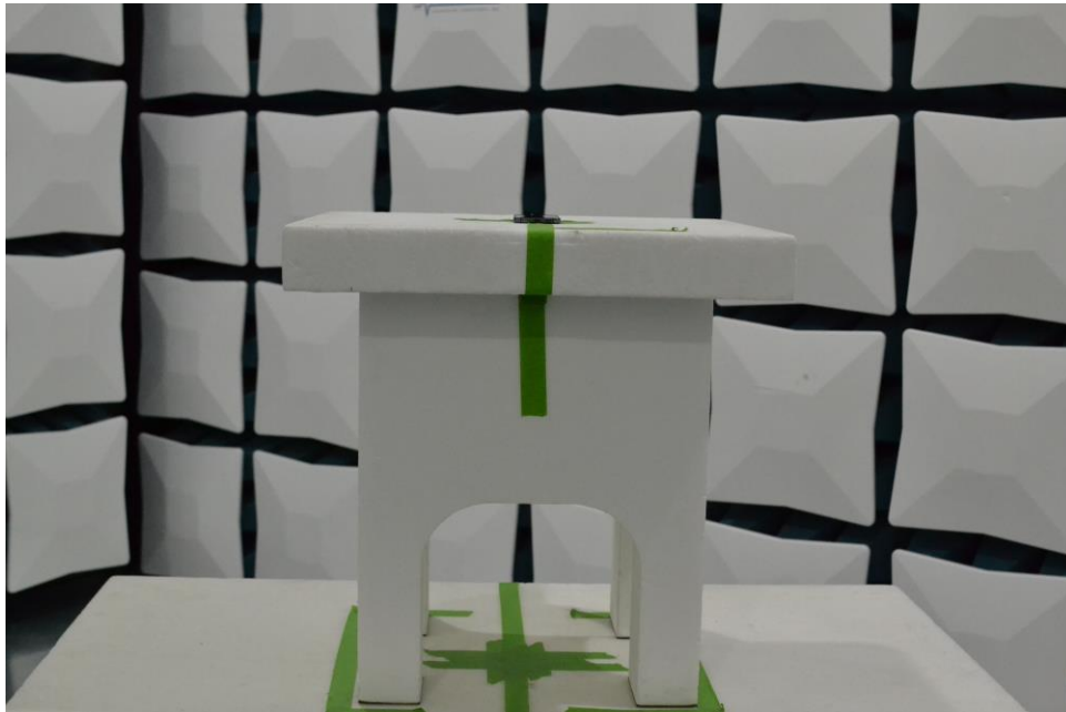
Figure 1. Test Setup – X Position – 1GHz-18GHz – Open
