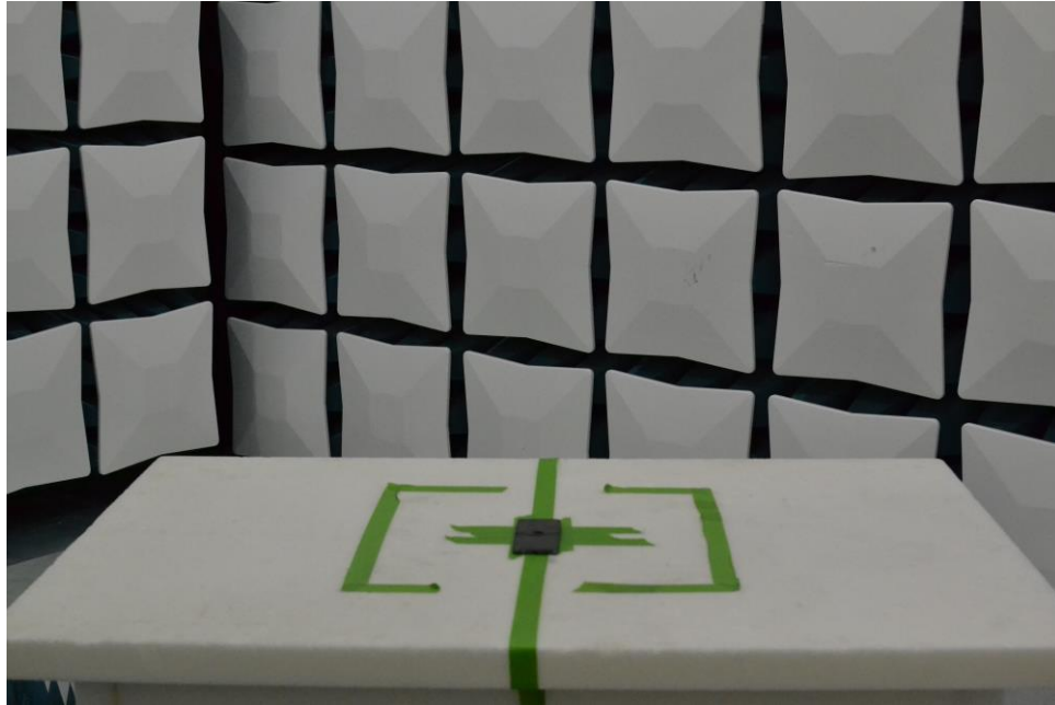
Figure 17. Test Setup – X Position – 30MHz-1GHz – Open
