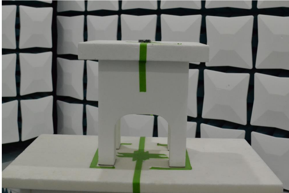
Figure 13. Test Setup – X Position – 1GHz-18GHz – Closed
