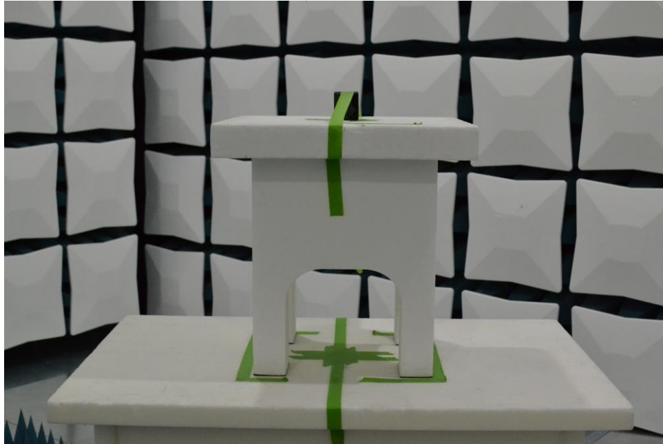
Figure 15. Test Setup – Z Position – 1GHz-18GHz – Closed
