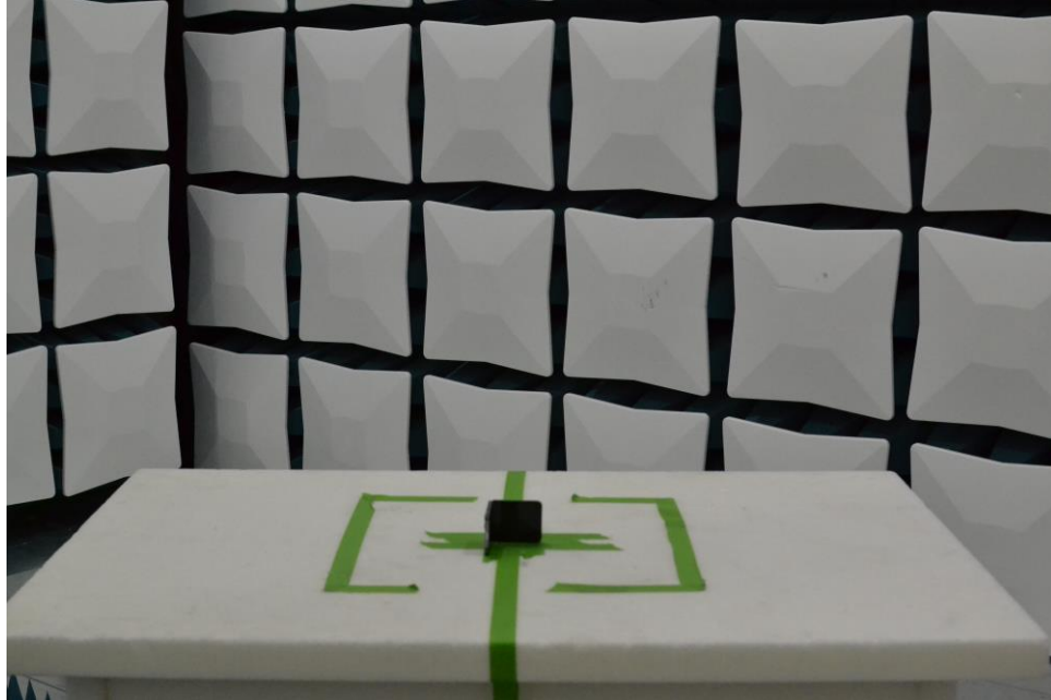
Figure 23. Test Setup – Y Position – 30MHz-1GHz – Half
