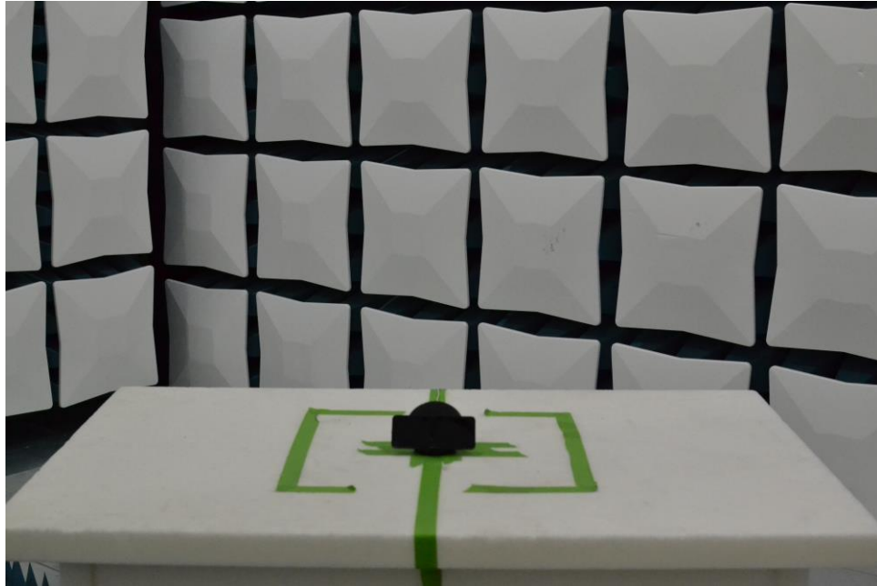
Figure 21. Test Setup – WCP Position – 30MHz-1GHz – Open
