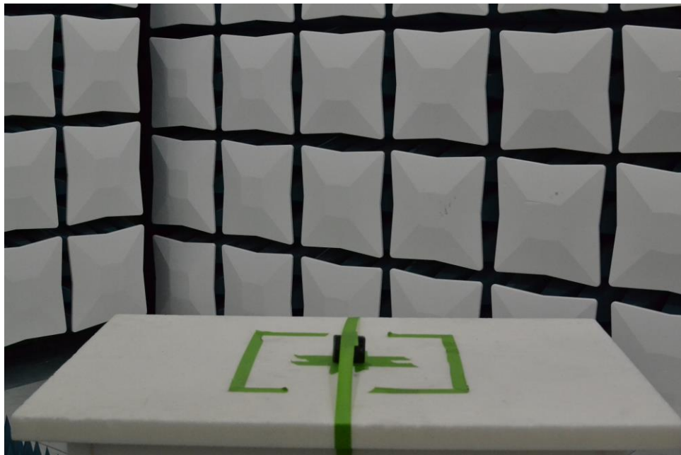
Figure 26. Test Setup – Y Position – 30MHz-1GHz – Closed
