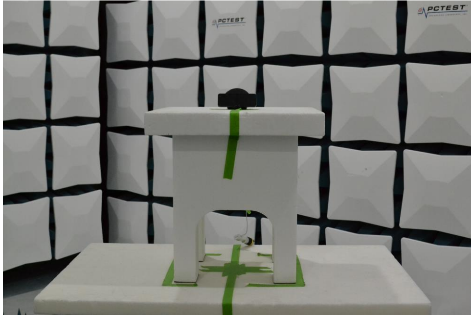
Figure 9. Test Setup – WCP Position – 1GHz-18GHz – Open
