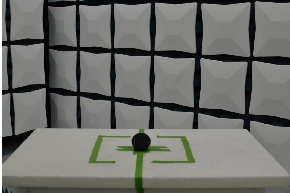
Figure 29. Test Setup – WCP Position – 30MHz-1GHz – Closed
