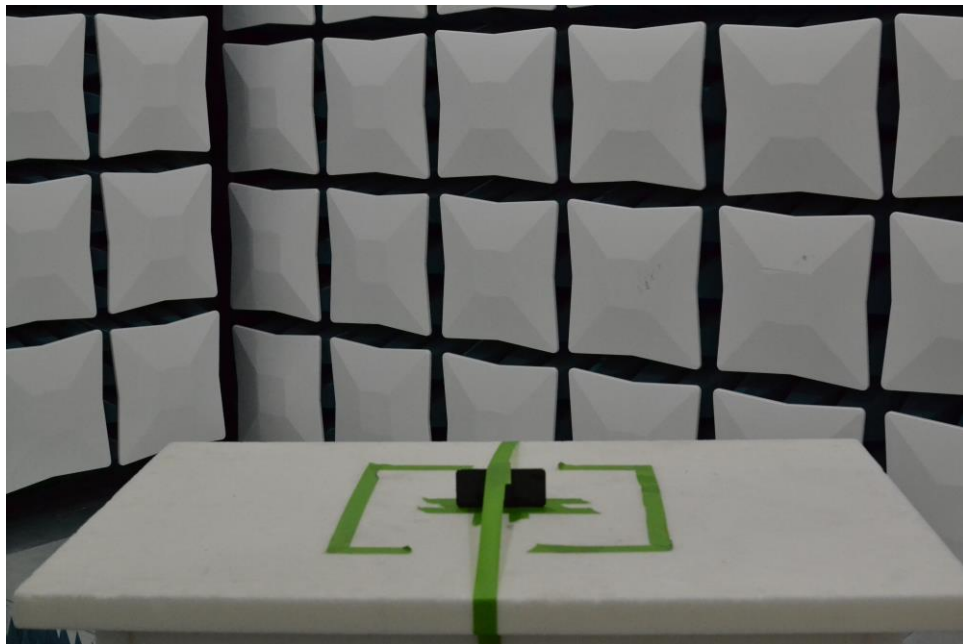
Figure 18. Test Setup – Y Position – 30MHz-1GHz – Open
