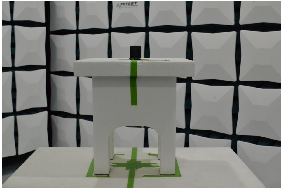
Figure 10. Test Setup – X Position – 1GHz-18GHz – Half
