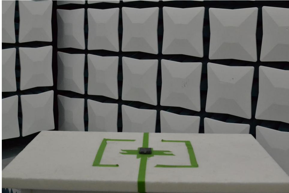
Figure 25. Test Setup – X Position – 30MHz-1GHz – Closed
