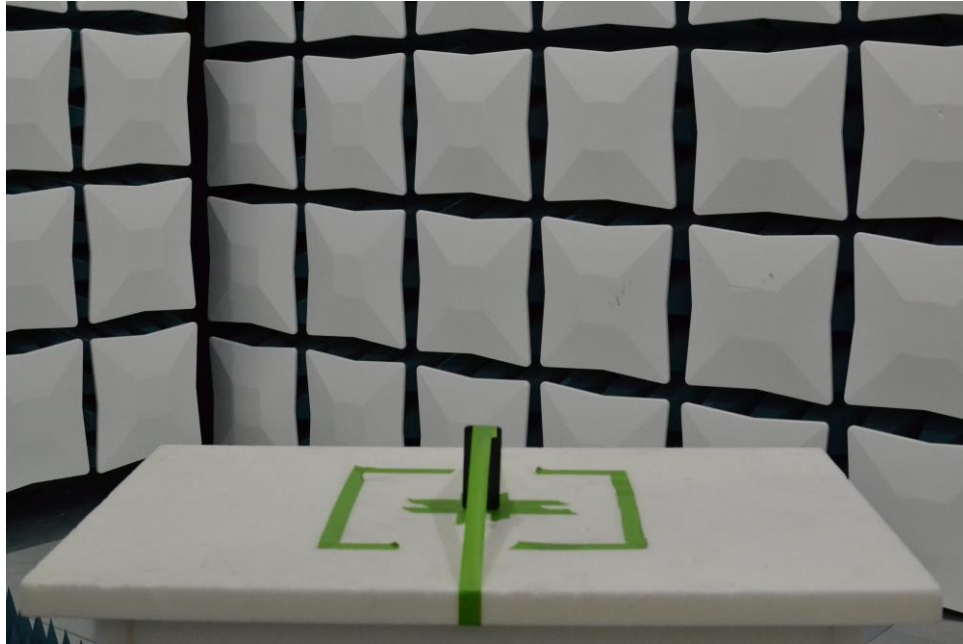
Figure 19. Test Setup – Z Position – 30MHz-1GHz – Open
