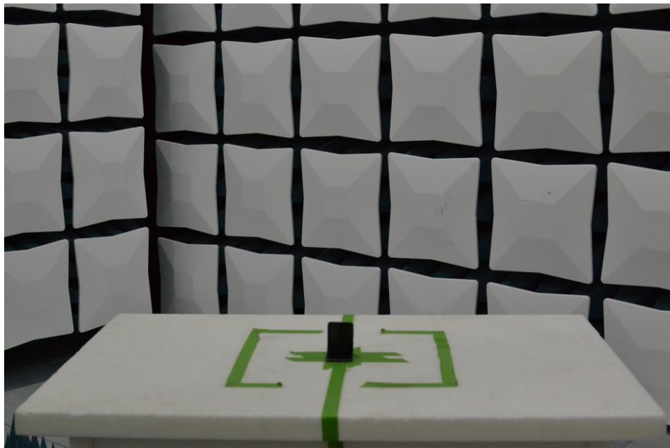
Figure 22. Test Setup – X Position – 30MHz-1GHz – Half
