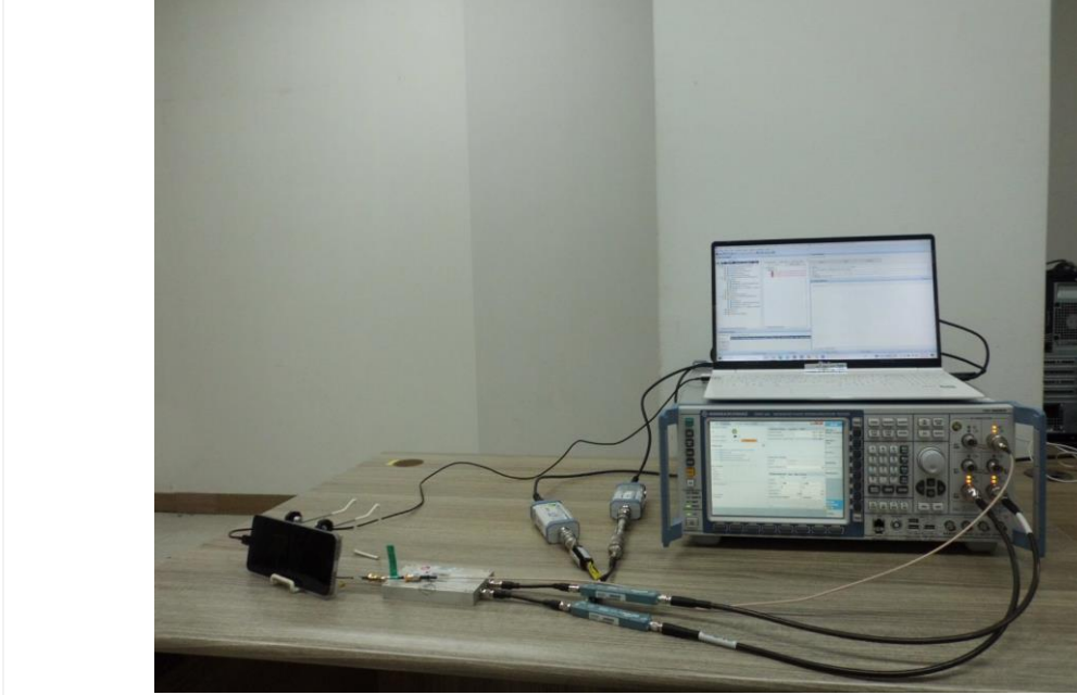
Test setup photo-7 (7-1(e) WLAN DBS)
