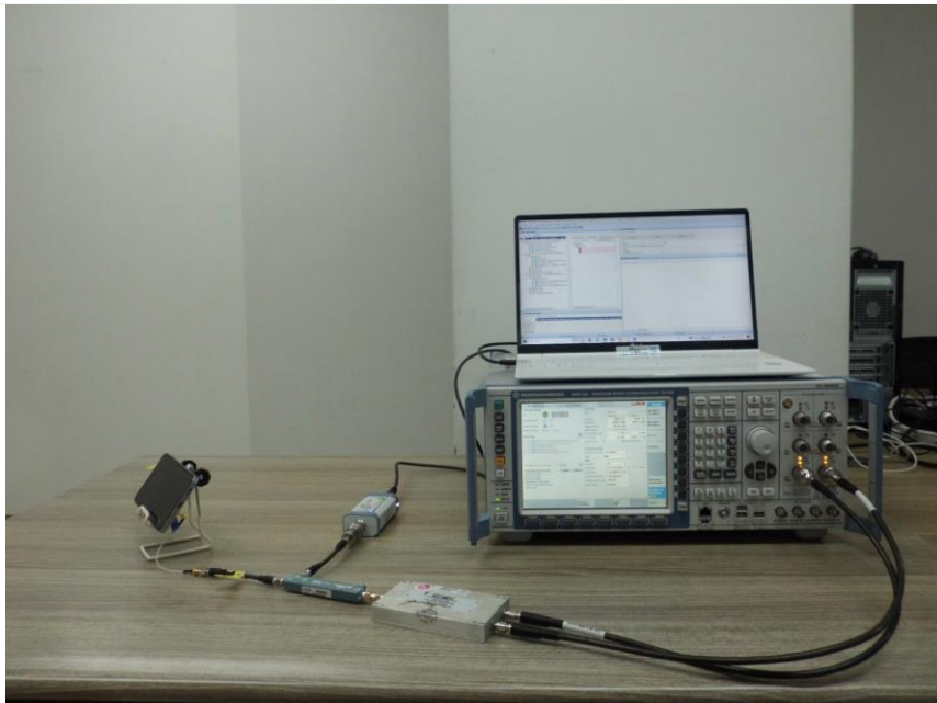
Test setup photo-2 (7-1(b) Legacy)
