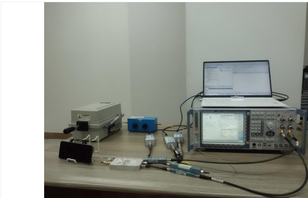
Test setup photo-8 (7-1(f) System level compliance)
