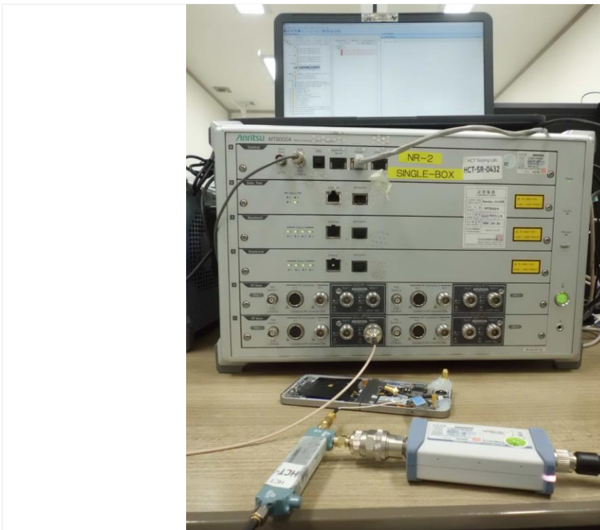
Test setup photo-4 (7-1(a) 5G Sub 6)
