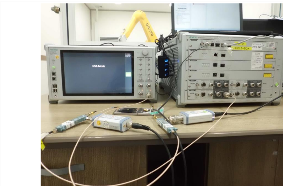
Test setup photo-6 (7-1(c) 5G Sub 6 NSA)
