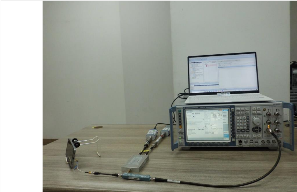
Test setup photo-3 (7-1(c) Legacy)
