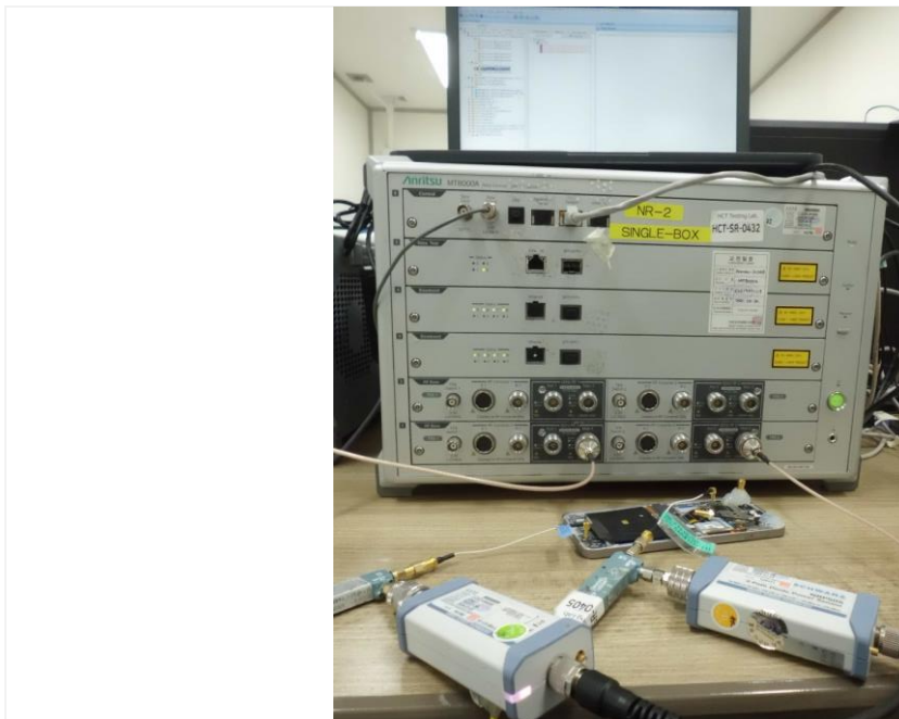
Test setup photo-6 (8-1(c) 5G Sub 6 NRDC)
