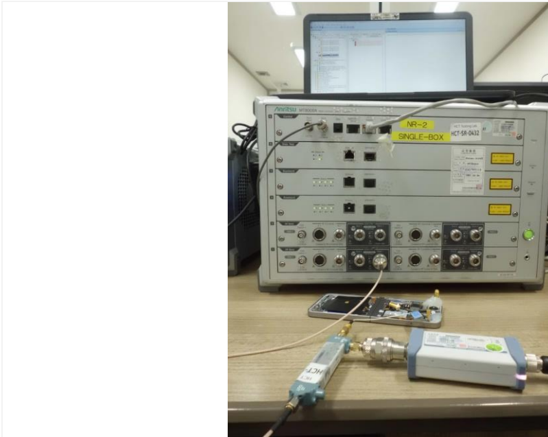
Test setup photo-3 (8-1(a) 5G Sub 6)
