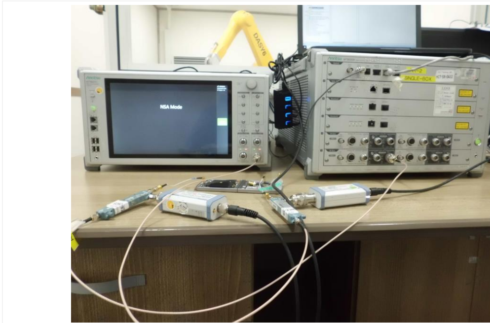
Test setup photo-5 (8-1(c) 5G Sub 6 NSA)
