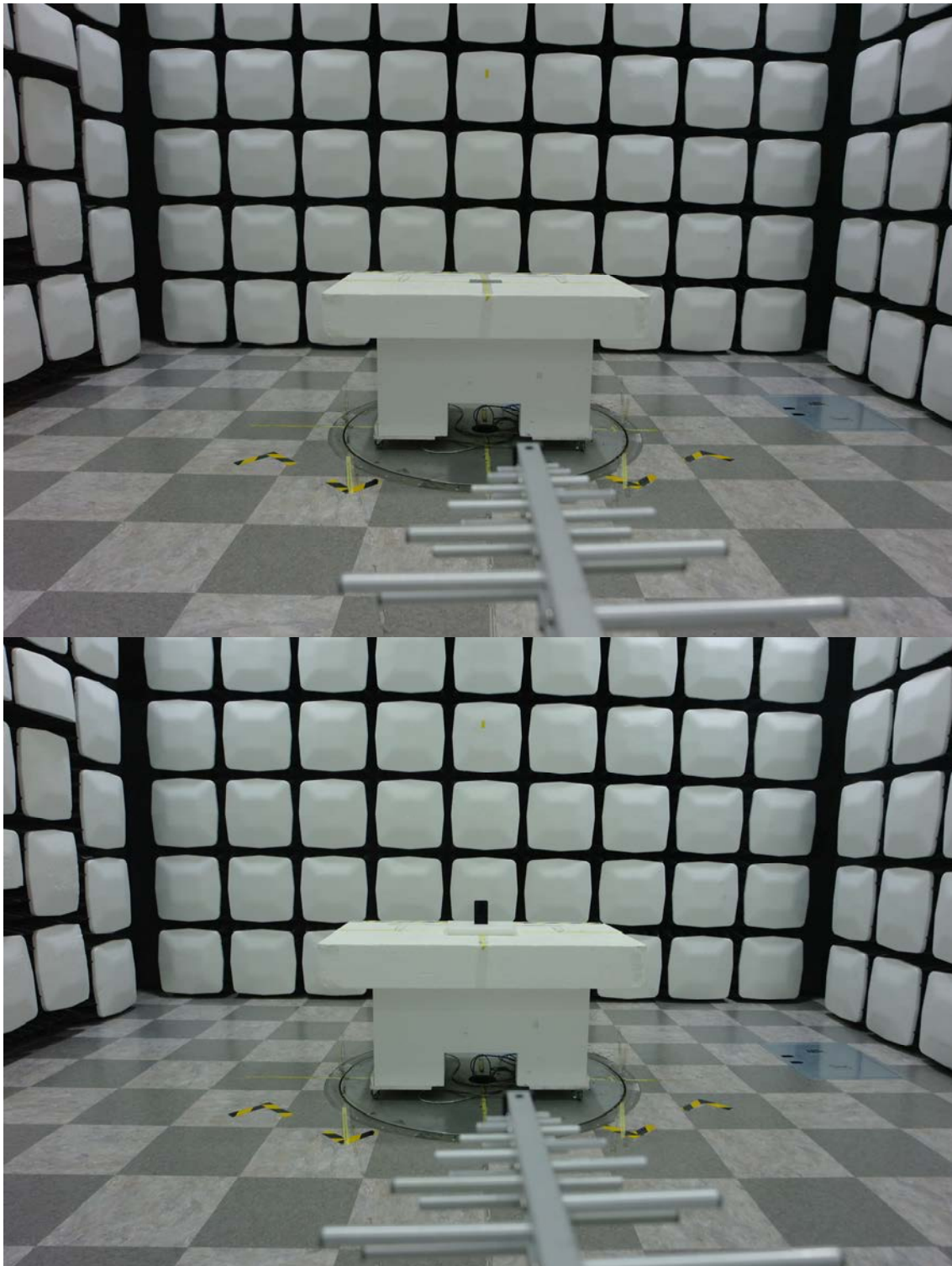
NFC, WPT Radiated Test Setup Photo for below 30 MHz:
