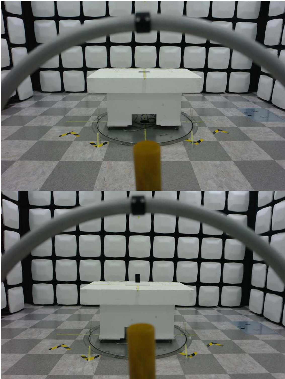
NFC, WPT Radiated Test Setup Photo for 30 MHz ~ 1 GHz :
