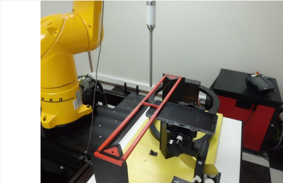
Test setup photo
