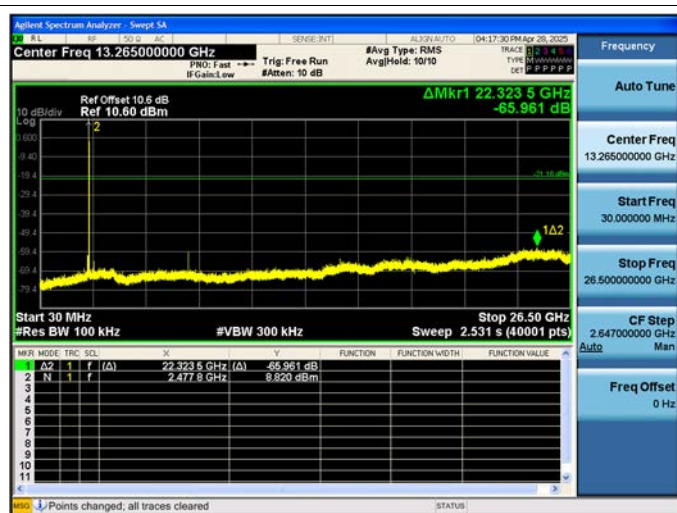
Dual BT Ant. 2 Conducted Spurious Emission
