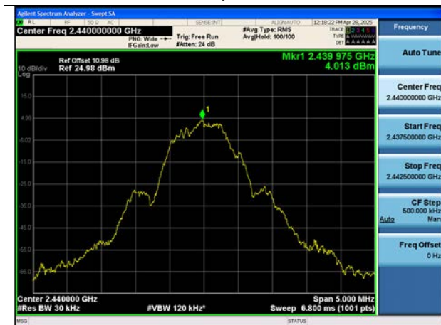
125k Bit/s 255 Byte (Mid-CH 17)
