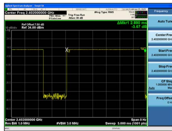
Dual ANT.1 8DPSK : Dwell Time(Ch. 0)
