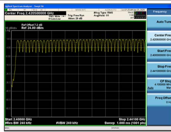
Dual ANT.2 8DPSK (2.4 GHz - 2.441 GHz)
