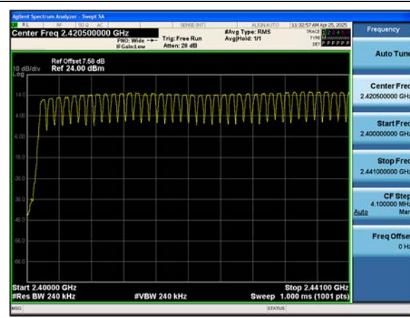
Dual ANT.1 8DPSK (2.4 GHz - 2.441 GHz)
