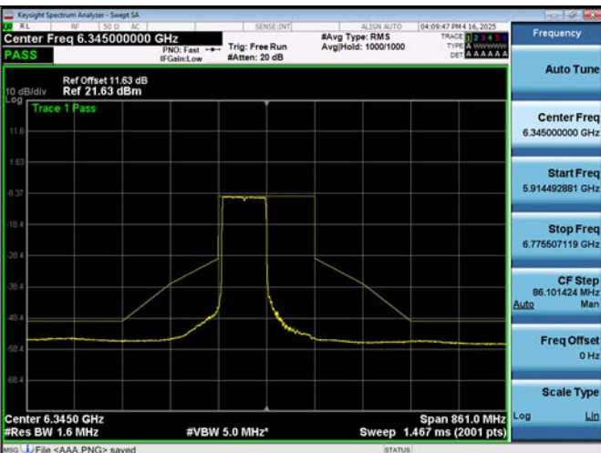
802.11ax HE160M_80L Ch.79(6345 MHz) 996 Tones 67 RU
