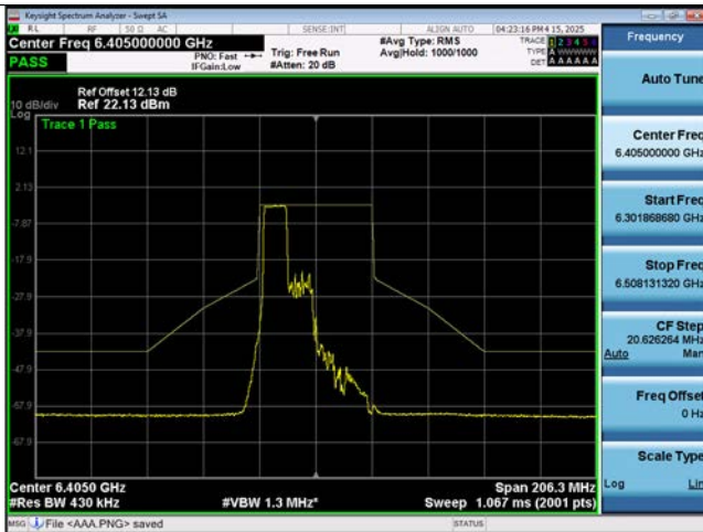
802.11ax HE40M Ch.91(6405 MHz) 484 Tones 65 RU
