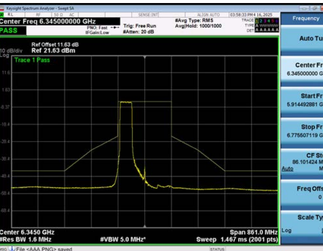
802.11ax HE160M_80L Ch.79(6345 MHz) 484 Tones 65 RU
