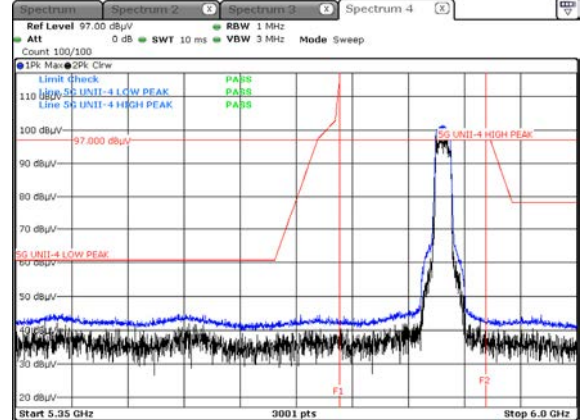
Peak Result (802.11n_HT40, Ch.167, Z-H)
