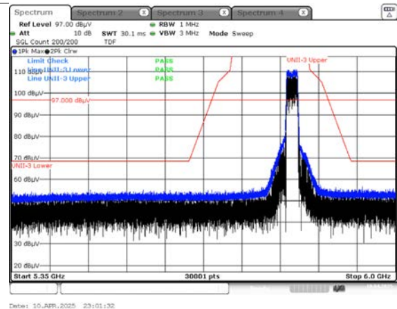
Peak result (802.11ax(HE20) Ch.165, 242T RU 61)
