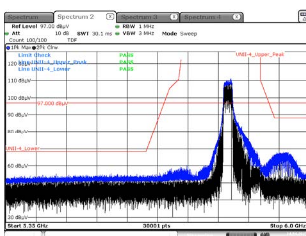
Peak result (802.11ax(HE80) Ch.171, 242T RU 61)
