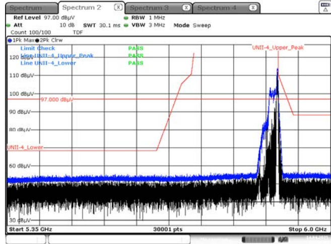
Peak result (802.11ax(HE40) Ch.175, 26T RU 17)
