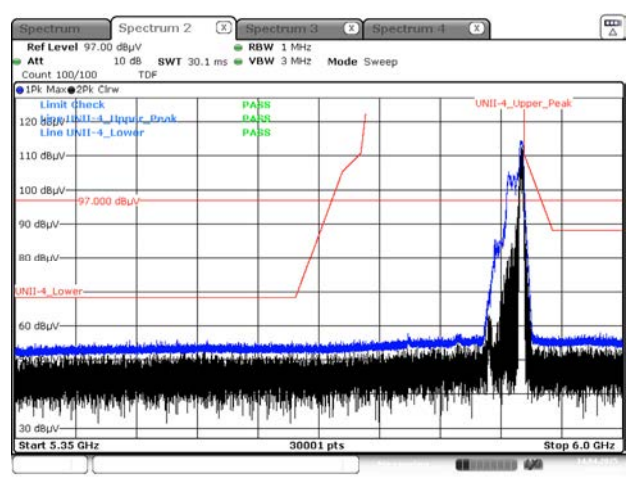
Peak result (802.11ax(HE40) Ch.175, 52T RU 44)
