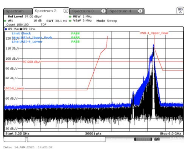
Peak result (802.11ax(HE80) Ch.171, 52T RU 52)
