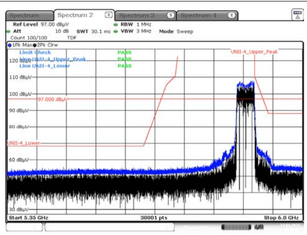
Peak result (802.11ax(HE40) Ch.175, SU)
