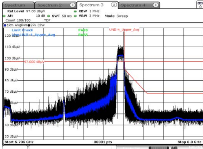
Average result (802.11ax(HE160_80U) Ch.163, 106T RU 60)
