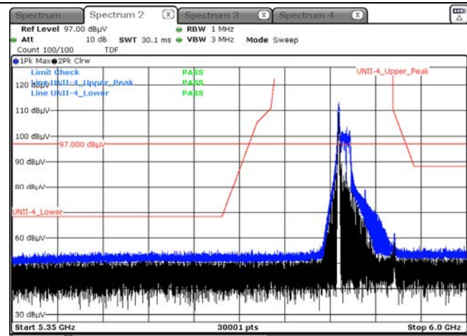
Peak result (802.11ax(HE80) Ch.171, 26T RU 0)
