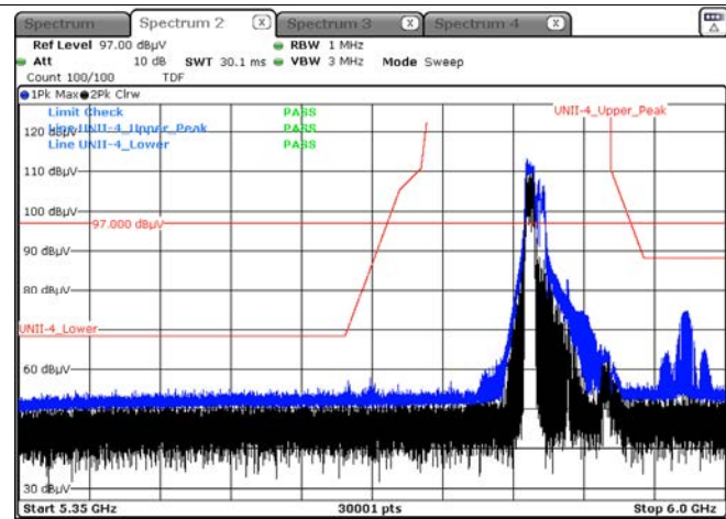
Peak result (802.11ax(HE80) Ch.171, 106T RU 53)
