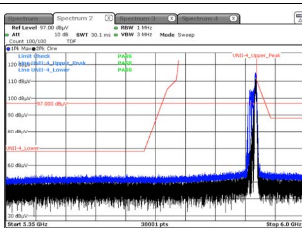
Peak result (802.11ax(HE20) Ch.177, 52T RU 40)
