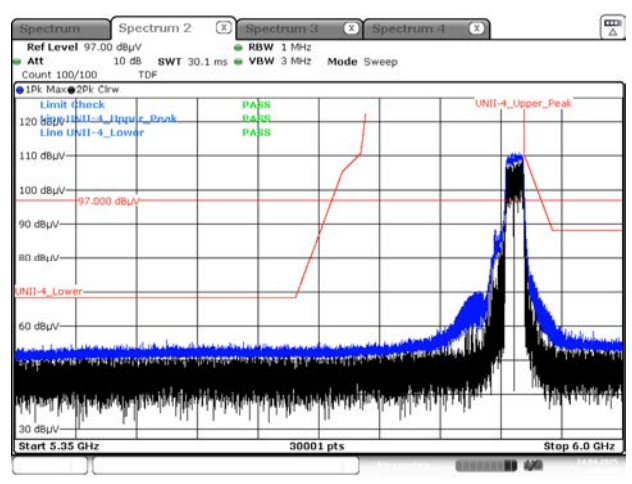
Peak result (802.11ax(HE40) Ch.175, 242T RU 62)
