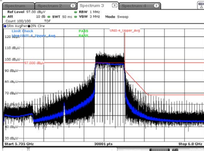
Average result (802.11ax(HE160_80U) Ch.163, 484T RU 66)
