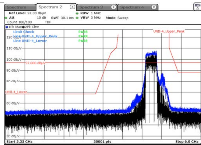
Peak result (802.11ax(HE80) Ch.171, 484T RU 65)
