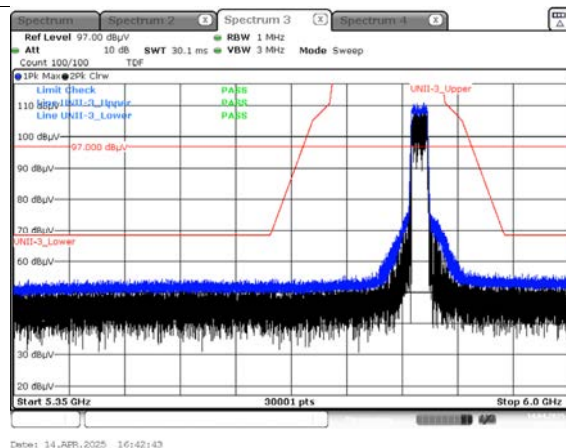
Peak result (802.11ax(HE20) Ch.165, SU)
