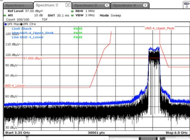
Peak result (802.11ax(HE40) Ch.175, 484T RU 65)
