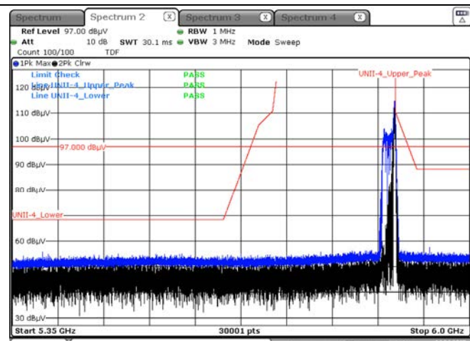
Peak result (802.11ax(HE20) Ch.177, 26T RU 8)
