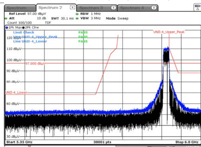
Peak result (802.11ax(HE20) Ch.177, SU)
