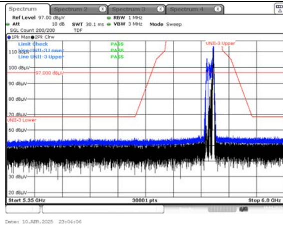
Peak result (802.11ax(HE20) Ch.165, 106T RU 54)
