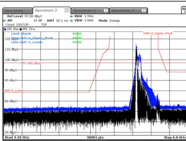
Peak result (802.11ax(HE80) Ch.171, 52T RU 37)
