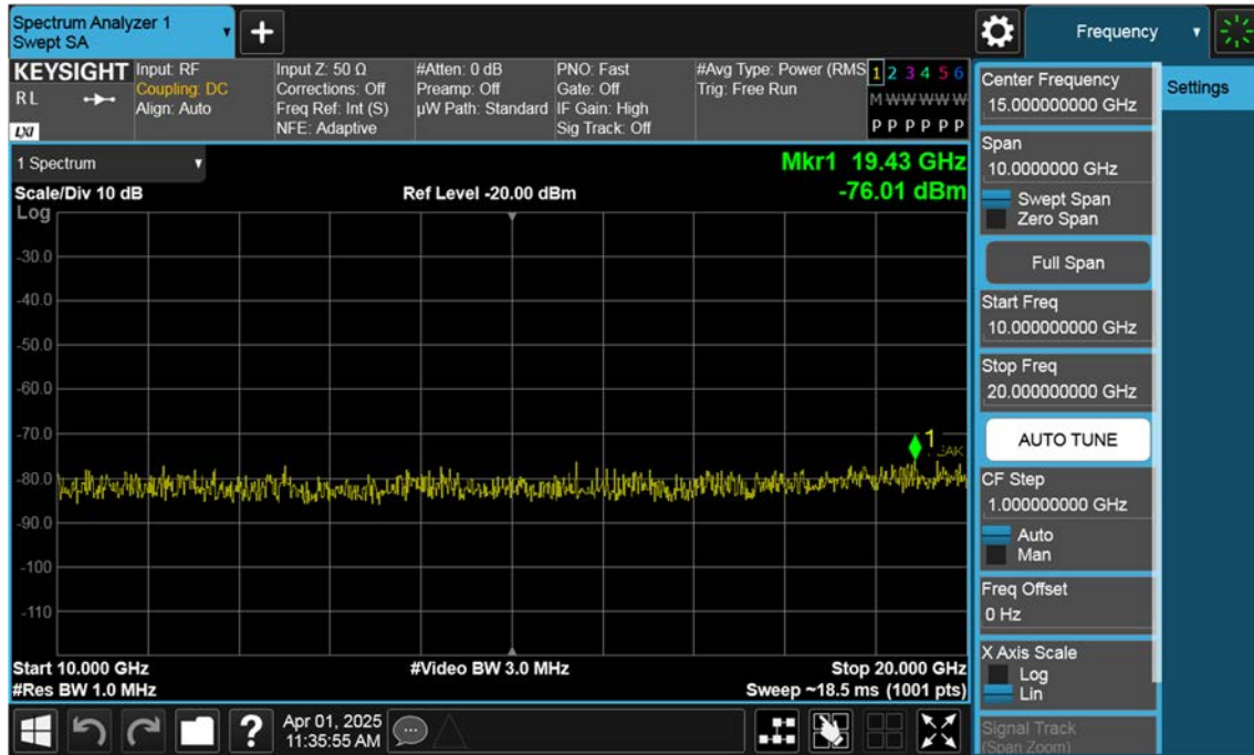
Sub_NR66_10 M_Conducted Spurious(Above10 G)_Low_BPSK_1RB
