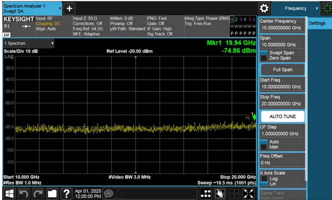
Sub_NR66_15 M_Conducted Spurious(Above10 G)_Low_BPSK_1RB
