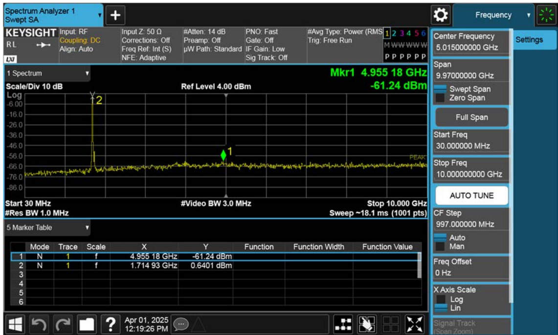
Sub_NR66_25 M_Conducted Spurious(30 M-10 G)_Low_BPSK_1RB
