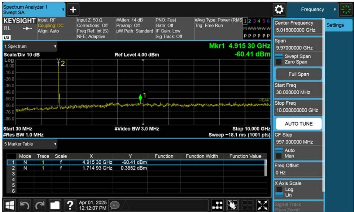
Sub_NR66_20 M_Conducted Spurious(30 M-10 G)_Low_BPSK_1RB
