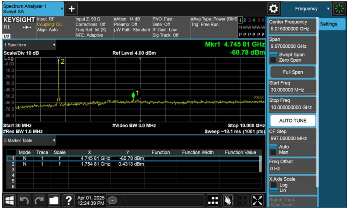
Sub_NR66_25 M_Conducted Spurious(30 M-10 G)_High_BPSK_1RB
