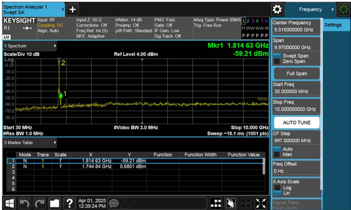
Sub_NR66_35 M_Conducted Spurious(30 M-10 G)_High_BPSK_1RB
