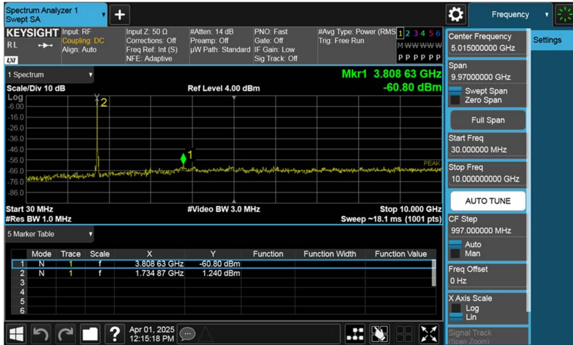
Sub_NR66_20 M_Conducted Spurious(30 M-10 G)_Mid_BPSK_1RB
