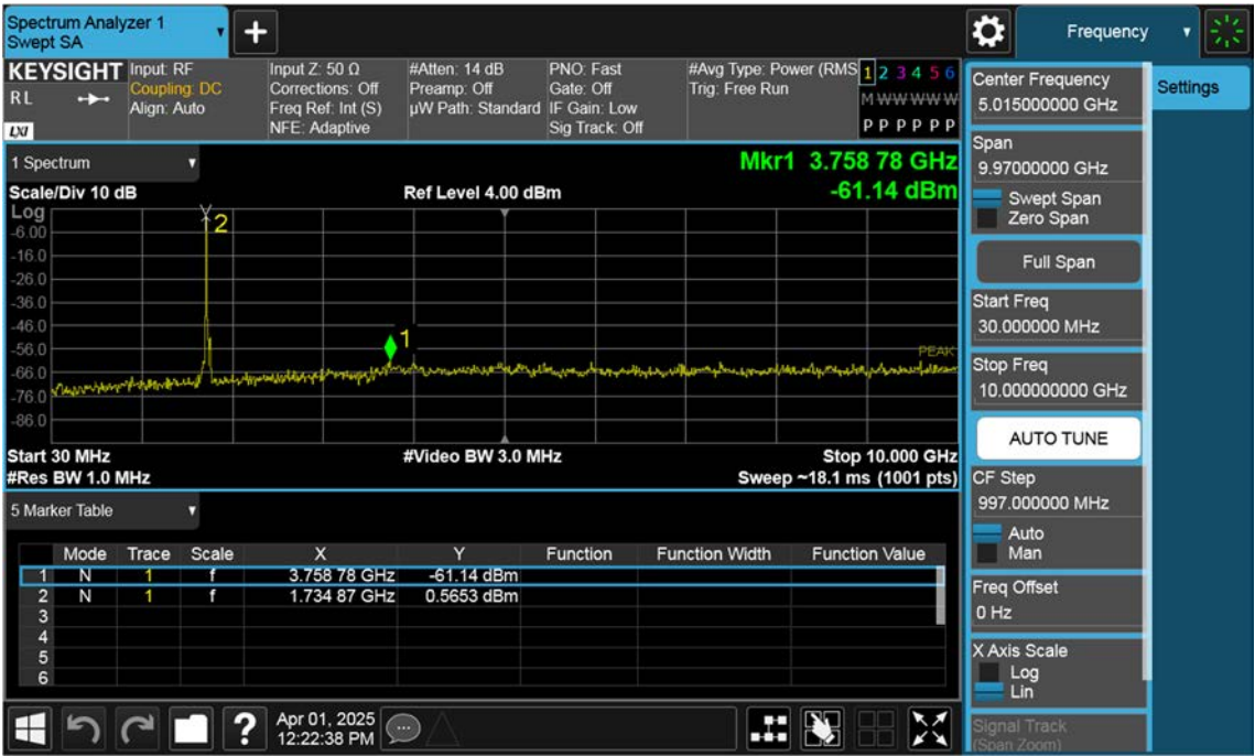
Sub_NR66_25 M_Conducted Spurious(30 M-10 G)_Mid_BPSK_1RB
