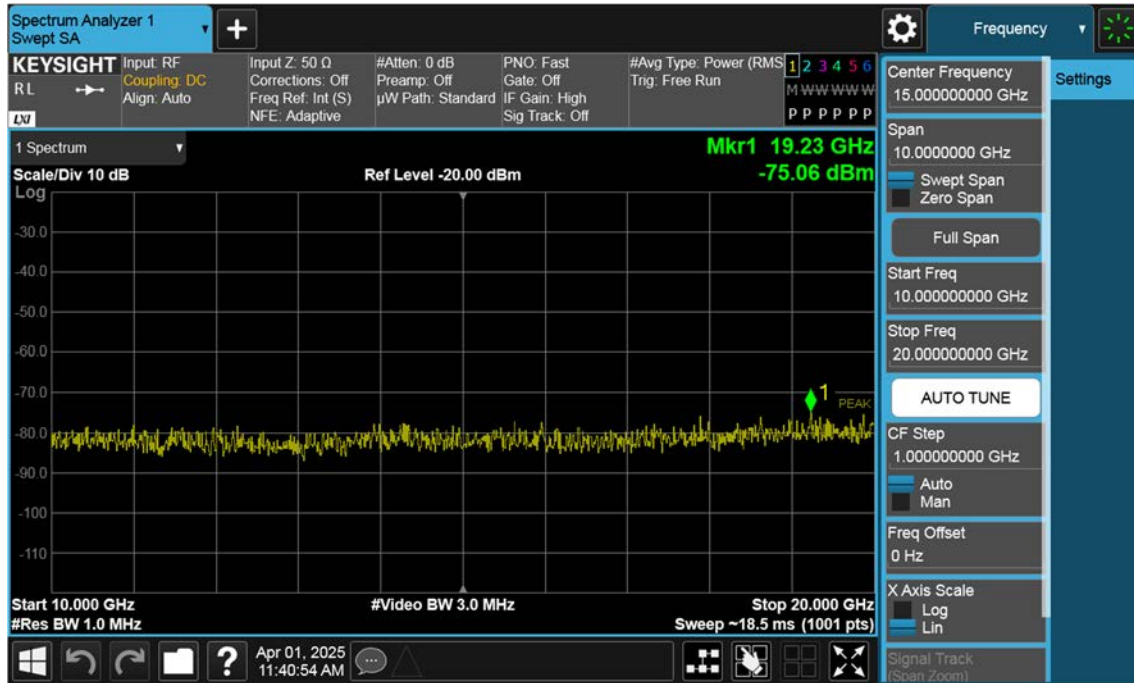
Sub_NR66_10 M_Conducted Spurious(Above10 G)_High_BPSK_1RB
