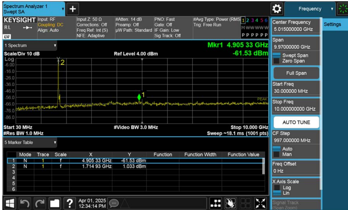
Sub_NR66_35 M_Conducted Spurious(30 M-10 G)_Low_BPSK_1RB
