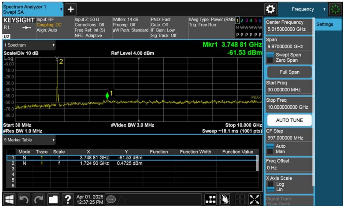
Sub_NR66_35 M_Conducted Spurious(30 M-10 G)_Mid_BPSK_1RB
