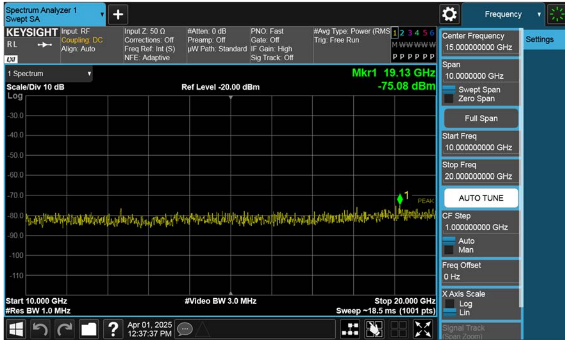
Sub_NR66_35 M_Conducted Spurious(Above10 G)_Mid_BPSK_1RB
