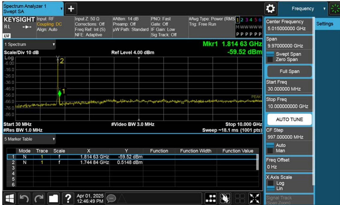
Sub_NR66_40 M_Conducted Spurious(30 M-10 G)_High_BPSK_1RB
