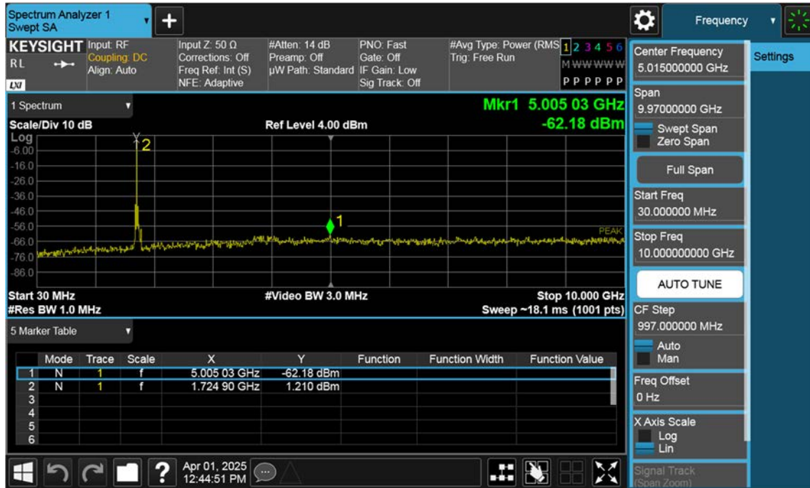
Sub_NR66_40 M_Conducted Spurious(30 M-10 G)_Mid_BPSK_1RB
