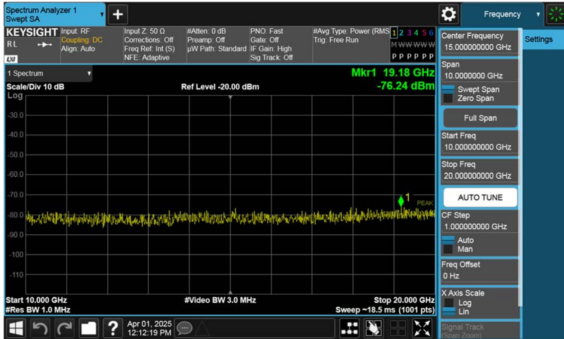
Sub_NR66_20 M_Conducted Spurious(Above10 G)_Low_BPSK_1RB
