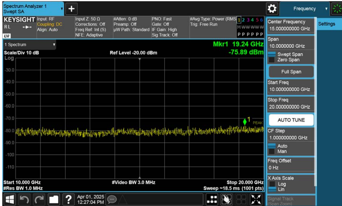
Sub_NR66_30 M_Conducted Spurious(Above10 G)_Low_BPSK_1RB
