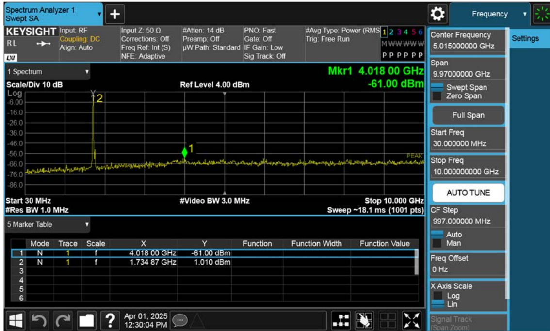
Sub_NR66_30 M_Conducted Spurious(30 M-10 G)_Mid_BPSK_1RB
