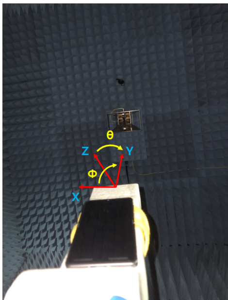
Figure 1: Geometry for SM-F761B for Radiation patterns.
