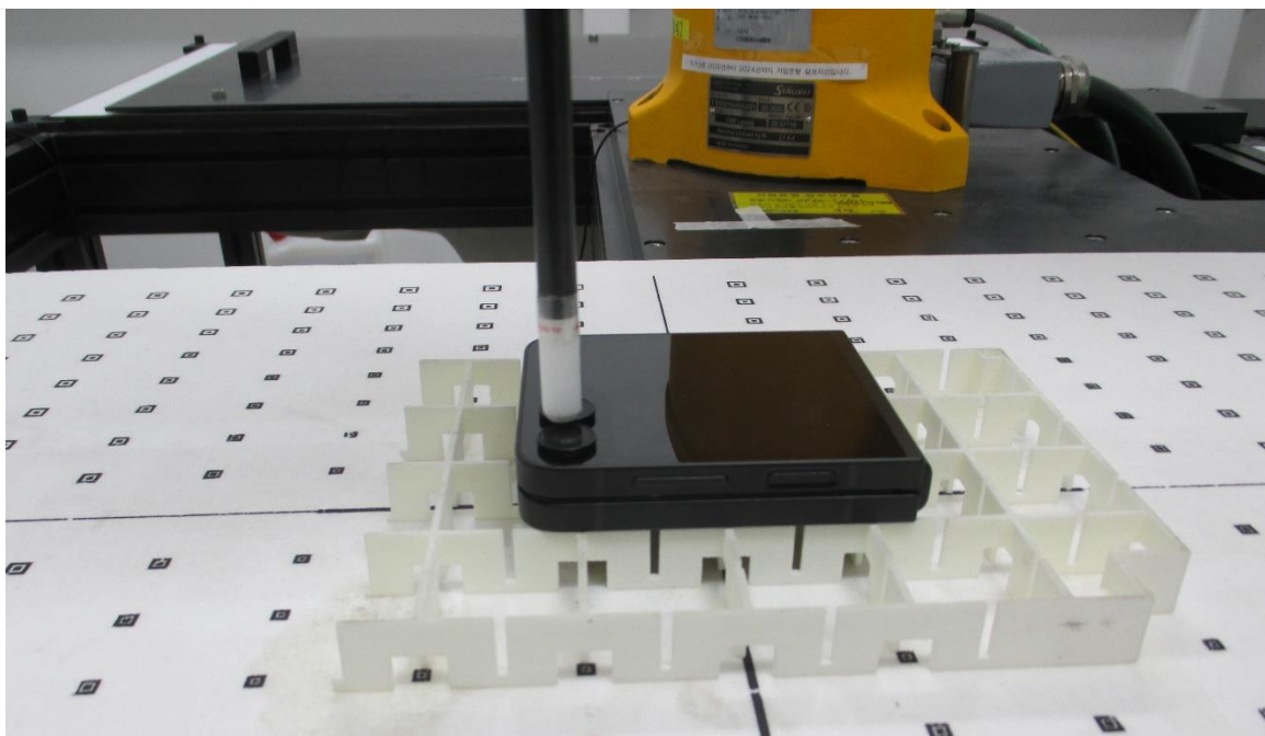
Distance of 2 mm from the EUT
