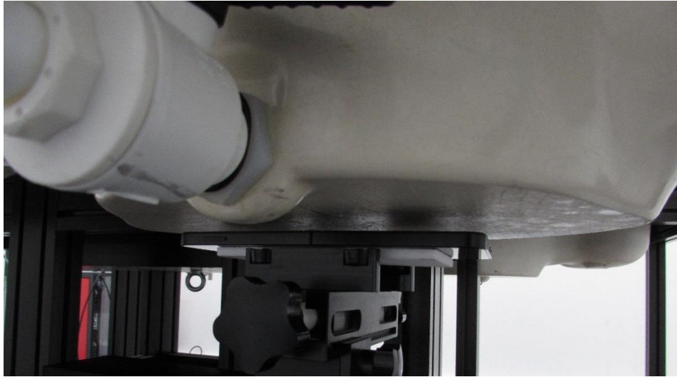
Distance of 5 mm from the EUT
