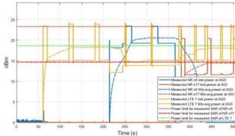
Figure 11.4-1 Conducted Transmitted power for LTE B7(AG0) and NR n5(AG0), n77(AG1) in Test TC14
