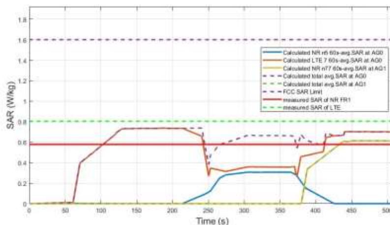
Figure 11.4-2 Total time-averaged SAR in TC3
