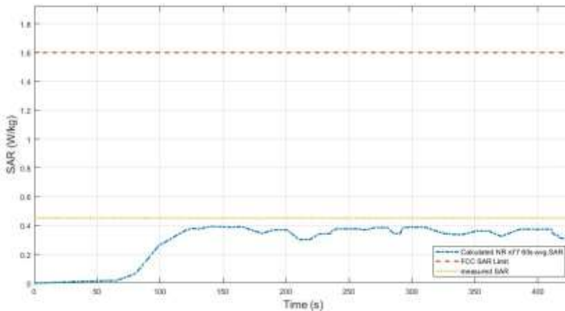
Figure 11.3-4 Total time-averaged SAR in TC02
