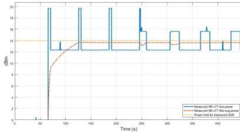
Figure 11.3-1 Time average conducted power of NR n77 in TC01
