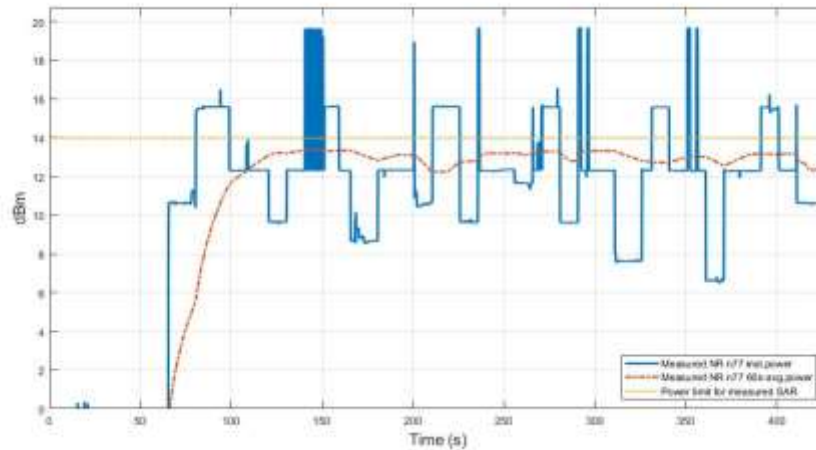
Figure 11.3-3 Conducted Tx power of NR n77 in TC02
