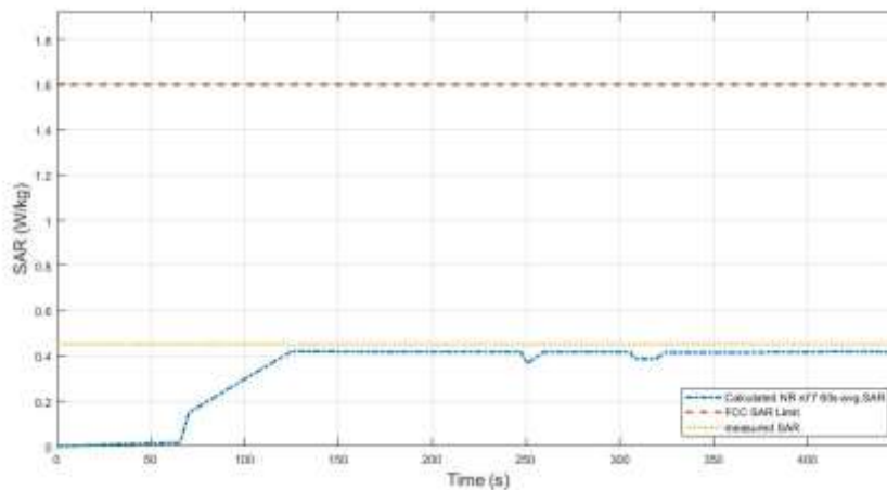
Figure 11.3-2 Total time-averaged SAR in TC01
