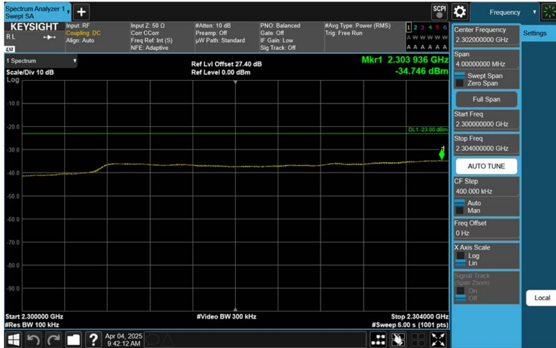
LTE B30_5 M_Band Edge(2300MHz-2304MHz)_Low_QPSK_FullRB
