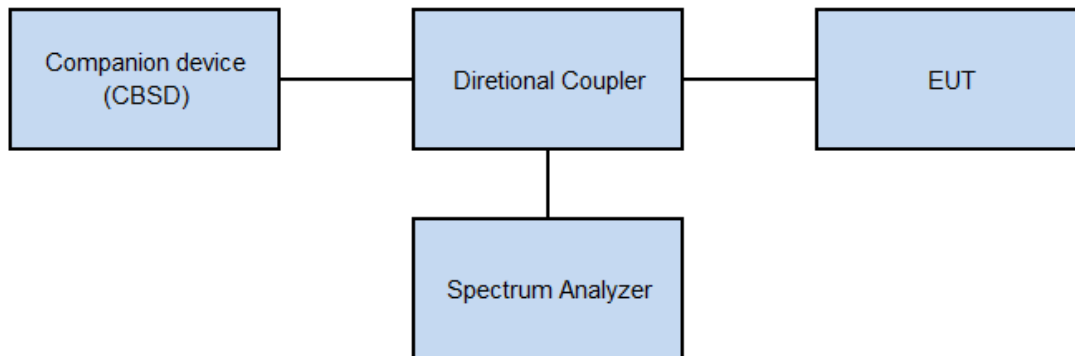
Test setup
